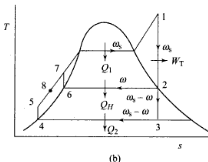
Fig. 2.35 Cogeneration plant with a pass-out turbine
