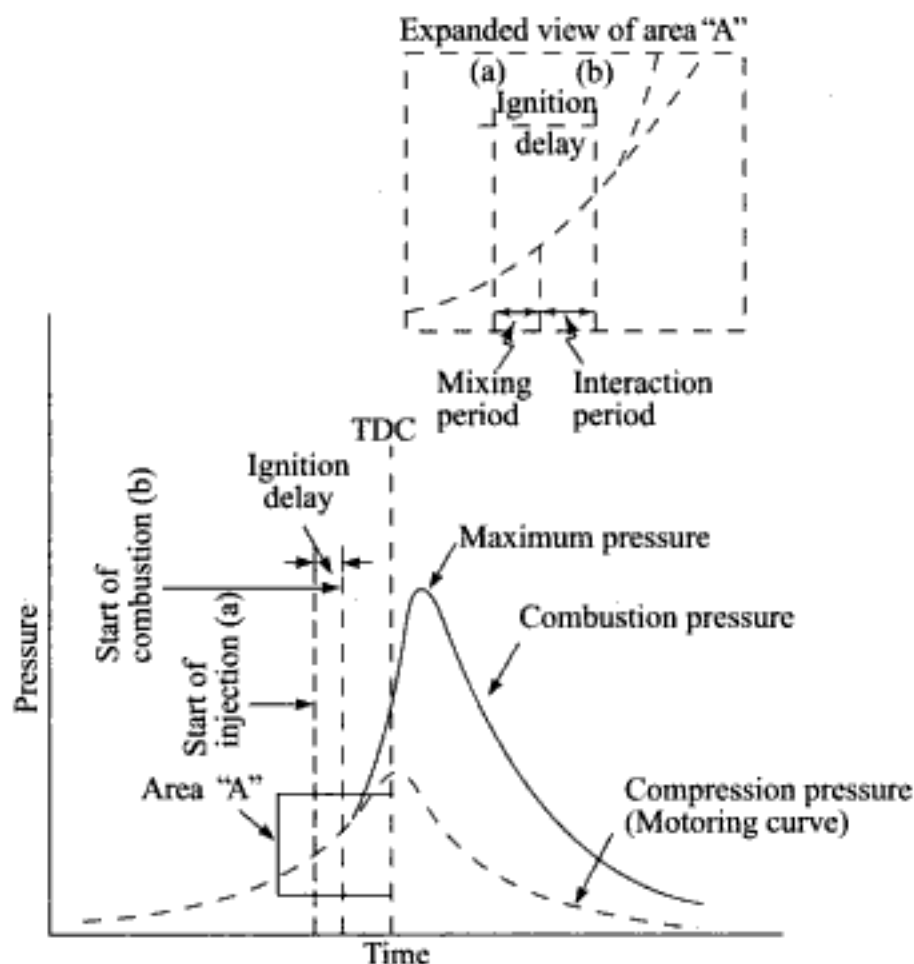
Fig. 11.19 Pressure-time diagram illustrating ignition delay in a CI engine
