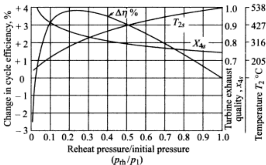
Fig. 2.16 Effect of reheat-to-initial pressure ratio on cycle efficiency, h.p. turbine exit temperature and l.p. turbine exhaust quality with initial steam at 172 bar, 538 °C and steam reheat to 538 °C
