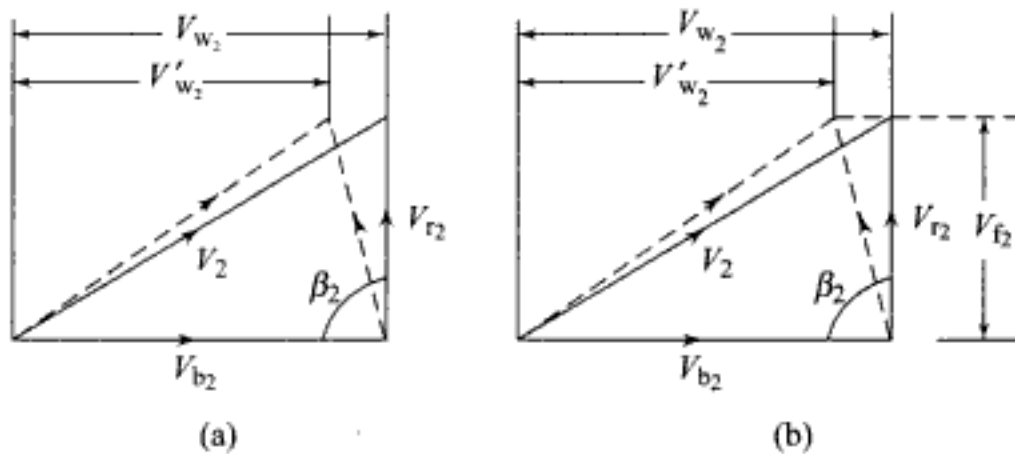
Fig. 11.57 Blade velocity diagrams at blade outlet of a centrifugal compressor for (a) Radially inclined and (b) Backward inclined blading
