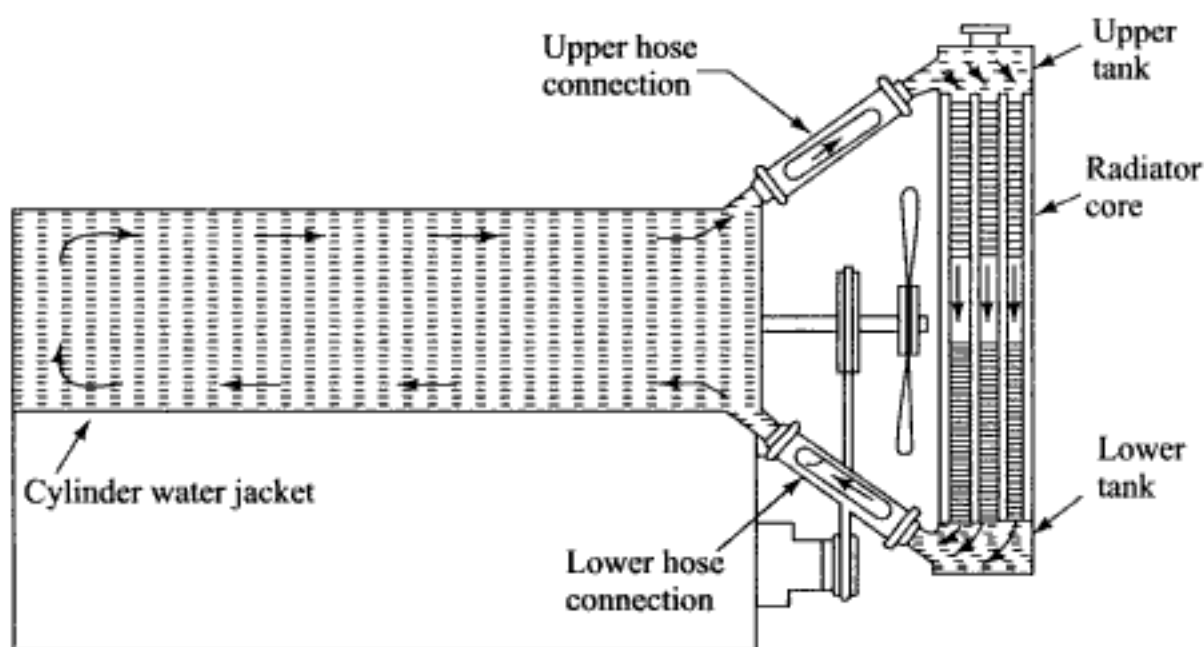
Fig. 11.11 Thermosiphon cooling
