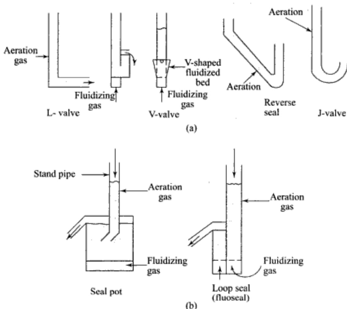
Fig. 6.52 Non-mechanical valves: (a) controllable, (b) automatic
