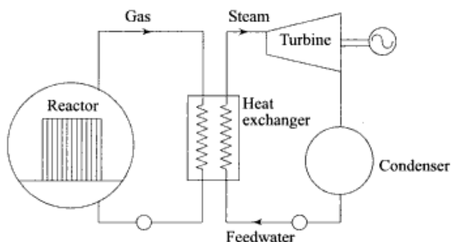
Fig. 9.22 Schematic of a gas-cooled reactor plant
