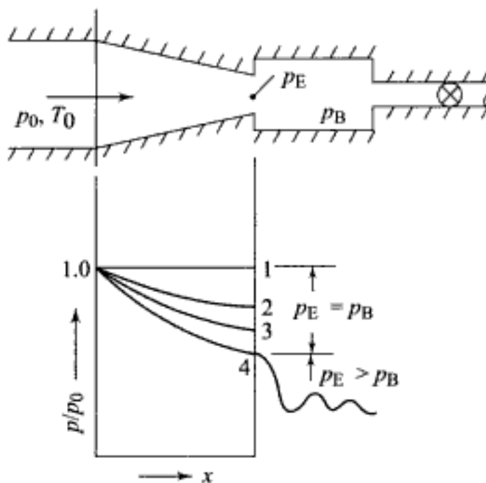
Fig. 7.11 Pressure distribution in a convergent nozzle
