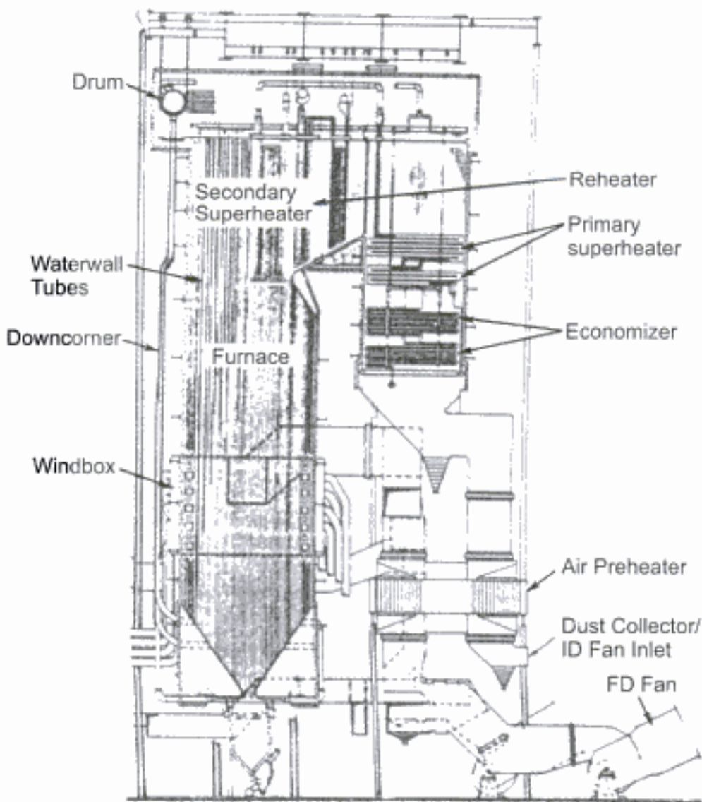
Fig. 6.20 (a) General arrangement of a modern water-tube steam generator
