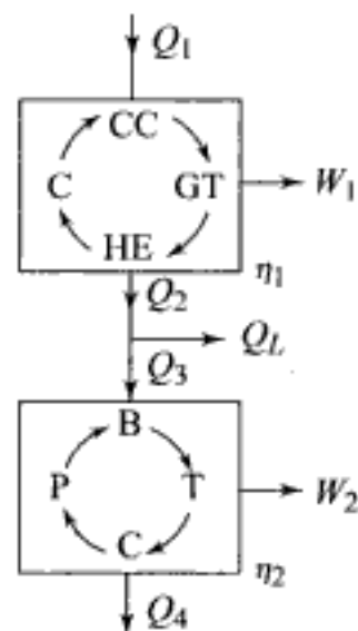
Fig. 3.8 Heat loss in between two plants in series
