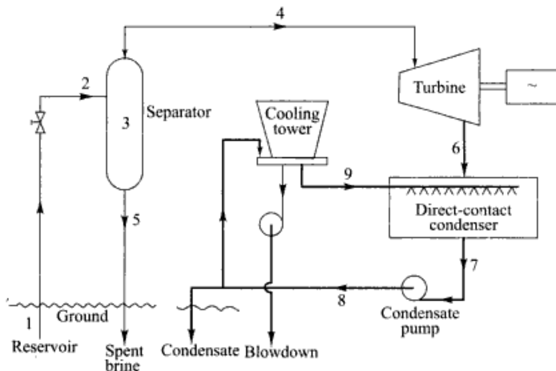
Fig. 14.34 Schematic of a liquid-dominated single-flash steam system
