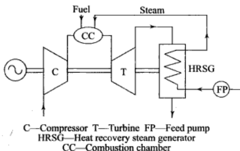
Fig. 3.26 Basic steam injection gas turbine (STIG)
