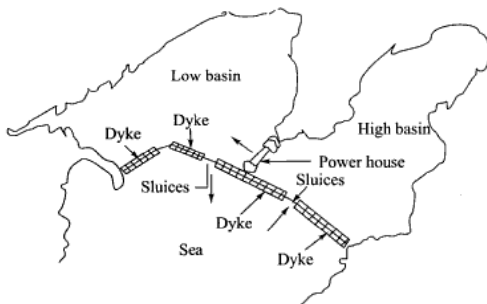
Fig. 14.28 (a) Linked basin scheme
