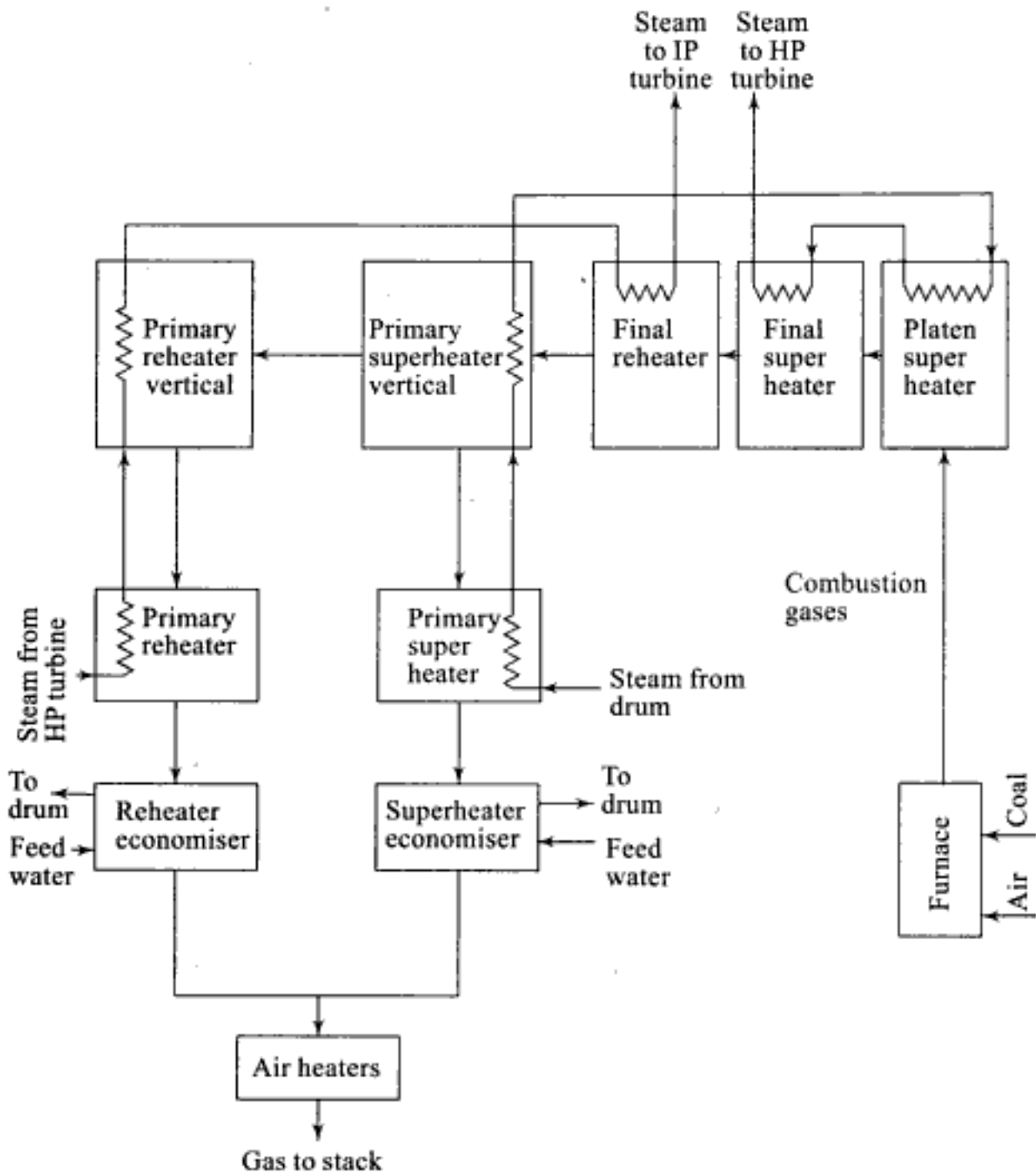
Fig. 6.20 (d) Block diagram showing boiler elements and flowpaths in the 660 MW CEGB steam generator
