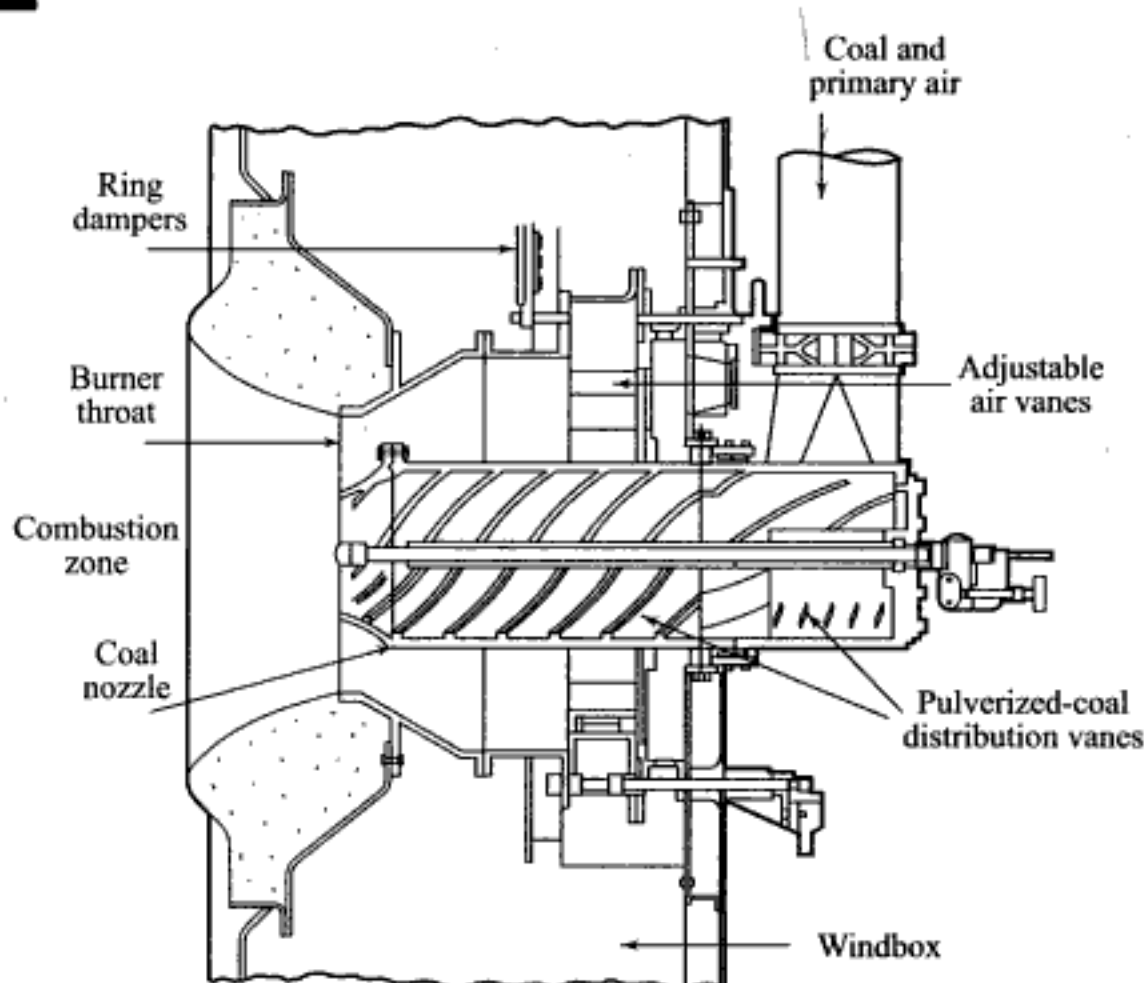
Fig. 5.29(b) Burner for horizontal firing of coal
