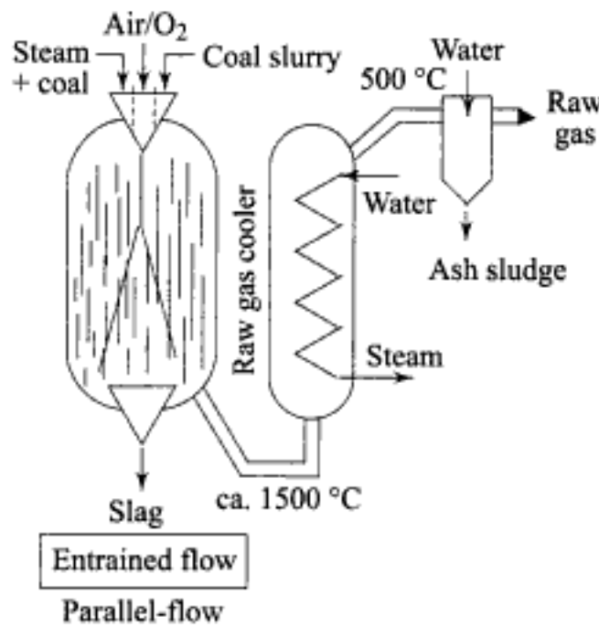
Fig. 5.57 Entrained parallel flow gasifier
