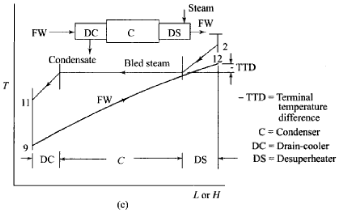
Fig. 2.22 Temperature-length diagram for l.p. and h.p. feedwater heaters
