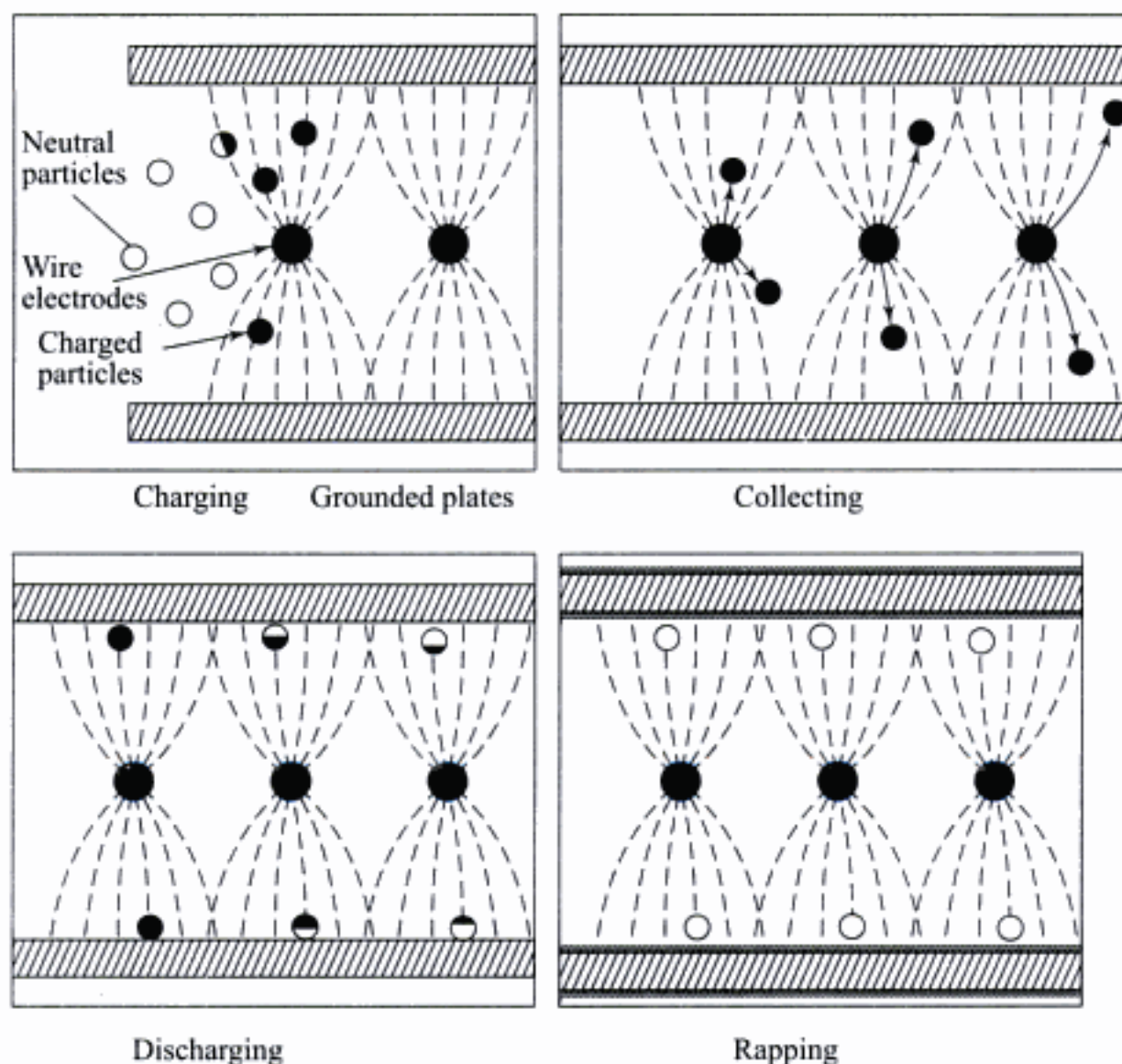
Fig. 6.61 Vertical electrodes and grounded plates in an ESP showing four basic operations
