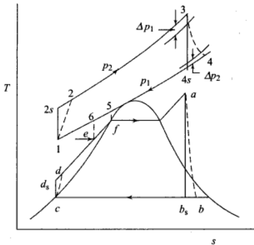
Fig. 3.15 Combined GT-ST cycle for exergy analysis
