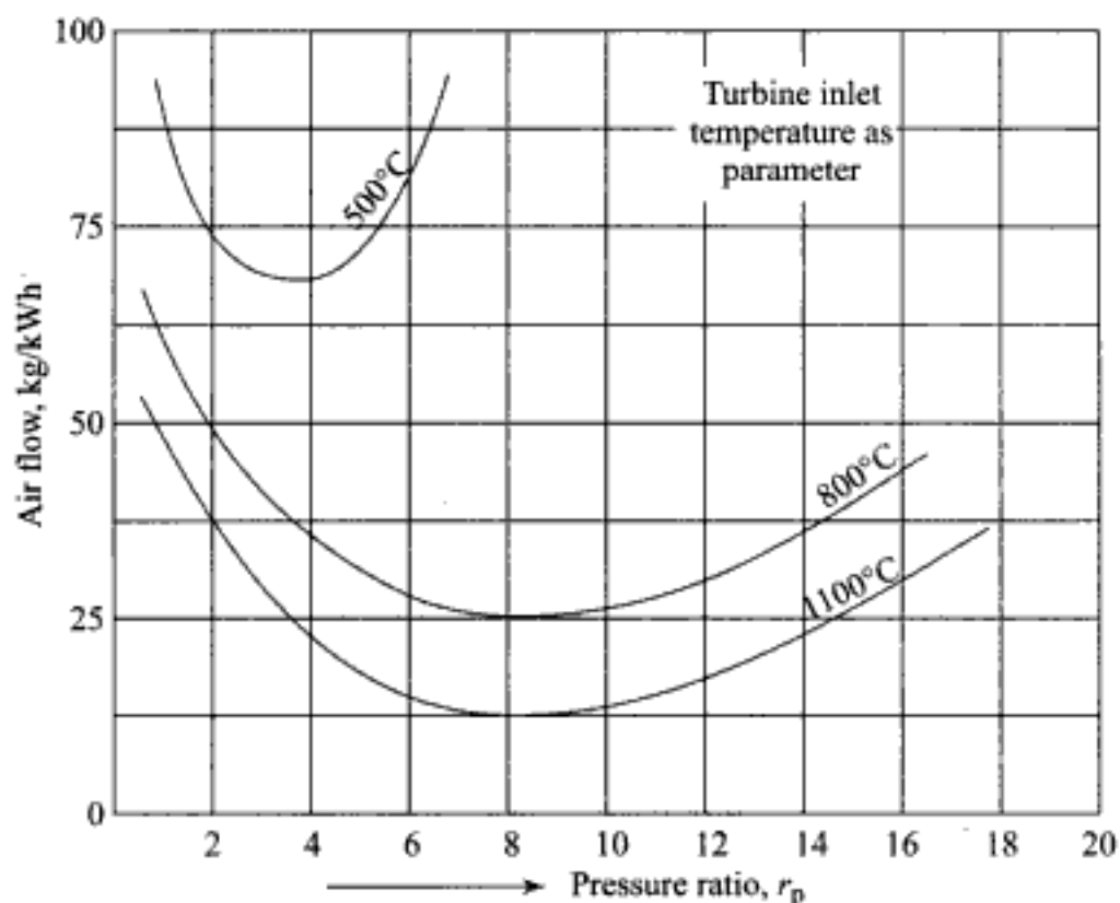
Fig. 11.50 Effect of pressure ratio on air mass flow per unit output
