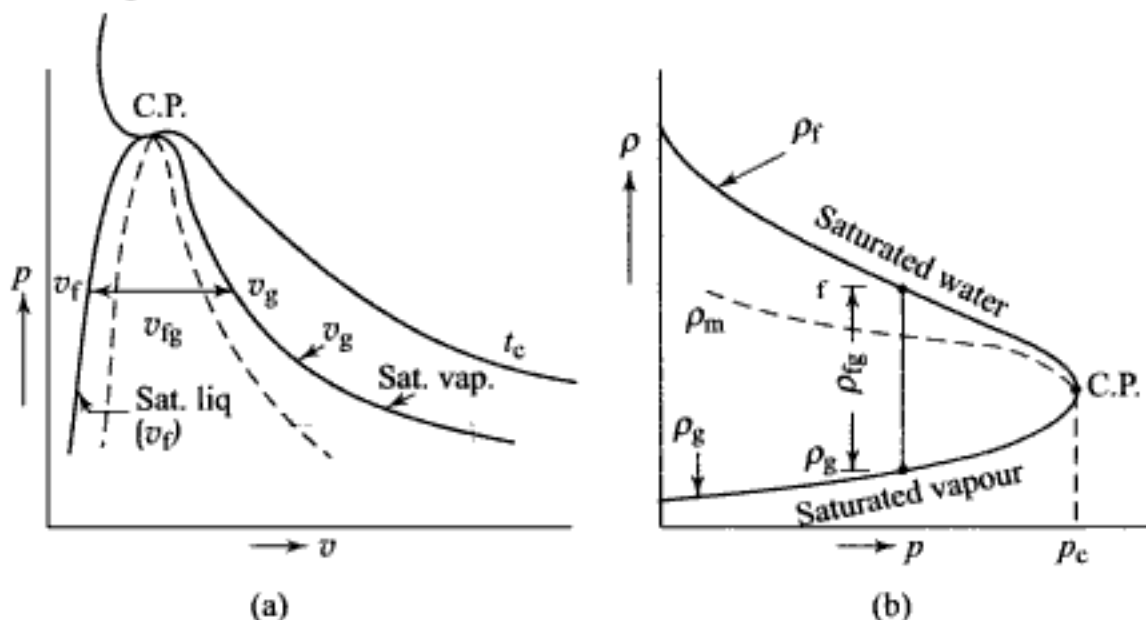
Fig. 6.9 Differentials in specific volume and density varying with pressure
