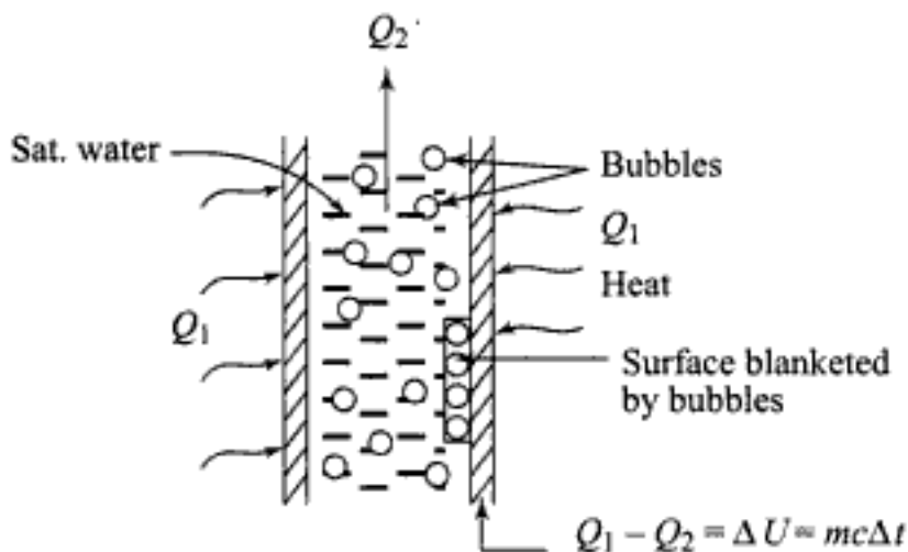
Fig. 6.11 Nucleate and film boiling in a riser tube
