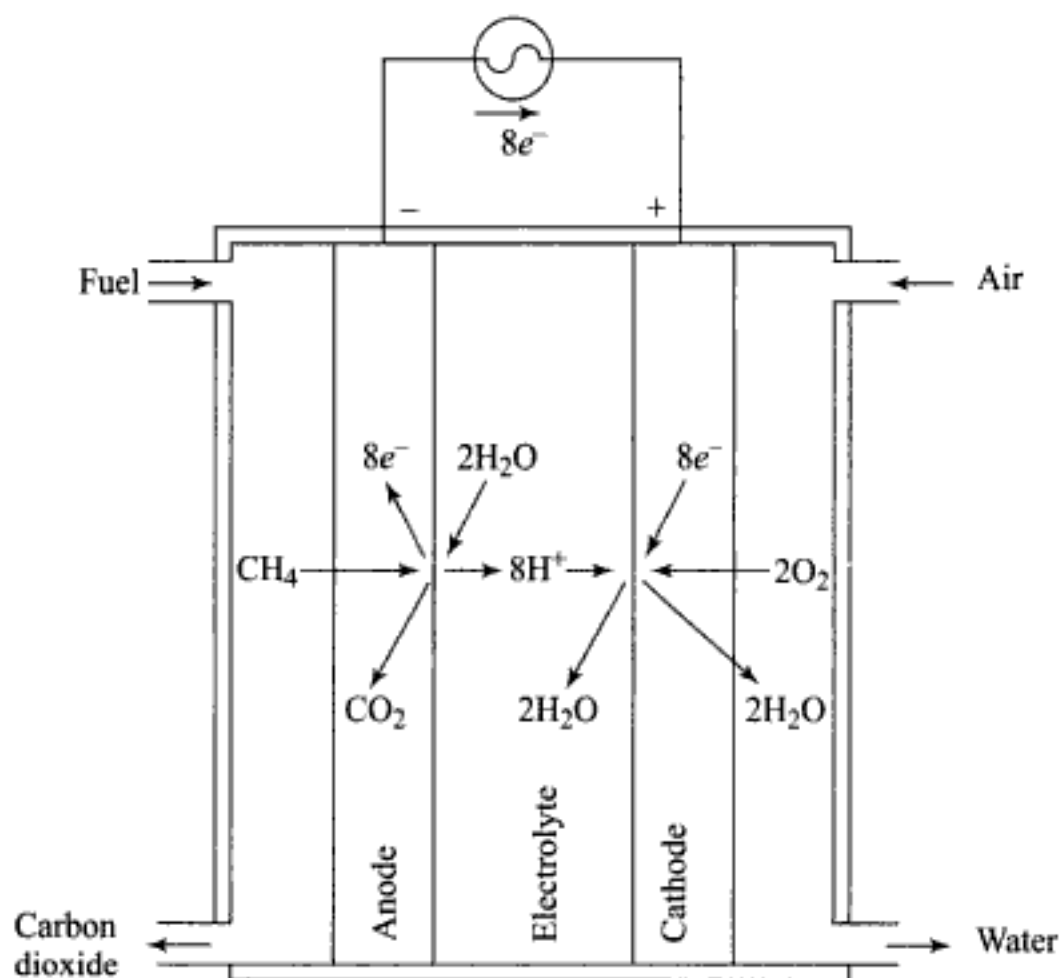
Fig. 13.26 Schematic representation of the methane-oxygen fuel cell
