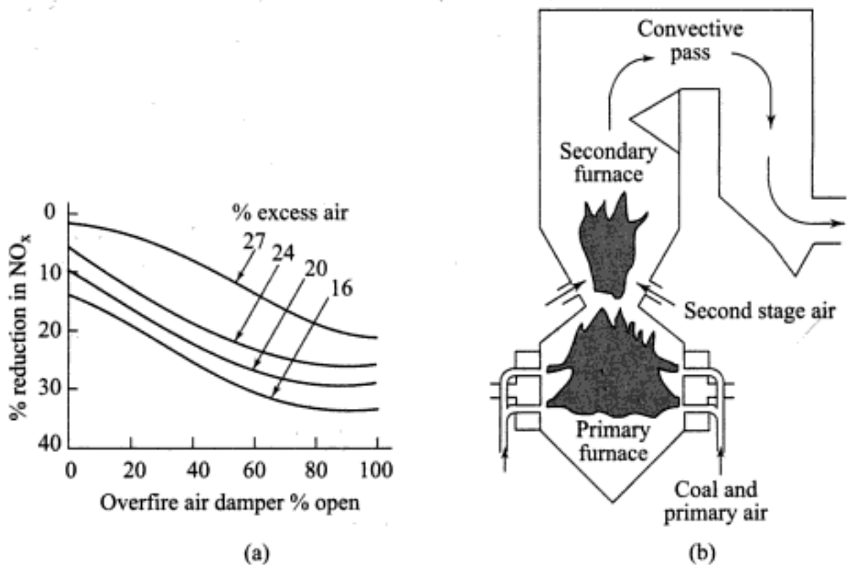
Fig. 5.31 (a) Effect of overfire air on \text{NO}_x production (b) Babcock and Wilcox two-stage venturi furnace (for low \text{NO}_x production)
