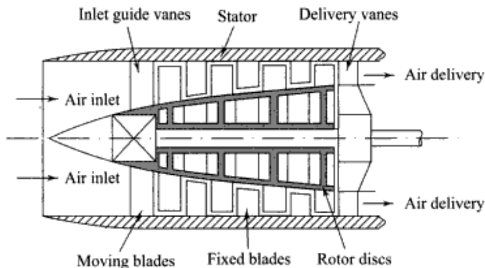
Fig. 11.58 Axial flow compressor
