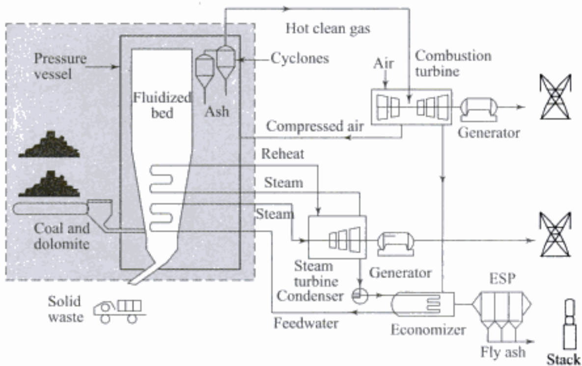
Fig. 6.57 Schematic of a pressurized bubbling fluidized bed combustor
