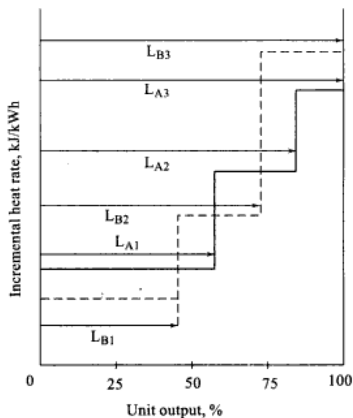
Fig. 1.12 Incremental heat rate curves for unit A and B
