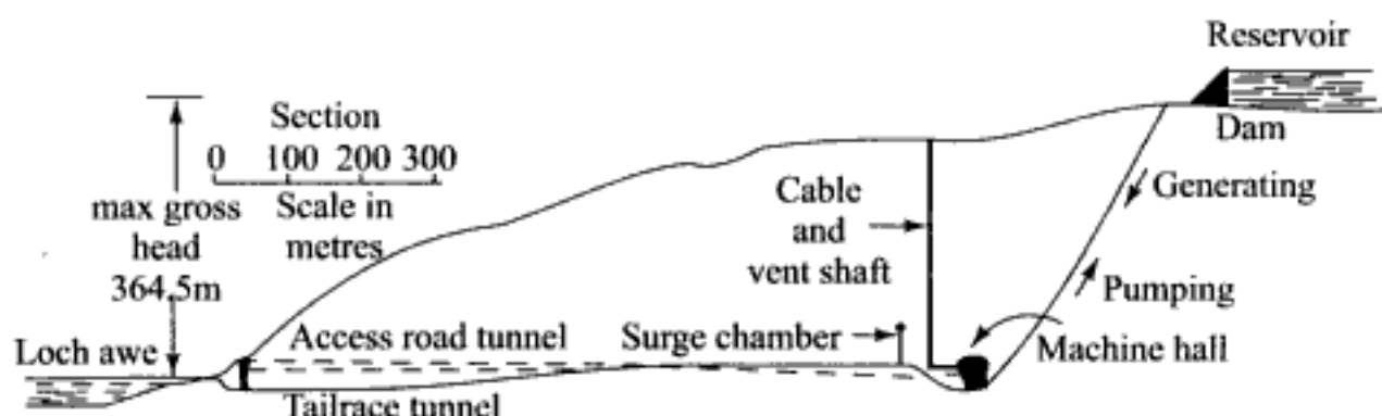
Fig. 12.5 Crauchan station of the north of Scotland Hydroelectric Board
