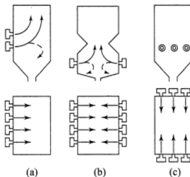
Fig. 5.33 Arrangement of turbulent burners on furnace walls: (a) front firing; (b) opposed firing; (c) opposed firing on side walls
