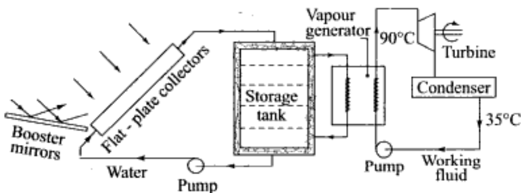
Fig. 14.7 Low temperature Rankine cycle
