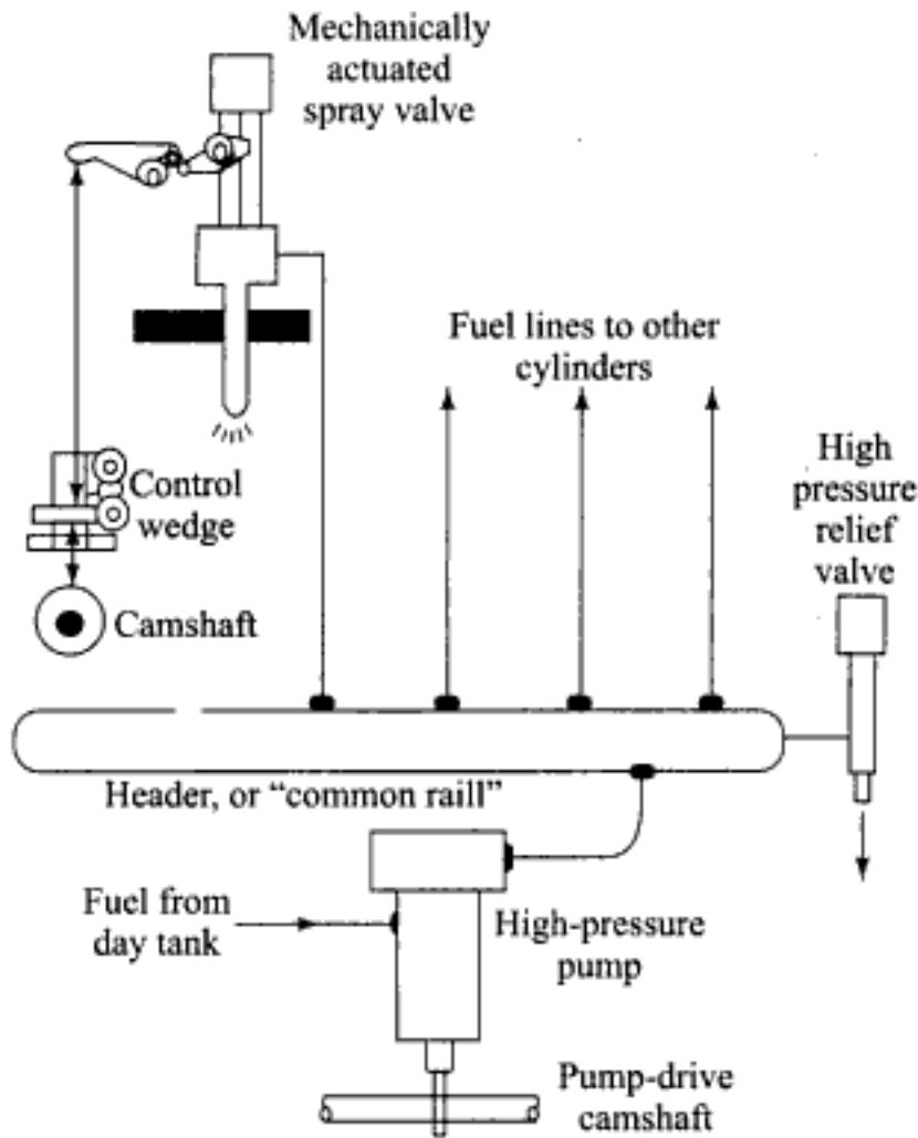
Fig. 11.5 Common-rail injection system
