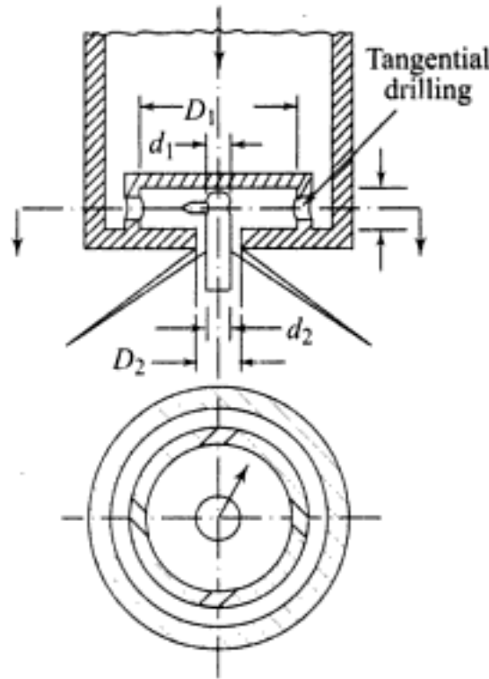
Fig. 5.63 Pressure atomiser with tangential oil feed
