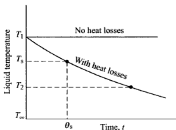
Fig. 12.20 Stored liquid temperature-time change in sensible energy storage. T_1 = fully charged, T_2 = end of energy withdrawal, T_\infty = ambient
