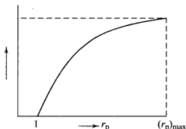
Fig. 11.41 Variation of cycle efficiency with r_p
