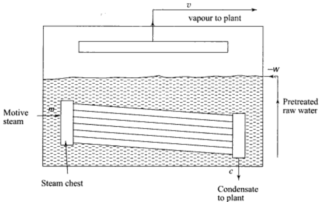
Fig. 6.68 Schematic of a single-effect submerged evaporator
