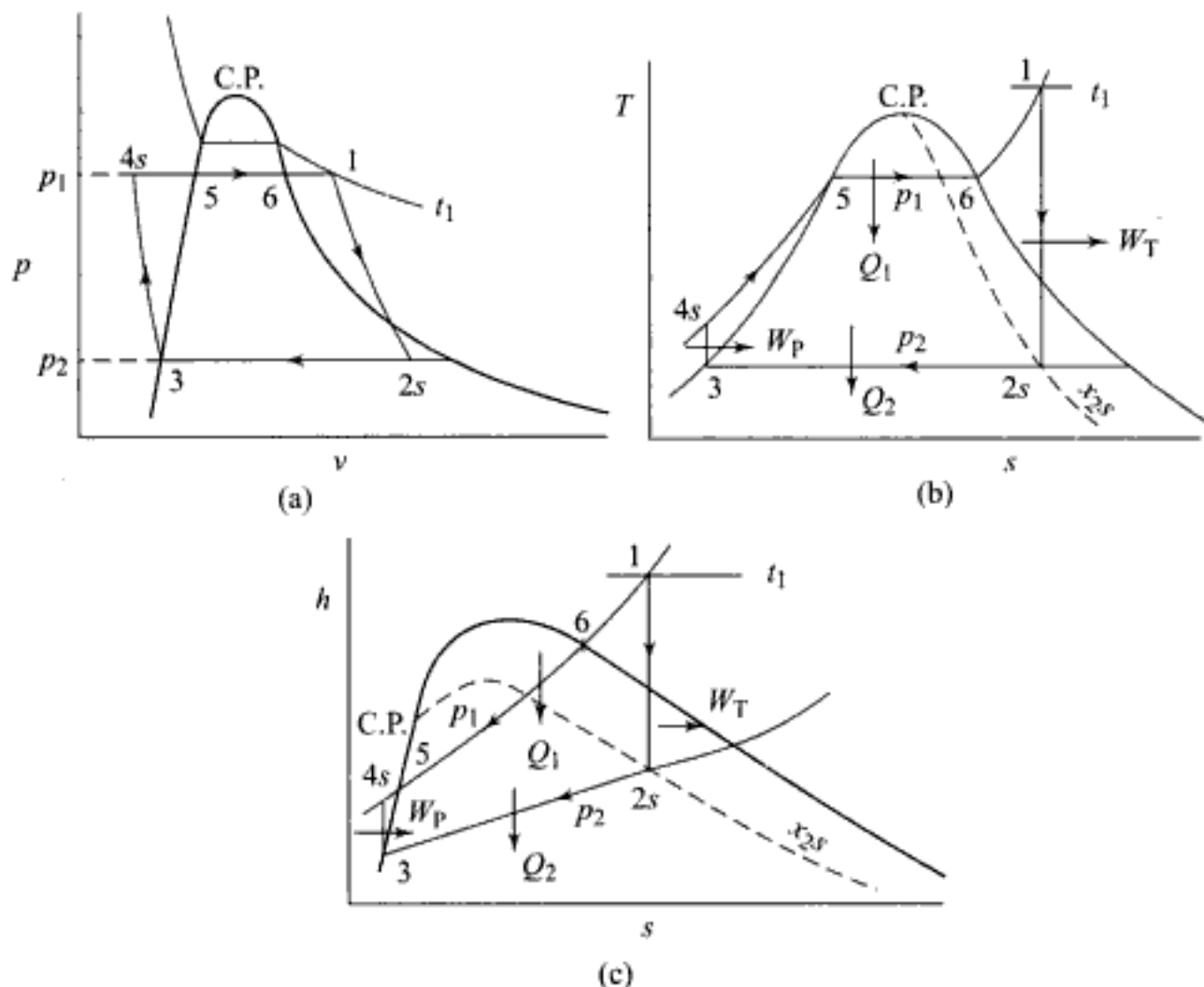
Fig. 2.3 Rankine cycle on p-v , T-s and h-s coordinates (a, b and c)
