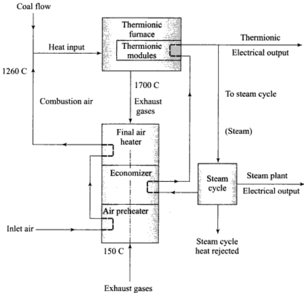
Fig. 13.11a Block diagram for a thermionic topped steam power plant
