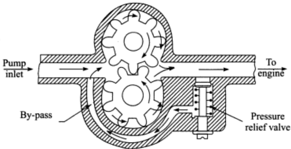
Fig. 11.16 Gear oil pump with relief valve
