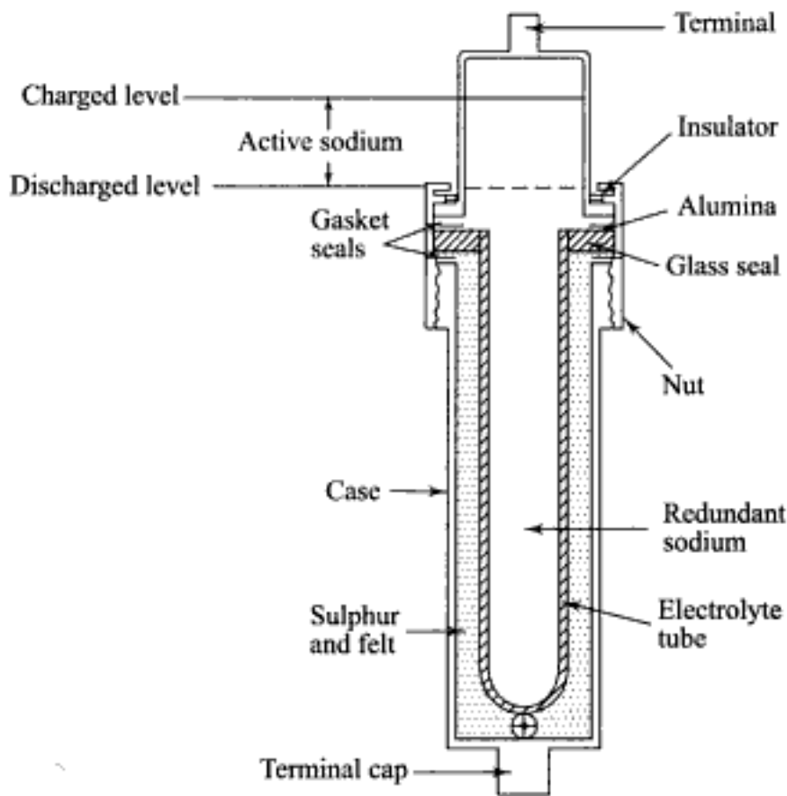
Fig. 12.14 Schematic diagram of the sodium-sulphur battery which uses a sodium beta alumina solid electrolyte as the separator between liquid electrodes (sodium anode and sulphur cathode). The operation temperature is 300–400°C
