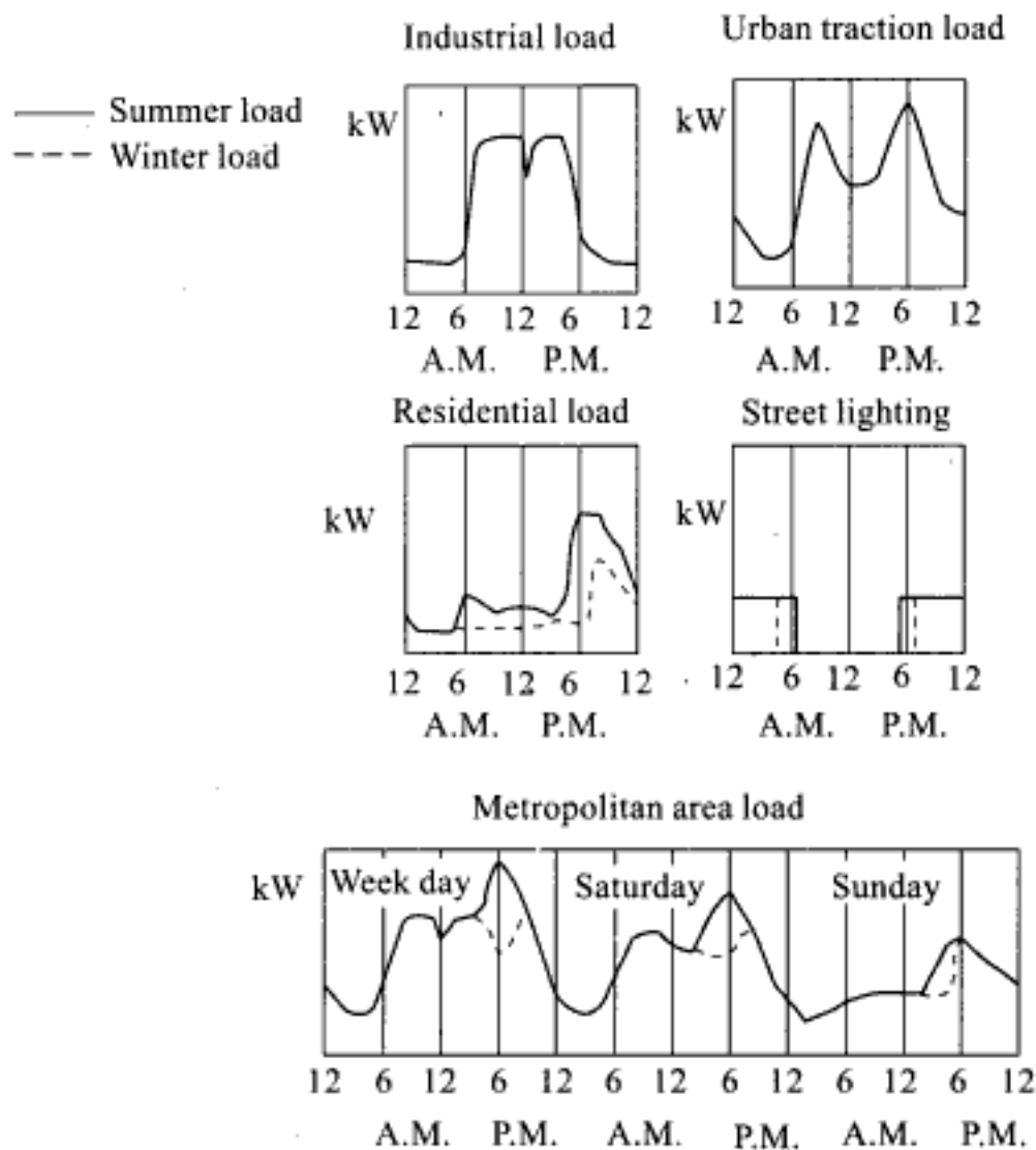
Fig. 1.1 Typical hourly variation in energy demand for different types of electrical load and curves of total load in a metropolitan area
