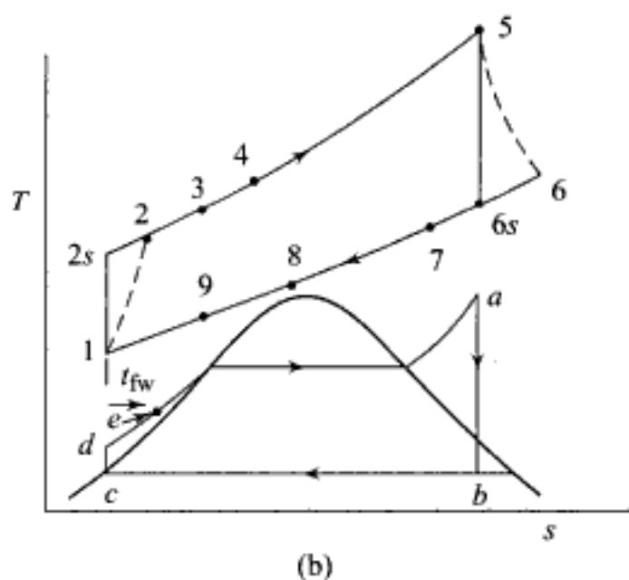
Fig. 13.3 An open cycle MHD-steam power plant
