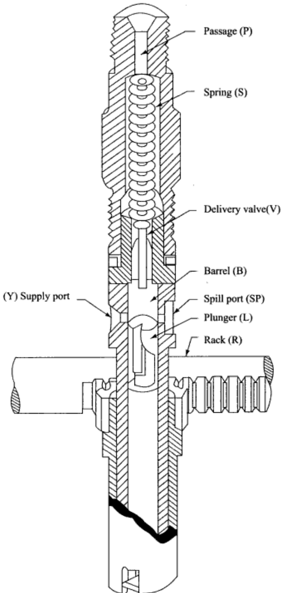
Fig. 11.8 Fuel pump
