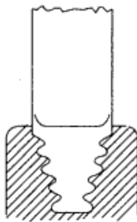
Fig. 7.63 Fir-tree attachment
