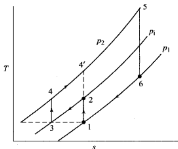
Fig. 11.44 Effect of intercooling on brayton cycle
