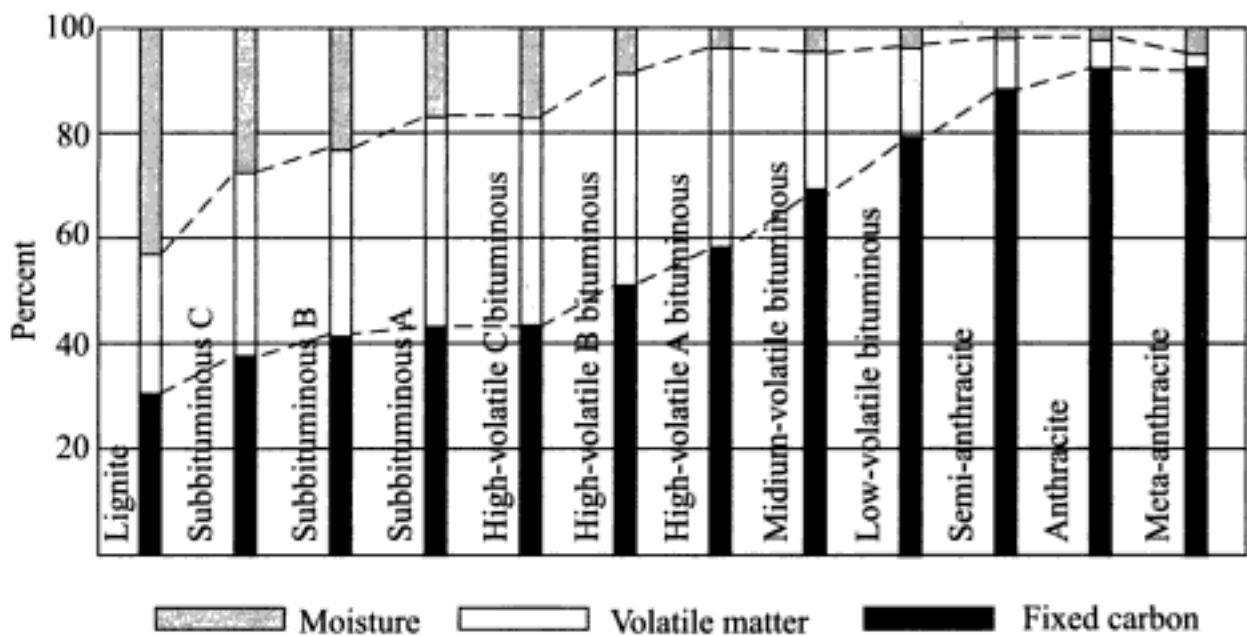
Fig 4.1 Coal rank compared with proximate analysis
