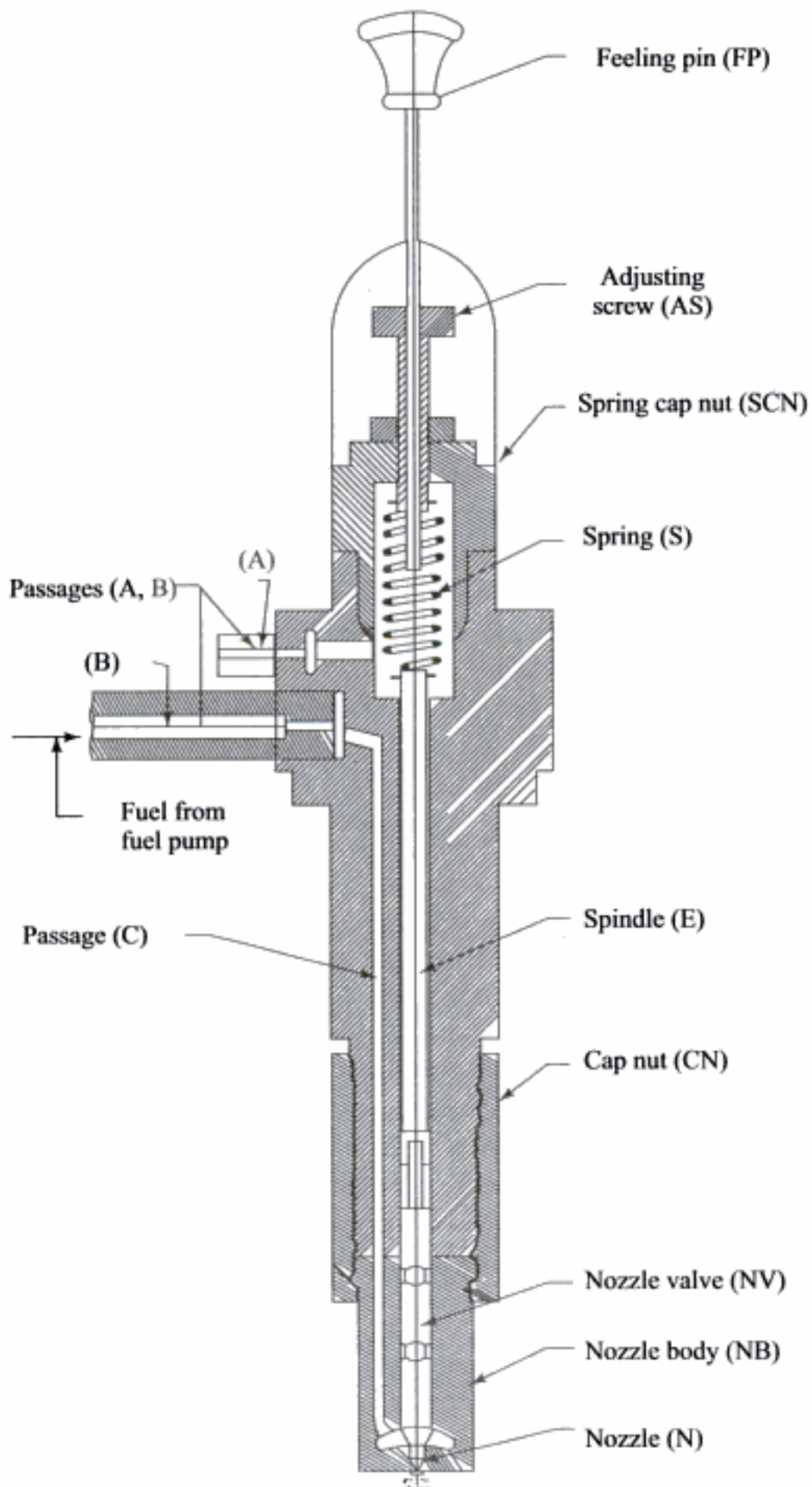
Fig. 11.9 Fuel injector
