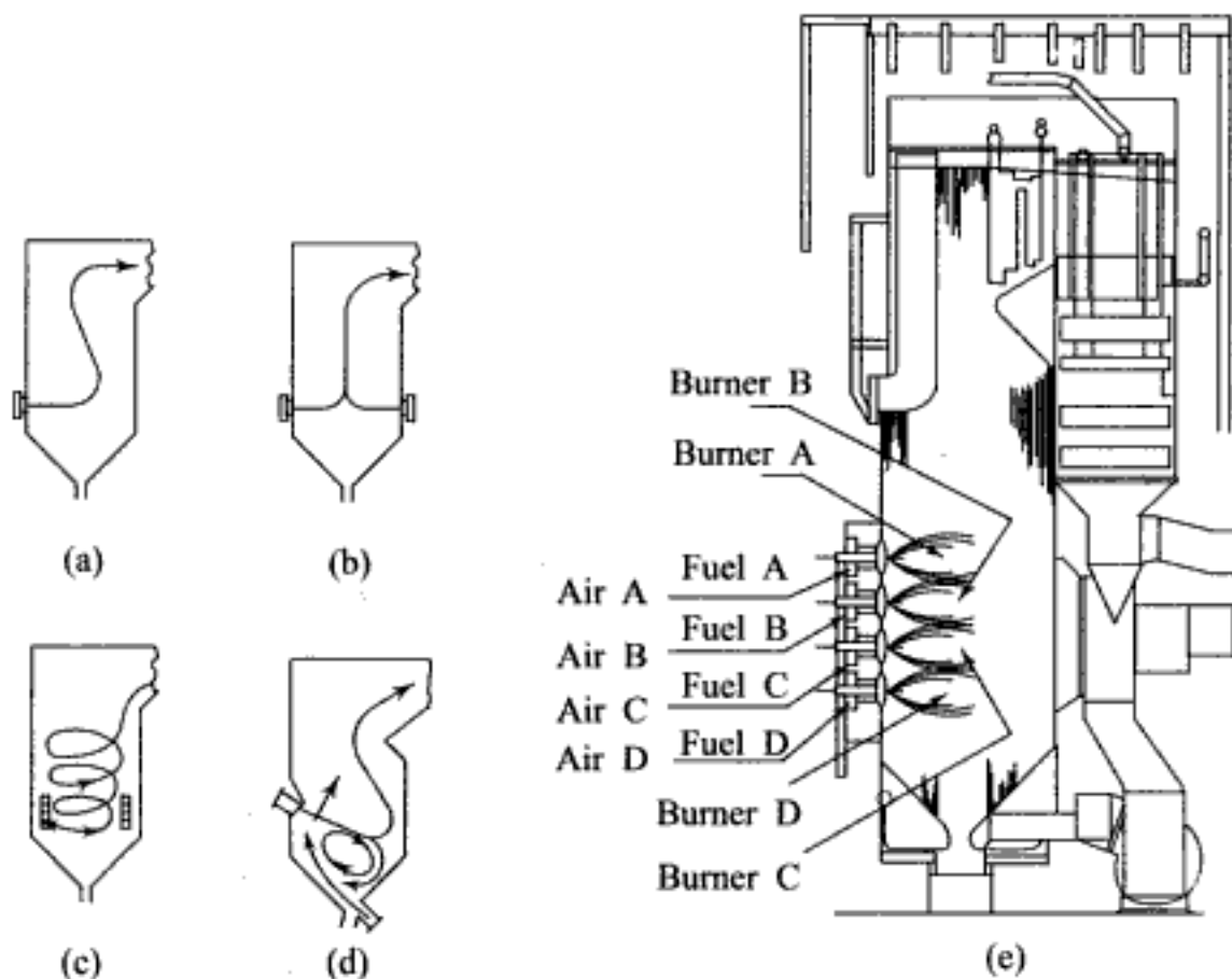
Fig. 5.34 (ii) Patterns of flame motion in dry-bottom furnaces: (a) straight-flow S-shaped flame; (b) opposite straight-flow flame; (c) vertically turbulized flame; (d) combination of straight-flow and horizontally turbulized flame; (e) flow pattern of horizontal (wall) firing
