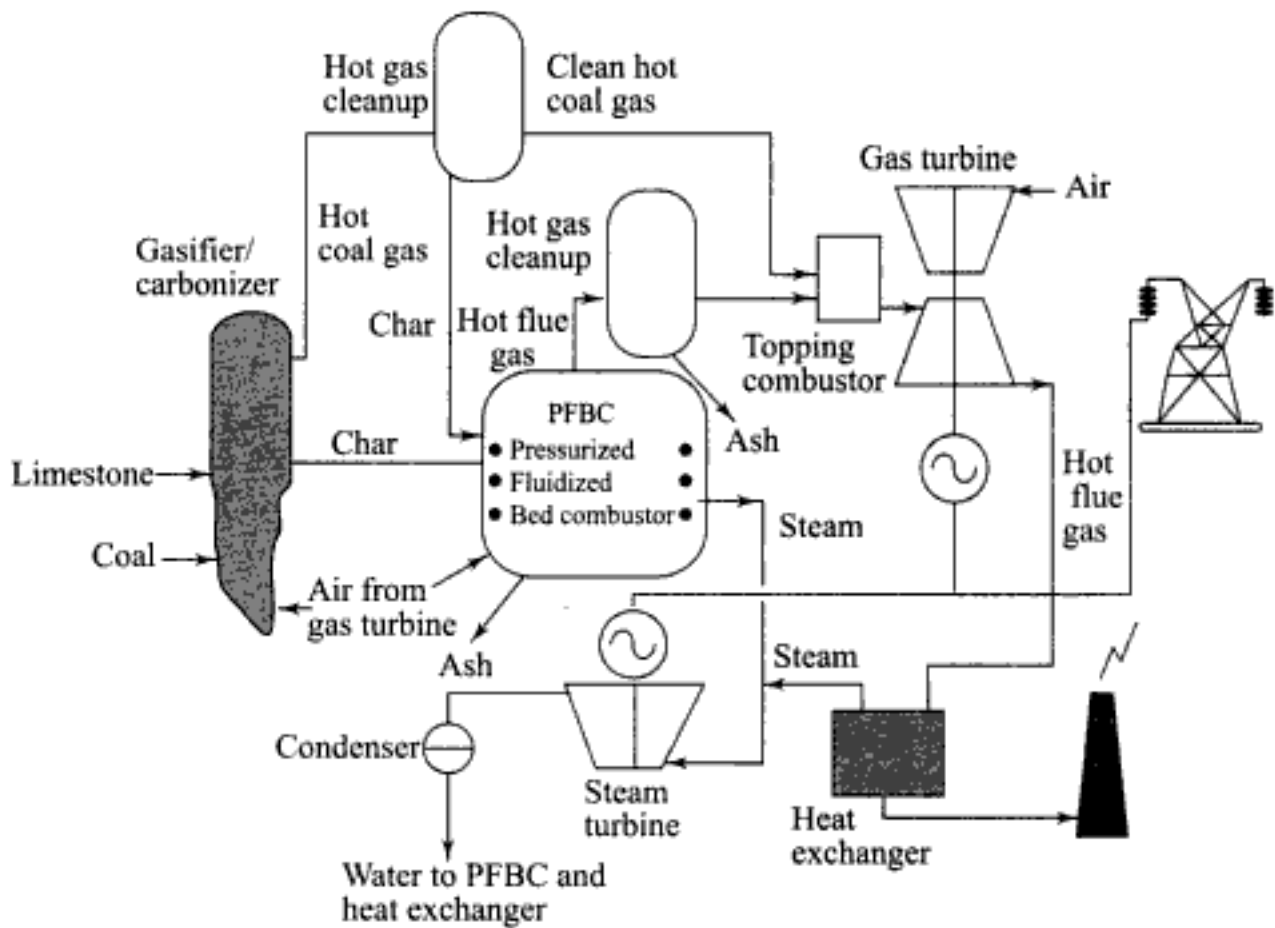
Fig. 5.55 Advanced PFBC system
