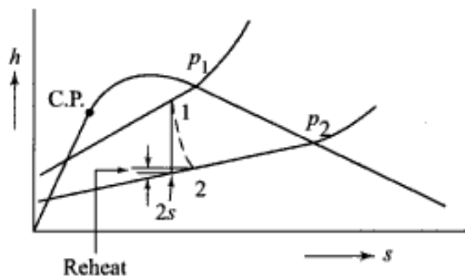
Fig. 7.48 Expansion in a single stage with reheat
