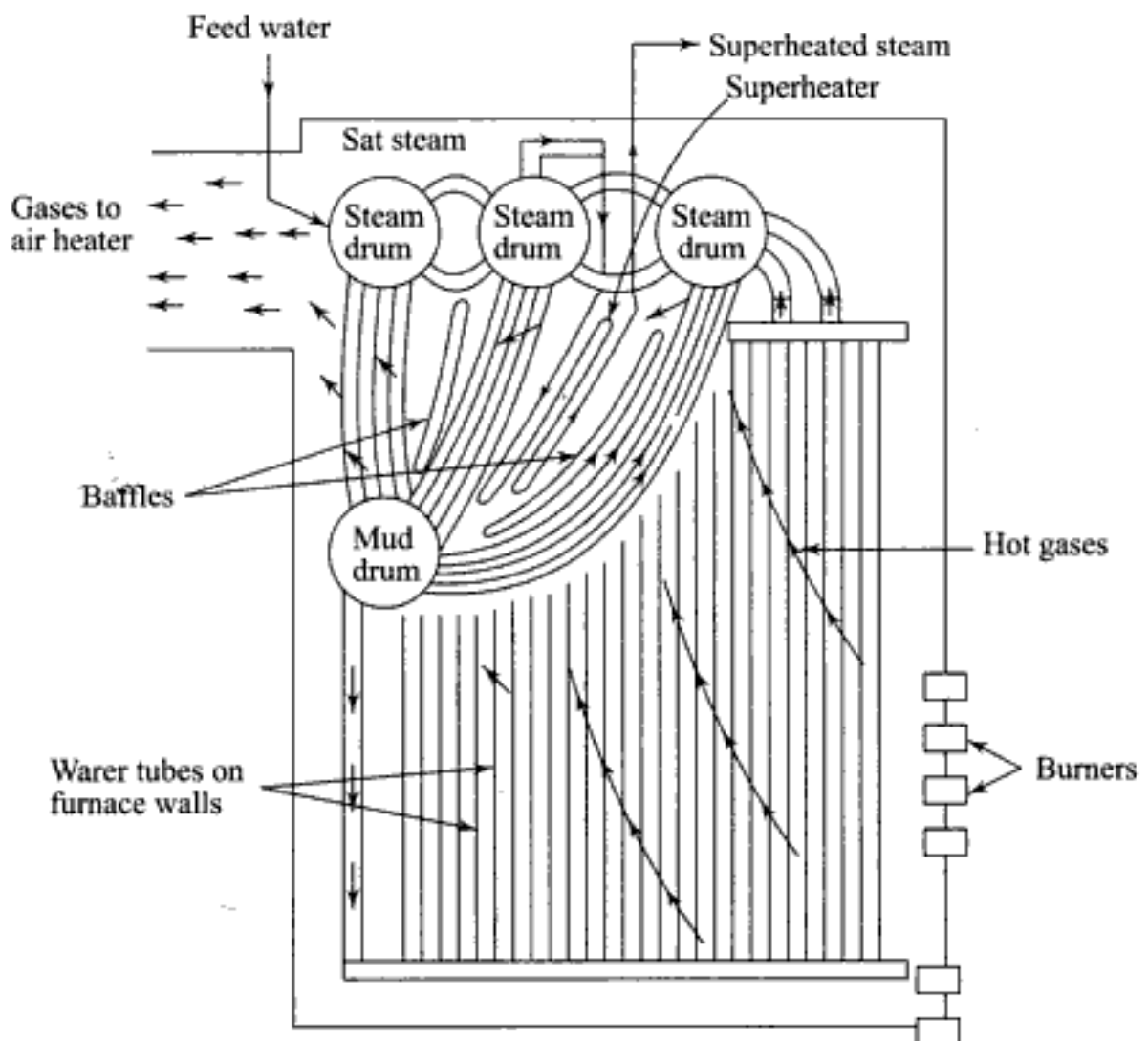
Fig. 6.4 A four-drum bent tube boiler
