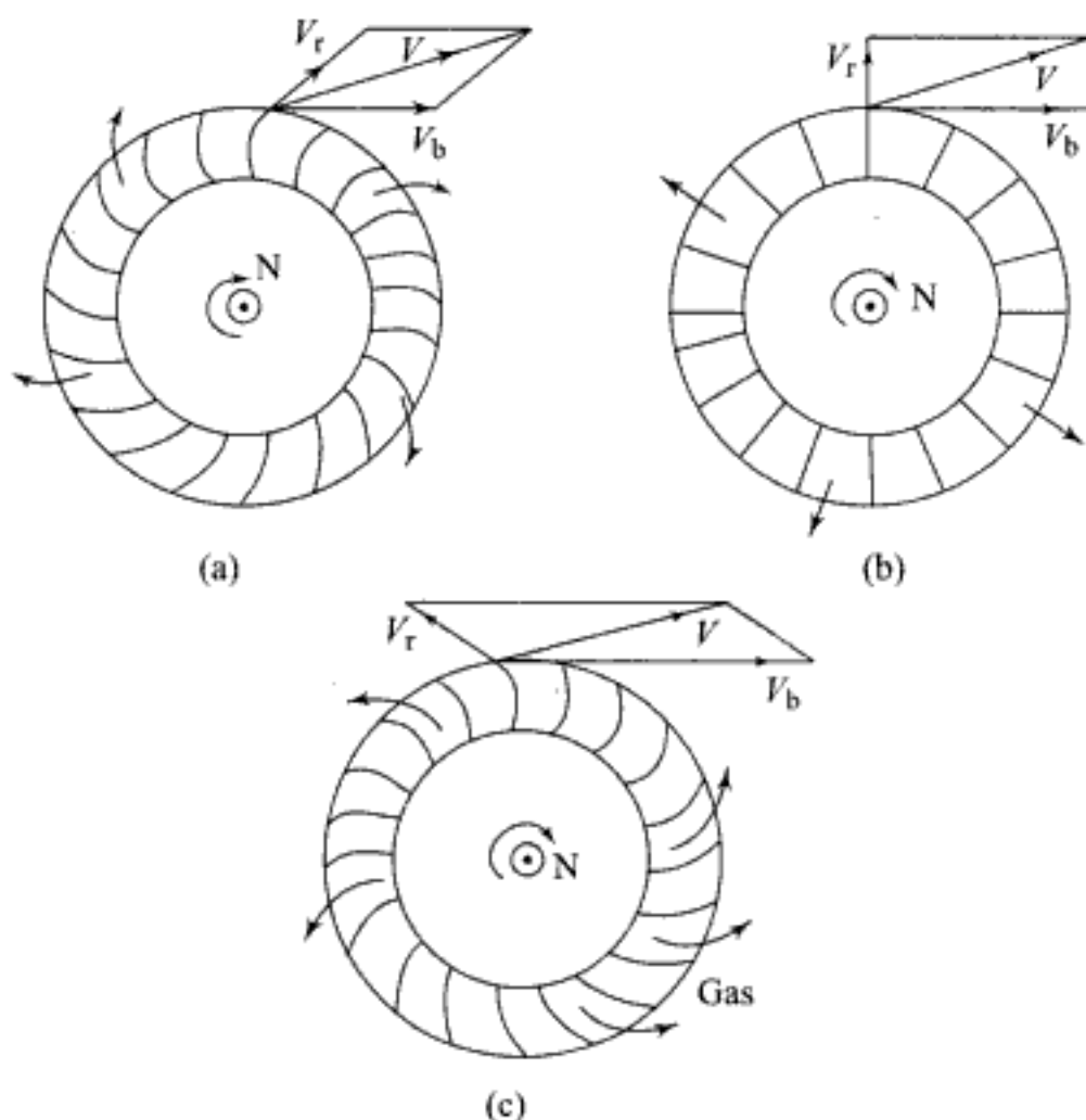
Fig. 4.17 Centrifugal blading: (a) forward-curved, (b) flat, and (c) backward-curved. Vector diagrams show blade tip velocity V_b , gas velocity relative to blade V_r , and absolute velocity of gas leaving blade V . In all cases, V is the same
