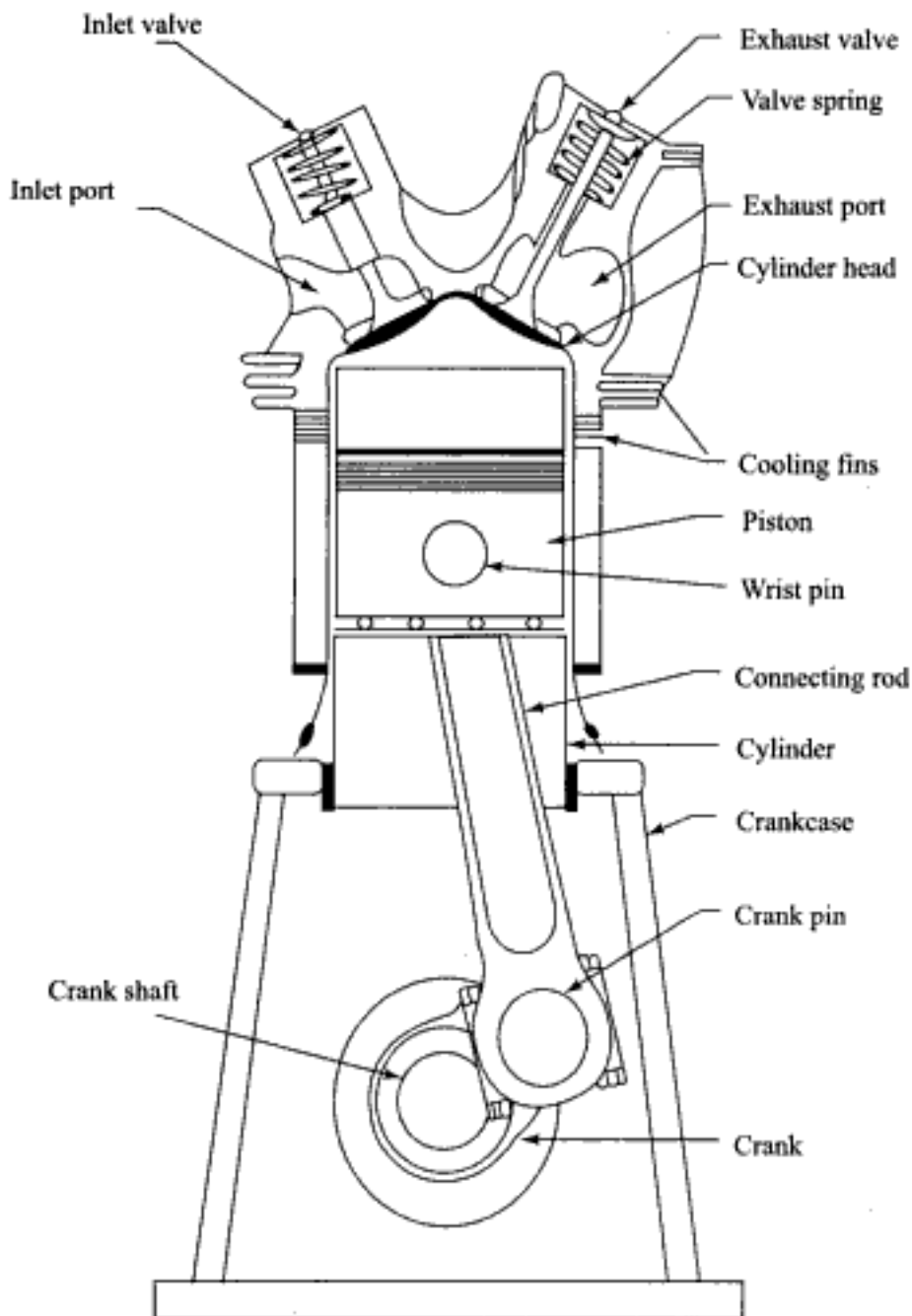
Fig. 11.1 General View of an air-cooled IC engine
