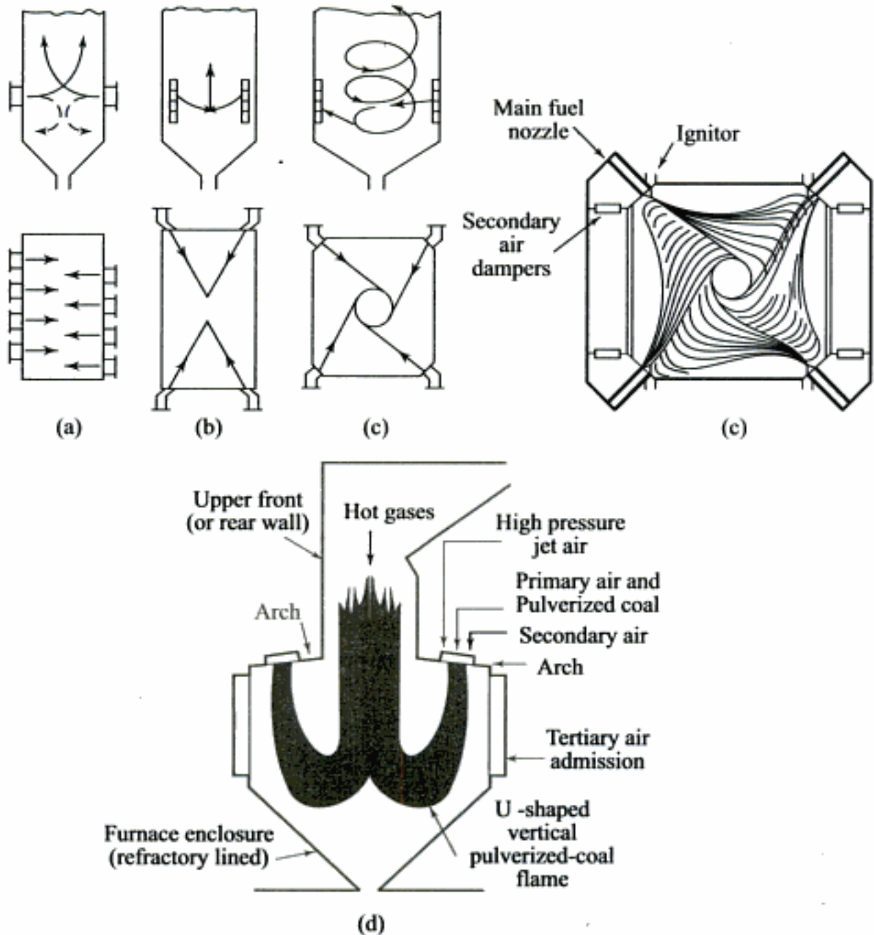
Fig. 5.34 (i) Arrangement of straight flow burners on furnace walls: (a) opposed displaced firing, (b) corner firing with encountering jets; (c) corner firing with tangential jets; (d) vertical firing
