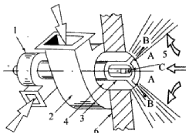
Fig. 5.28 Two scroll turbulent burner. 1-Scroll for fuel-air mixture; 2-secondary air scroll; 3-annular channel for discharging fuel-air mixture into furnace; 4-ditto, for secondary air; 5-main fuel oil burner; 6-furnace lining; AB-boundary of fuel-air mixture ignition; C-suction of gases to flame root
