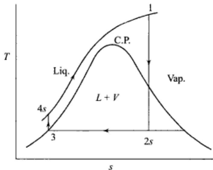
Fig. 2.5 Rankine cycle with supercritical boiler pressure
