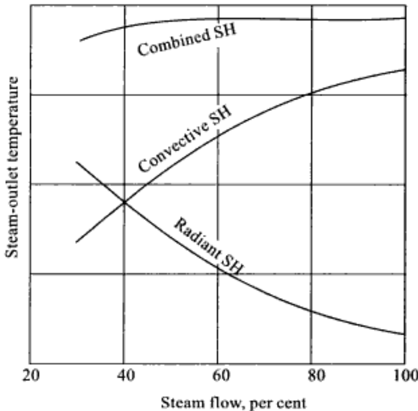
Fig. 6.29 Steam-outlet temperature response of convective, radiant, and combined (in series) superheater
