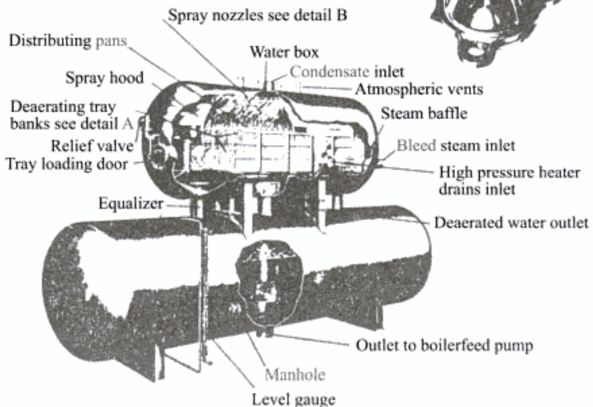
Fig. 8.15 A typical open-type deaerating feedwater heater
