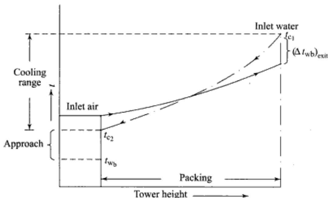
Fig. 8.29 Temperature relationship in a counterflow cooling tower
