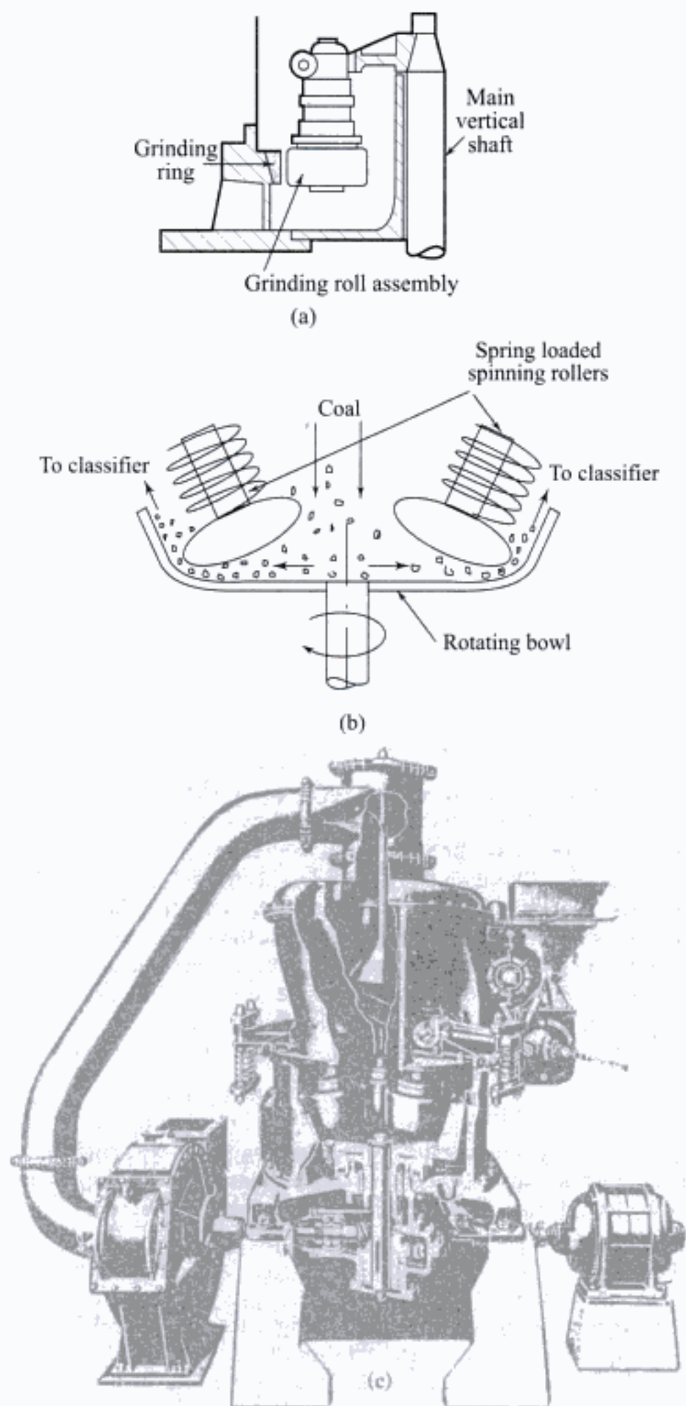
Fig. 5.18 (a) Roller-type ring-rong mill, (b) Bowl mill, (c) Raymond bowl mill
