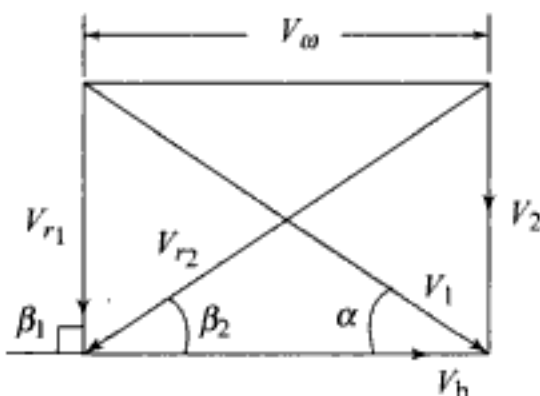
Fig. 7.32 Velocity diagram of a 50% reaction turbine operating with maximum blading efficiency
