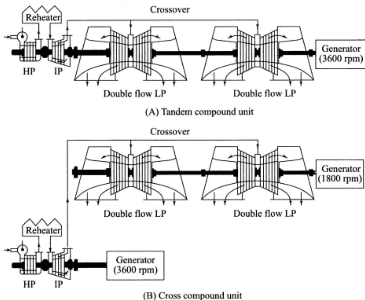
Fig. 7.1 (c) Turbine shaft orientations
