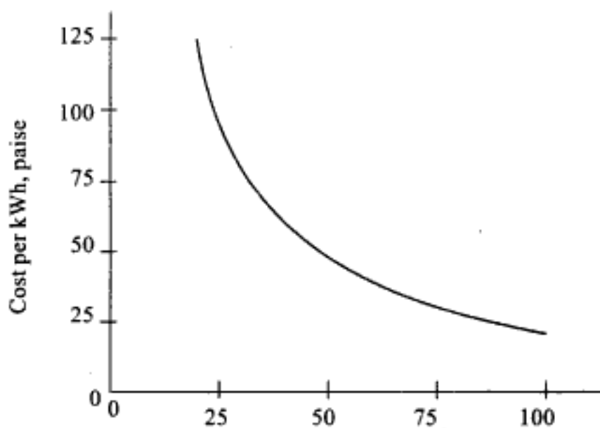
Fig. 1.13 Effect of load factor on cost of energy
