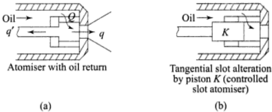
Fig. 5.64 Methods of output control in pressure atomisers
