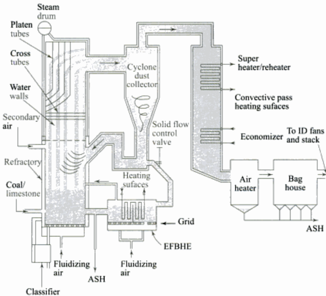
Fig. 6.50 (a) Schematic of a circulating fluidized bed boiler
