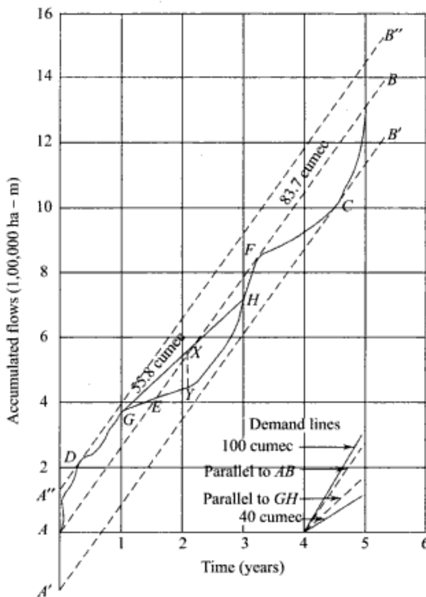
Fig. 10.4 Mass Curve
