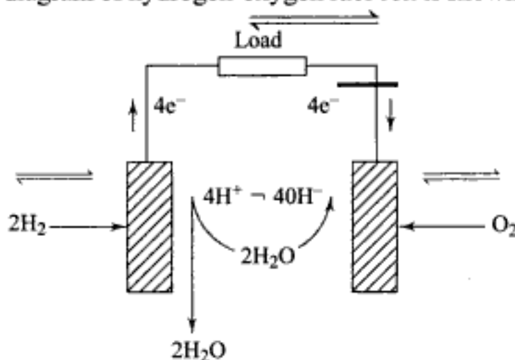
Fig. 12.16 A hydrogen-oxygen fuel cell
