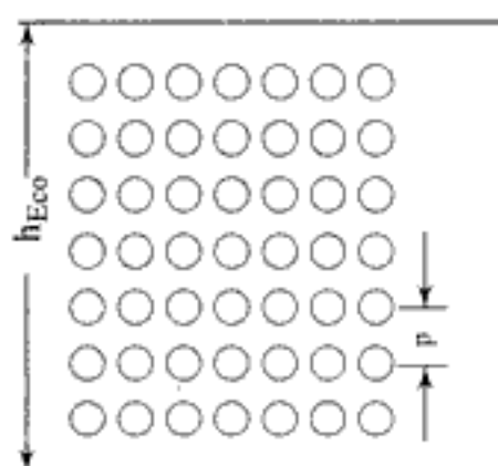
Fig. 6.26 Section x - y in Fig. 6.25(a): height of the economiser duct
