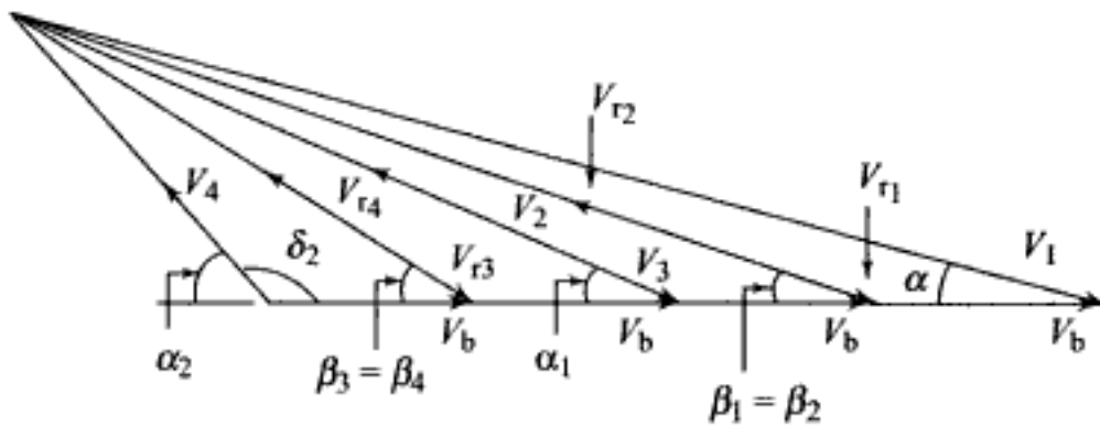
Fig. 7.29 Velocity diagram of a two-row Curtis stage with frictionless symmetrical blading and non-axial discharge
