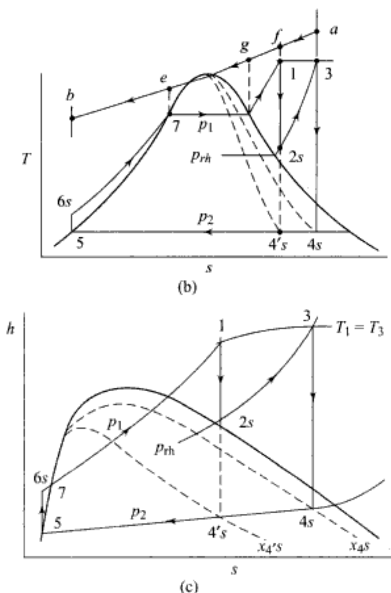
Fig. 2.15 Reheat Cycle
