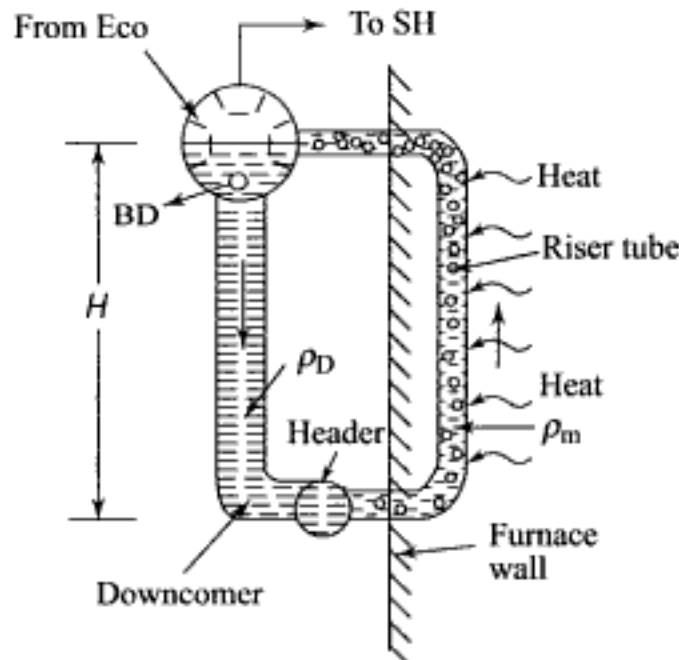
Fig. 6.8 Natural circulation in a downcomer–riser circuit
