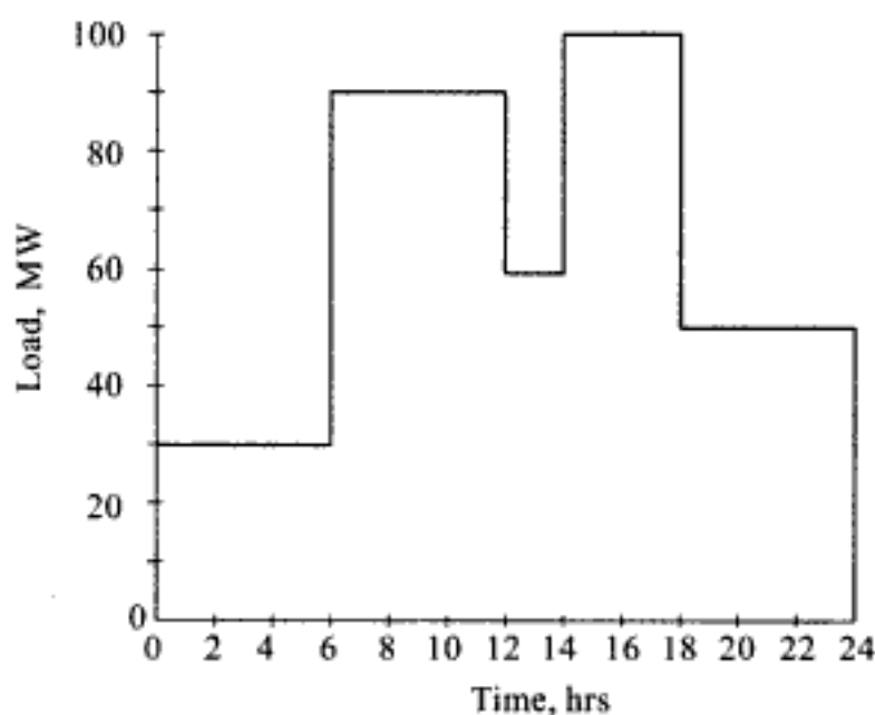
(a) Load curve
