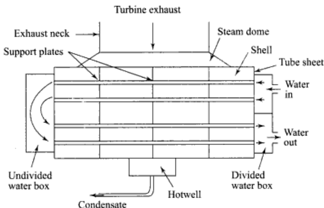
Fig. 8.4 Schematics of a two-pass surface condenser
