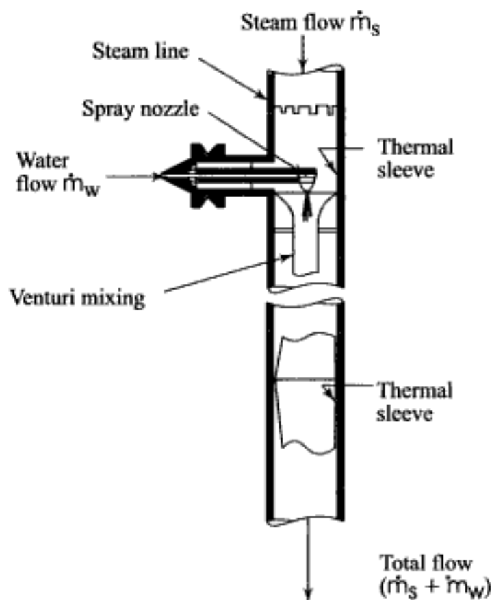
Fig. 6.37 A spray attemperator for steam temperature control
