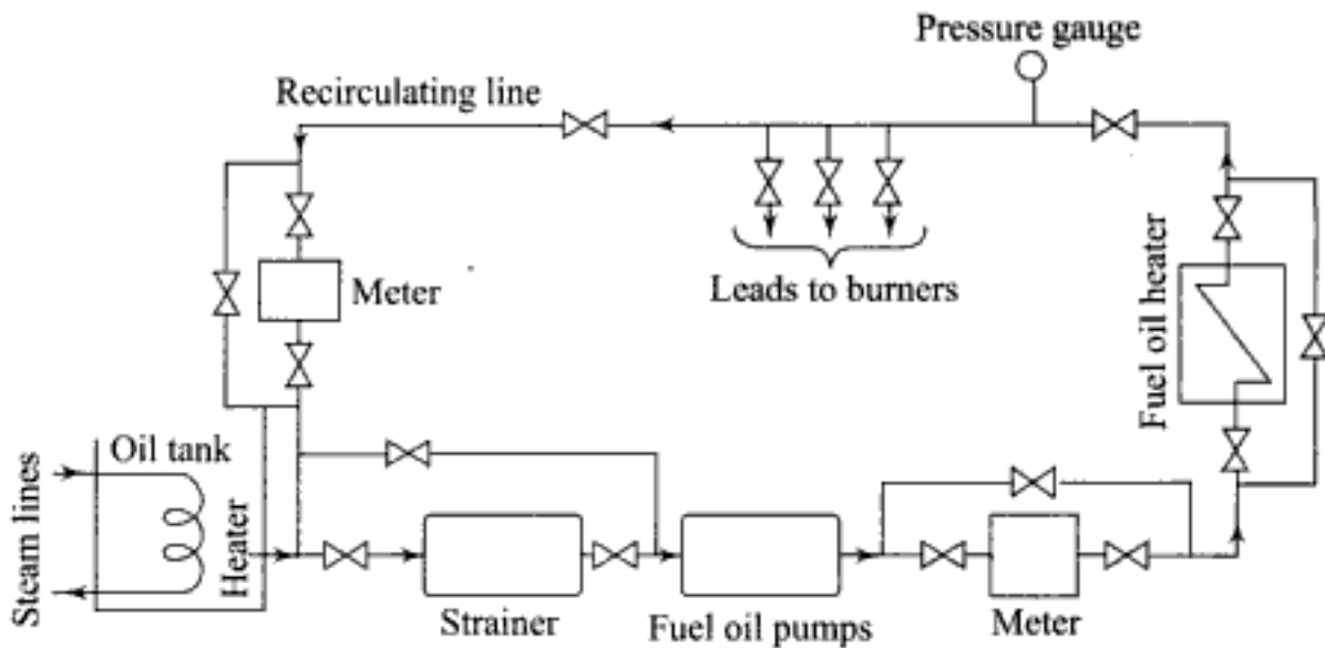
Fig. 5.60 Schematic of an oil burning installation
