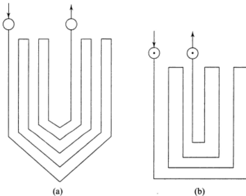
Fig. 6.32 Types of platens (SH): (a) triangular, (b) rectangular
