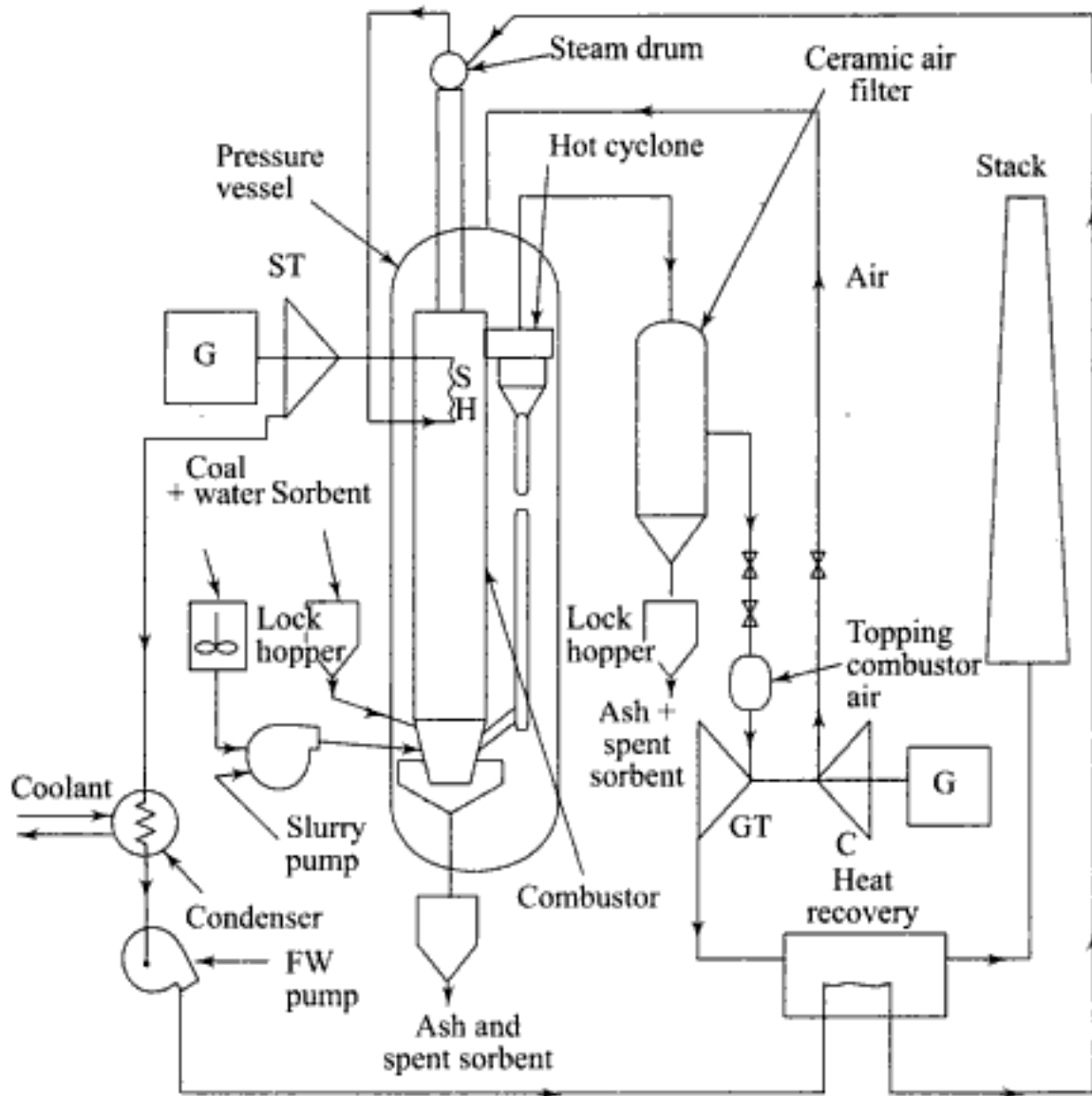
Fig. 6.58 A pressurized circulating fluidized bed combustor
