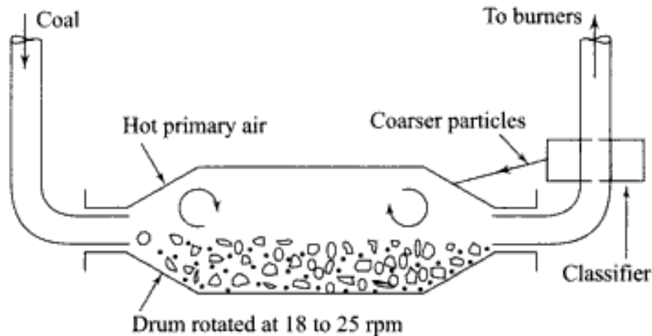
Fig. 5.16 Ball mill
