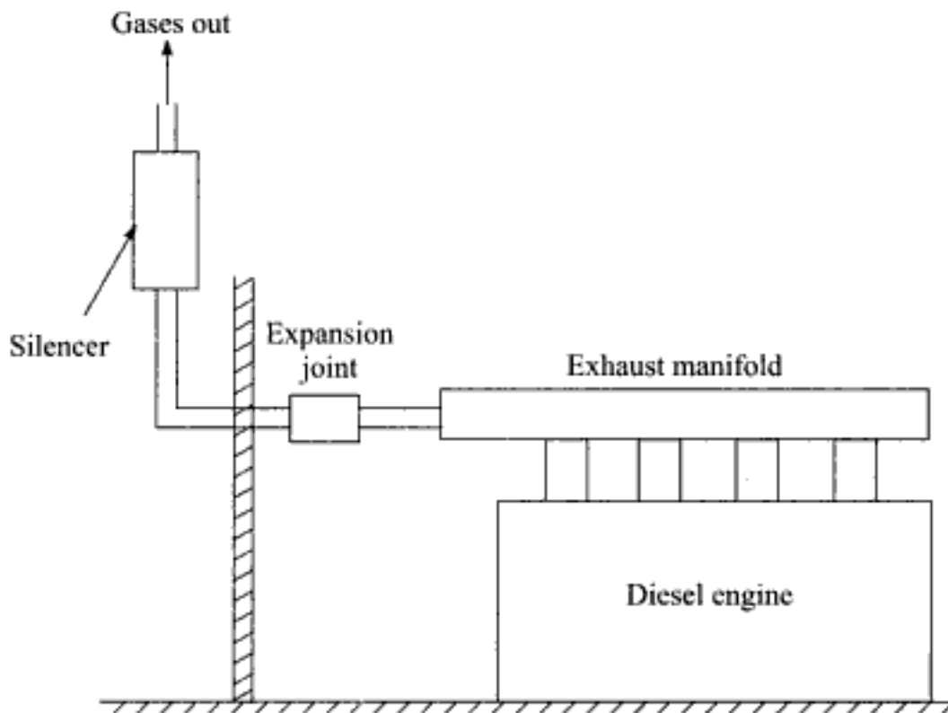
Fig. 11.3 Diesel engine exhaust system
