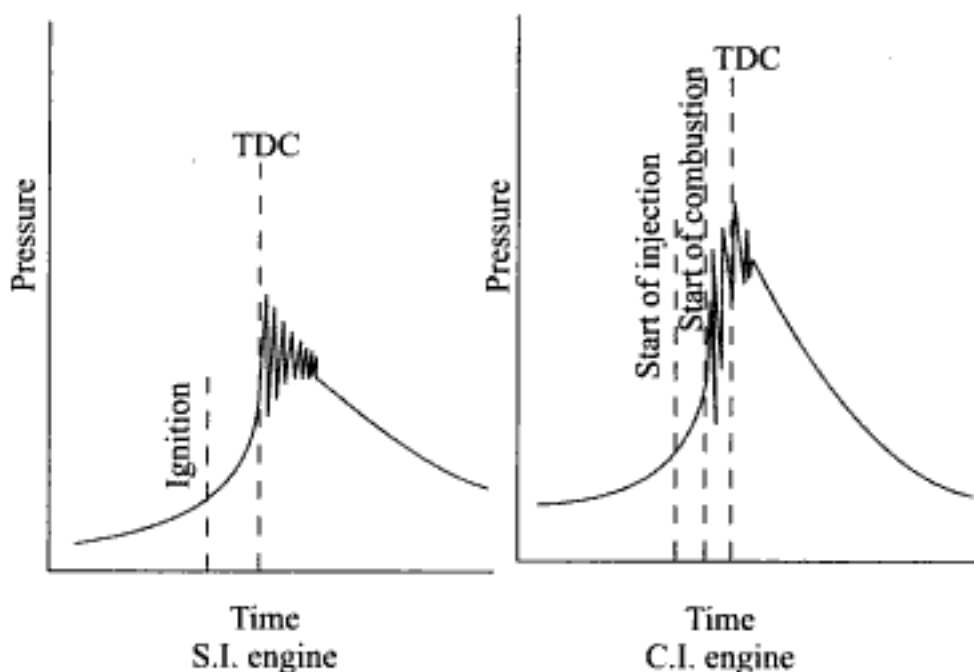
Fig. 11.20 Diagrams illustrating knocking combustion in SI and CI engines
