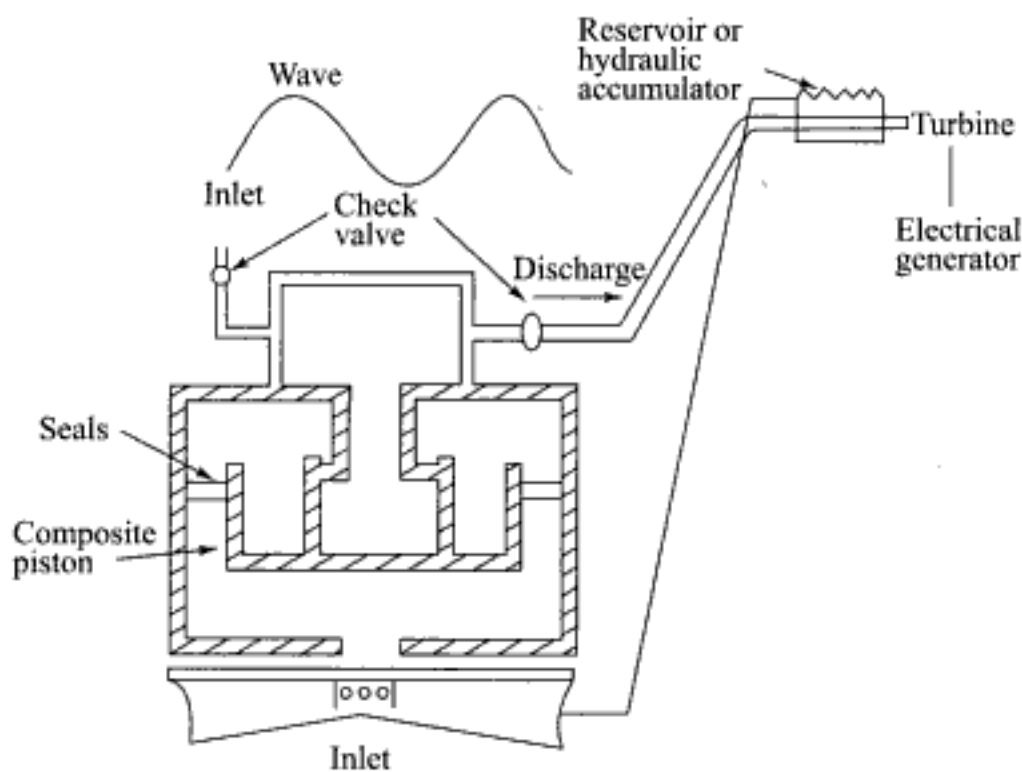
Fig. 14.19 Schematic of a high-level reservoir wave machine (hydraulic accumulator wave machine)
