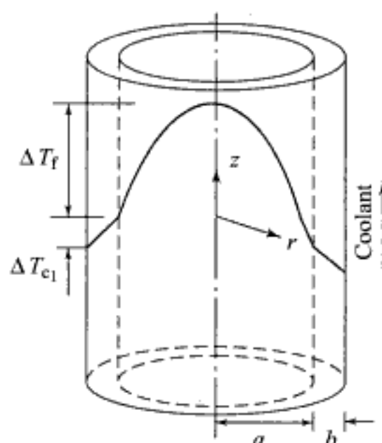
Fig. 9.13 Temperature distribution in cylindrical fuel element
