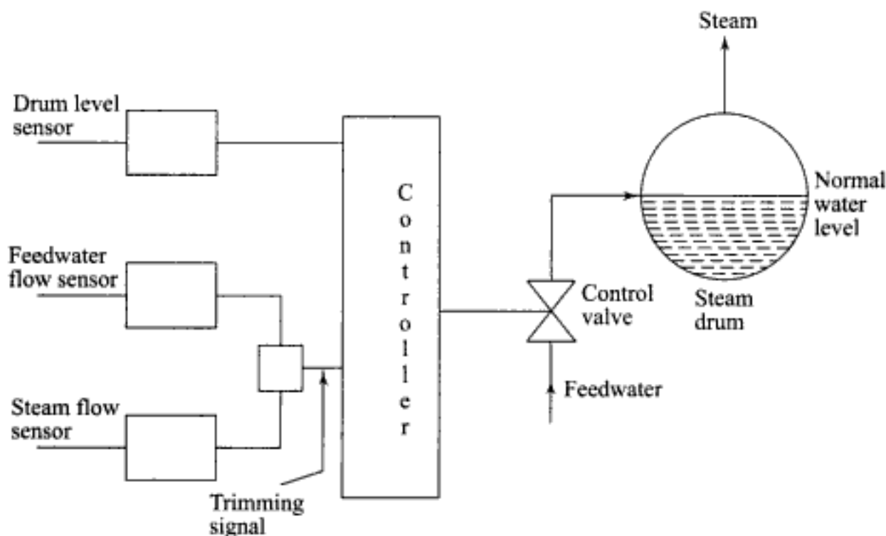
Fig. 6.34 Schematic of a three-element feedwater control system
