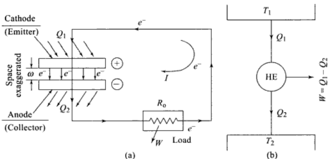
Fig. 13.7 A basic thermionic generator
