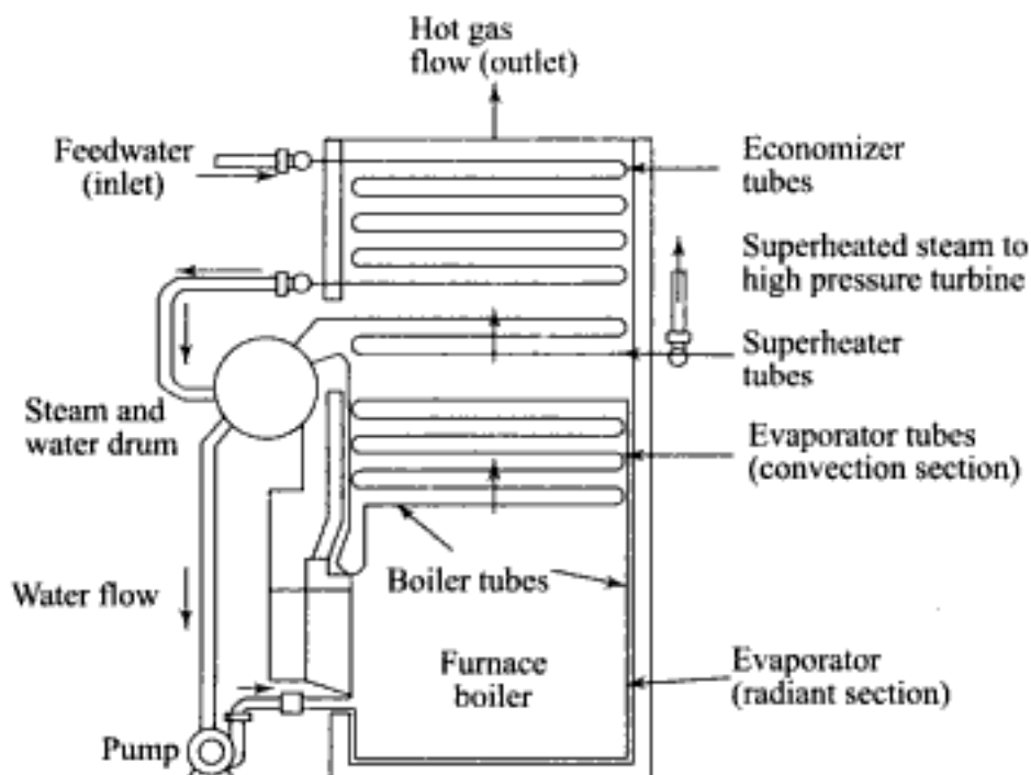
Fig. 6.22 Modern forced circulation steam generator of La Mont type
