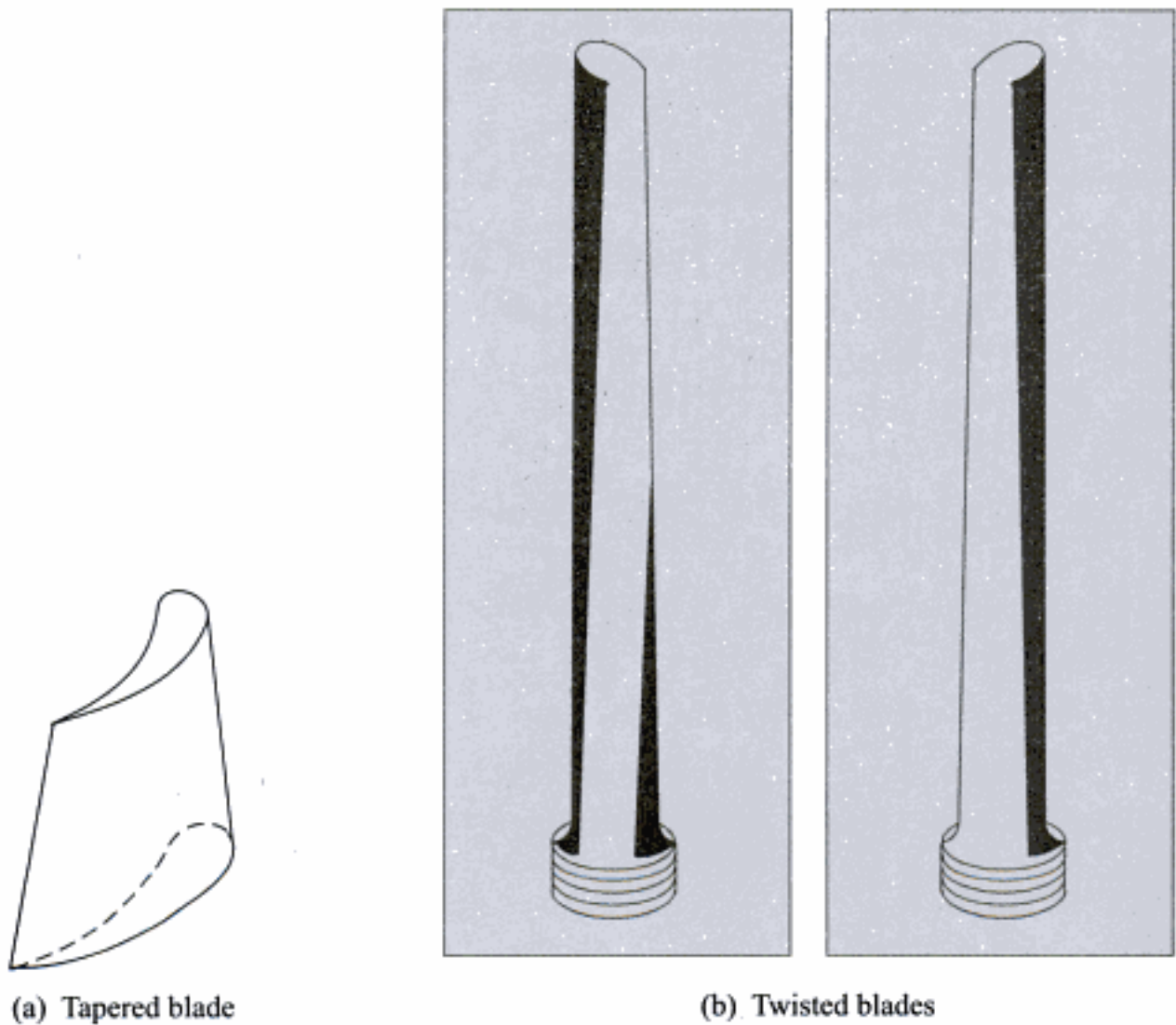
Fig. 7.40 Tapered and twisted blades
