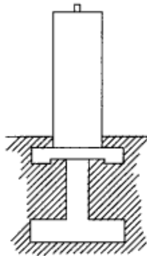
Fig. 7.62 Stradle-T fastening
