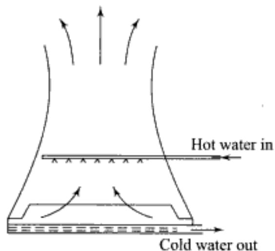
Fig. 8.20(a) Natural draught cooling tower
