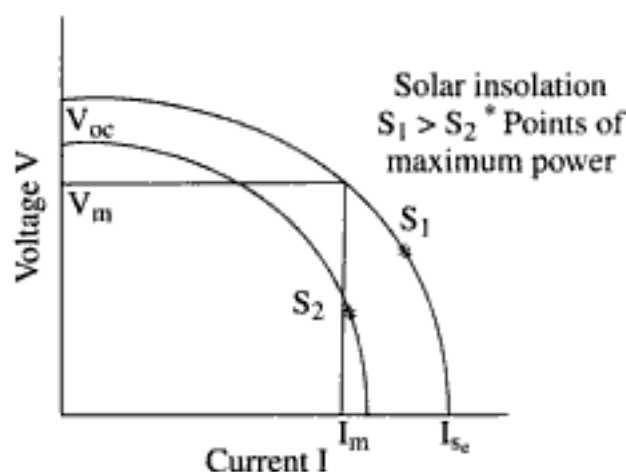
Fig. 14.13 Typical performance characteristics of a silicon solar cell at two solar radiations
