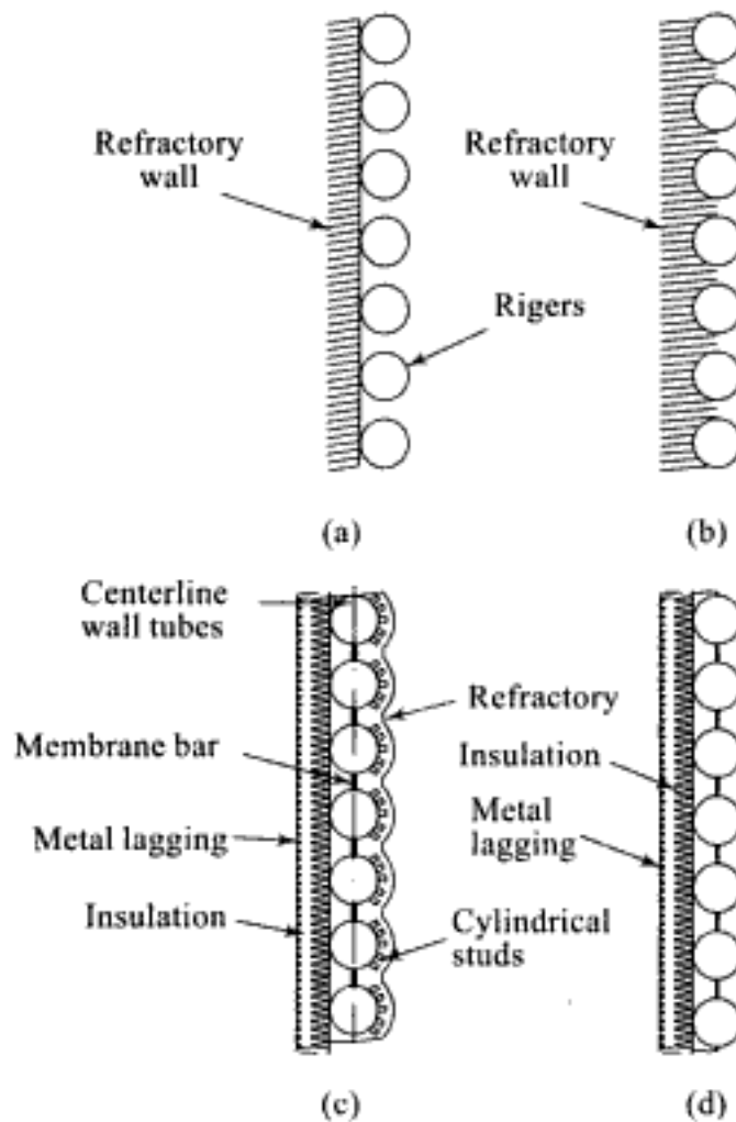
Fig. 6.21 Different types of water-wall: (a) tangent tubes touching the refractory wall, (b) tangent tubes embedded in the refractory, (c) studded tubes, (d) membrane tubes
