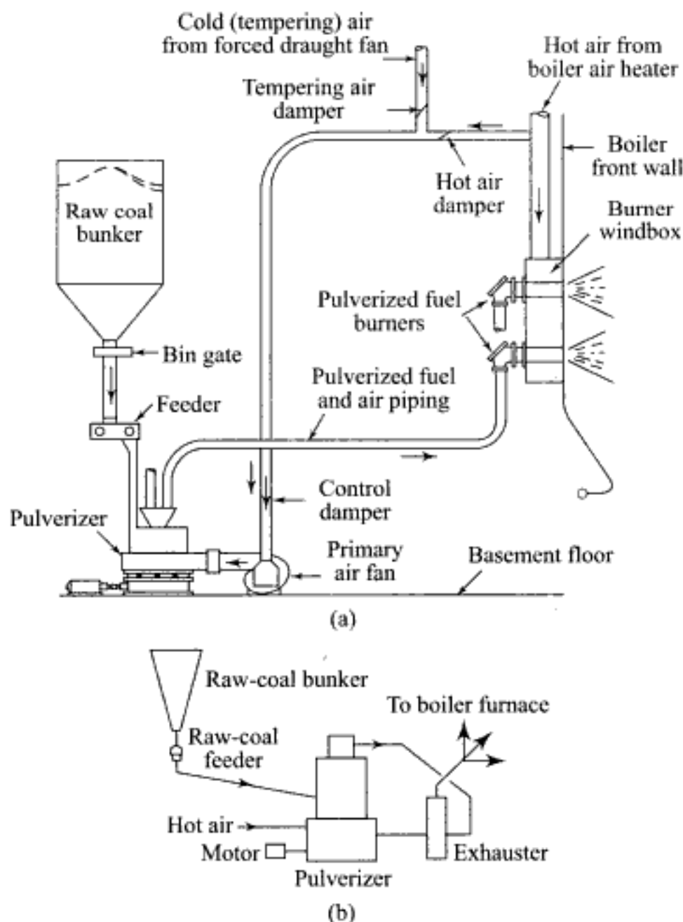
Fig. 5.19 Pulverized coal direct firing system
