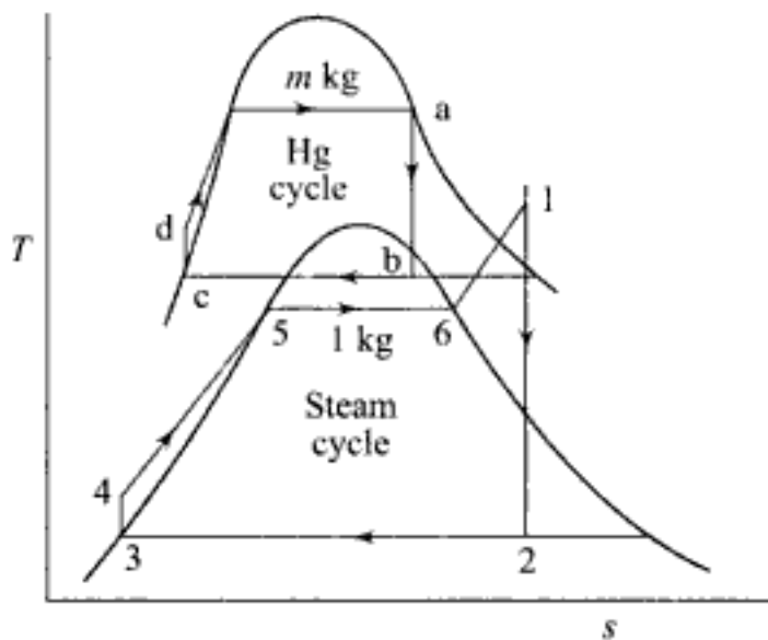
Fig. 3.3 T-s diagram of mercury-steam binary cycle
