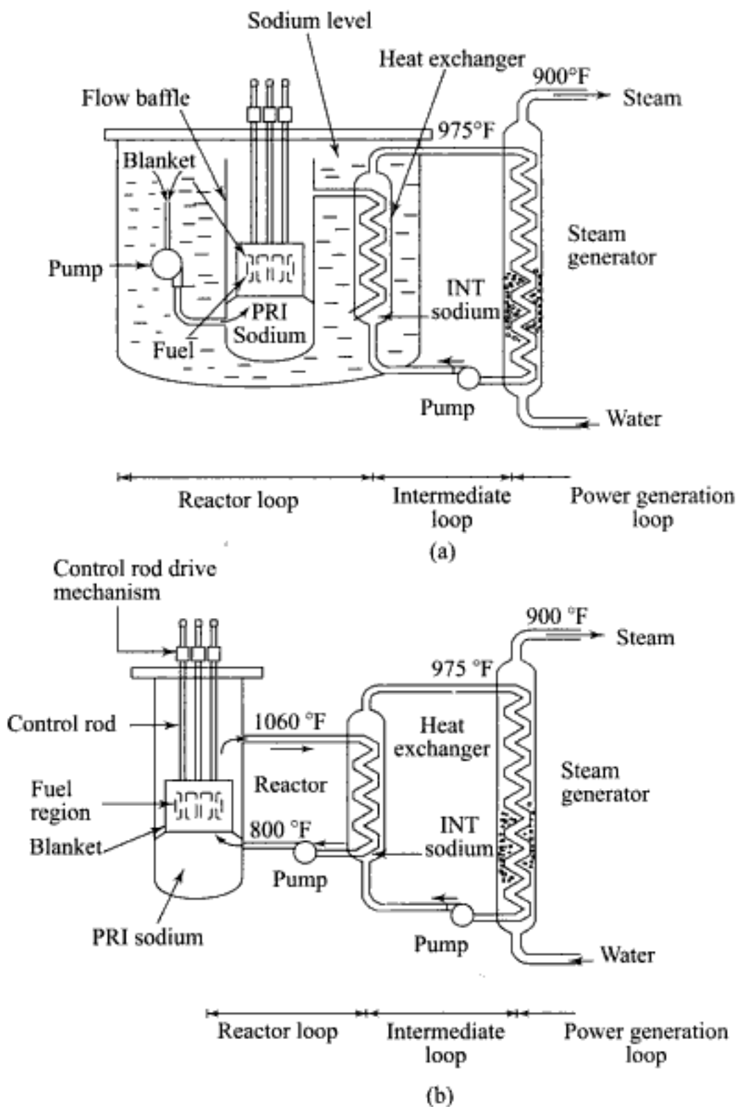
Fig. 9.25 Liquid metal fast breeder reactor (a) Pool type, (b) Loop type
