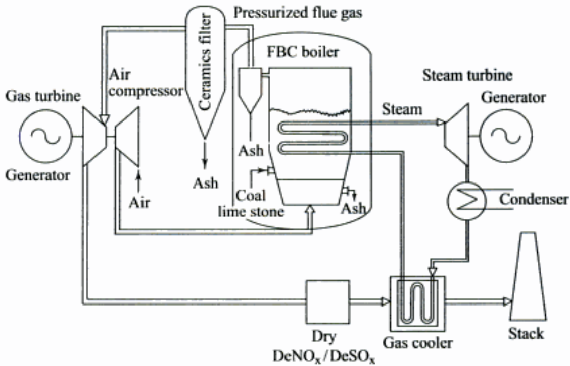
Fig. 5.51 Simplified Cycle of Wakamatsu Plant, Japan
