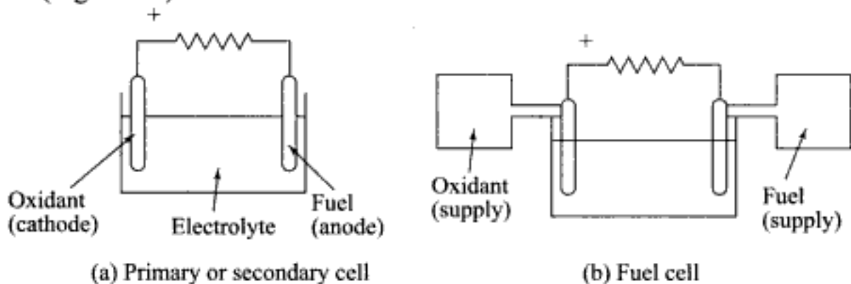
Fig. 12.11 Comparison of a battery and a fuel cell
