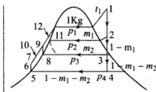
Fig. 2.21 Regenerative feedwater heating with two closed heaters
