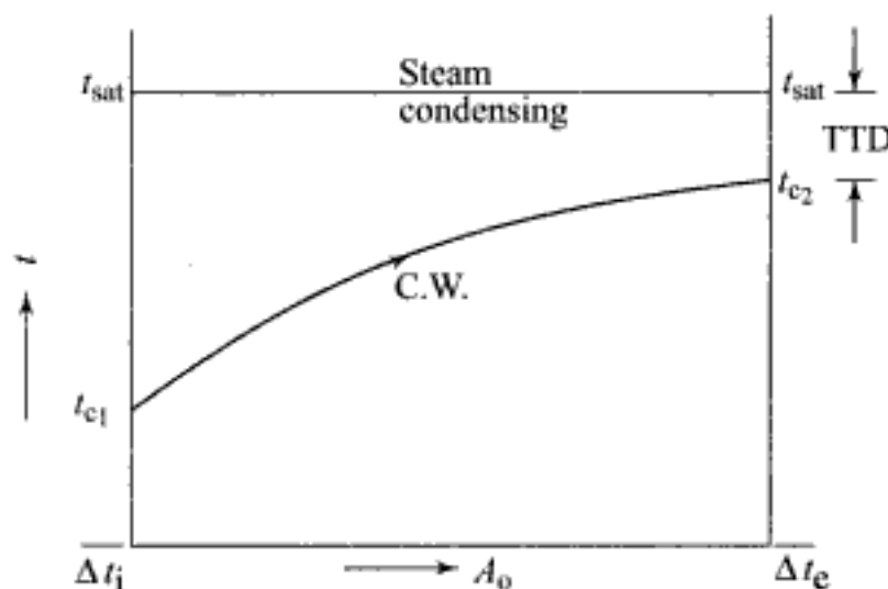
Fig. 8.9 Temperature profiles in a condenser
