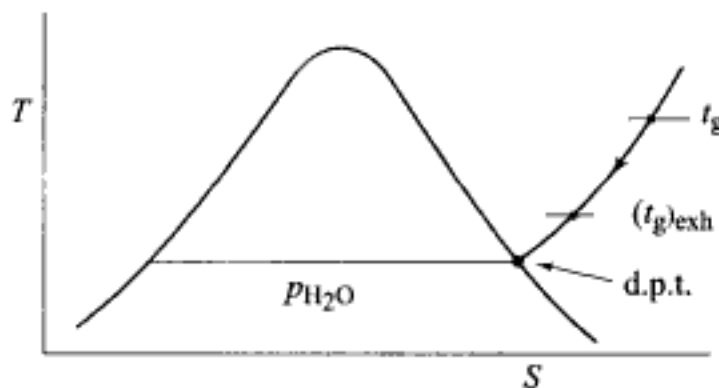
Fig. 4.8 Dew point temperature of the exhaust flue gases
