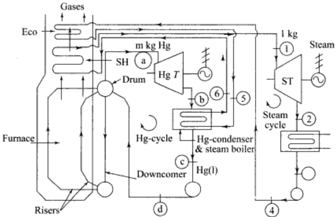
Fig. 3.2 Flow diagram of mercury-steam binary cycle
