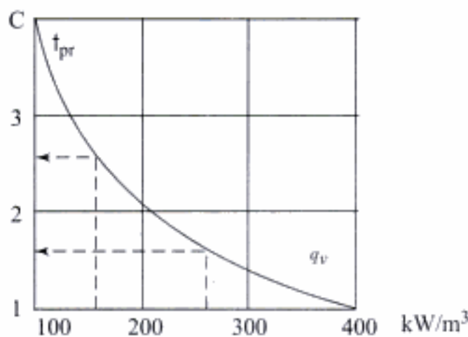
Fig. 5.22 Relation between heat release rate per unit volume ( q_v ) and the time of residence in furnace( t )
