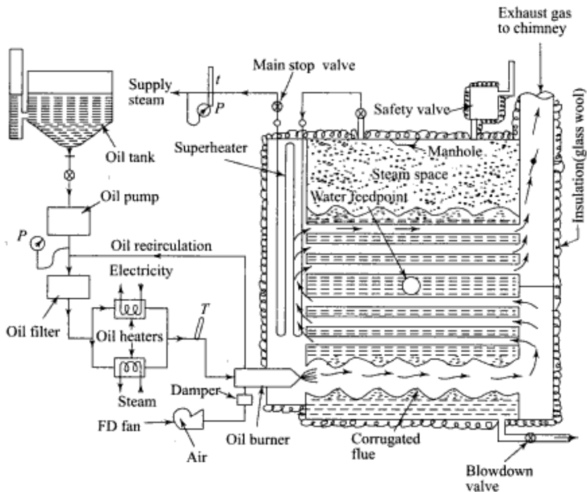
Fig. 6.2 An oil-fired package boiler
