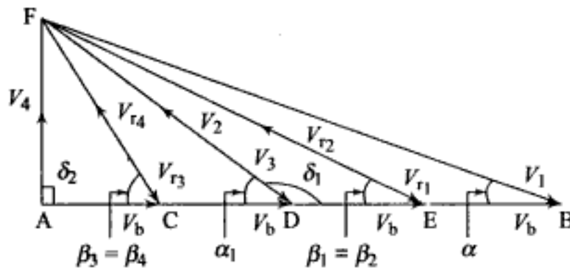
Fig. 7.28 Velocity diagram of a two-row Curtis stage having frictionless symmetrical blading with axial discharge of steam
