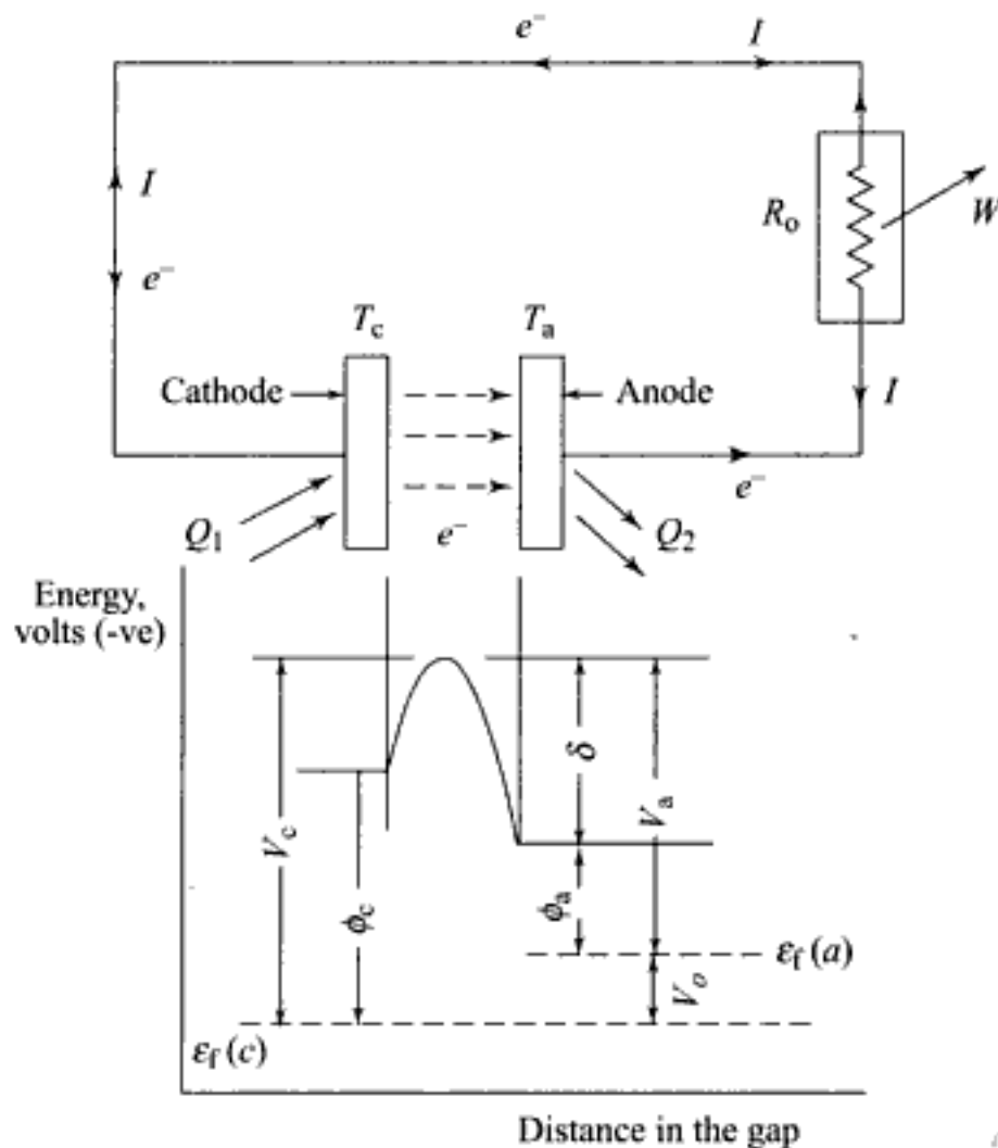
Fig. 13.8 A thermionic generator with interspace retarding potential
