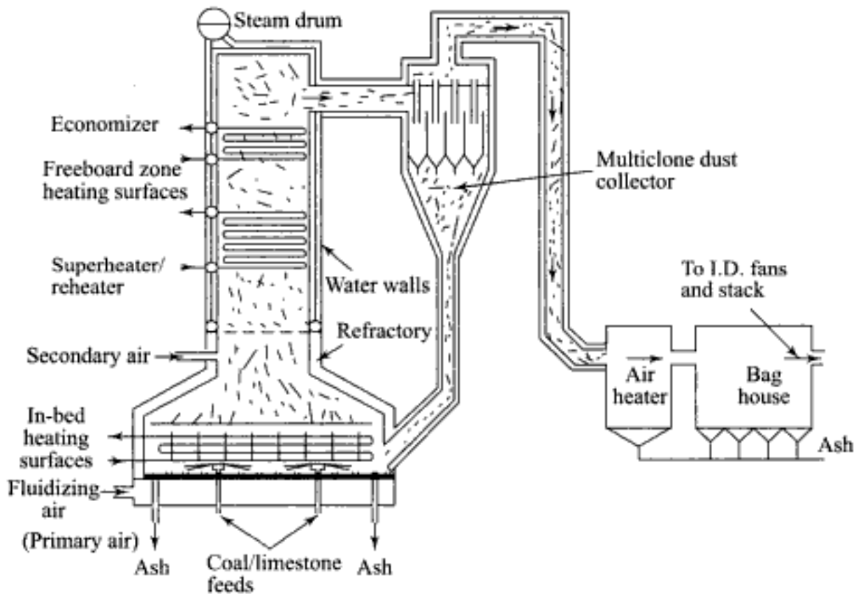
Fig. 6.49 An atmospheric bubbling fluid bed boiler system
