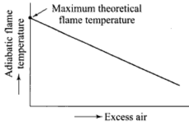
Fig. 4.20 Variation of adiabatic flame temperature with excess air
