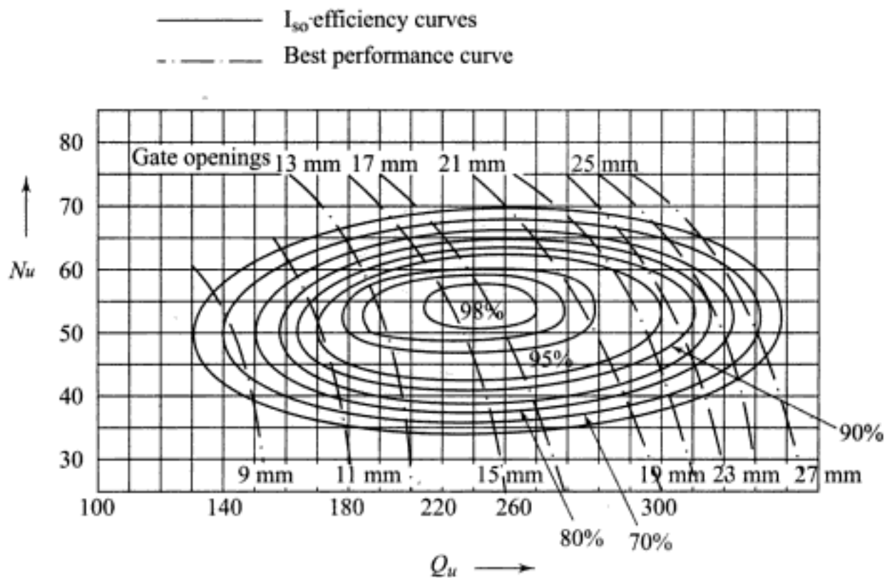
Fig. 10.42 Constant efficiency and best performance curves (universal characteristics) of a Francis turbine
