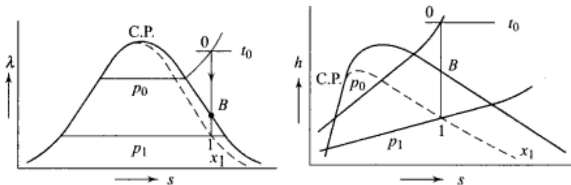
Fig. 7.14 Slow and isentropic expansion of steam from the superheated into the two phase region
