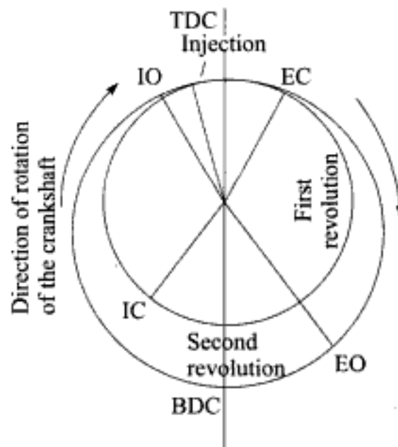
Fig. 11.22 Valve timing diagram for a four-stroke CI engine
