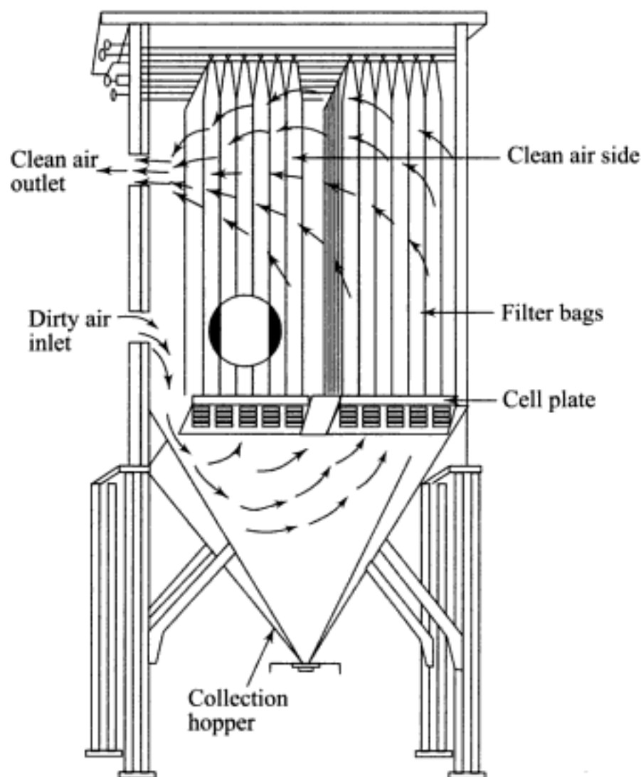
Fig. 6.63 Typical baghouse with mechanical shakers
