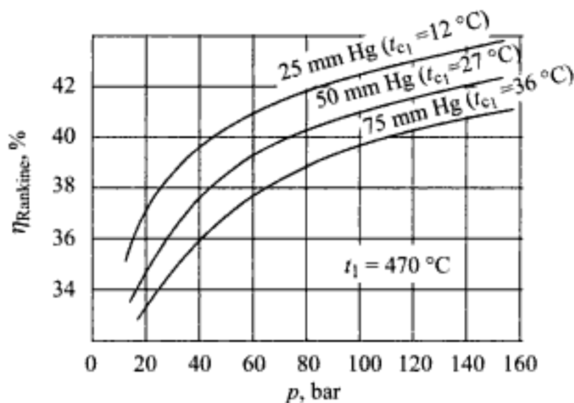
Fig. 2.14 Effect of inlet steam pressure ( p_1 ) and condenser pressure on Rankine efficiency with constant inlet steam temperature of 470^\circ\text{C}
