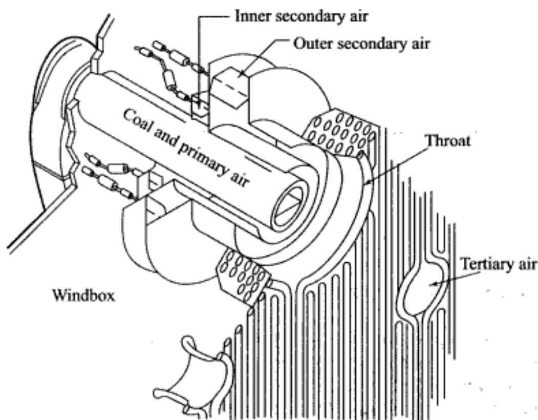
Fig. 5.30(a) Distributed mixing burner (DMB)
