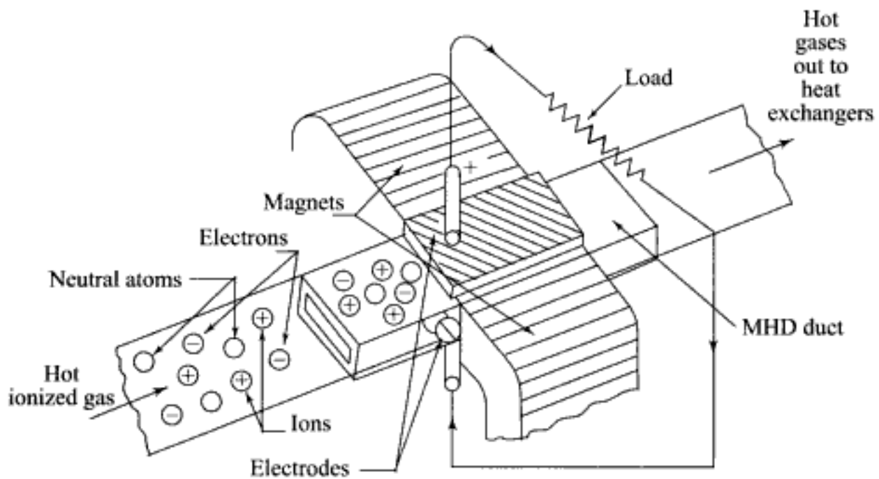
Fig. 13.1 Simplified view of an MHD generator
