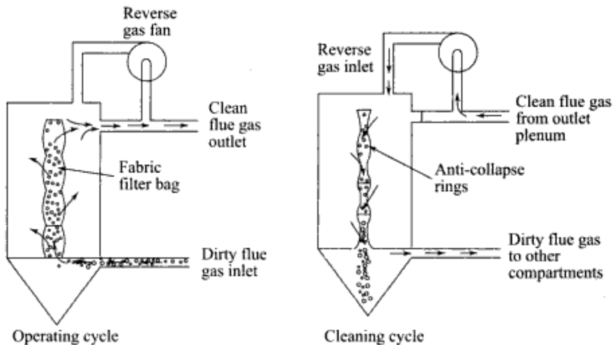
Fig. 6.64 (a) Operating Schematic Reverse Air Fabric Filter
