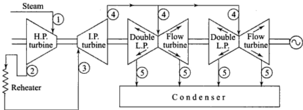
Fig. 7.43 Casing arrangement of a steam turbine having four parallel exhausts
