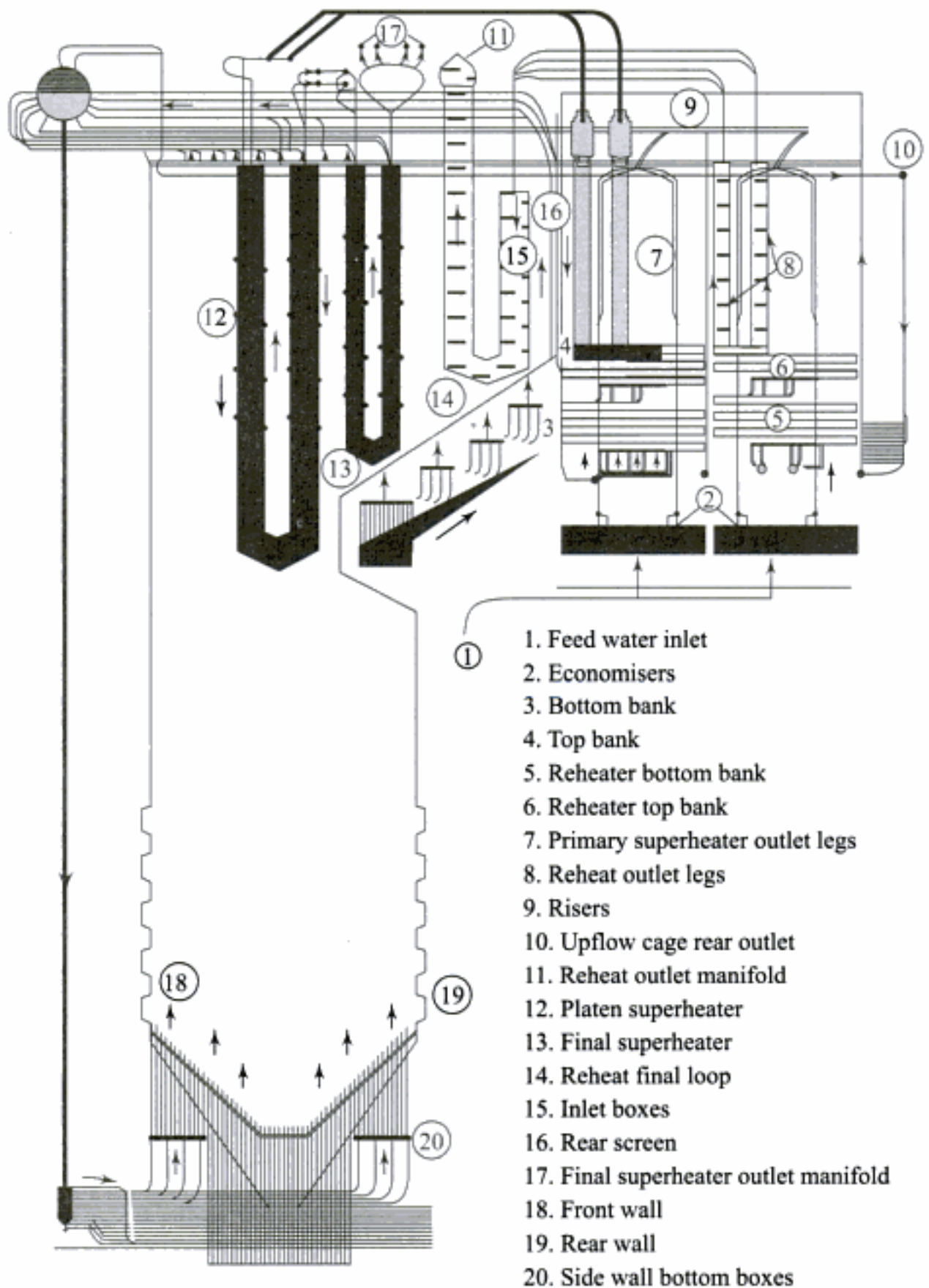
Fig. 6.20 (c) Section through a 660 MW CEGB steam generator
