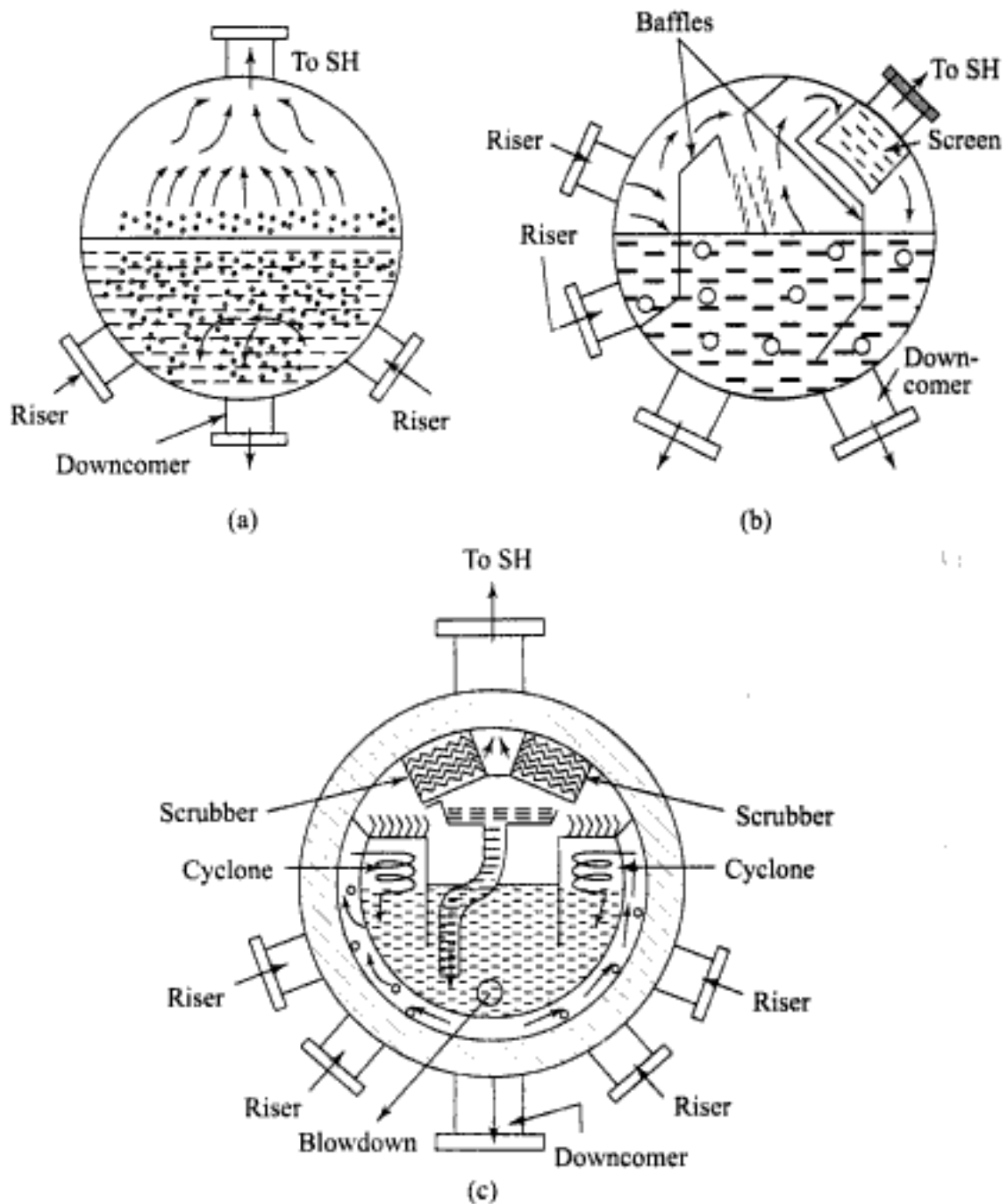
Fig. 6.15 Steam drum separation (a) gravity, (b) baffle and screen, (c) cyclone and scrubber
