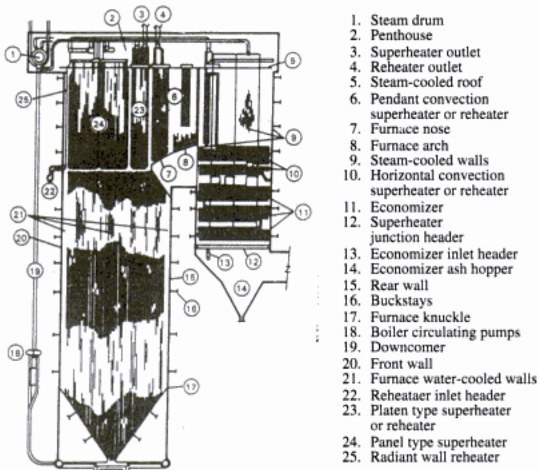
Fig. 6.6 (a) Boiler Nomenclature
