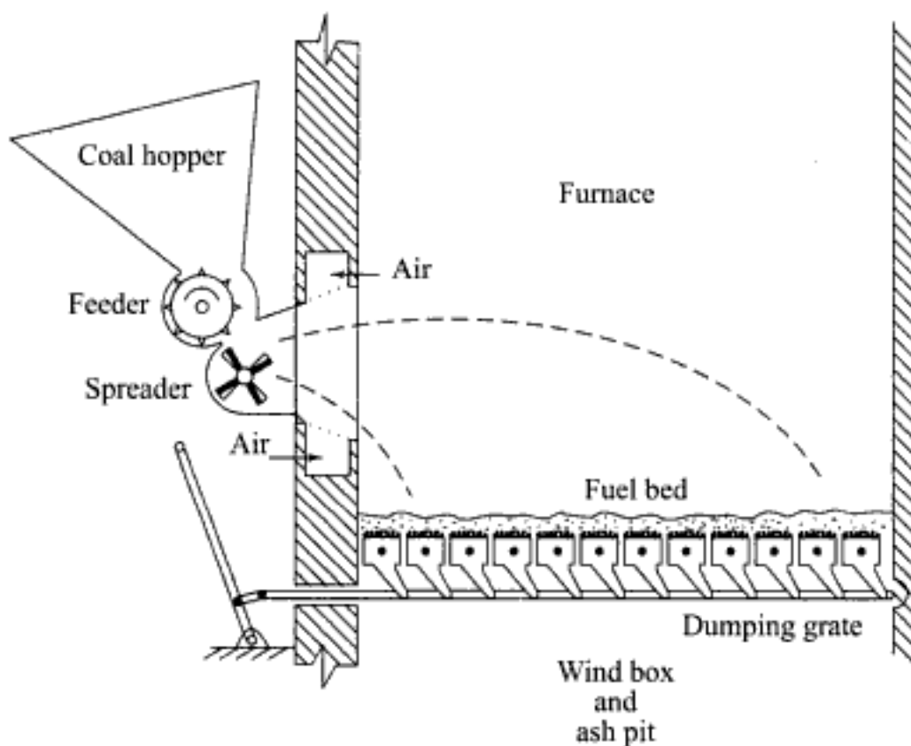
Fig. 5.10 Spreader stoker hurling coal particles into furnace
