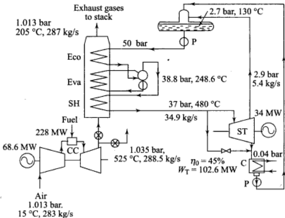
Fig. 3.17 Combined cycle plant with single pressure steam cycle
