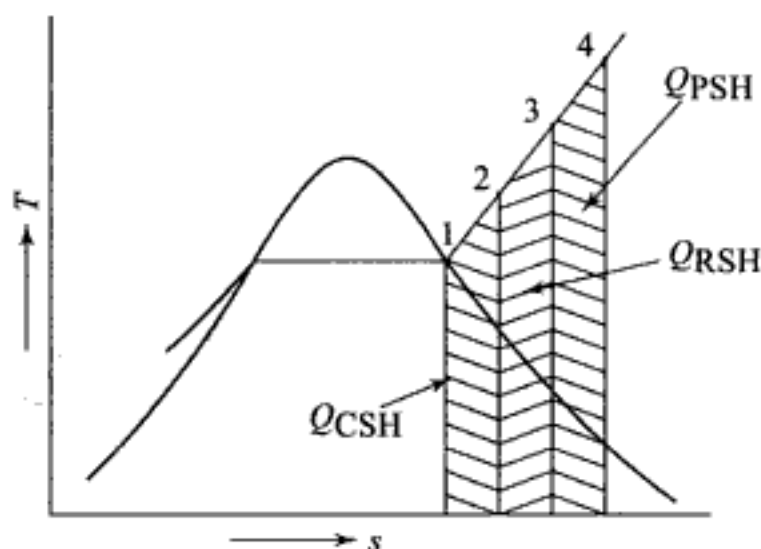
Fig. 6.27 Heat absorption in the three kinds of superheater
