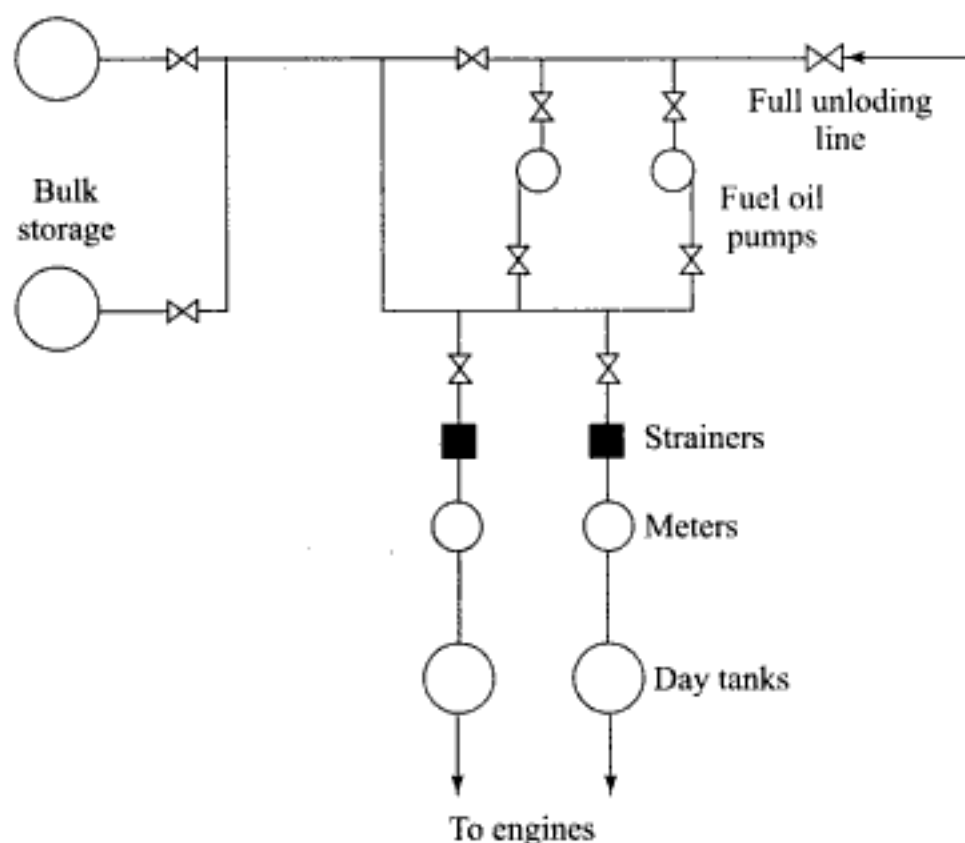
Fig. 11.4 Fuel storage in a diesel engine power plant
