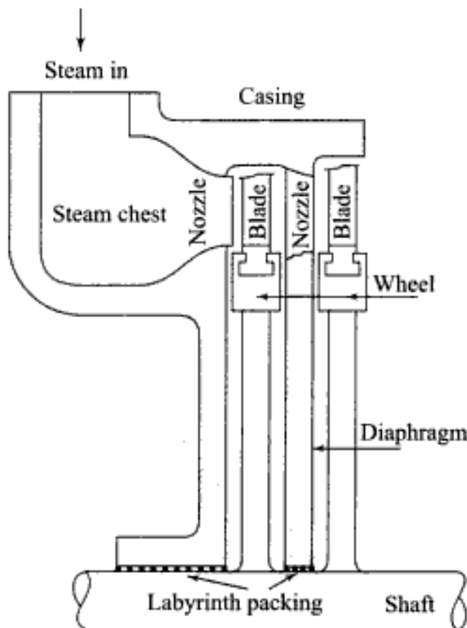
Fig. 7.23 (a) Pressure-compounded impulse turbine
