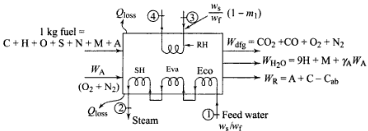
Fig. 4.13 Energy balance of a steam generator
