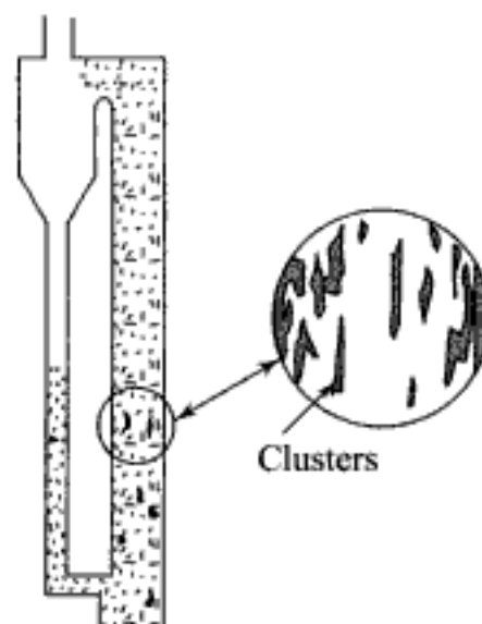
Fig. 5.40 A fast fluidized bed in which solid agglomerates move up and down in a very dilute dispersion of solids
