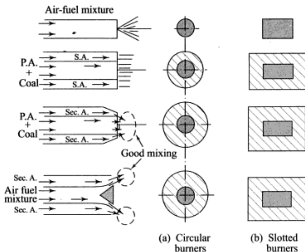
Fig. 5.25 Pulverized coal burners: (a) circular cross-section, (b) rectangular cross-section
