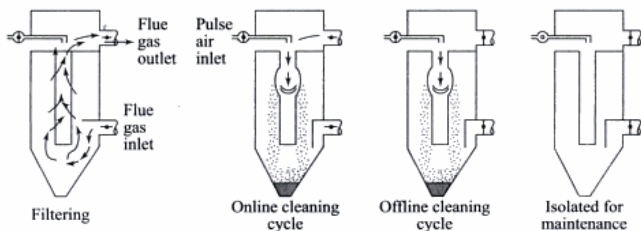
Fig. 6.64 (b) Operating schematic pulse jet fabric filter
