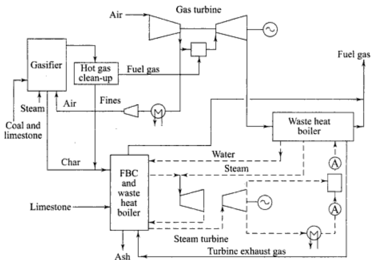
Fig. 5.50 Outline of the Topping Cycle
