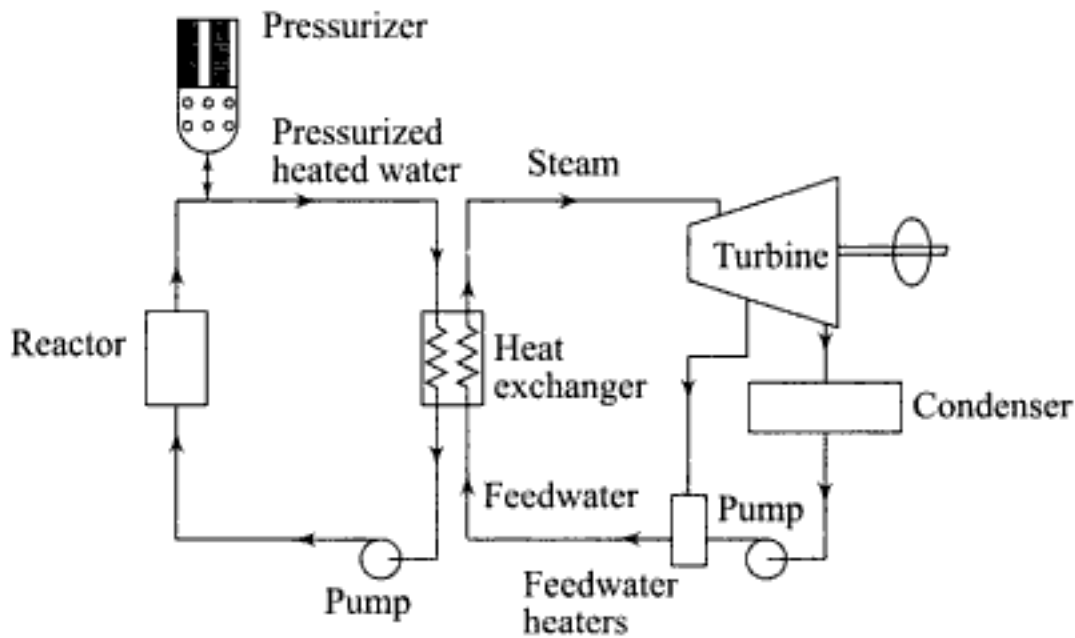
Fig. 9.16 Schematic of a PWR power plant
