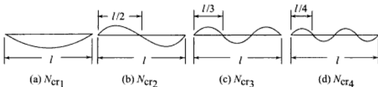
Fig. 7.68 Form of whirling shaft at second, third and fourth critical speeds
