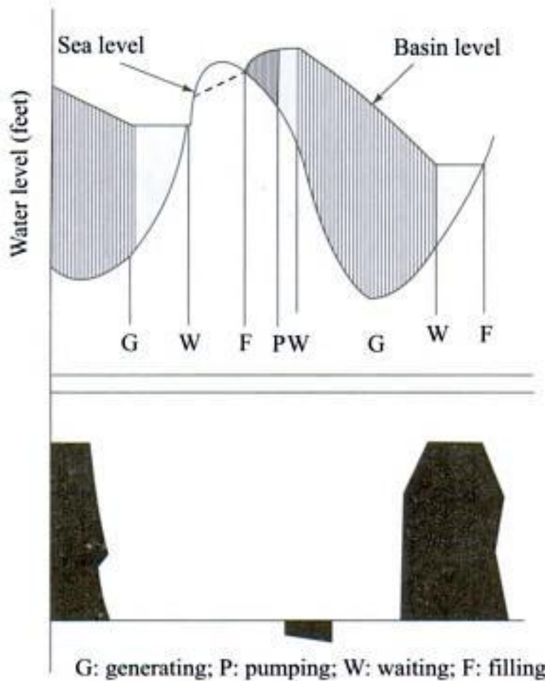
Fig. 14.26 (b) Single basin, single effect tidal power scheme: schematic top view
