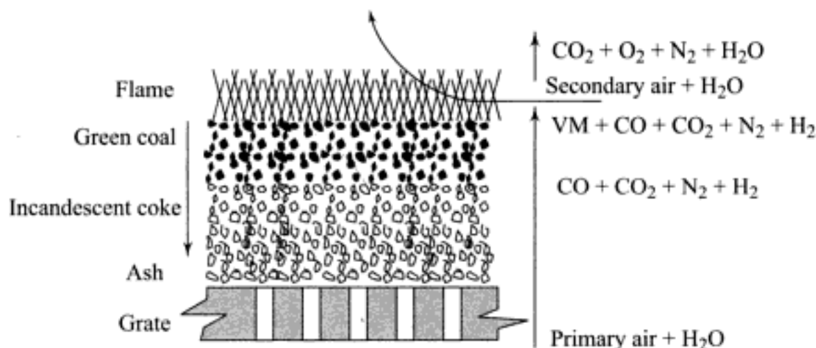
Fig. 5.7 Overfeed fuel bed section receives fresh coal on top surface; ignition plane lies between green coal and incandescent coke
