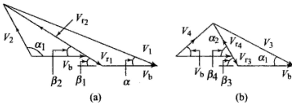
Fig. 7.27 Two-row Curtis stage with symmetrical blades: (a) first row of moving blades, (b) second row of moving blades
