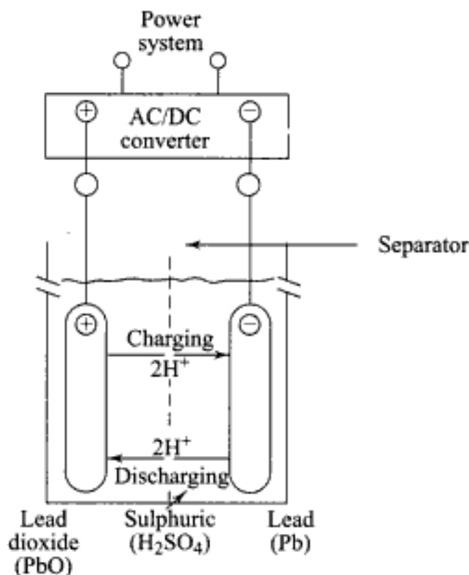
Fig. 12.13 Lead-acid storage battery
