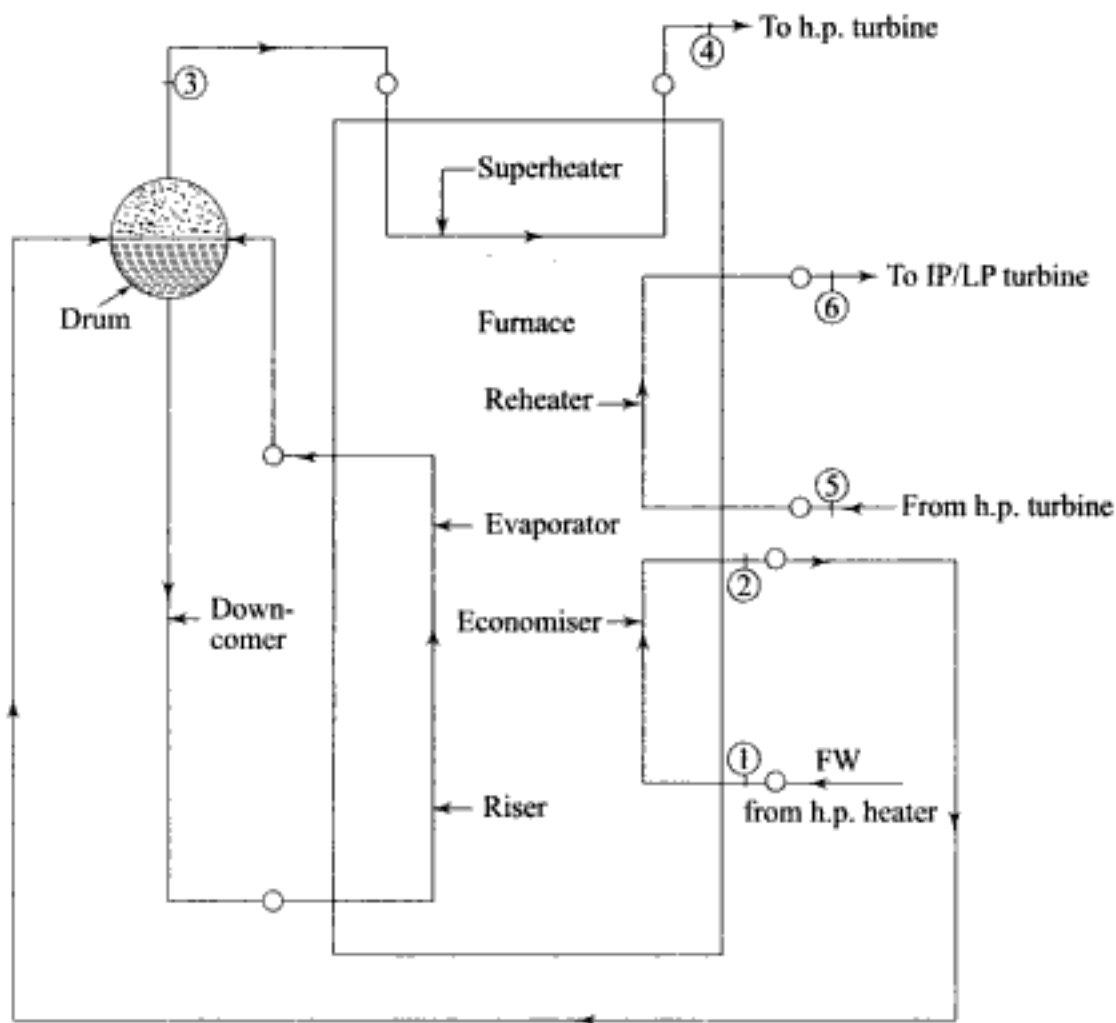
Fig. 6.7(a) Heat absorption in a water-tube boiler
