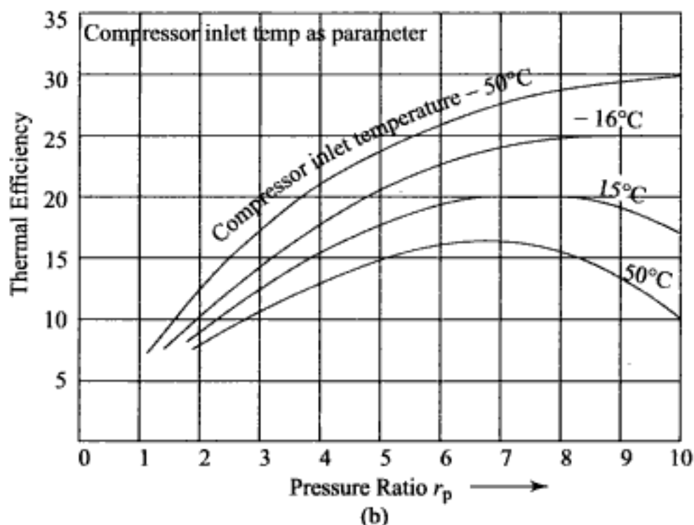
Fig. 11.51 Effect of pressure ratio on thermal efficiency of a simple open cycle plant with (a) Turbine inlet temperature and (b) Compressor inlet temperature as parameters
