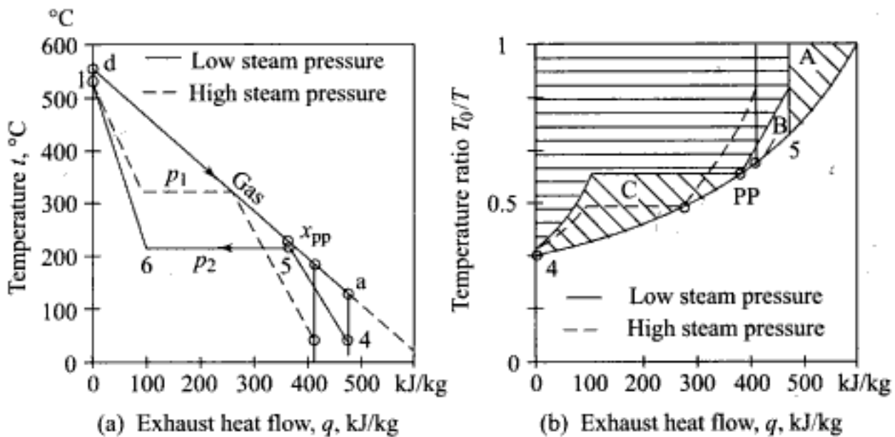
Fig. 3.12 Effect of live steam pressure on energy utilization and overall energy loss
