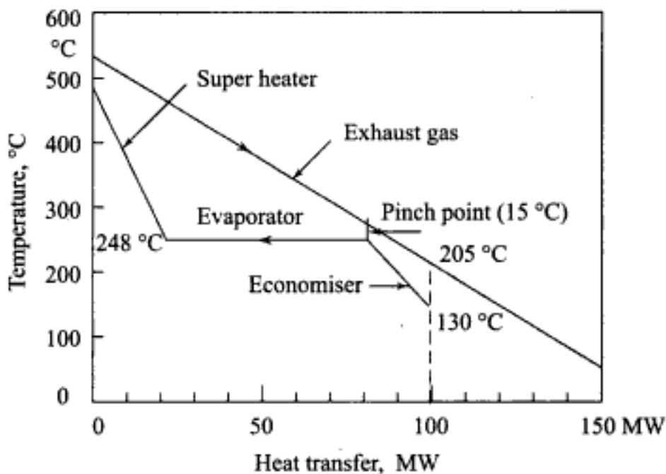
Fig. 3.18 Temperature profiles of exhaust gas and water-steam along with heat absorption rates
