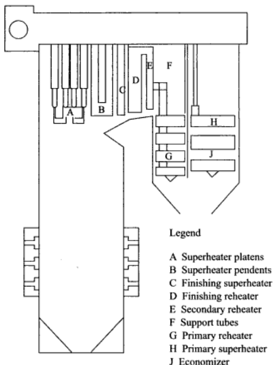
Fig. 4.6 Example of steam generator surface arrangement
