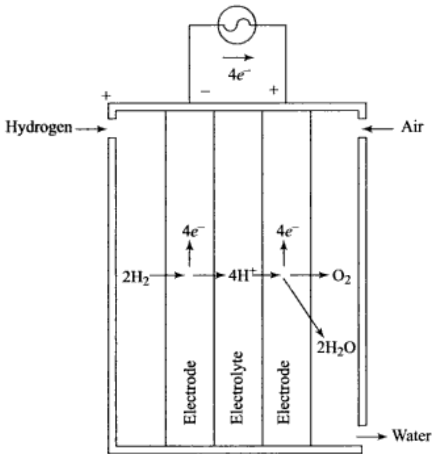
Fig. 13.23 Hydrogen-oxygen fuel cell, Type A
