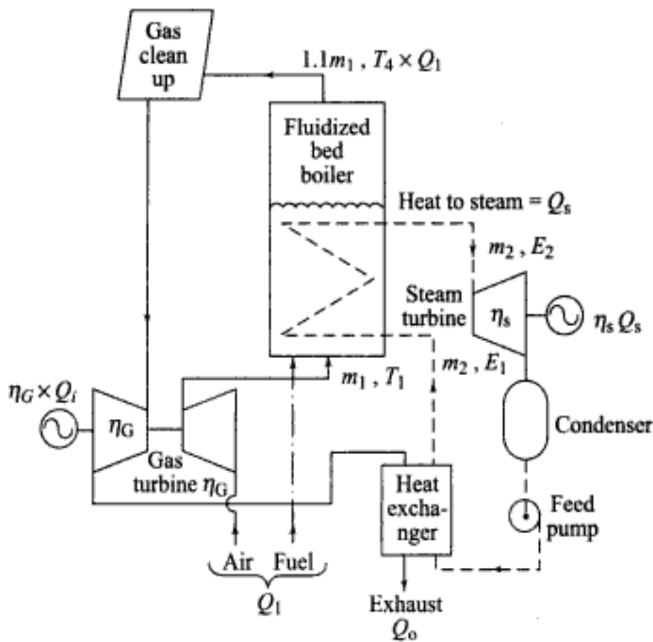
Fig. 5.47 A combined cycle plant with a pressurized fluidized bed combustor (PFBC)
