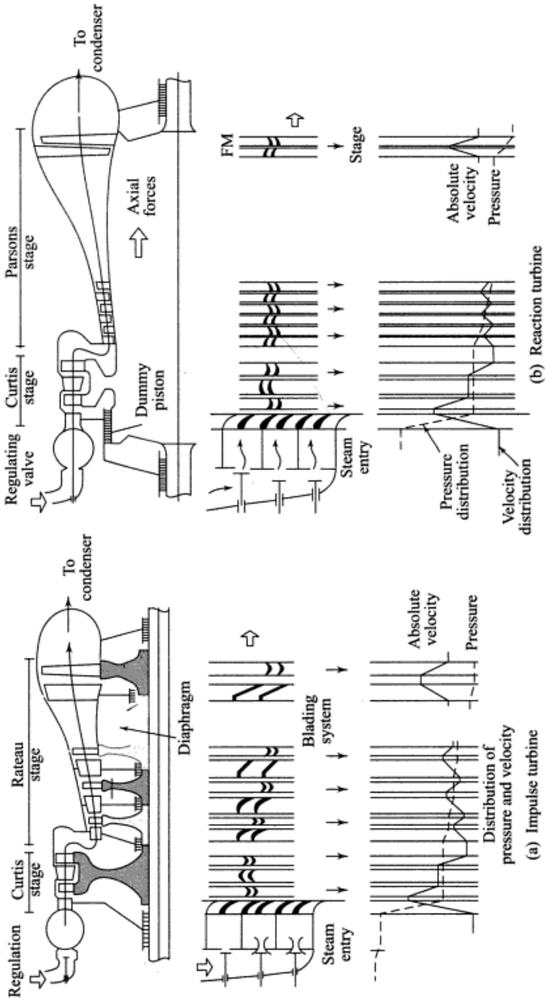
Fig. 7.35 Layouts of impulse and reaction steam turbines
