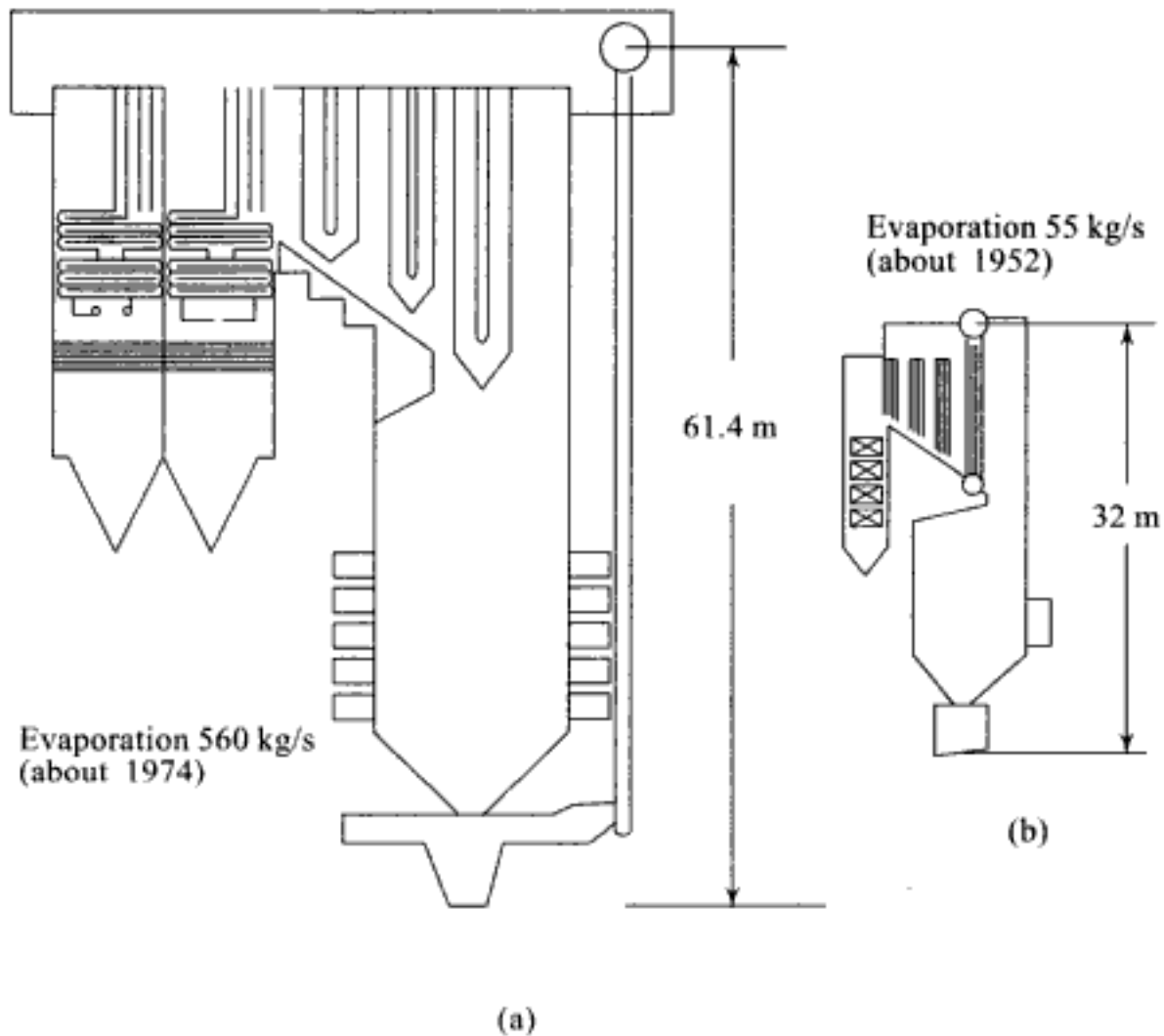
Fig. 6.20 (e) Comparison of fossil fuel-fired steam generators over 25 years
