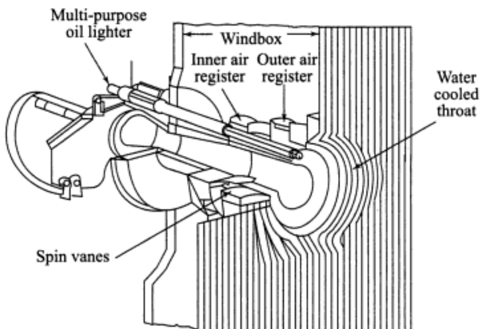
Fig. 5.32 (a) Multifuel burner for pulverized coal, oil and gas
