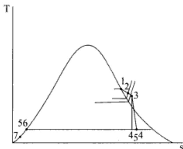
Fig. 14.33 T-s diagram of the cycle shown in Fig. 14.32
