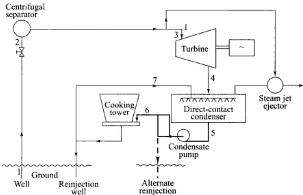
Fig. 14.32 Schematic of a vapour-dominated powerplant
