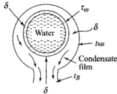
Fig. 8.7 Film condensation of steam on a horizontal tube
