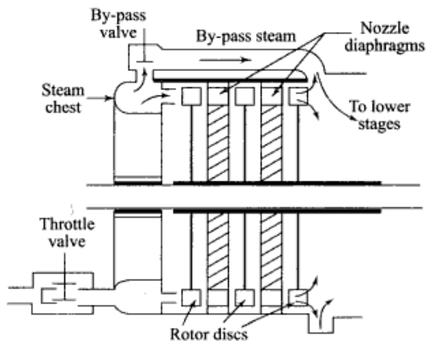
Fig. 7.55 By-pass governing
