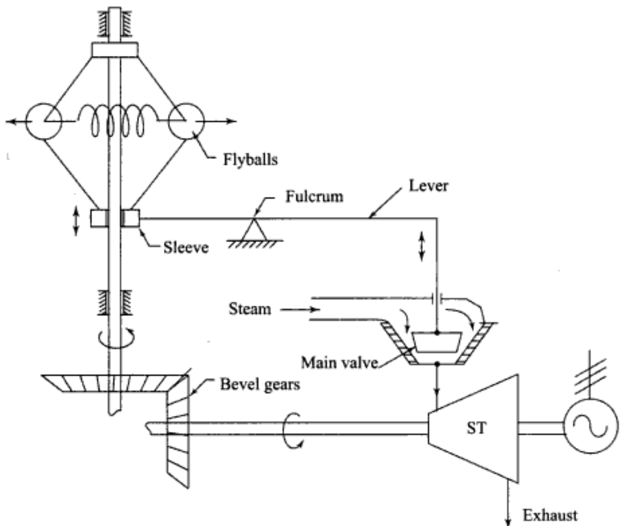
Fig. 7.50 Centrifugal flyball governor
