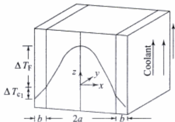
Fig. 9.12 Temperature distribution in a plate type fuel element
