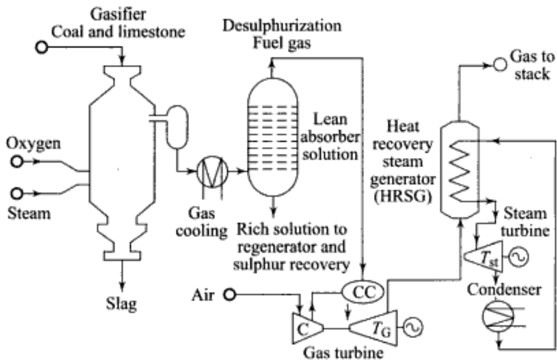
Fig. 3.23 Gasifier combined plant (IGCC)
