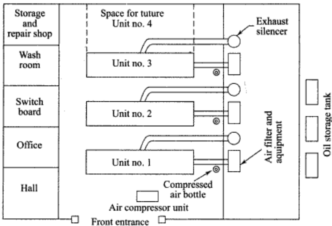
Fig. 11.37 Typical layout of a diesel engine power plant
