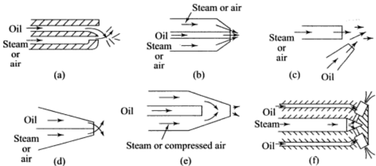
Fig. 5.62 Steam- or air-atomised oil burners
