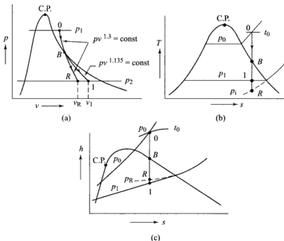
Fig. 7.16 Supersaturated flow on (a) p - v , (b) T - s and (c) h - s diagrams
