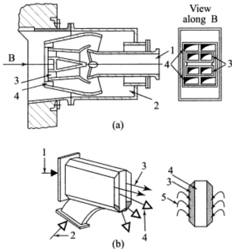
Fig. 5.26 Straight-flow burners for pulverized coal: (a) with tilting nozzle at the exit of fuel-air mixture; (b) with central channel for hot air; 1- supply of fuel-air mixture; 2-supply of hot air; 3-fuel-air mixture outlet; 4-hot air outlet; 5-suction of furnace gases
