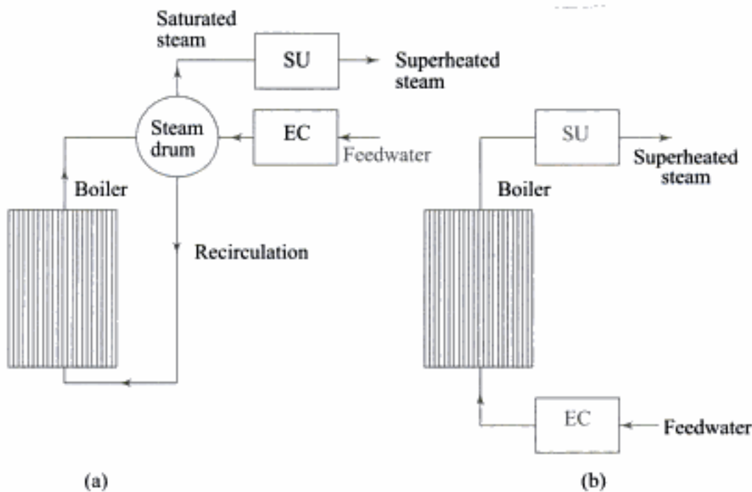
Fig. 6.23 Schematic flow diagram of (a) drum type and (b) once-through steam generators. SU = superheater, EC = economiser
