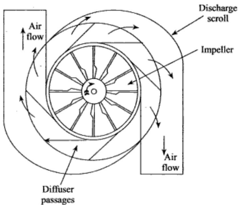
Fig. 11.54 Centrifugal compressor showing discharge scroll
