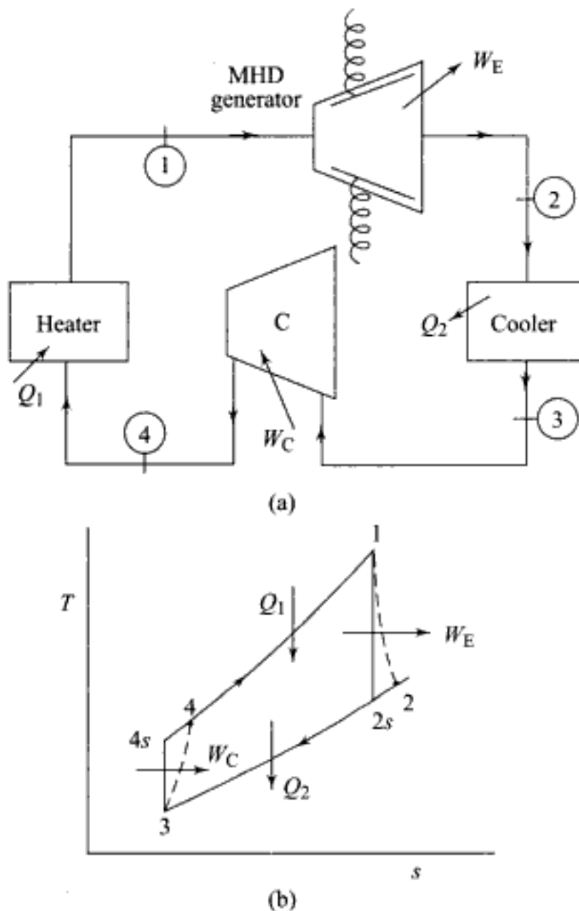
Fig. 13.2 MHD plant as a cyclic heat engine
