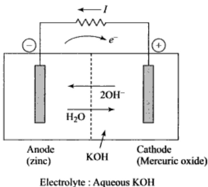
Fig. 13.20 Typical electric battery
