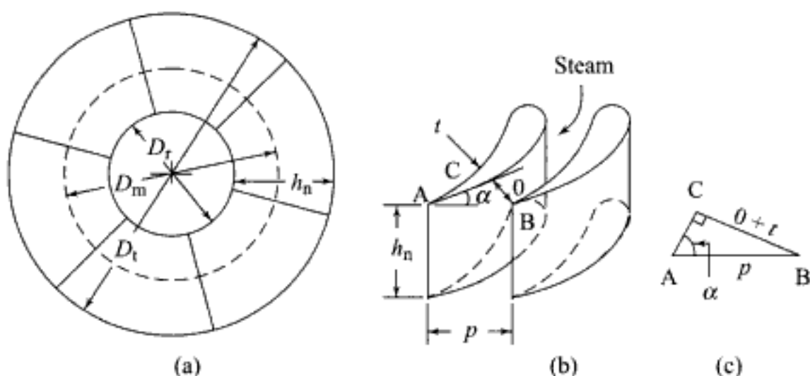
Fig. 7.38 Flow through a nozzle passage
