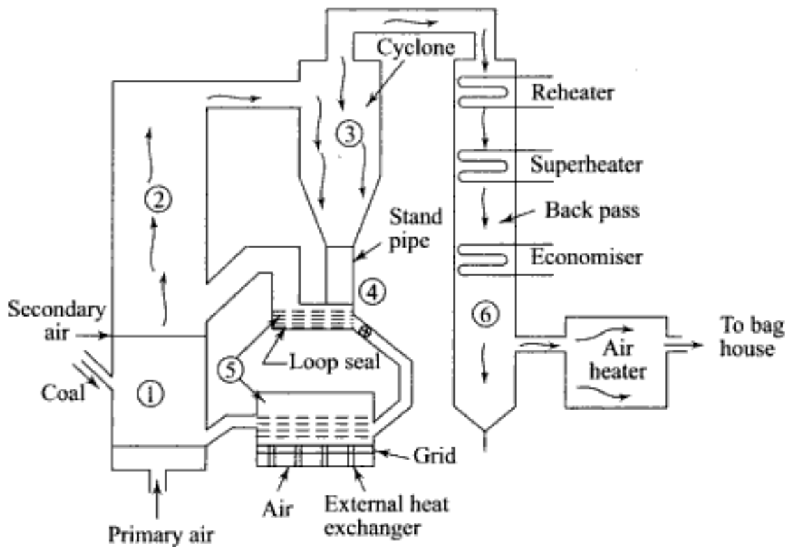
Fig. 6.51 Flow regimes in a CFB boiler: 1. Turbulent/bubbling fluidized bed, 2. Fast fluidized bed 3. Swirl flow, 4. Moving packed bed, 5. Bubbling fluidized bed, 6. Pneumatic transport
