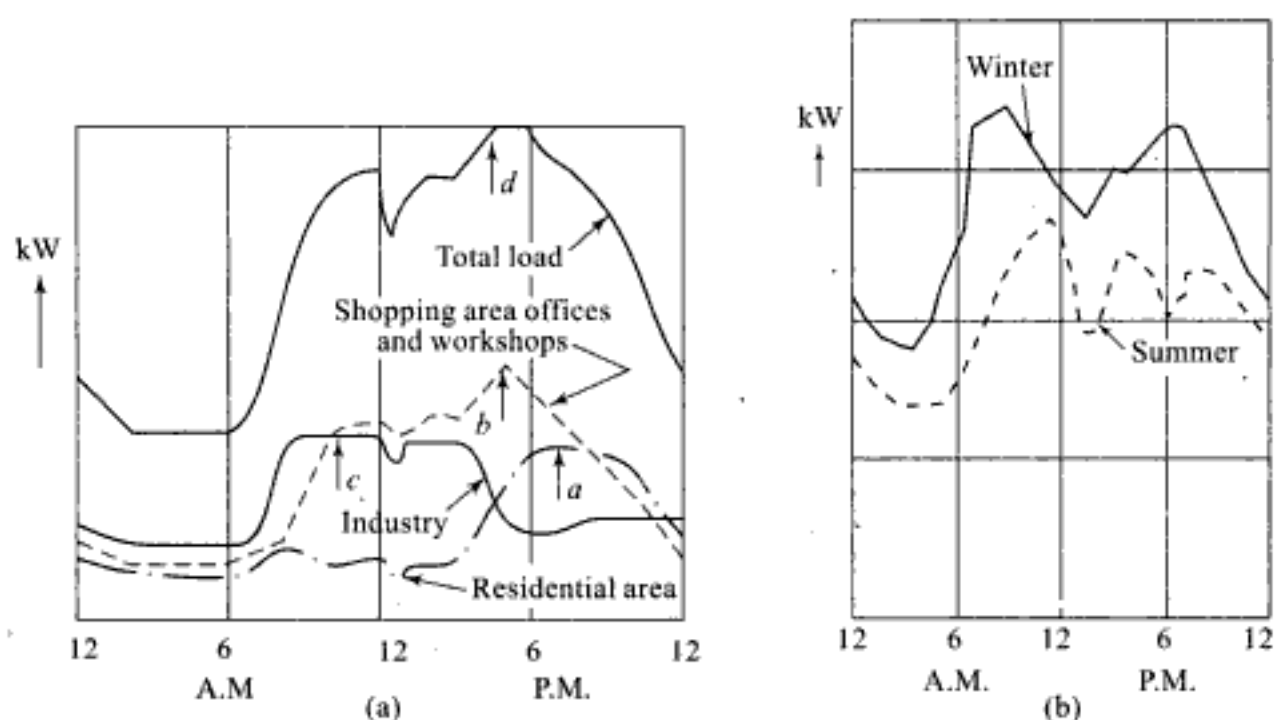
Fig. 1.3 (a) Diversity of loads of consumer groups (b) Load curves of an industrialized country on typical winter and summer week-days
