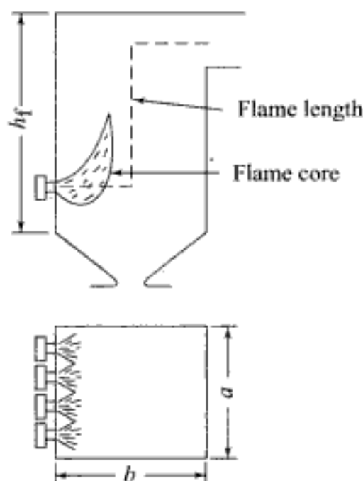
Fig. 5.21 Main dimensions of a furnace
