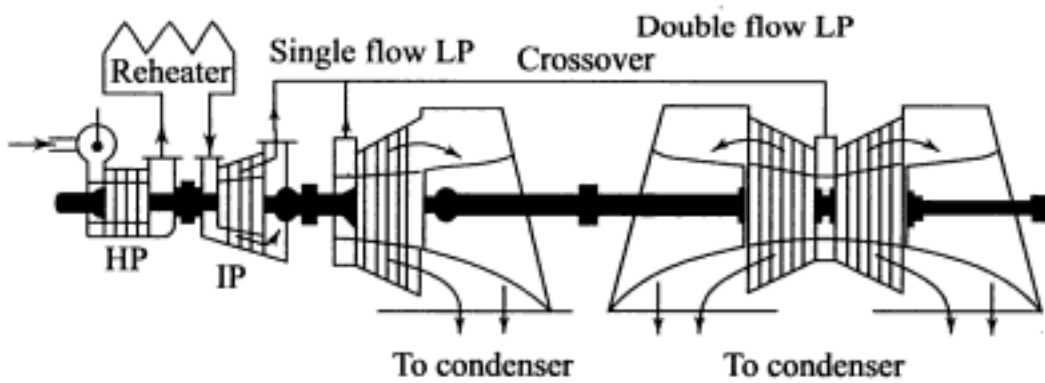
(F) Triple flow low pressure turbine cycle
