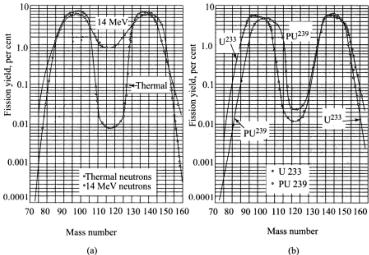
Fig. 9.6 Fission product data for (a) U-235 by thermal and 14 MeV neutrons, and (b) U-233 and Pu-239 by thermal neutrons
