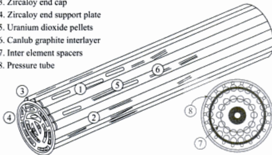
Fig. 9.27 CANDU fuel element assembly
