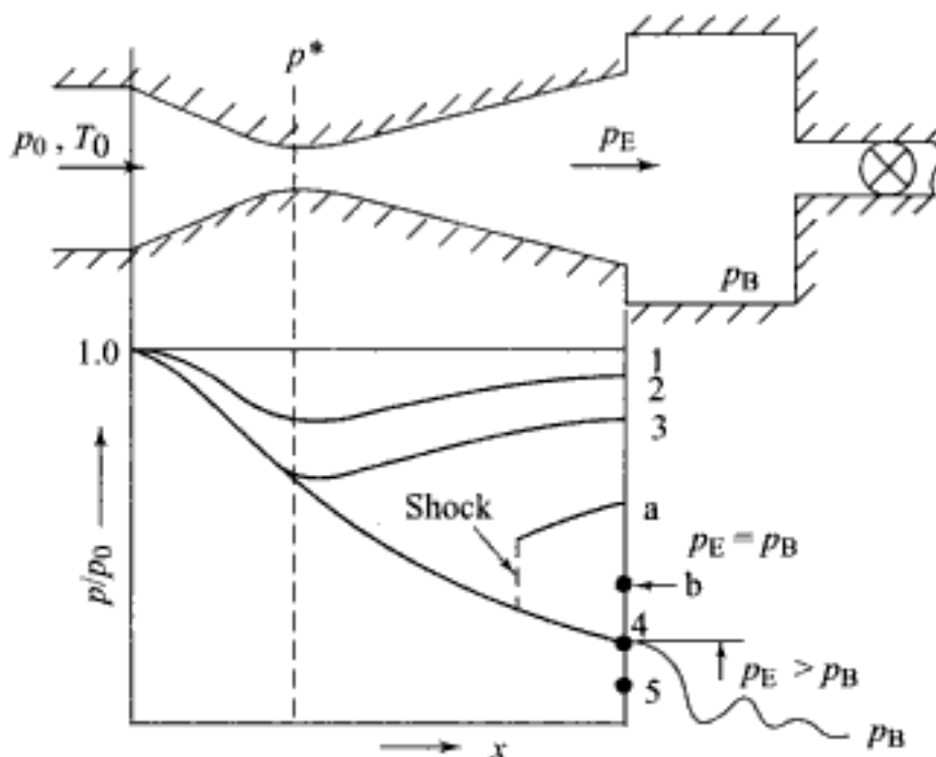
Fig. 7.13 Pressure distribution in a convergent-divergent nozzle
