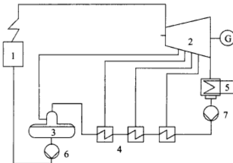
Fig. 3.27 Steam Power plant before conversion to a combined cycle plant
