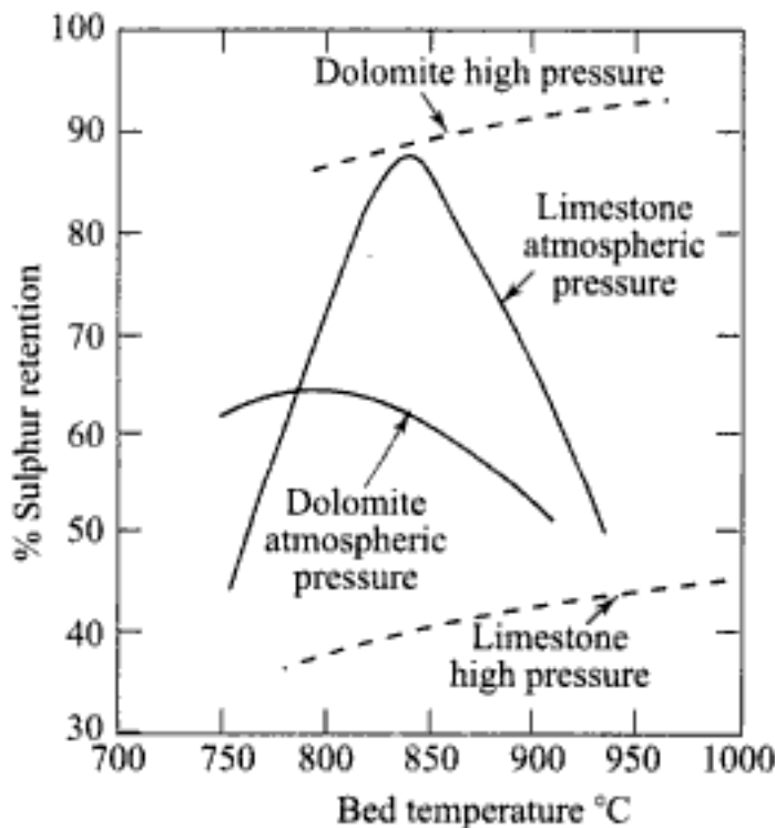
Fig. 6.55 (b) Effect of pressure on sulphur retention for reactive limestone and dolomites sized 0-1600 \mu\text{m} , normalized to Ca/S = 2 and reaction time = 0.5 s
