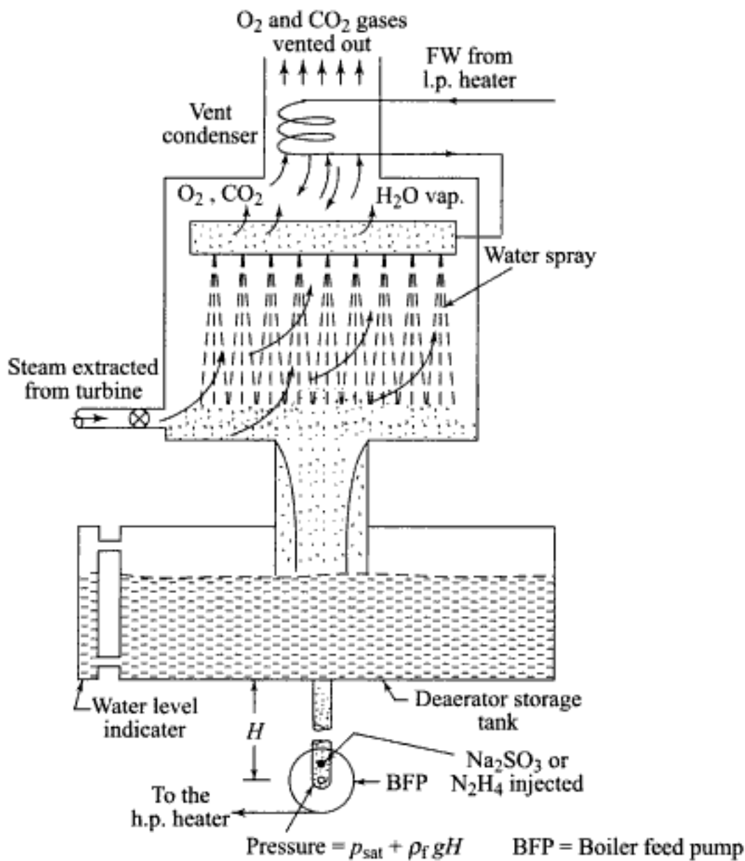
Fig. 2.30 Deaerator with storage tank
