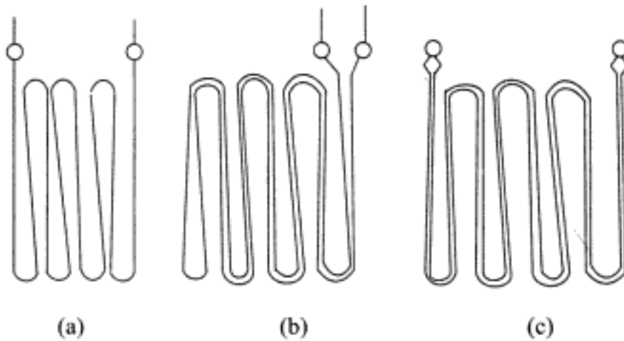
Fig. 6.31 Types of superheater coils: (a) single coil, (b) double coil one tube, (c) double coil two-tube
