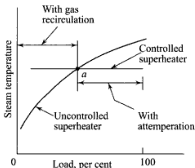
Fig. 6.43 Gas recirculation and attemperation in series
