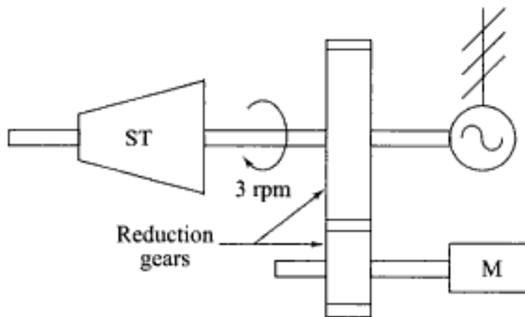
Fig. 7.69 Turning gear operation during start-up and shut-down
