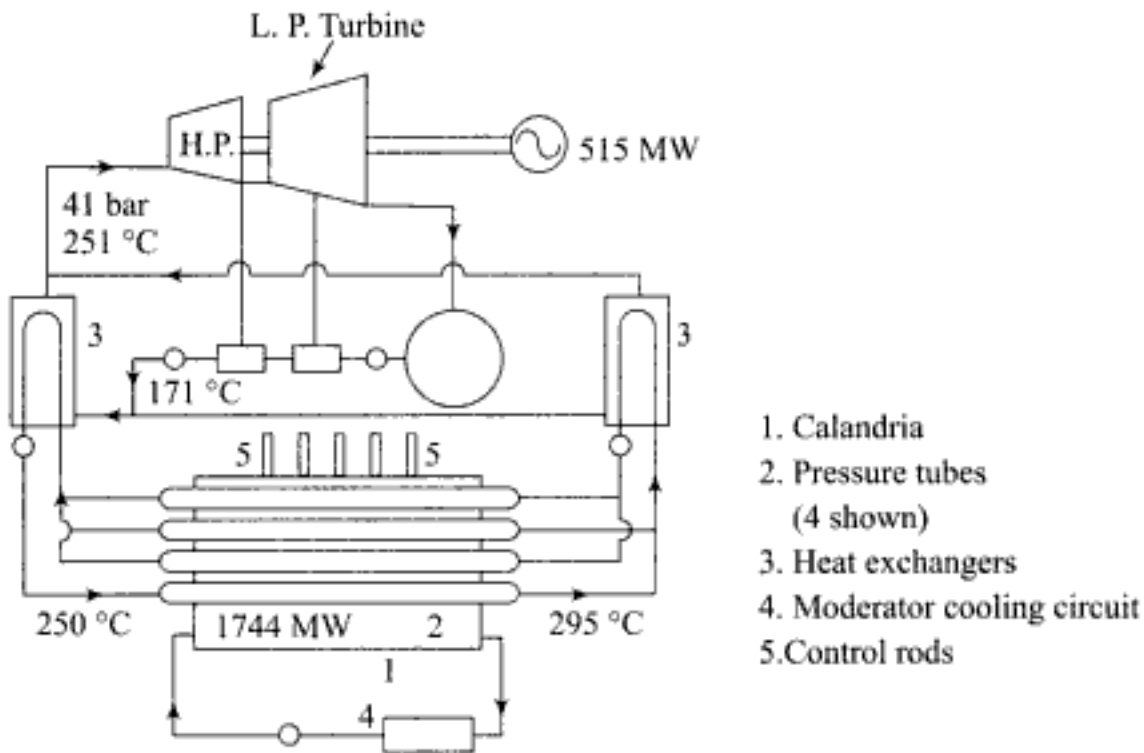
Fig. 9.26 Layout of the calandria, heat exchangers and simplified steam cycle of the CANDU reactor
