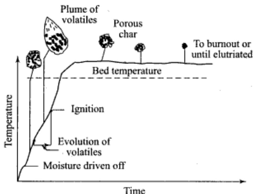
Fig. 5.45 Temperature history of a single fuel particle introduced into a fluidized bed combustor
