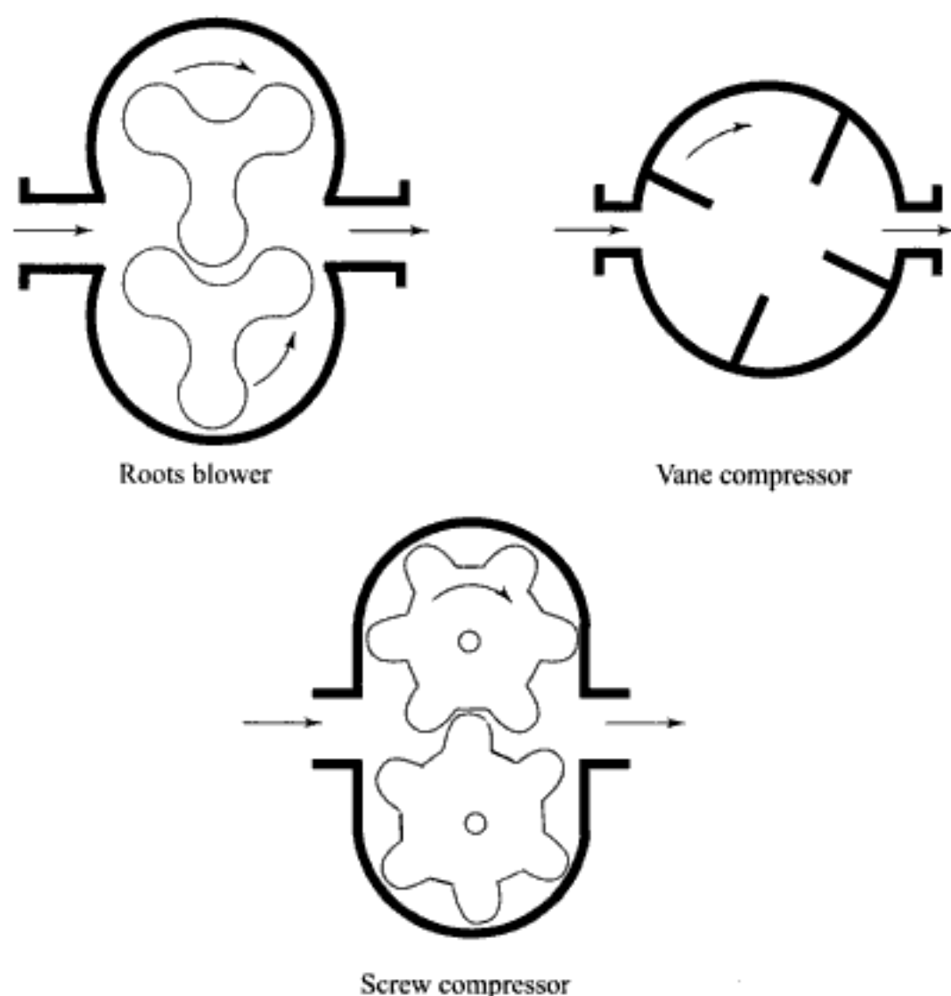
Fig. 11.33 Types of positive displacement compressor
