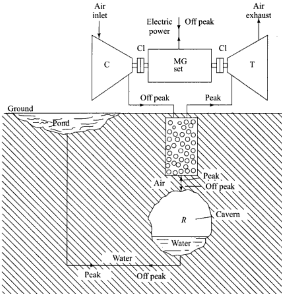
Fig. 12.6 Simple single-stage adiabatic compressed air energy storage system with pressure compensation pond
