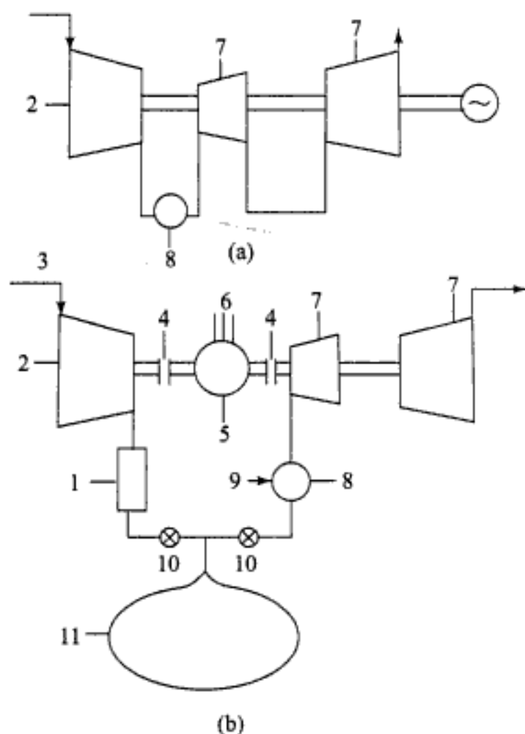
Fig. 12.7 Development of the CAES concept (a) Simple gas turbine cycle (b) Gas turbine cycle modified to CAES configuration
