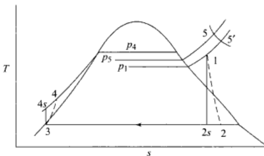
Fig. 2.6 Internally irreversible Rankine cycle
