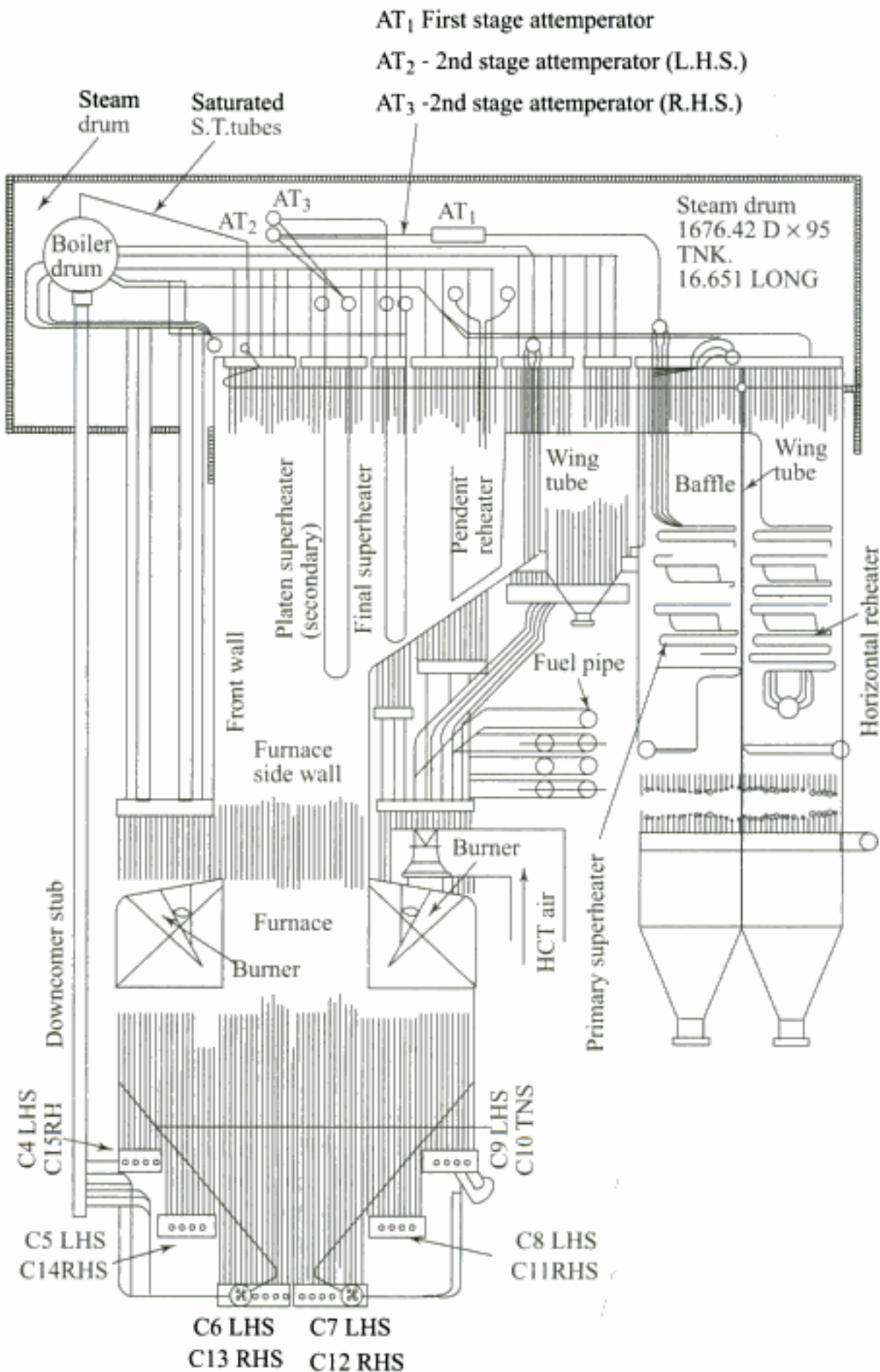
Fig. 6.20 (b) Cross-section of a 210 MW Babcock down-fired steam generator (Bokaro 'B' thermal power plant, DVC)
