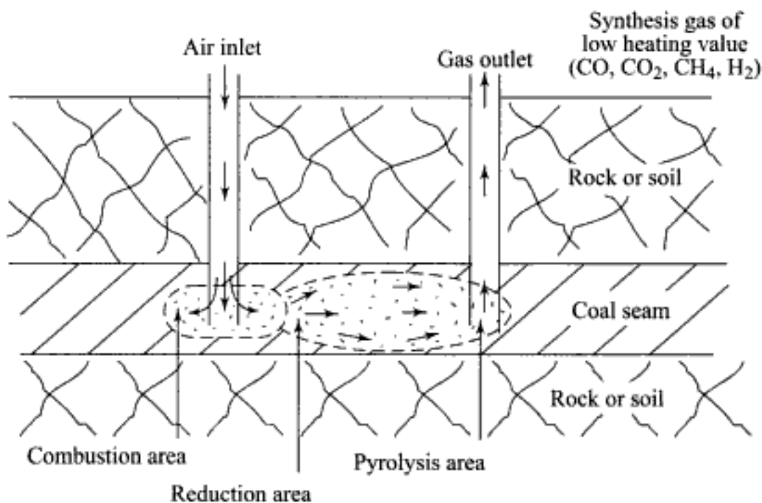
Fig. 4.4 In-situ coal gasification
