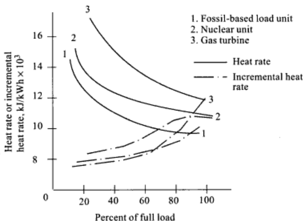
Fig. 1.10 Plant net heat rate and incremental heat rate
