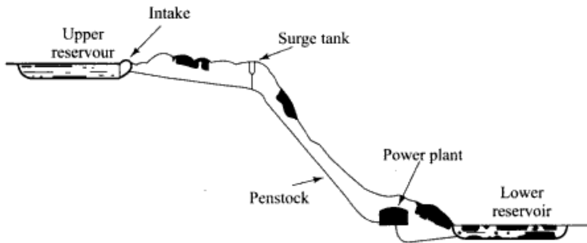
Fig. 12.4 Schematic of a conventional above ground pumped hydro storage system
