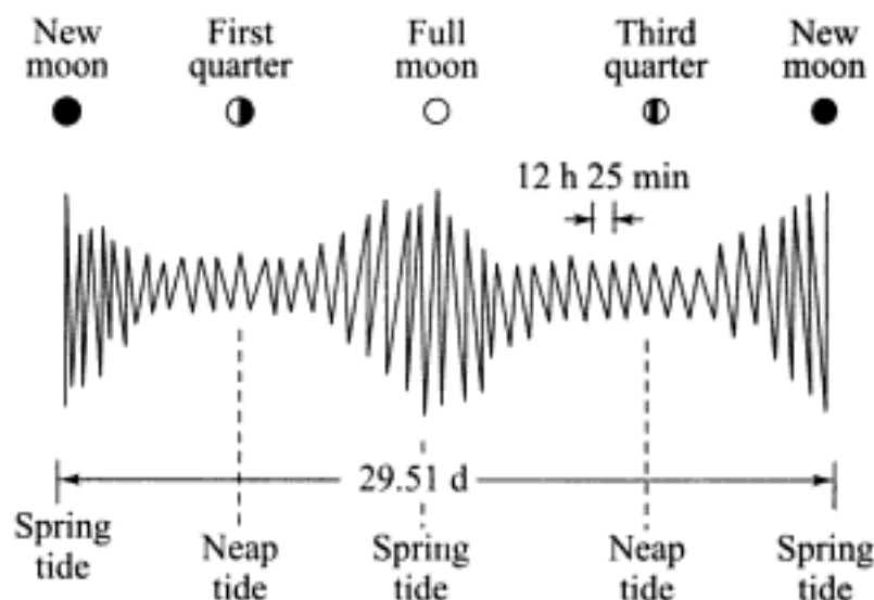
Fig. 14.25 Relative high and low tides showing variation in range during lunar month
