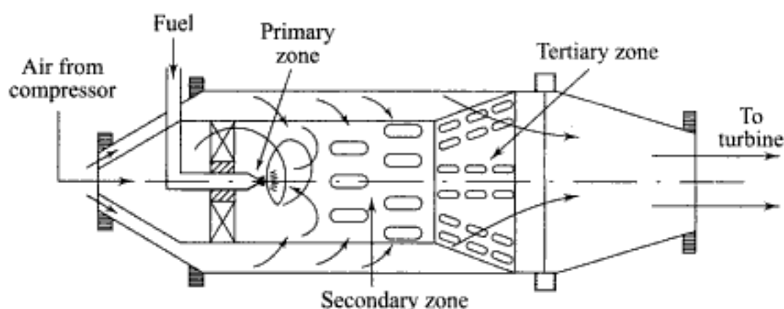
Fig. 11.60 Can-type combustor with swirl flow flame stabilizer
