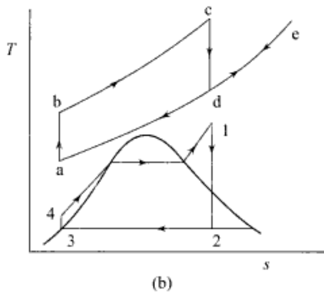
Fig. 3.10 Brayton/Rankine cyclic plants with supplementary heating
