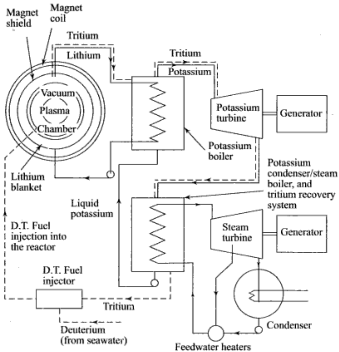
Fig. 9.28 Deuterium-tritium (D-T) fusion power plant conceptual design
