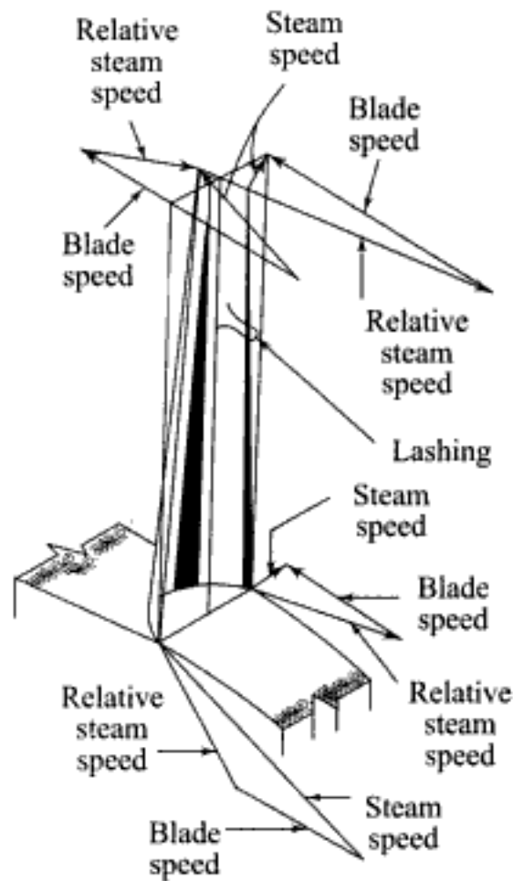
Fig. 7.41 A twisted blade with impulse flow at root and reaction at tip
