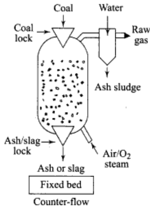
Fig. 5.56 Fixed bed counterflow gasifier
