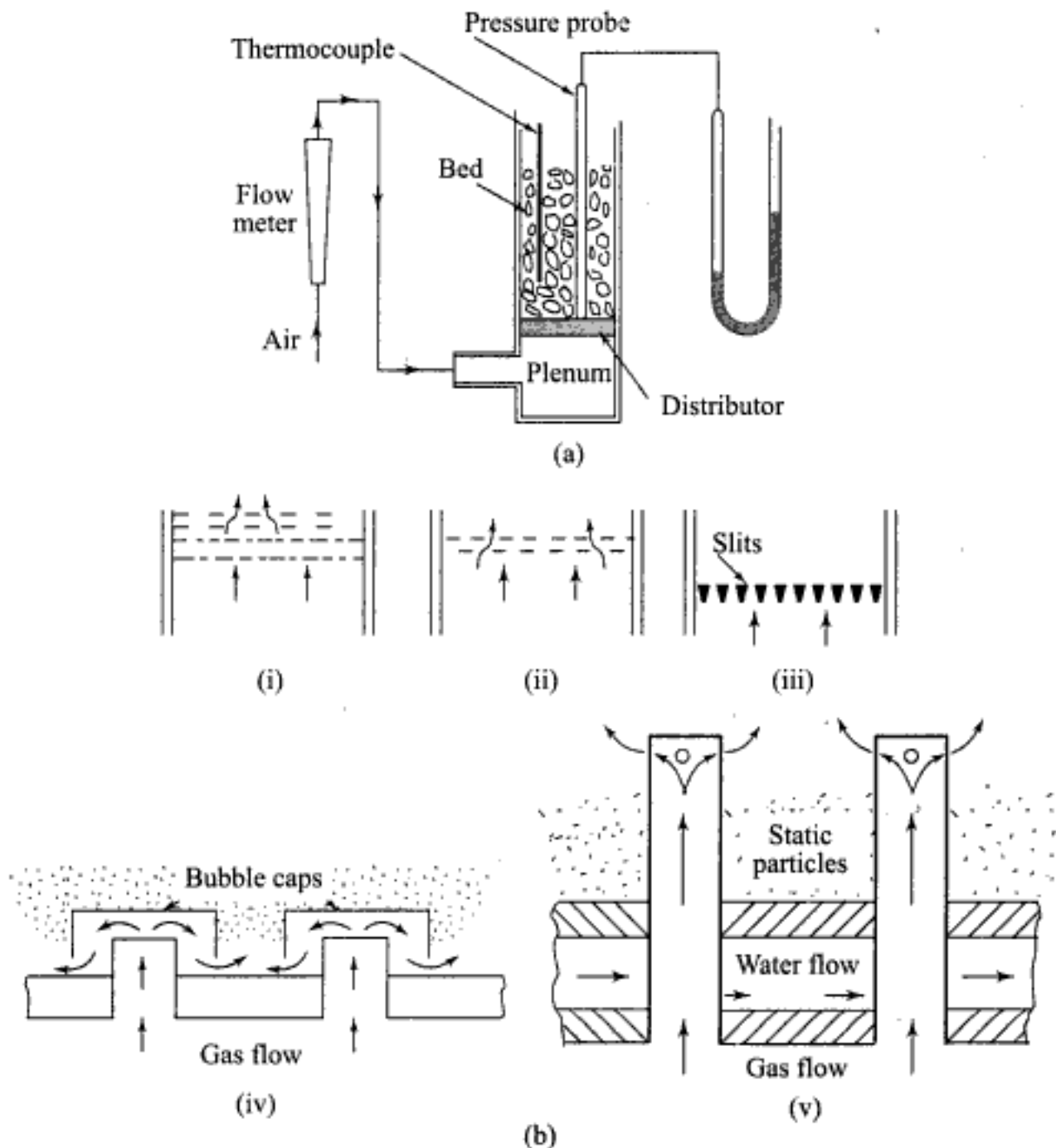
Fig. 5.36 (a) Measurement of U_{mf} and U_t of a fluidized bed (b) Few types of distributors; (i) sandwiching perforated plates, (ii) staggered perforated plates; (iii) grate bars, (iv) bubble cap type, (v) water-cooled type
