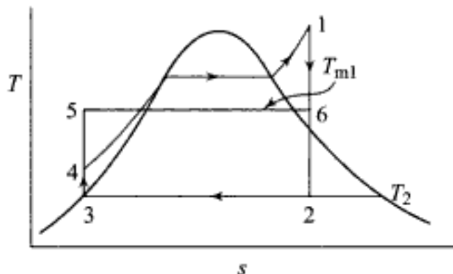
Fig. 2.9 Mean temperature of heat addition
