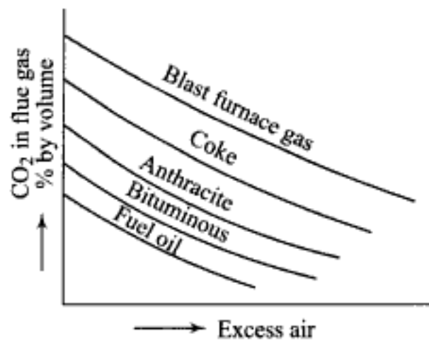
Fig. 4.9 \text{CO}_2 variation in flue gas with fuels and excess air
