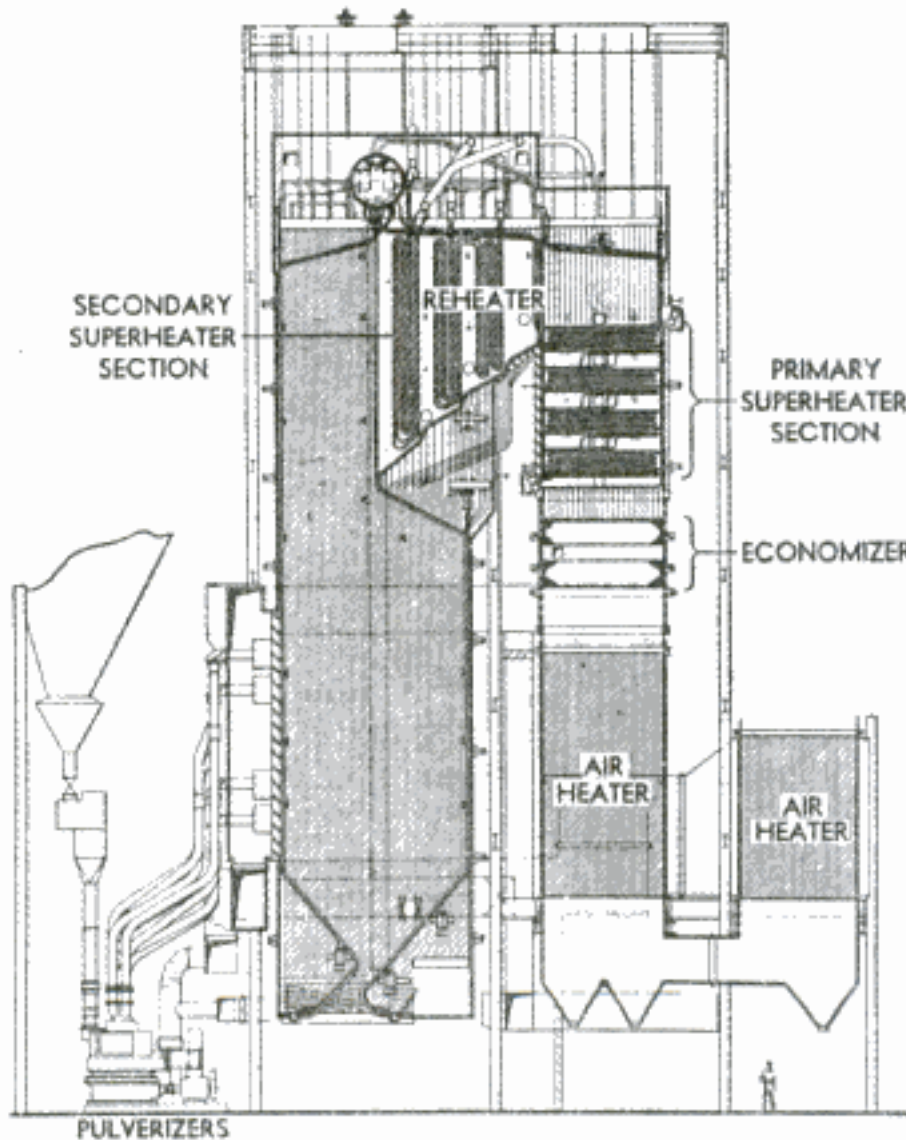
Fig. 6.19 Radiant boiler for pulverized coal
