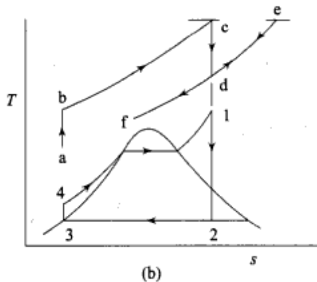
Fig. 3.11 GT-ST combined plant with supplementary combustion of fuel
