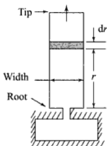
Fig. 7.58 Centrifugal and bending forces on the turbine blade
