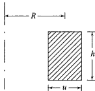
Fig. 12.17 Dimensions of a cylindrical coil with rectangular conductors
