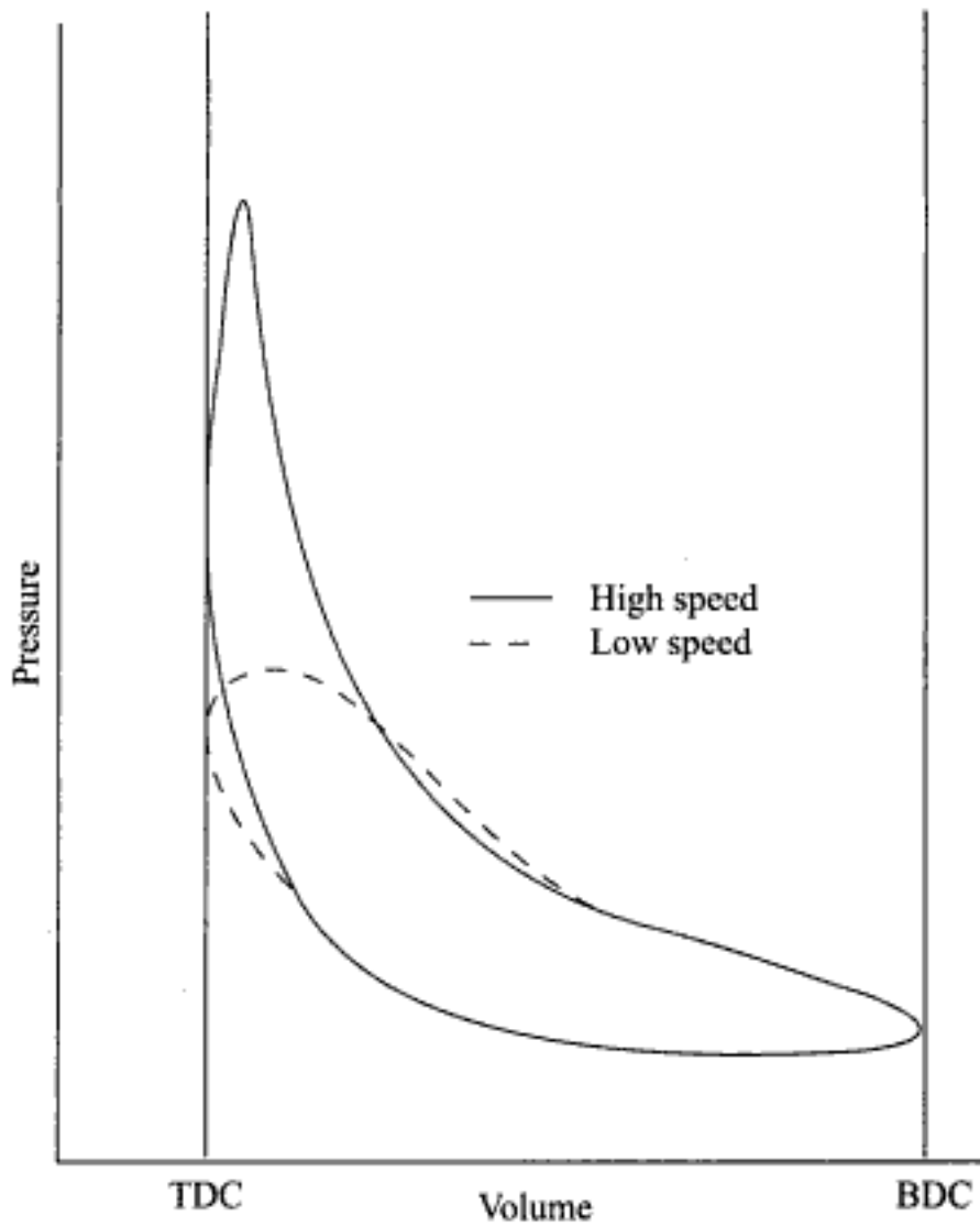
Fig. 11.21 Diagram illustrating the difference between a high speed and a low speed four-stroke cycle unsupercharged CI engine
