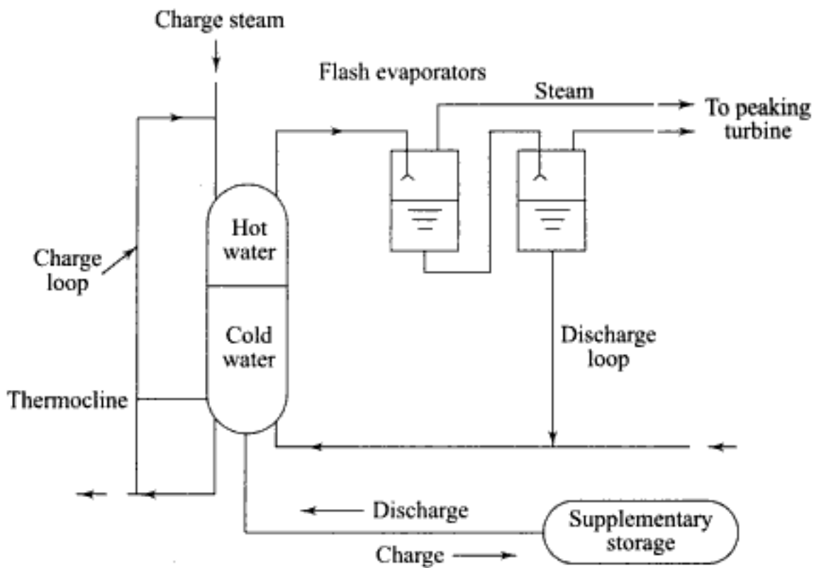
Fig. 12.23 Displacement accumulator with flash evaporators
