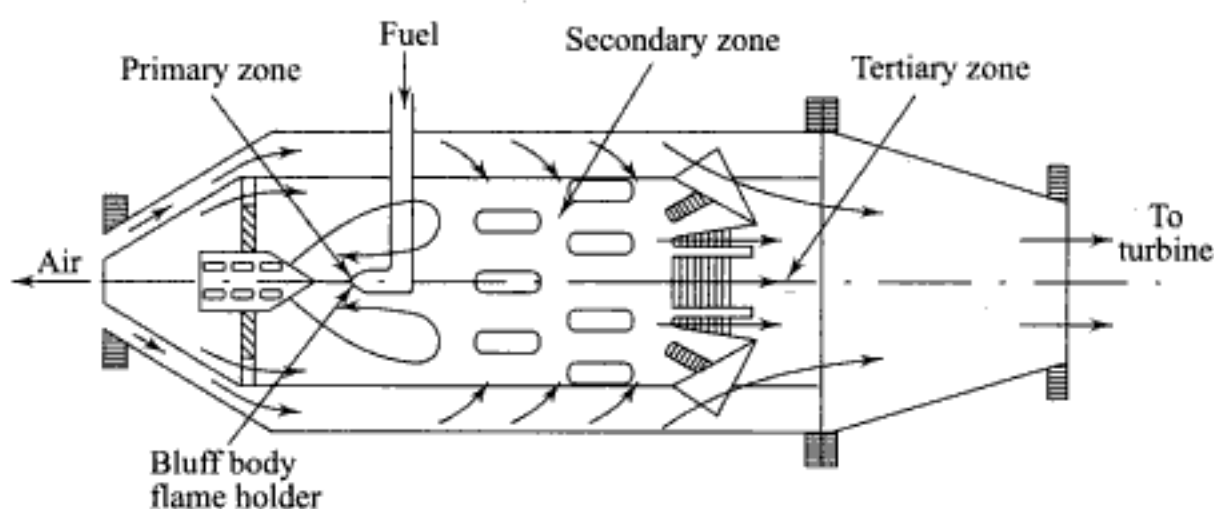
Fig. 11.61 Can-type combustor with bluff-body flame stabilizer
