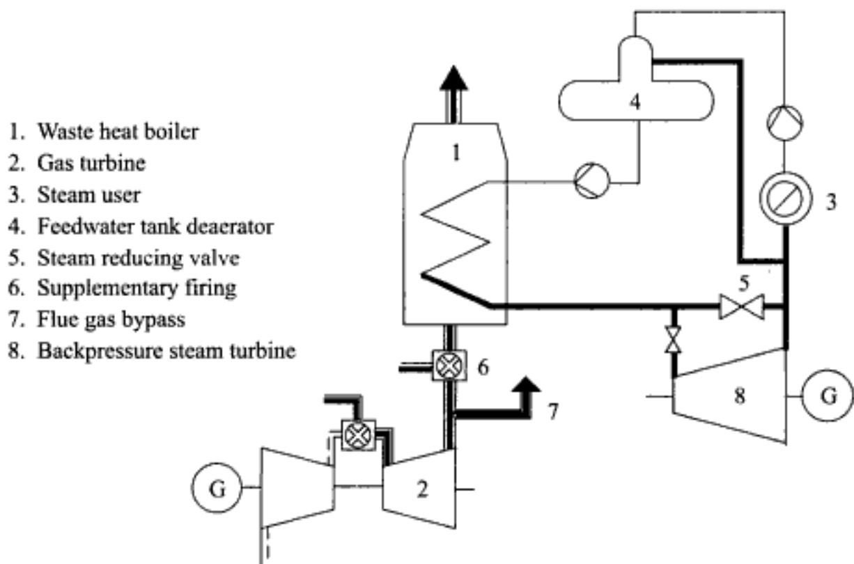
Fig. 3.29 Diagram of the principle of a combined-cycle plant used for cogeneration
