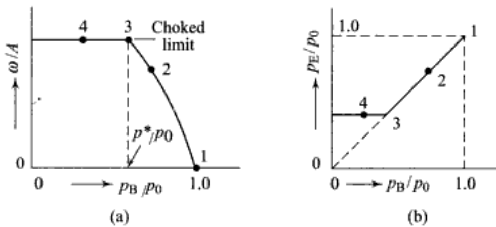
Fig. 7.12 Mass flow rate and exit pressure as a function of back pressure in a convergent nozzle
