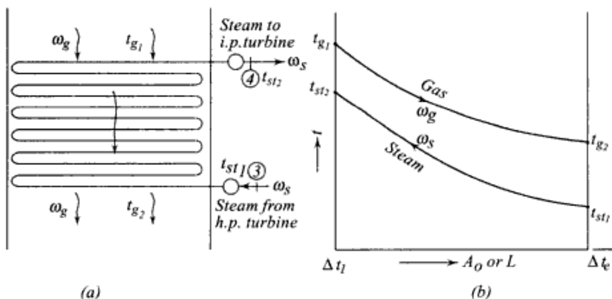
Fig. 6.33 Convective reheater
