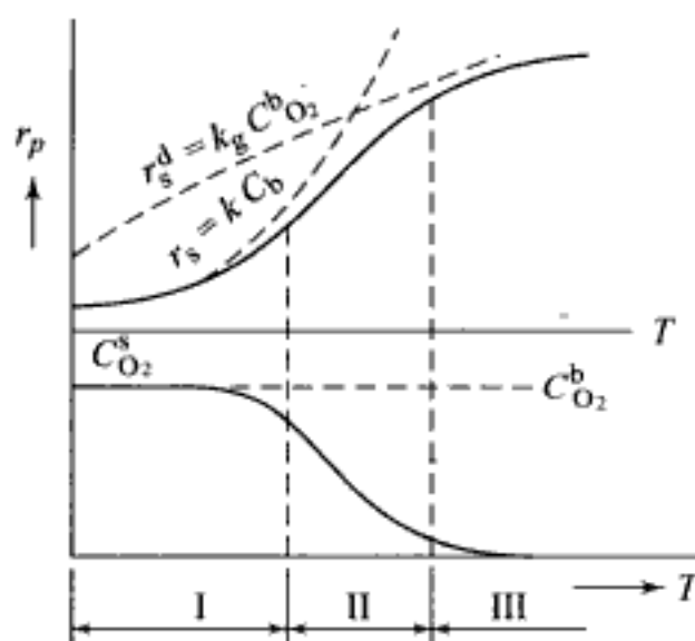
Fig. 5.6 Variation of oxygen concentration near the burning coke particle surface. I = kinetic region, II = transition zone, III = diffusion region of burning
