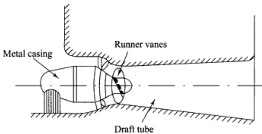
Fig. 10.34 Bulb turbine
