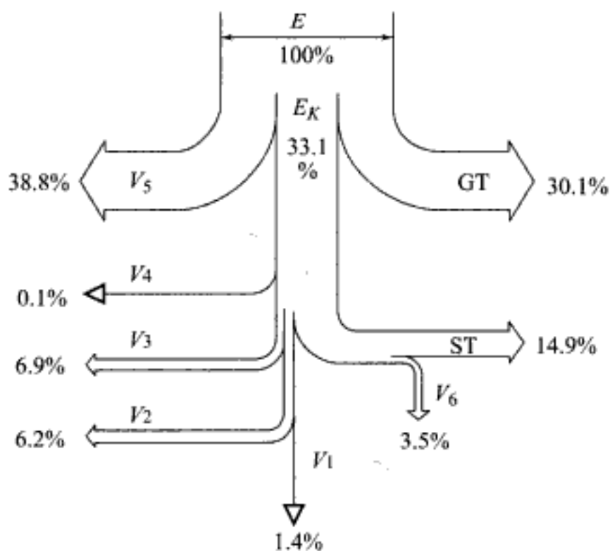
Fig. 3.20 Exergy flow diagram of a typical combined cycle power plant
