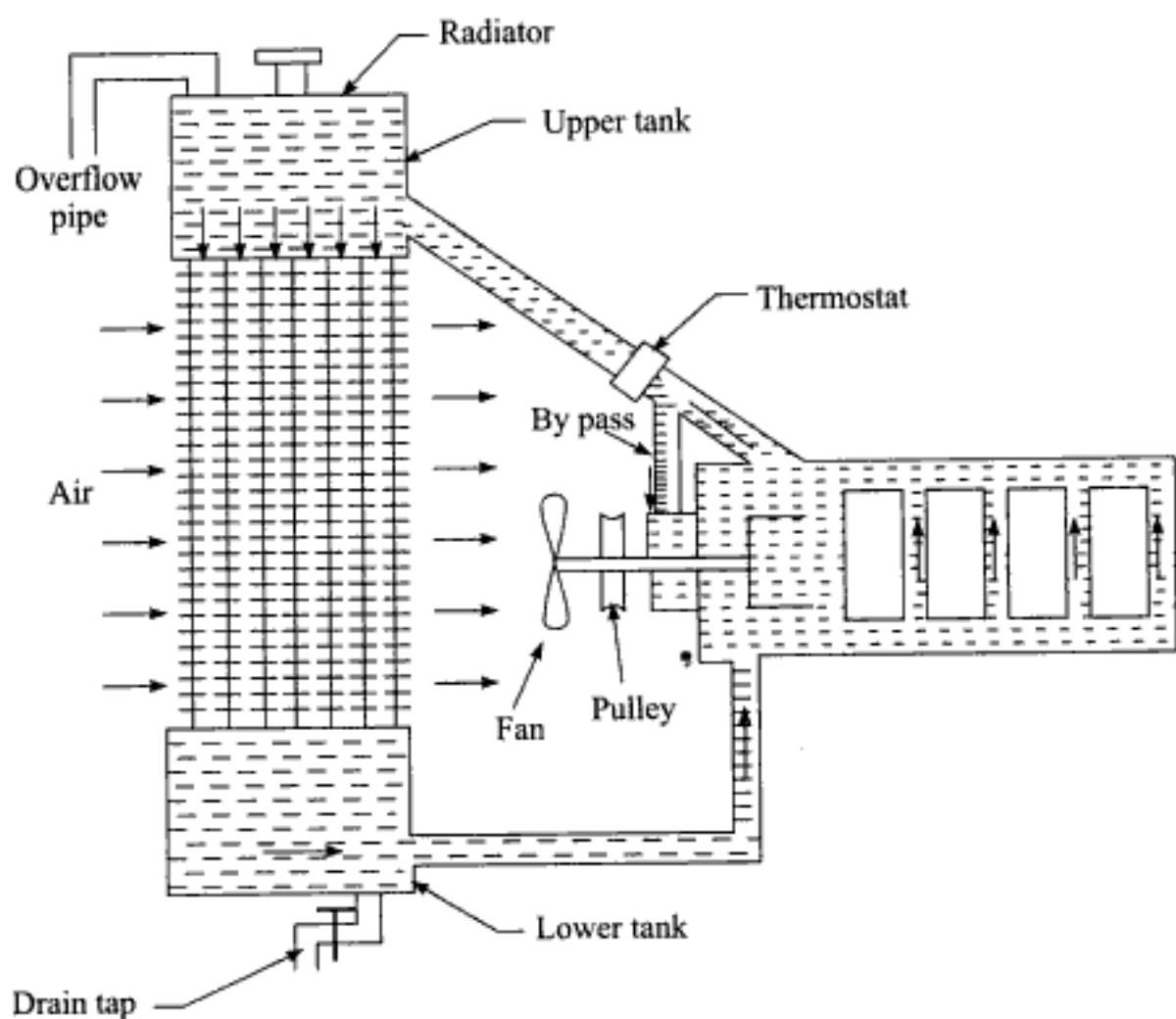
Fig. 11.12 Thermostat cooling
