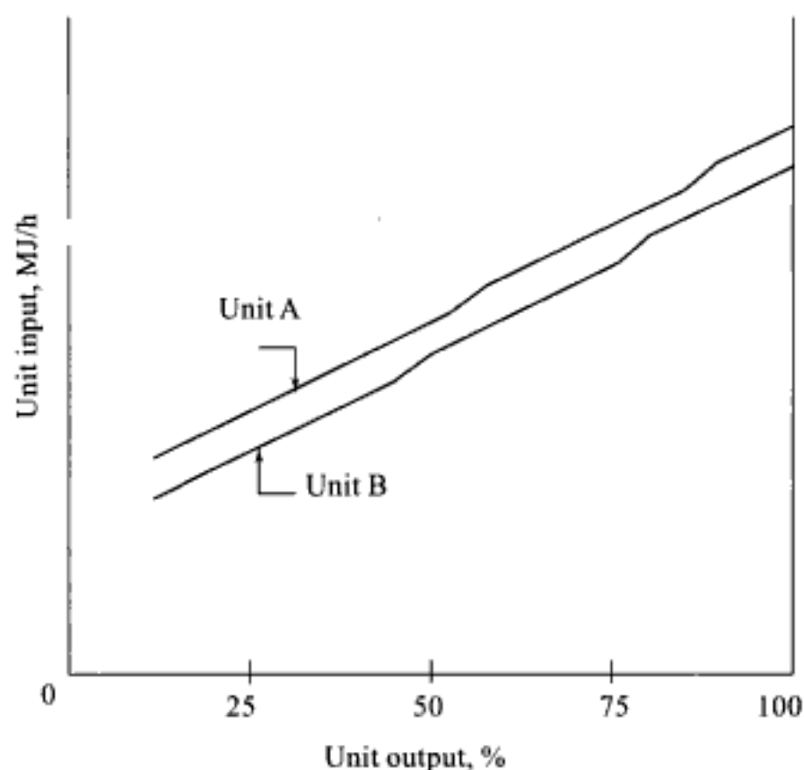
Fig. 1.11 Input-output curves
