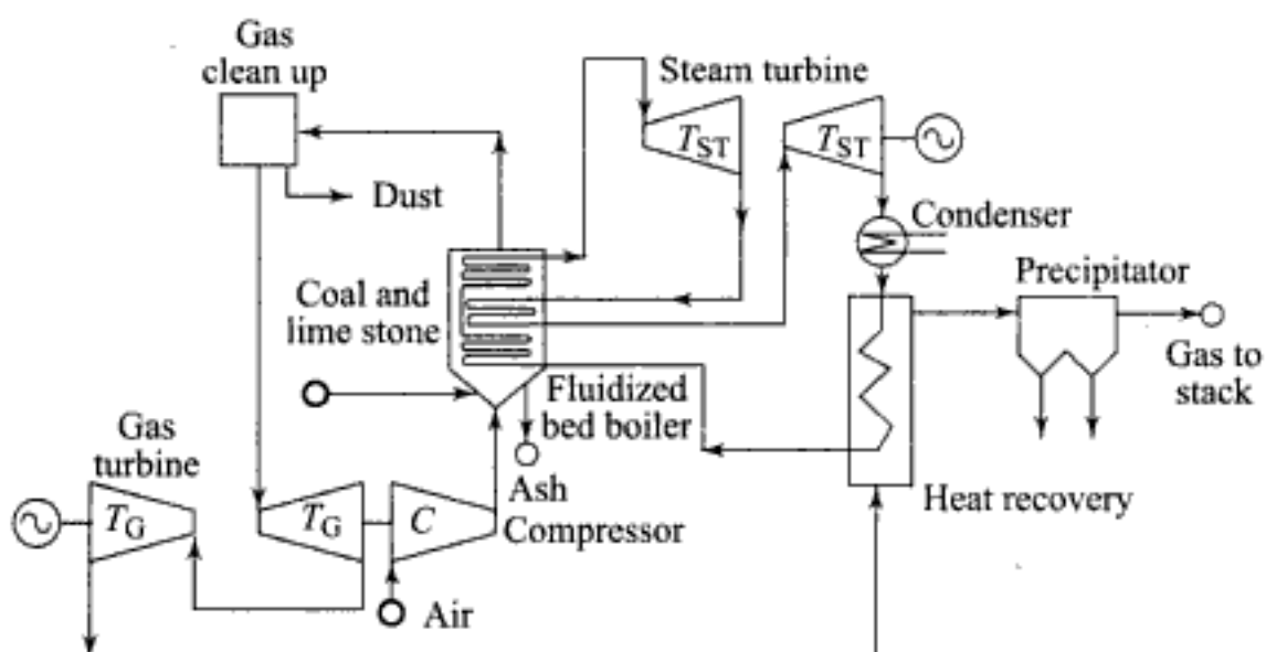
Fig. 3.22 A PFBC combined cycle
