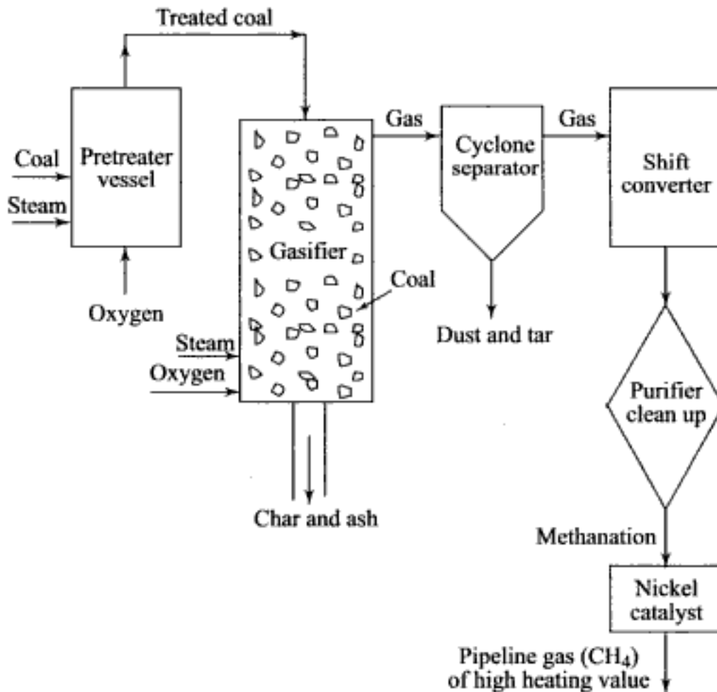
Fig. 4.3 Synthane coal gasification process
