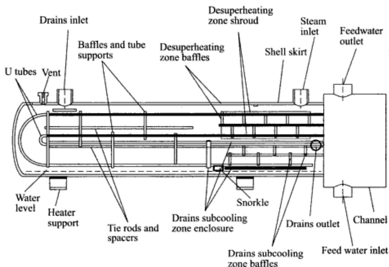
Fig. 8.13(a) A three-zone horizontal closed-type feedwater heater
