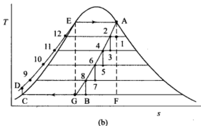
Fig. 2.23 Regenerative feed cycle with four extractions
