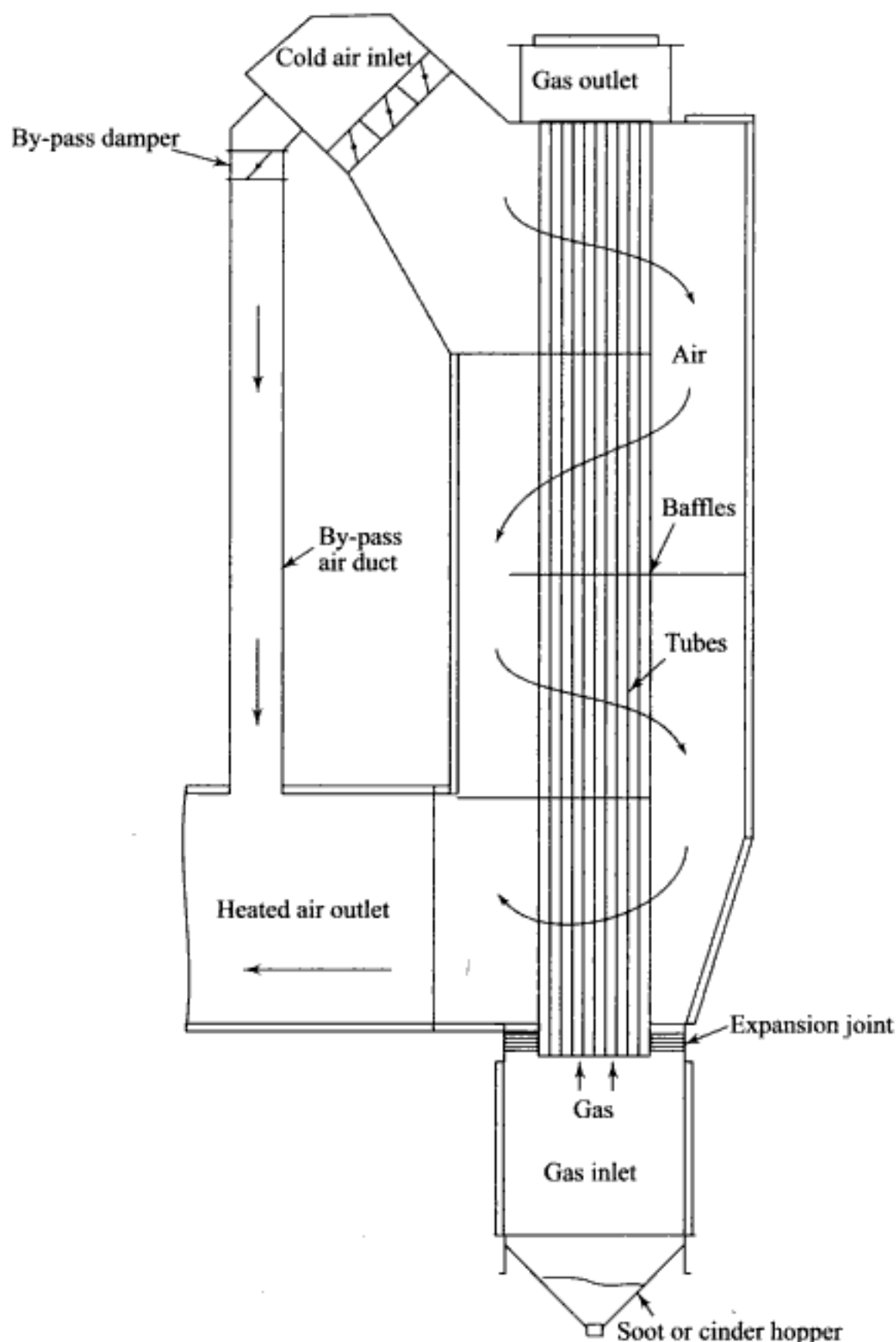
Fig. 6.45 (b) Air heater arrangement
