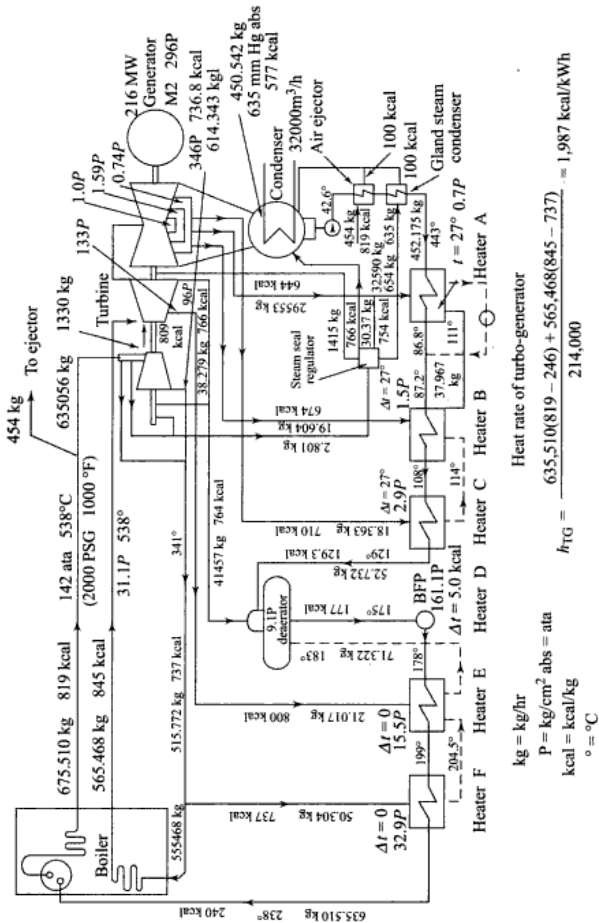
Fig. 2.31 (b) Heat balance diagram of a 214 MW reheat unit (1 kcal = 4.187 kJ)
