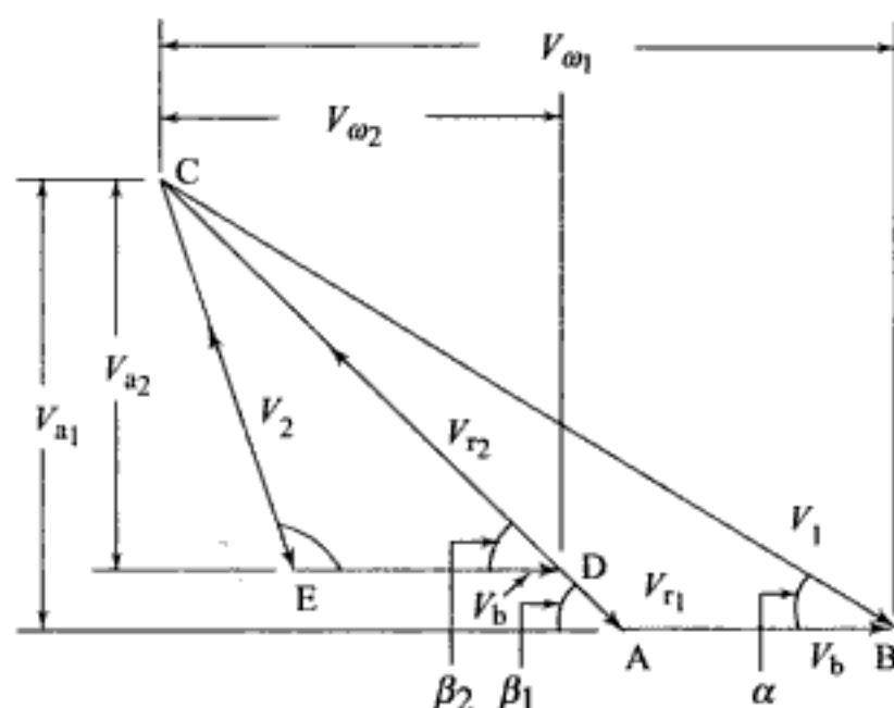
Fig. 7.20 Velocity diagram with symmetrical impulse blading
