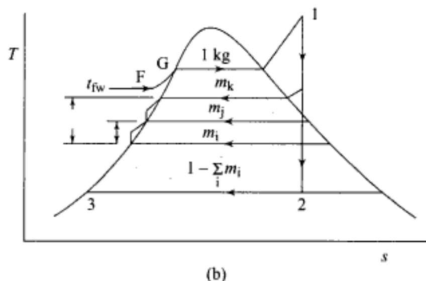
Fig. 2.25 Heater train of a steam power plant \left(\gamma = \frac{\alpha}{2}\right)
