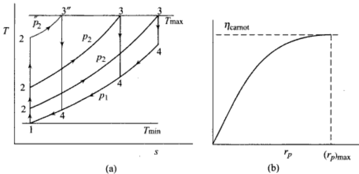
Fig. 3.16 Effect of pressure ratio on specific output and efficiency of Brayton cycle
