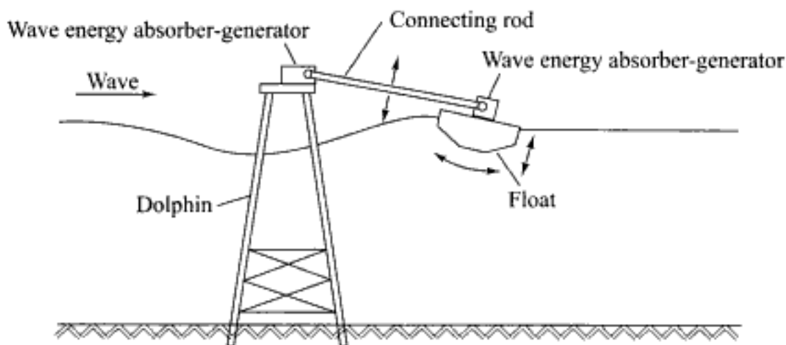
Fig. 14.20 Schematic of a Dolphin type wave generator
