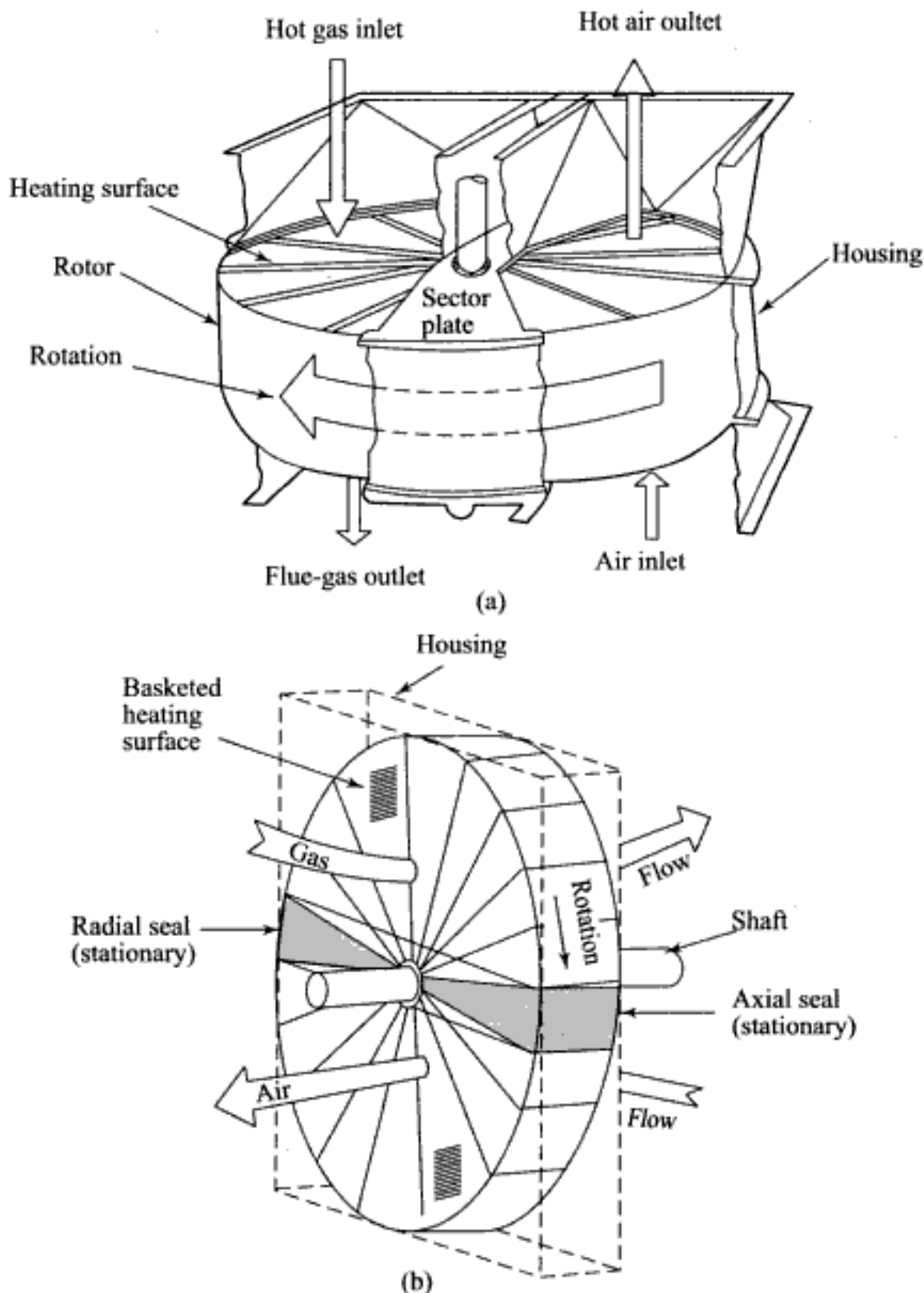
Fig. 6.47 (a) Details of a regenerative air preheater (Ljungstrom APH) (b) Another view of a regenerative air preheater
