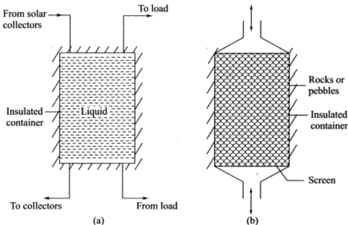
Fig. 14.6 Schematic of two forms of sensible heat storage: (a) liquid, (b) porous solid
