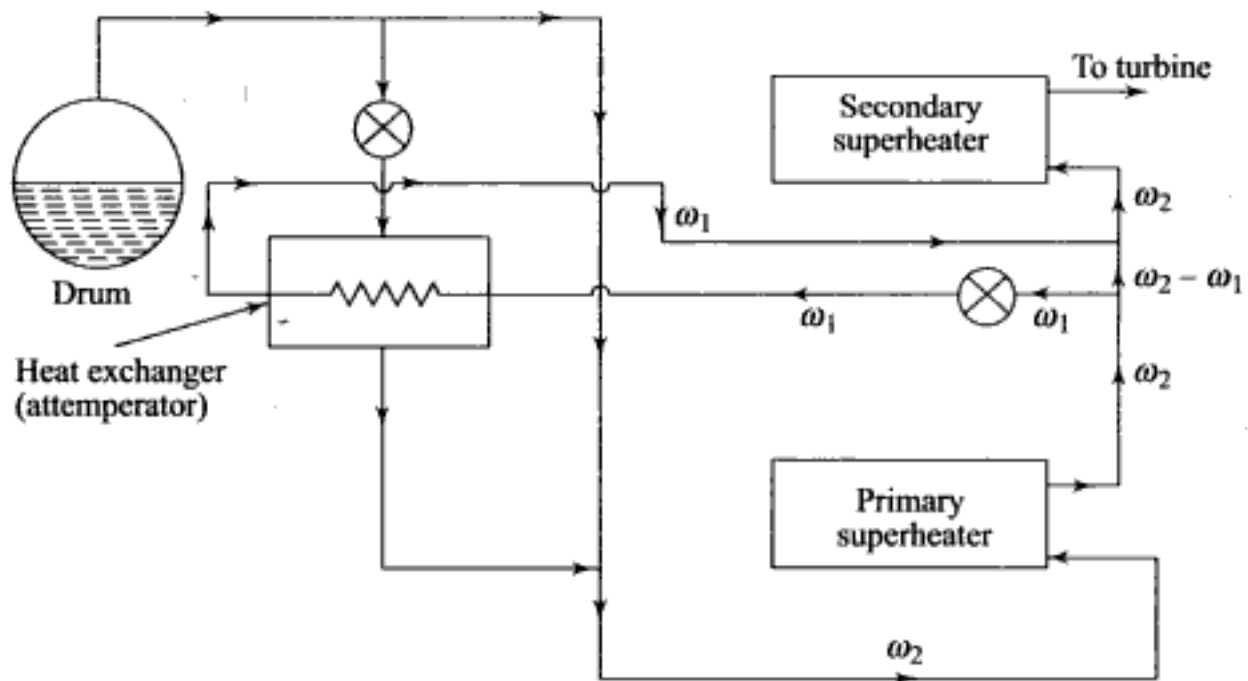
Fig. 6.36 Control of steam temperature by attemperation
