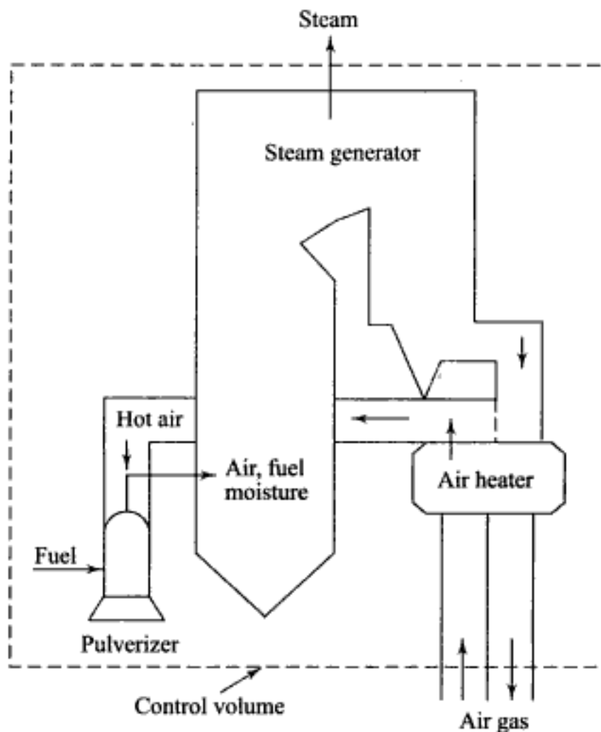
Fig. 4.5 Thermodynamic control volume drawn around equipment
