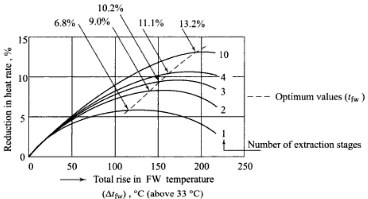
Fig. 2.28 Reduction of heat rate by regenerative feedwater heating
