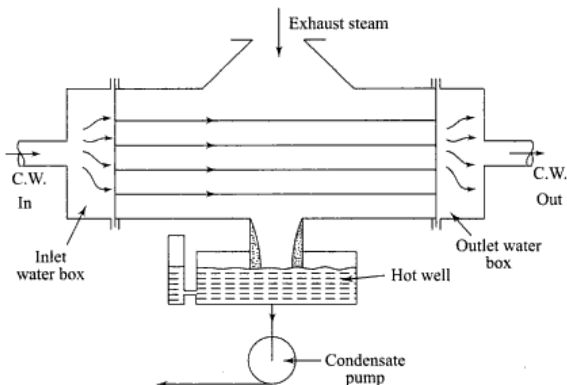
Fig. 8.5 Single-pass condenser with divided water boxes
