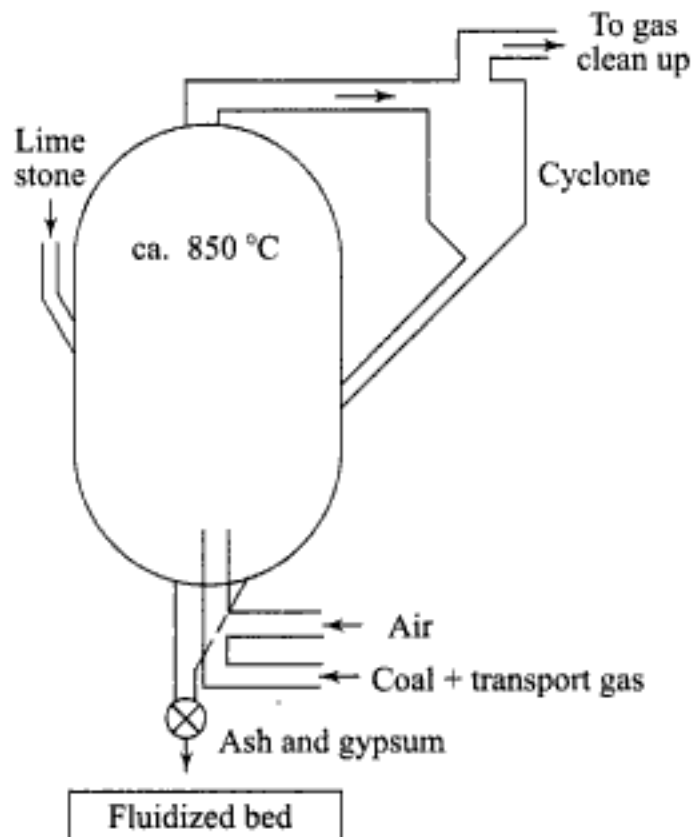
Fig. 5.58 Fluidized bed gasifier
