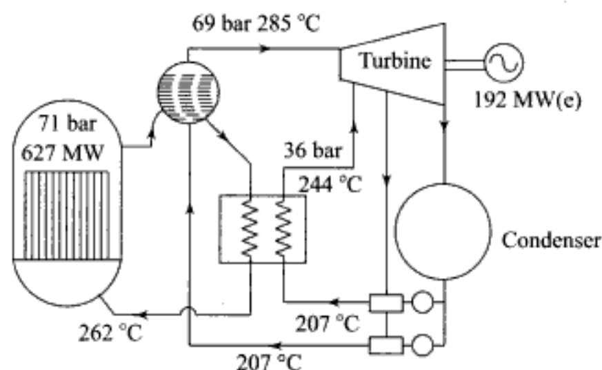
Fig. 9.21 Dresden (USA) dual-pressure direct-cycle BWR system
