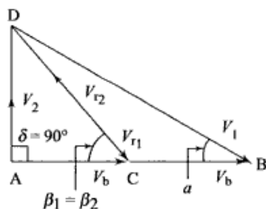
Fig. 7.21 Velocity diagram for frictionless symmetrical impulse blading with axial discharge.
