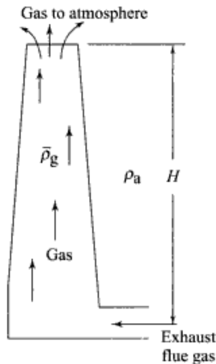
Fig. 4.14 Draught produced by a chimney
