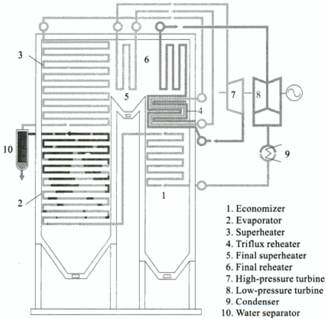
Fig. 6.24 Simplified diagram of a sulzer monotube steam generator with triflux reheater
