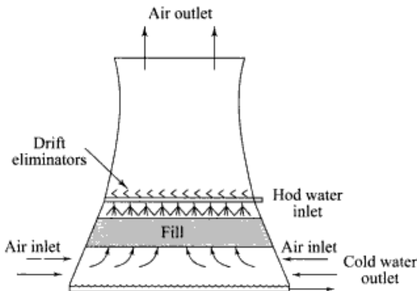
Fig. 8.20(b) Counterflow hyperbolic natural draught cooling tower
