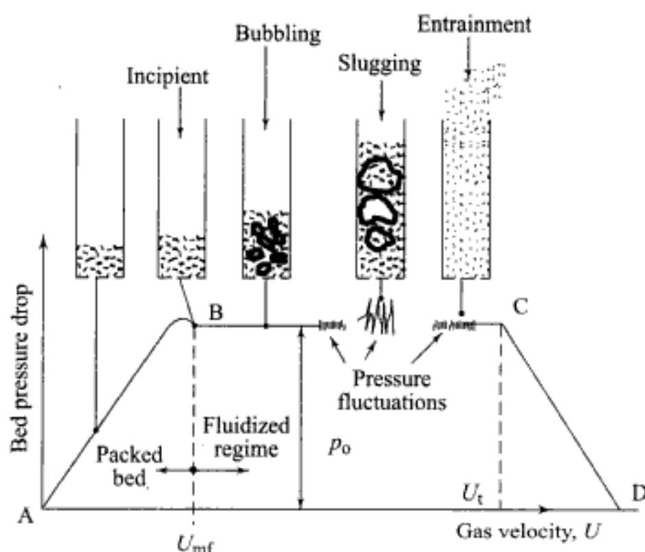
Fig. 5.37 (a) Variation of bed pressure drop with superficial velocity
