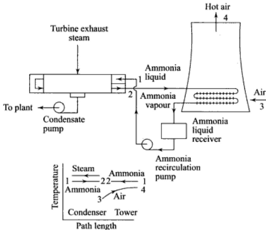
Fig. 8.25 Schematic of an indirect dry-cooling tower with a surface condenser having ammonia as the coolant
