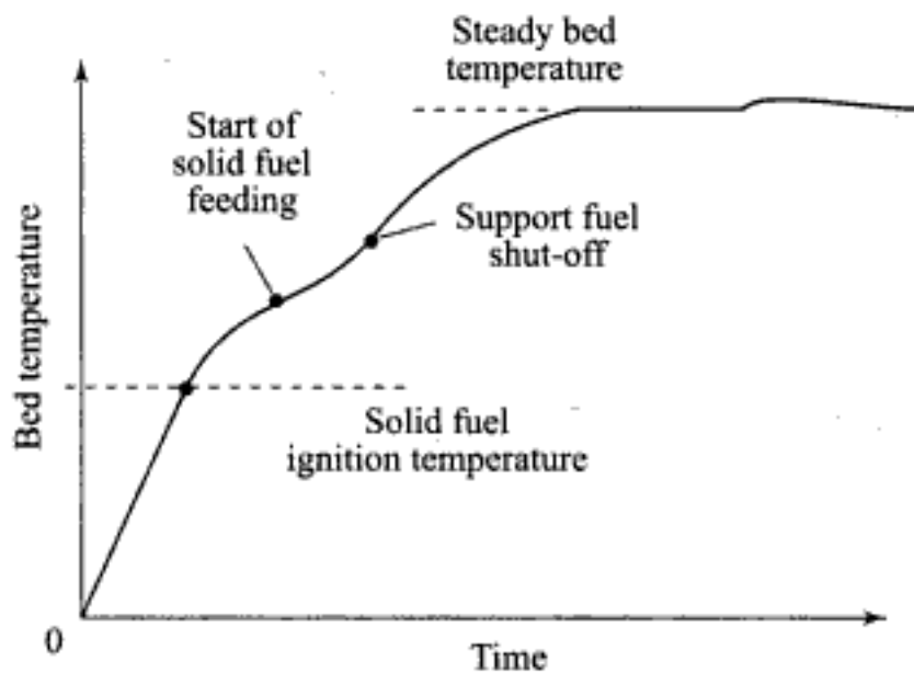
Fig. 5.44 Start-up transient of a fluidized bed combustor
