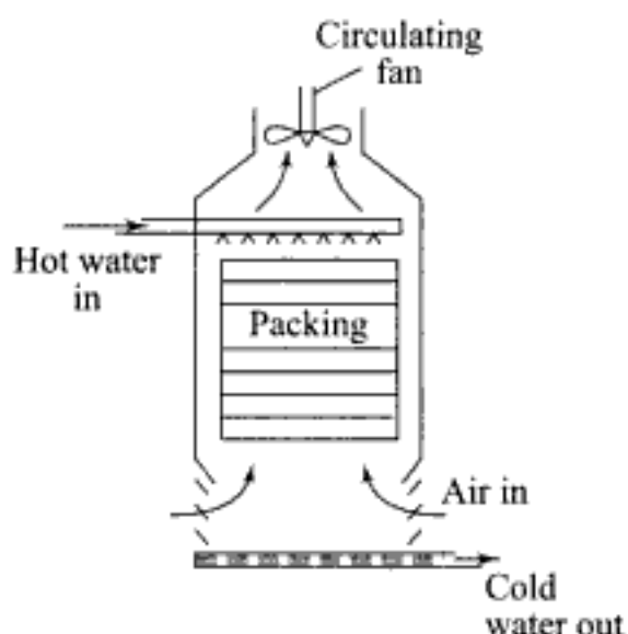
Fig. 8.18 Packing or fill in a wet cooling tower
