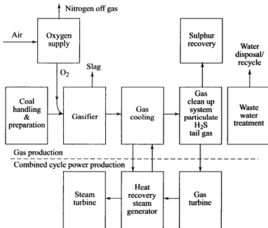
Fig. 5.59 Basic IGCC plant arrangement
