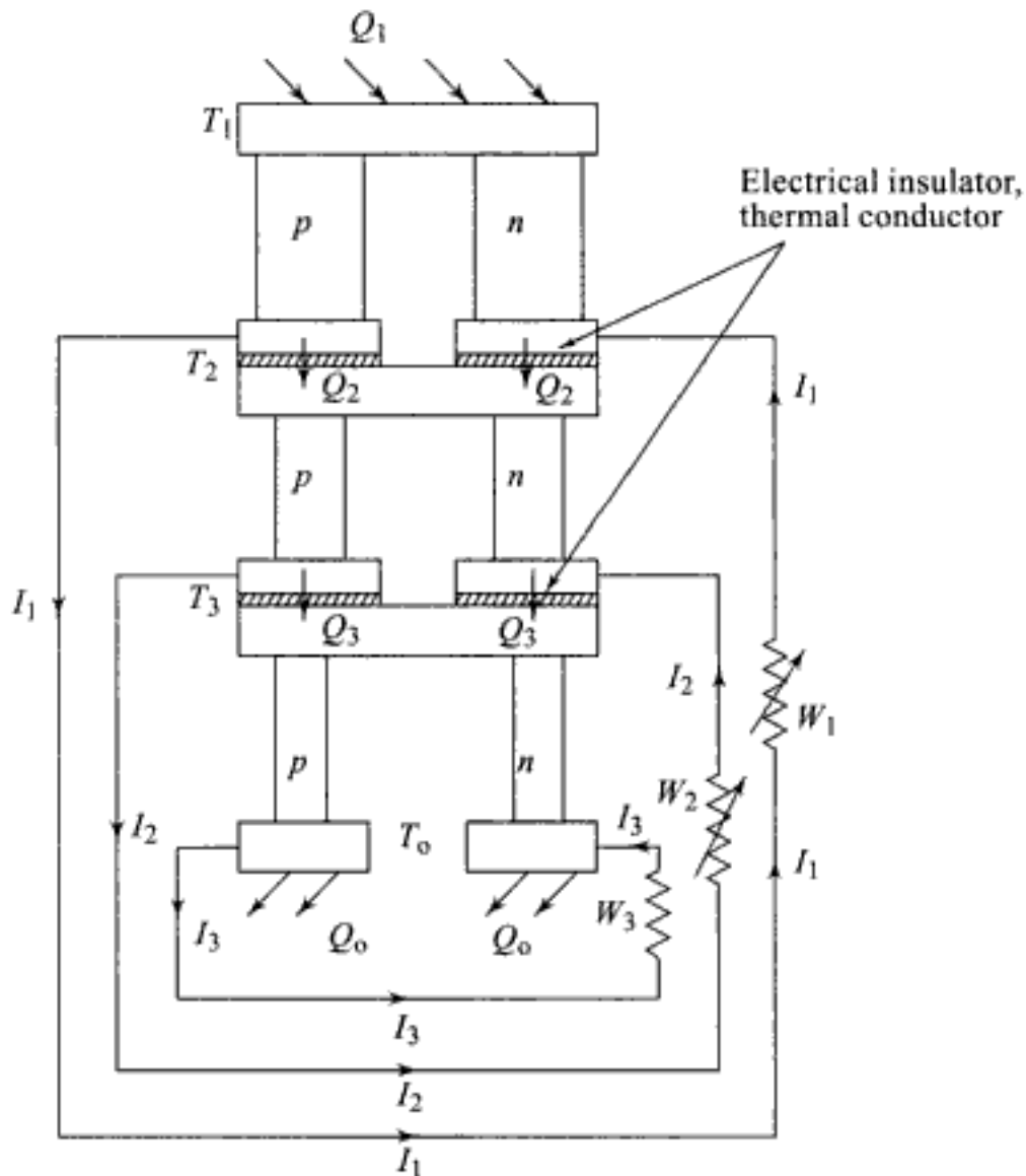
Fig. 13.15 A simple 3-stage cascade thermoelectric generator
