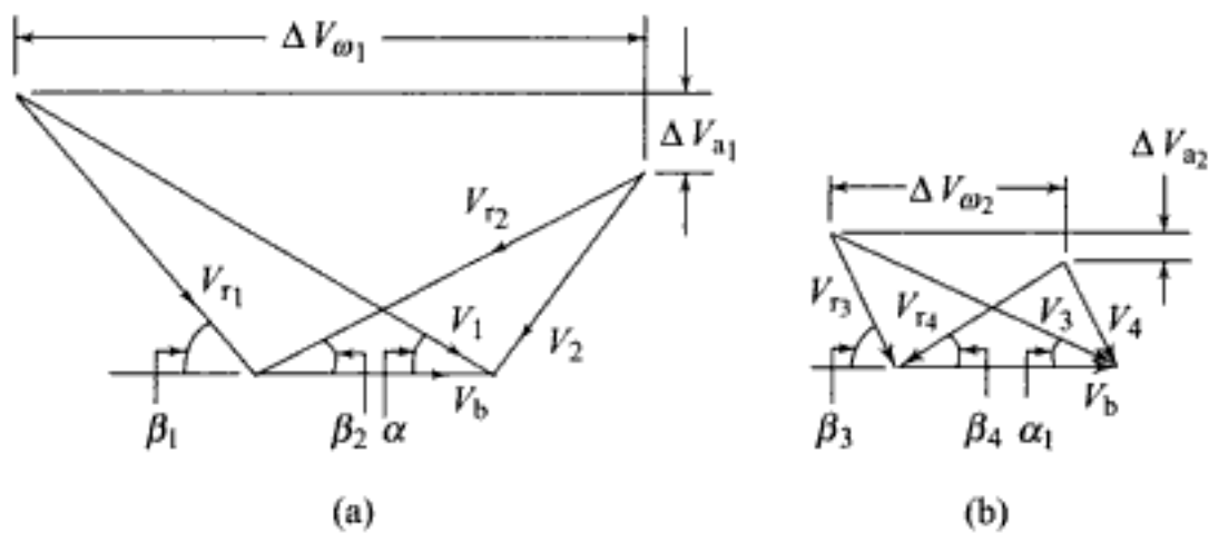
Fig. 7.26 Velocity diagrams for a 2-row Curtis stage: (a) first row of moving blades, (b) second row of moving blades
