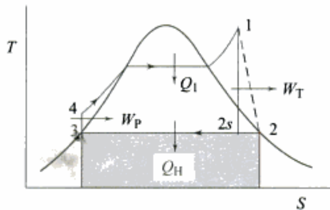
Fig. 2.34 By-product power cycle with a back pressure turbine
