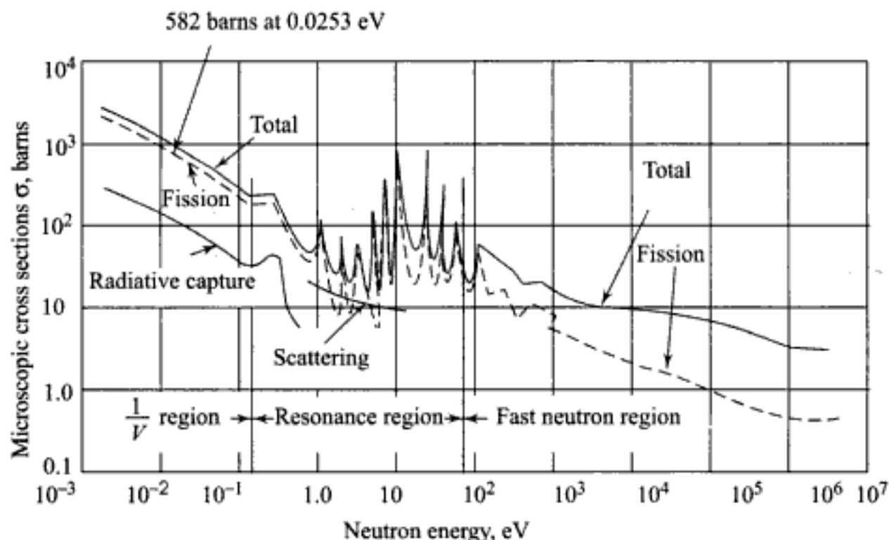
Fig. 9.8 Neutron cross-section for U-235
