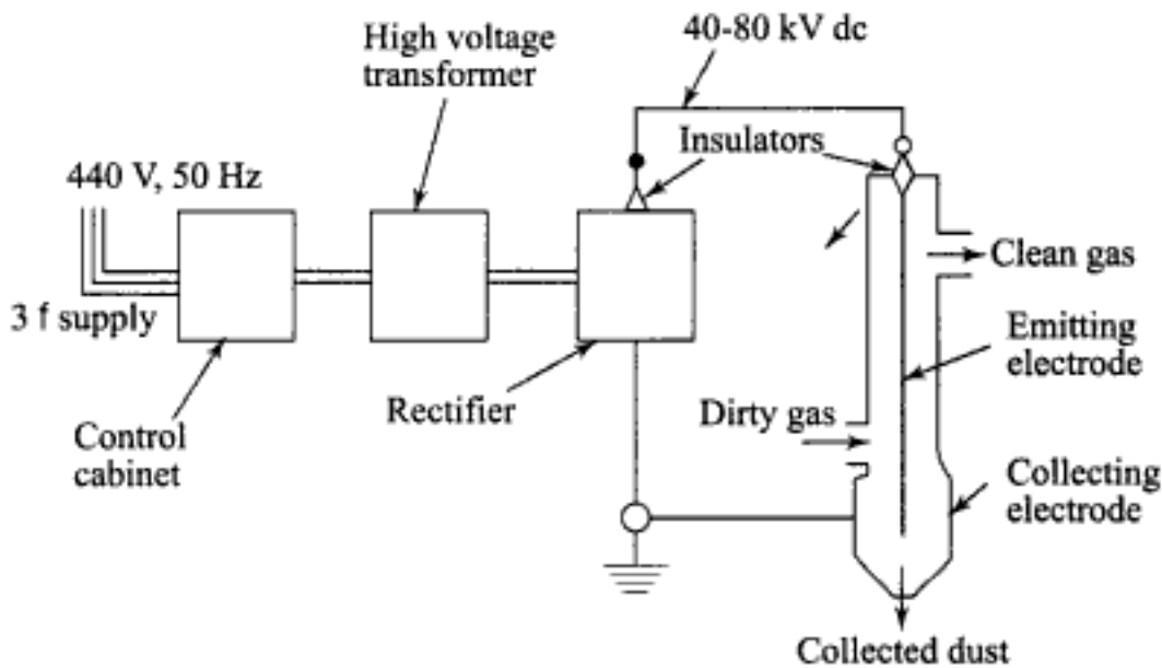
Fig. 6.60 Basic elements of an electrostatic precipitator
