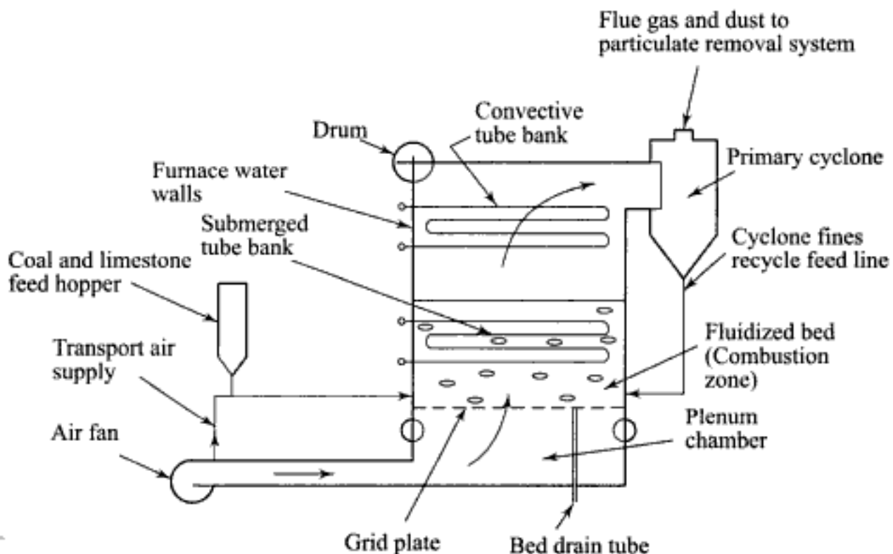
Fig. 6.48 Schematic of bubbling fluidized bed boiler
