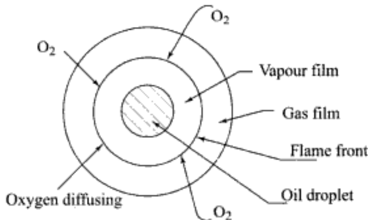
Fig. 5.61 Combustion of an oil droplet
