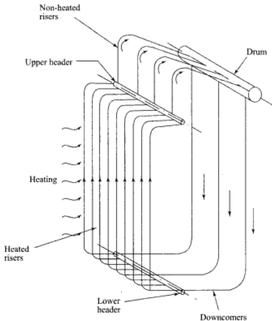
Fig. 6.13 Circulation circuit in a natural circulation boiler
