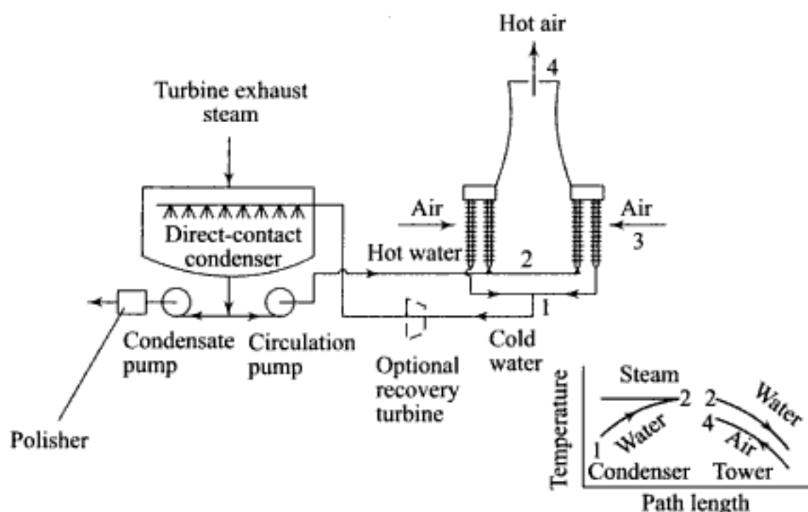
Fig. 8.24 Schematic of an indirect dry-cooling tower with an open-type condenser
