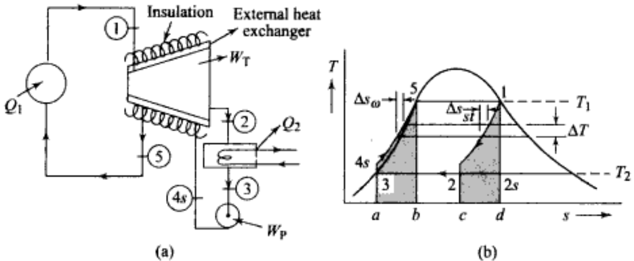
Fig. 2.18 Ideal regenerative cycle
