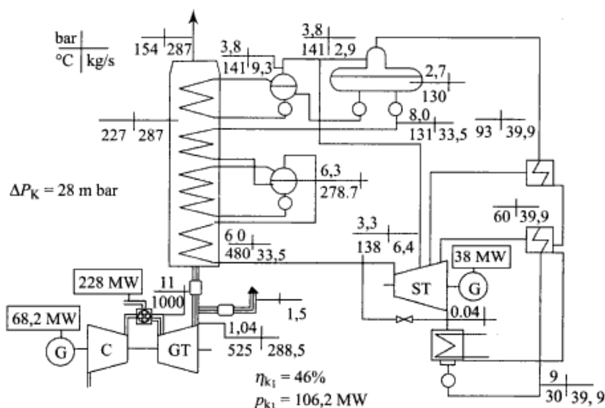
Fig. 3.21 A simplified flow diagram for a combined cycle plant with two-pressure steam cycle
