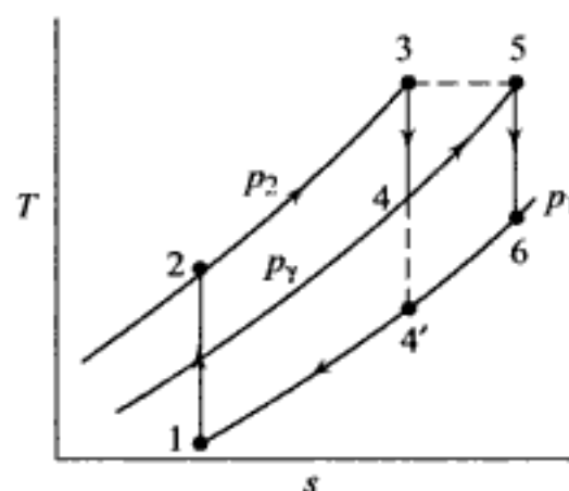
Fig. 11.45 Effect of reheat on brayton cycle
