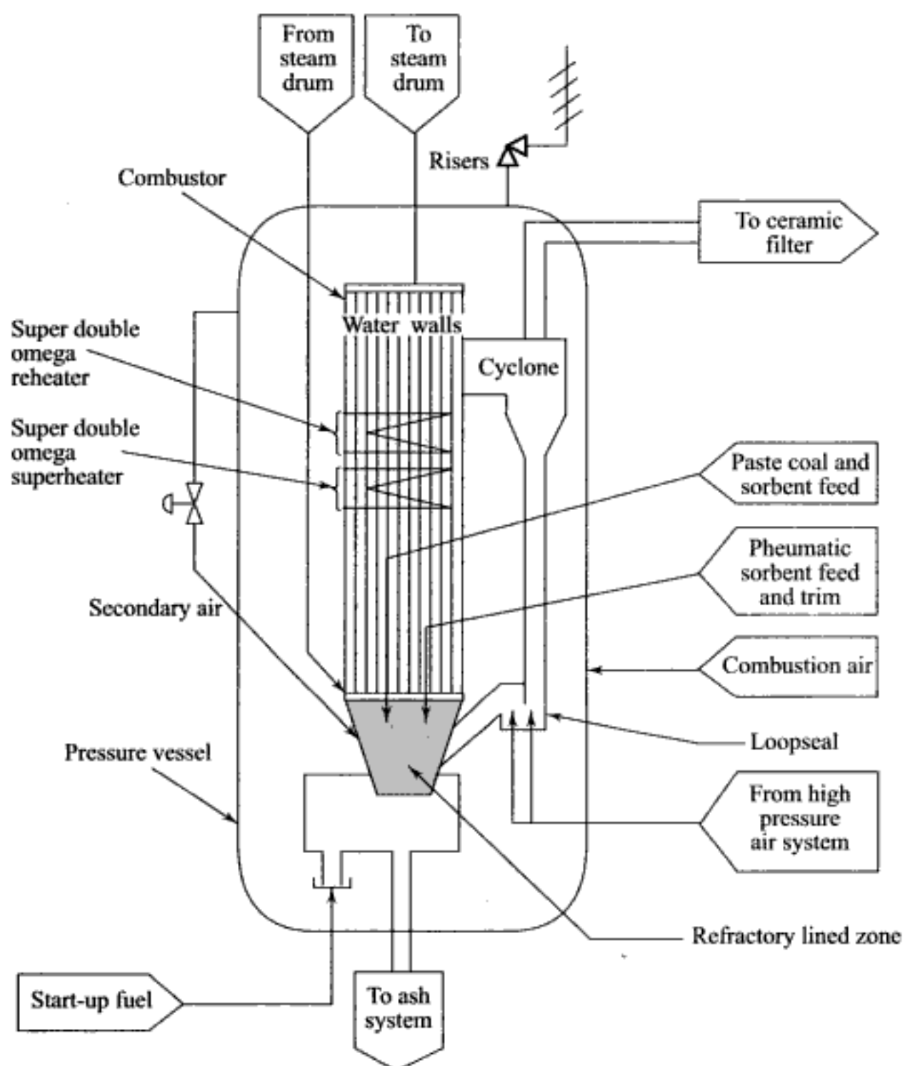
Fig. 5.54 Schematic PFBC hot loop
