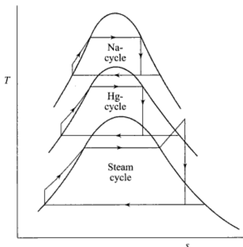
Fig. 3.4 Sodium-mercury-steam tertiary cycle
