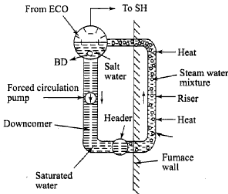
Fig. 6.10 Forced circulation system
