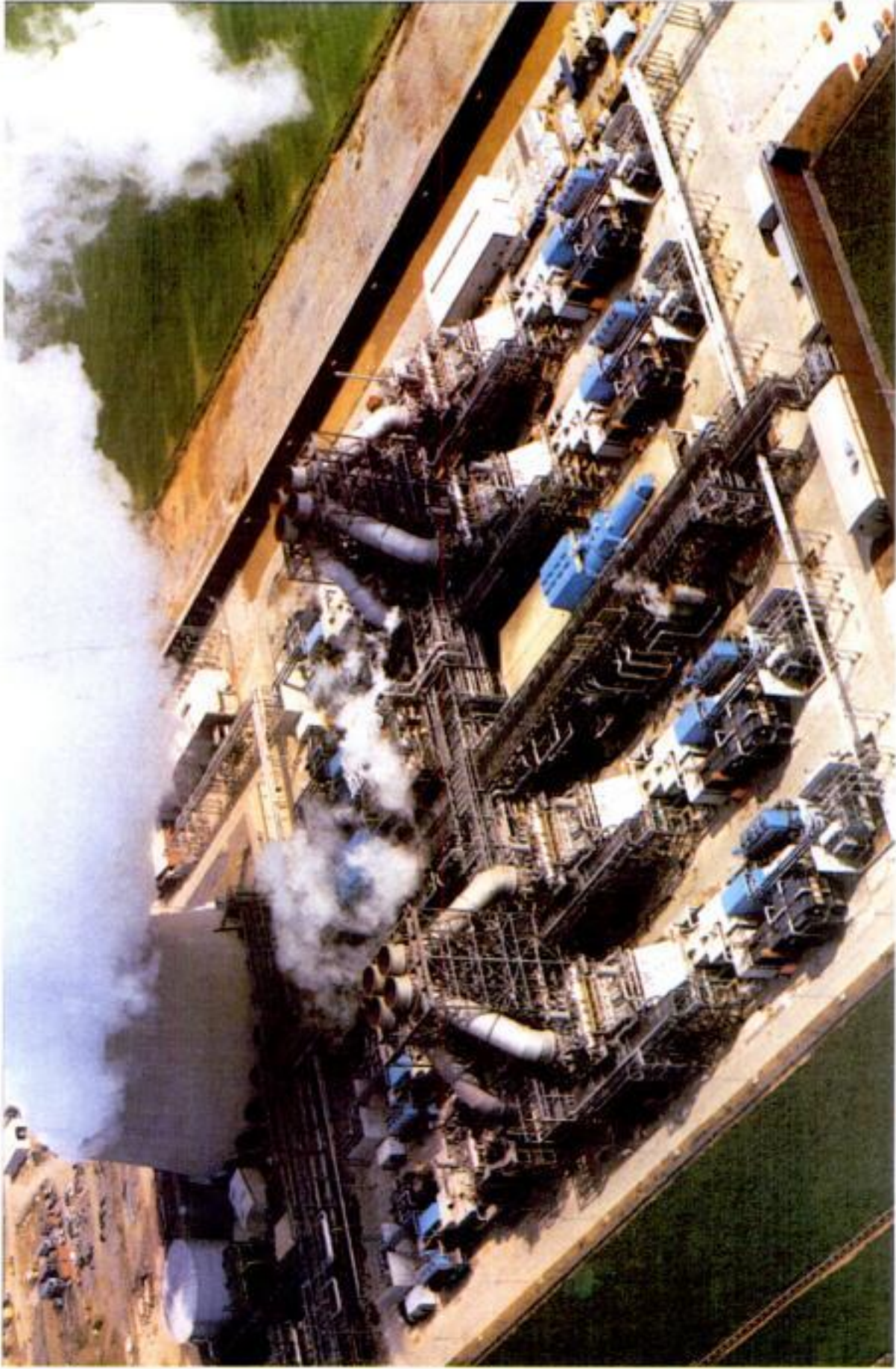
Fig. 3.14.2 (a) Combined cycle power plant at Teesside, England (1875 MW)
