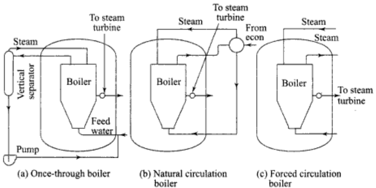
Fig. 6.59 Different steam–water circulation systems in PFBC boilers
