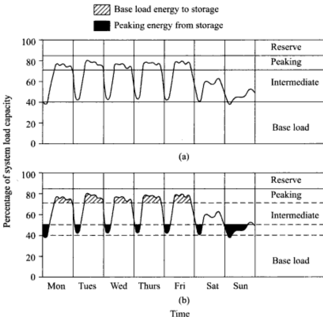
Fig. 12.1 Weekly load curve for a typical power utility (a) Current generation mix (b) Generation mix with energy storage
