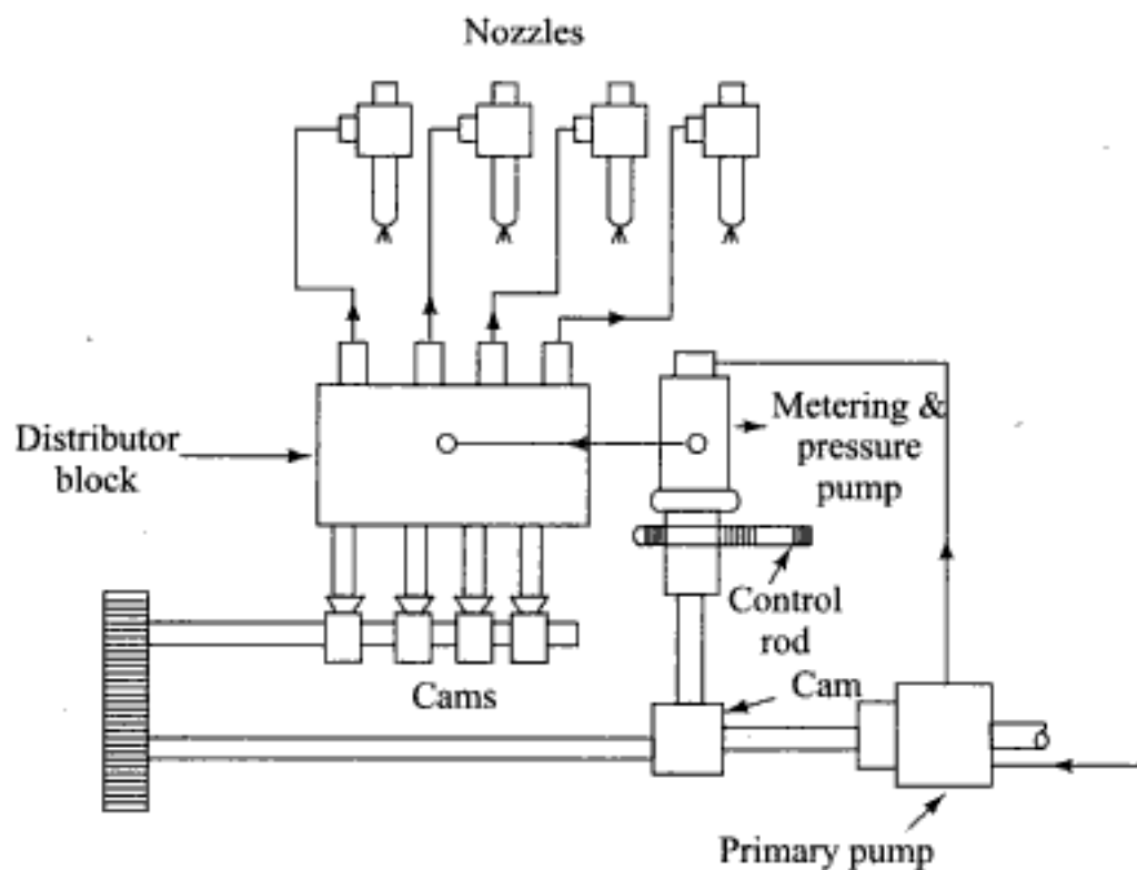
Fig. 11.7 Distributor fuel injection system
