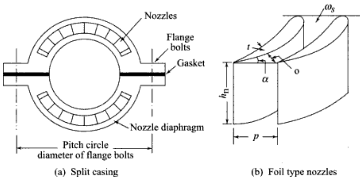
Fig. 7.10 Horizontally split diaphragm with nozzles
