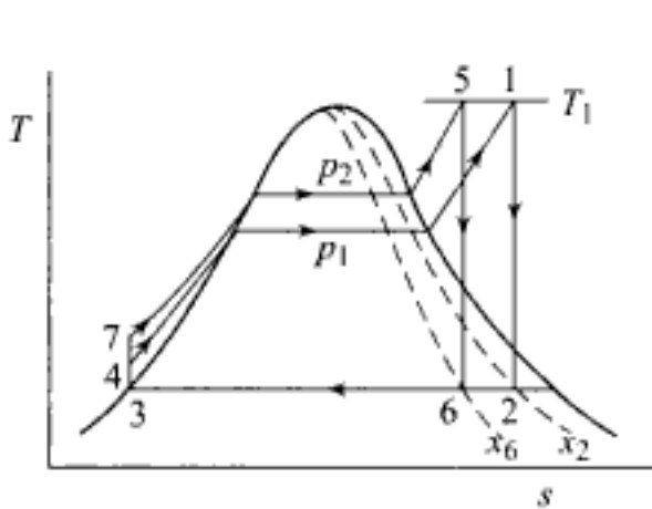
Fig 2.12 Effect of increase of pressure on Rankine cycle
