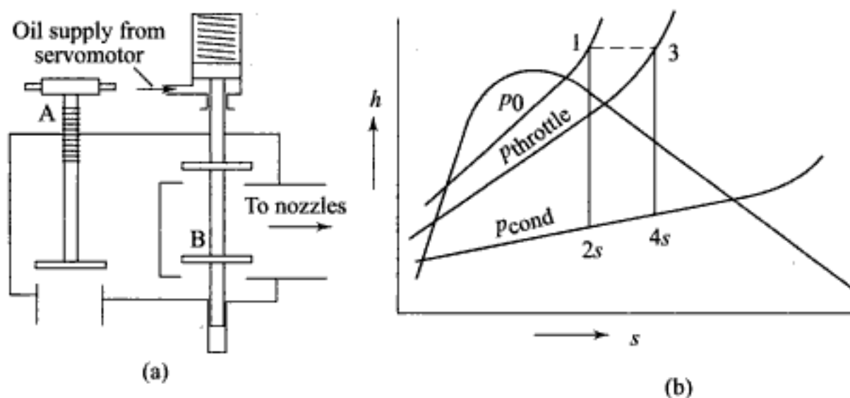
Fig. 7.52 Throttling of steam
