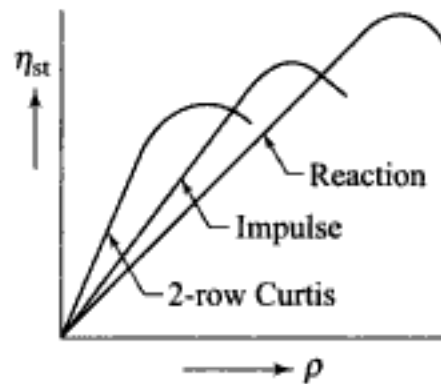
Fig. 7.47 Typical stage efficiencies
