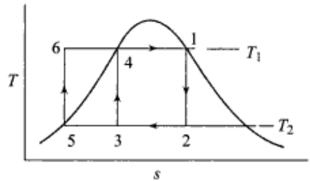
Fig. 2.8 Carnot cycle
