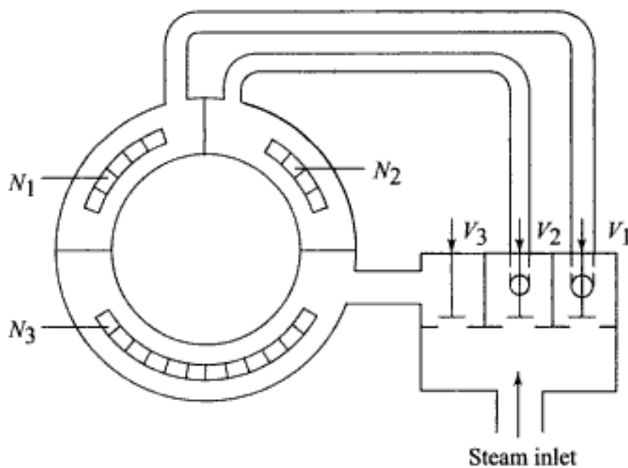
Fig. 7.54 Nozzle governing
