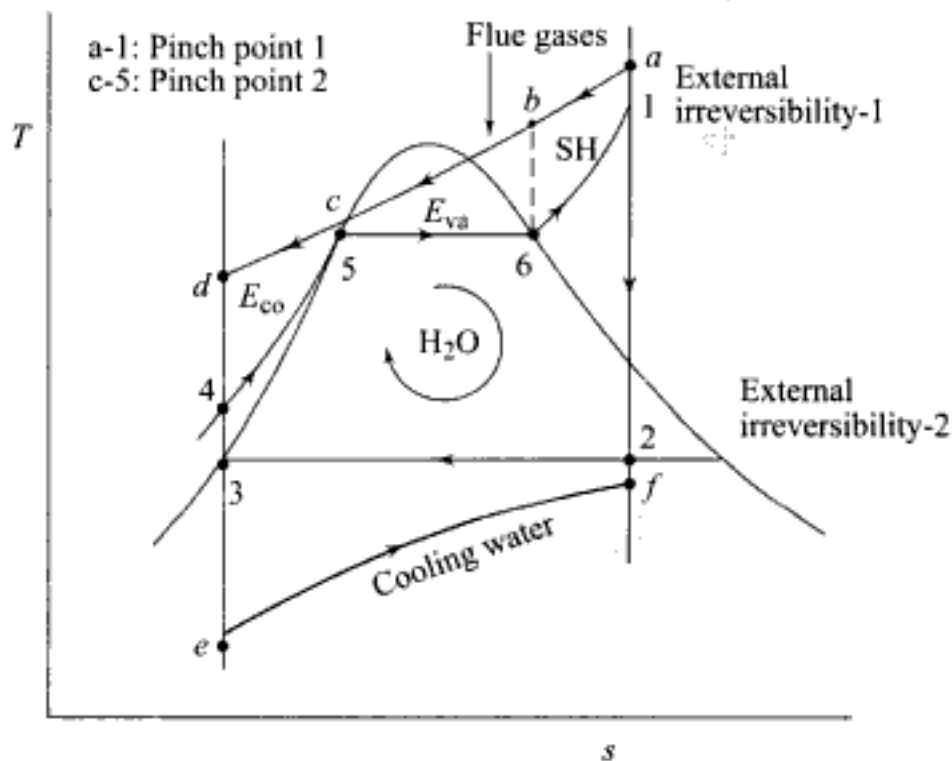
Fig. 2.7 External irreversibility with Rankine cycle
