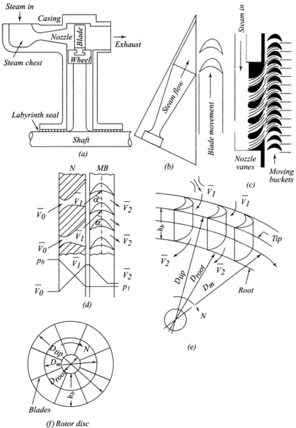
Fig. 7.17 Flow through impulse blades
