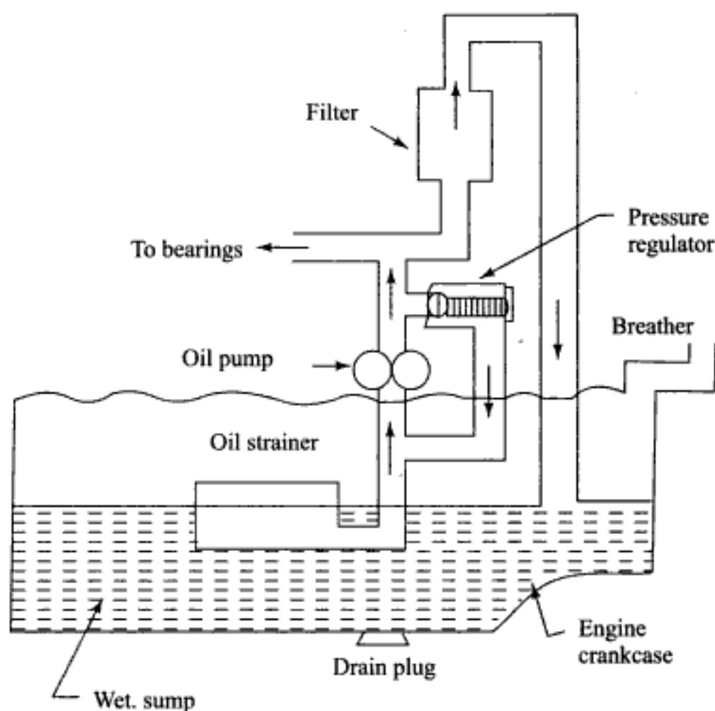
Fig. 11.18 By-pass type wet sump lubrication
