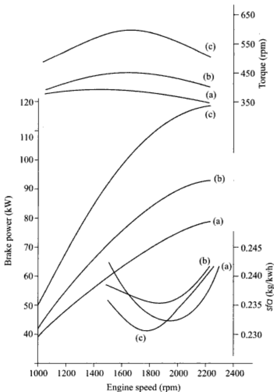
Fig. 11.35 Continuous running performance characteristics of a CI engine in three modes: (a) Normally aspirated, (b) Turbocharged and (c) Turbocharged with intercooling
