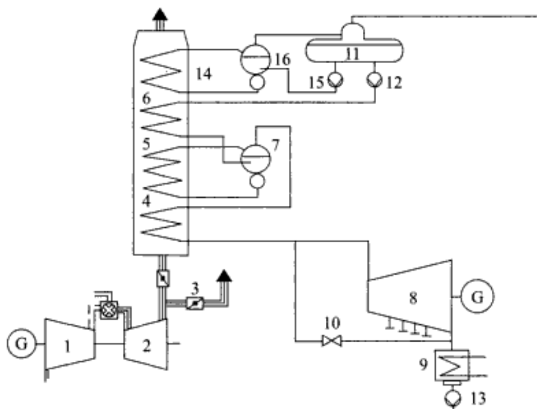
Fig. 3.28 Combined-cycle plant with existing steam turbine
