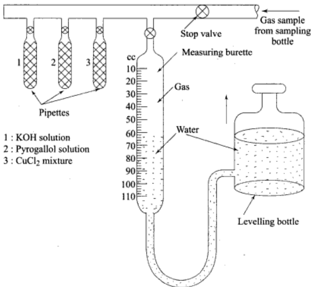
Fig. 4.7 Orsat analyzer
