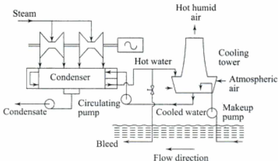
Fig. 8.17 Schematic usual view of a wet cooling tower operating in the closed mode
