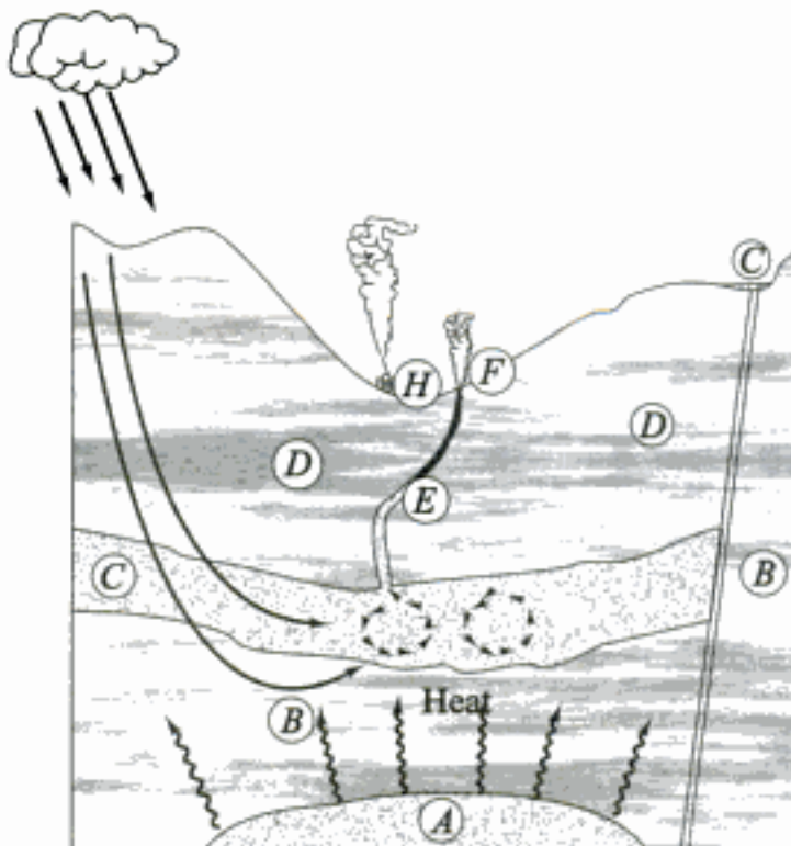
Fig. 14.31 A typical geothermal field
