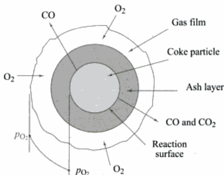
Fig. 5.5 Burning of a coke particle
