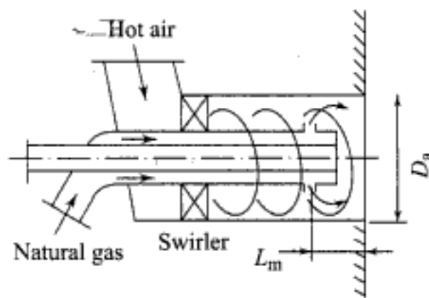
Fig. 5.65 Gas burner with central gas supply
