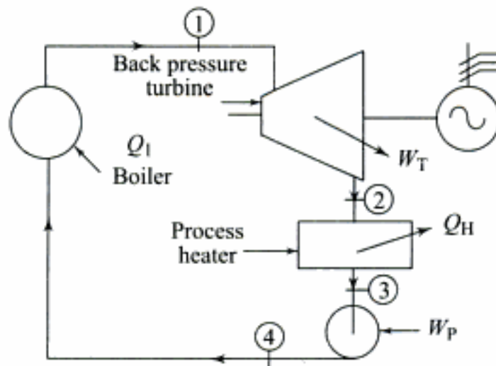
Fig. 2.33 Cogeneration plant with a back pressure turbine
