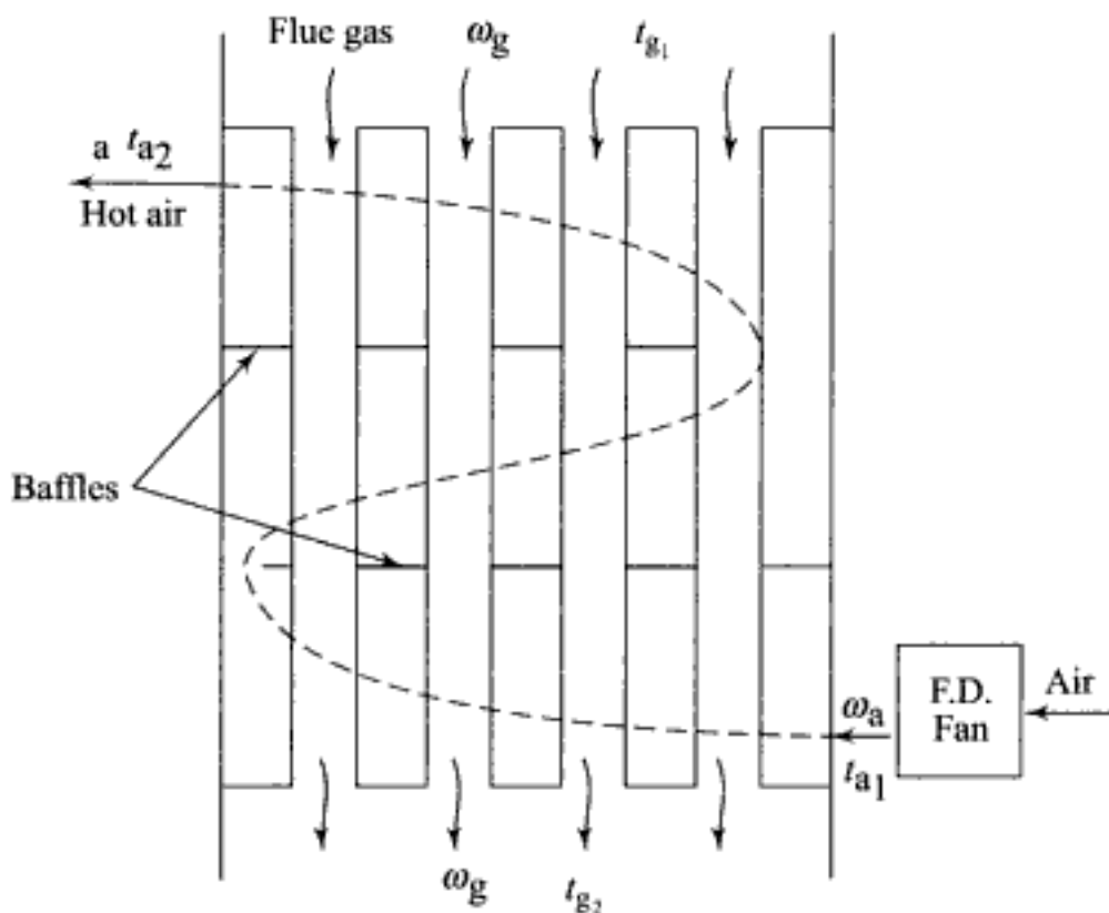
Fig. 6.45 (a) Tubular air preheater
