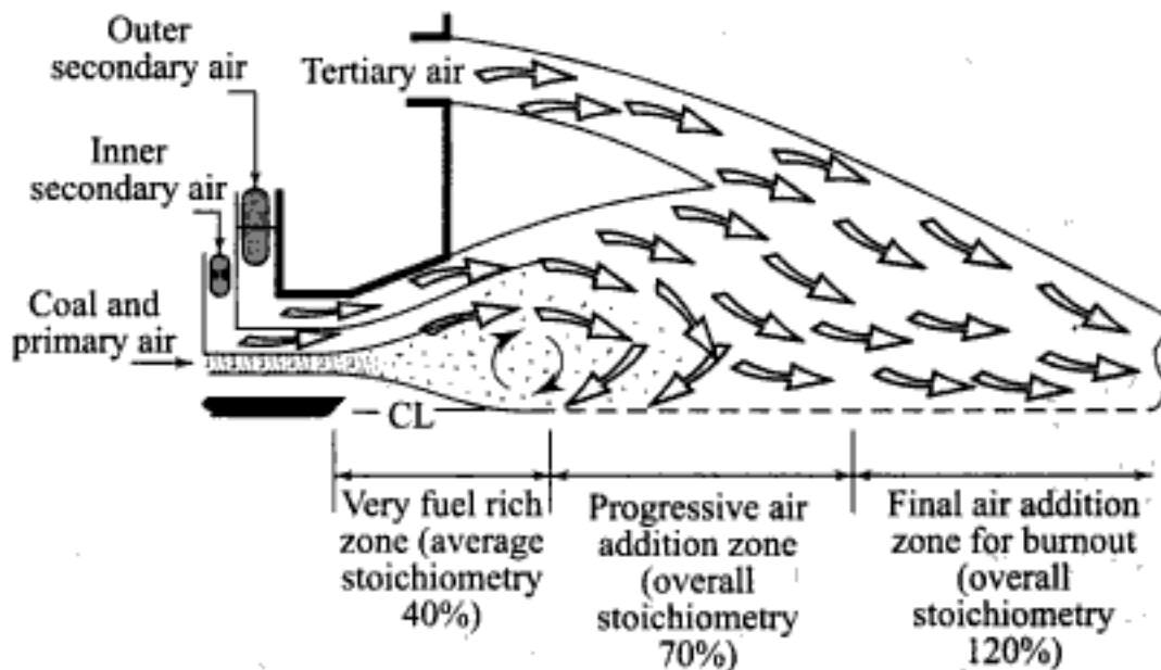
Fig. 5.30 (b) Distributed burner mixing concept
