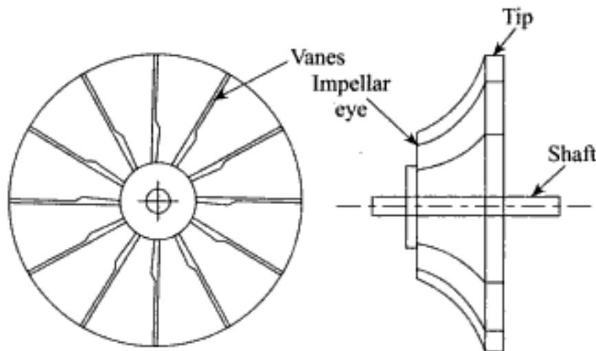
Fig. 11.53 Centrifugal compressor impeller
