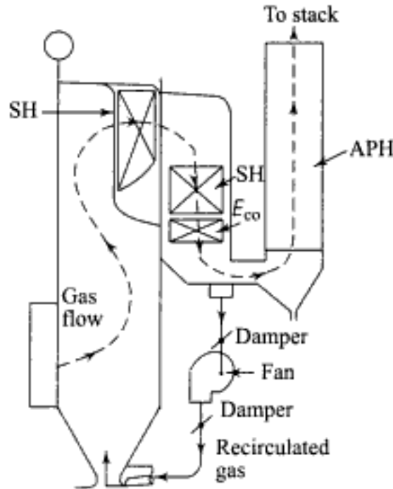
Fig. 6.41 Gas recirculation for steam temperature control
