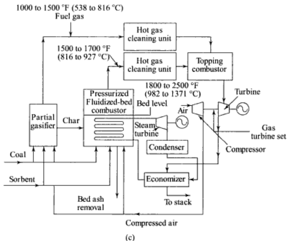
Fig. 6.56 PFBC units in (a) combined cycle, (b) turbocharged cycles, and (c) hybrid advanced cycle
