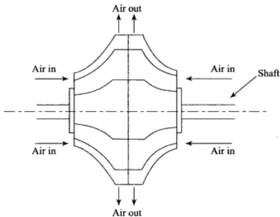
Fig. 11.55 Double-sided impeller of a centrifugal compressor
