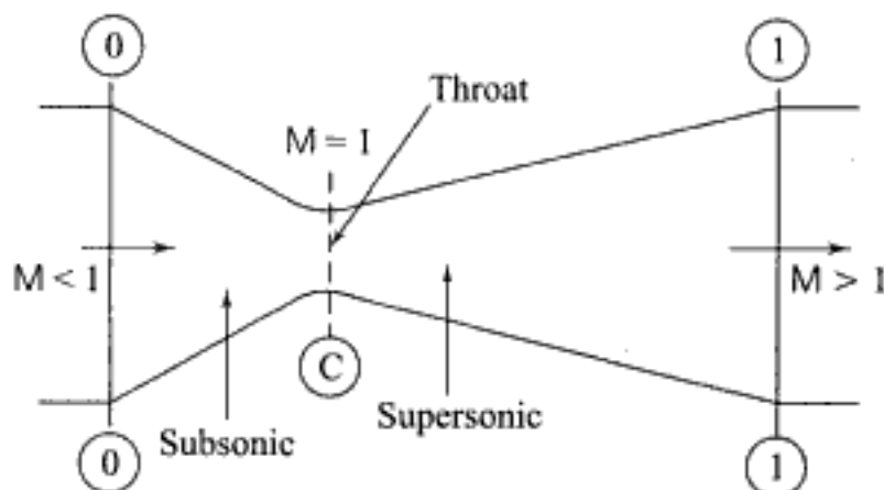
Fig 7.5 Choked flow in a convergent-divergent nozzle
