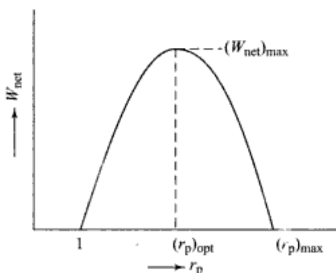
Fig. 11.42 Variation of net cycle work with r_p
