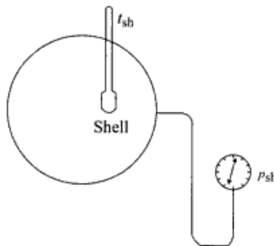
Fig. 8.10 Condenser shell pressure and temperature
