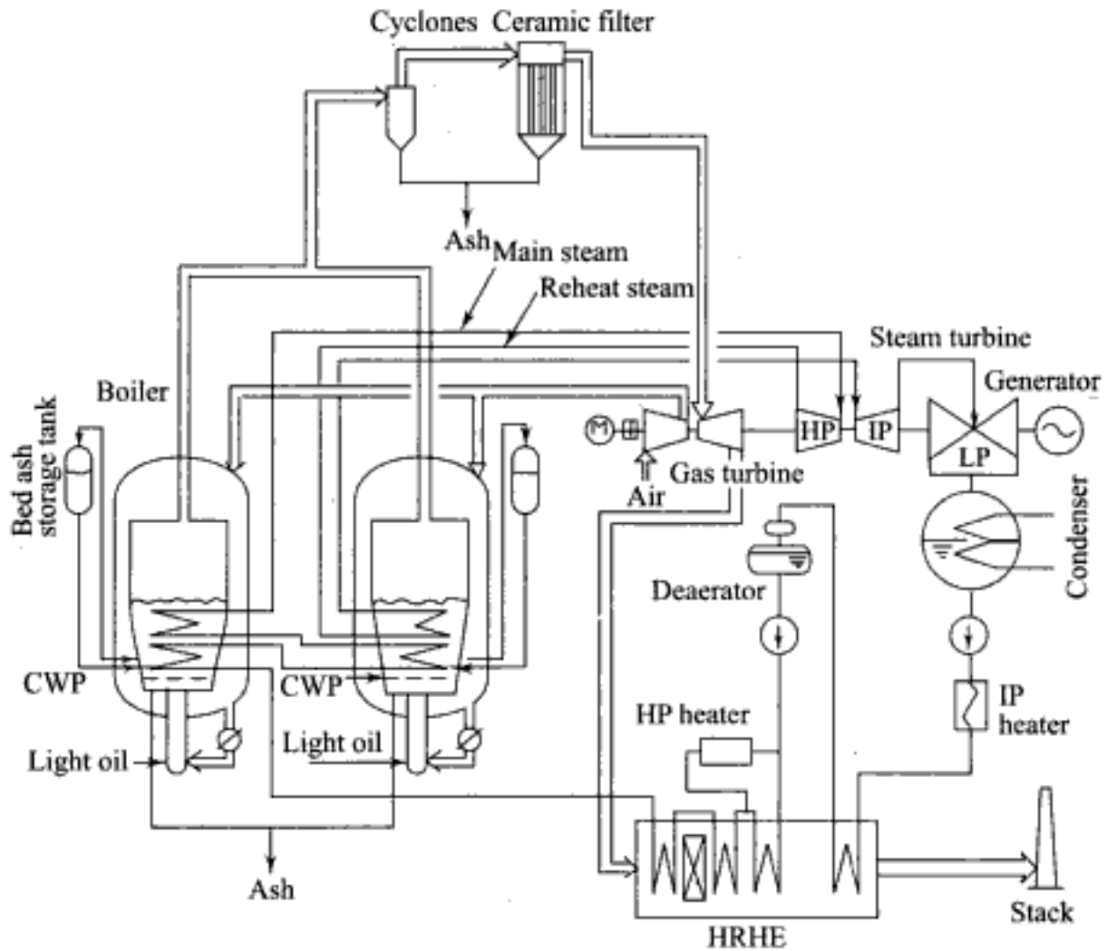
Fig. 5.52 Schematic diagram of the 250 MWe PFBC system at Ohsaki, Japan
