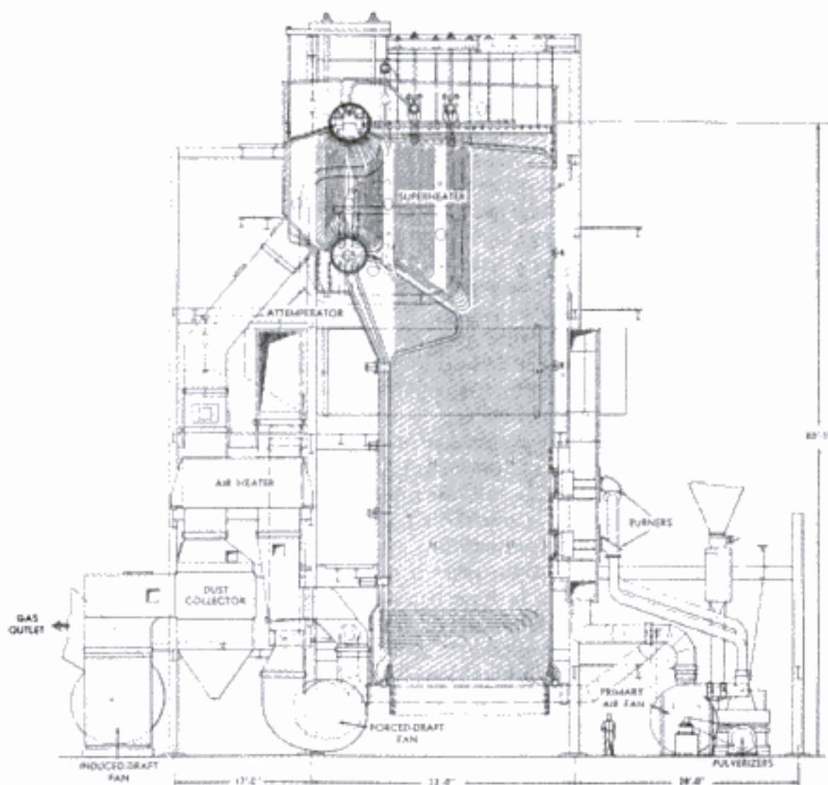
Fig. 6.18 A two drum natural circulation steam generator
