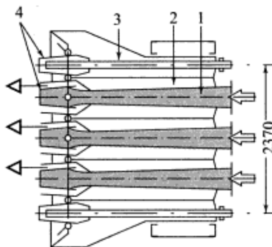
Fig. 5.27 An assembly of three straight-flow pulverized coal burners; 1-supply of fuel-air mixture to burner; 2-secondary air supply; 3-pipe for mounting the fuel-oil burner with electric gas igniter; 4-tilting air pipes
