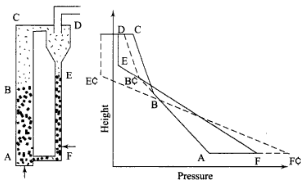
Fig. 5.42 Pressure balance around a CFB loop. The dotted lines indicate the pressure profile at a higher circulation rate
