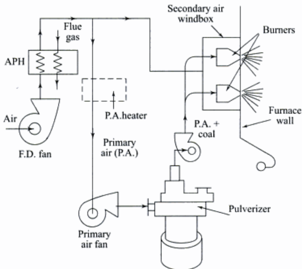
Fig. 5.12 Primary and secondary air in a pulverizer coal firing system
