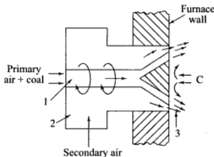
Fig. 5.29 (a) Straight-scroll burner; 1-channel for primary air and coal; 2-scroll for secondary air; 3-mixing zone and ignition; C-suction of gases to the flames
