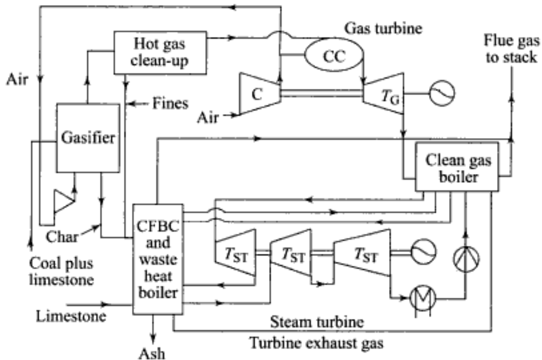
Fig. 3.25 Outline of circulating fluidized bed combustion (CFBC) topping cycle
