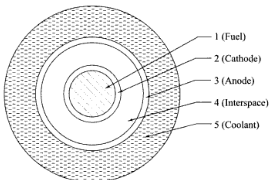
Fig. 13.9 Schematic of a thermionic generator in a nuclear reactor
