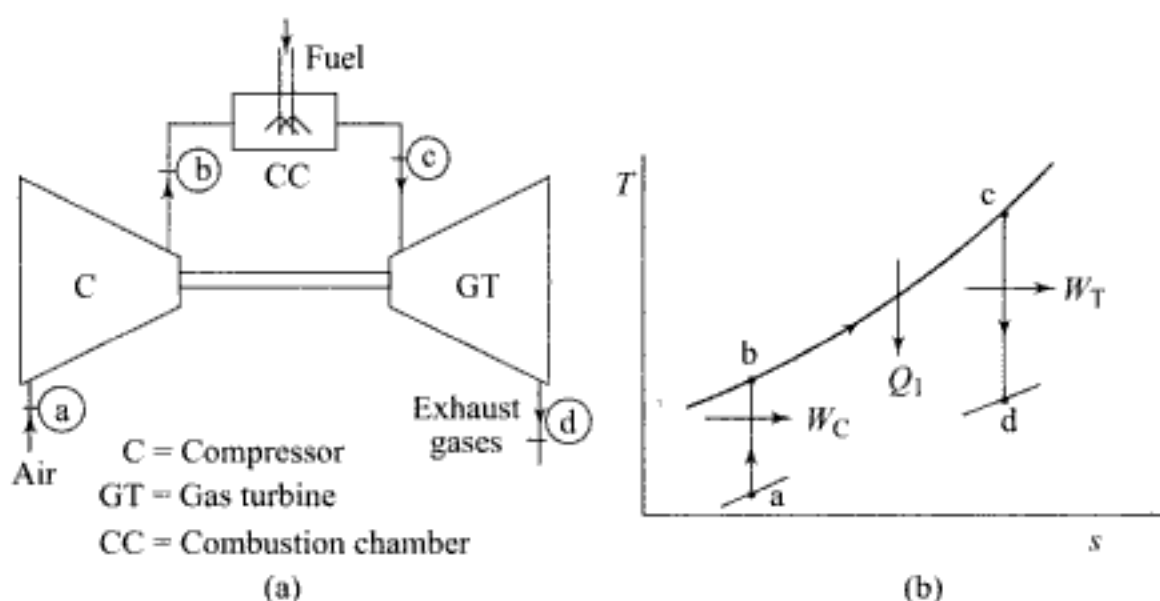
Fig. 3.6 Open cycle gas turbine plant
