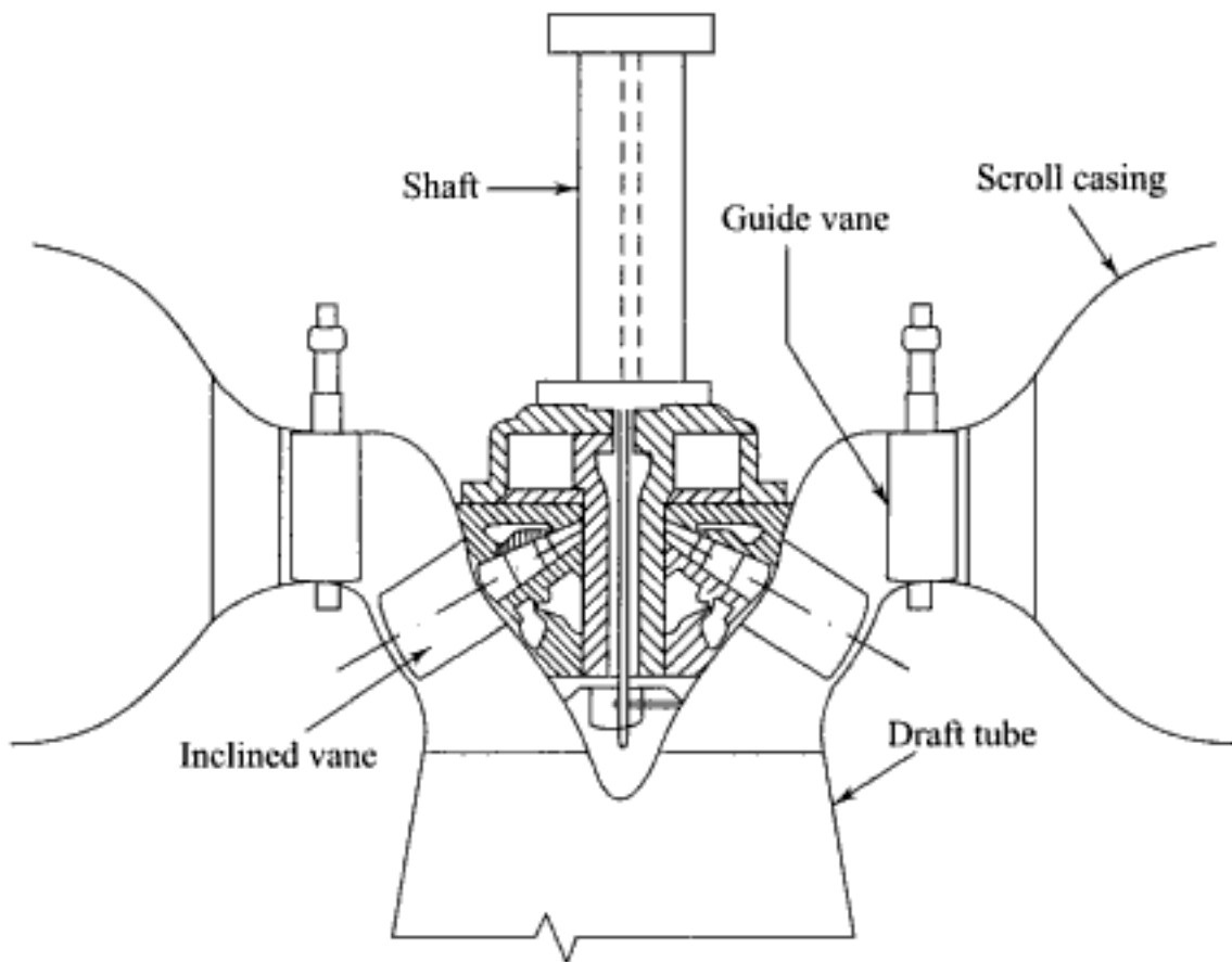
Fig. 10.33 Deriaz turbine
