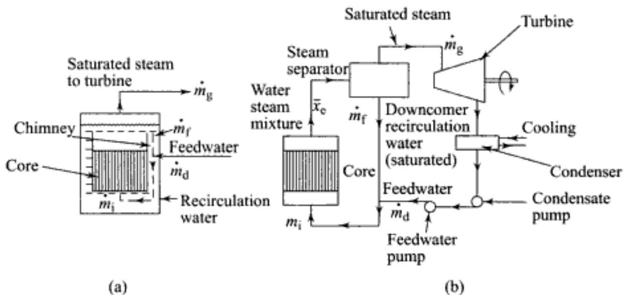
Fig. 9.20 A BWR system with (a) internal and (b) external circulation
