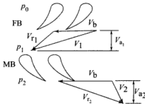
Fig. 7.56 Axial thrust on blades of reaction turbines
