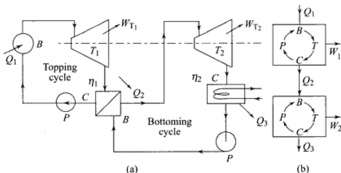
Fig. 3.5 Two vapour power cycles coupled in series
