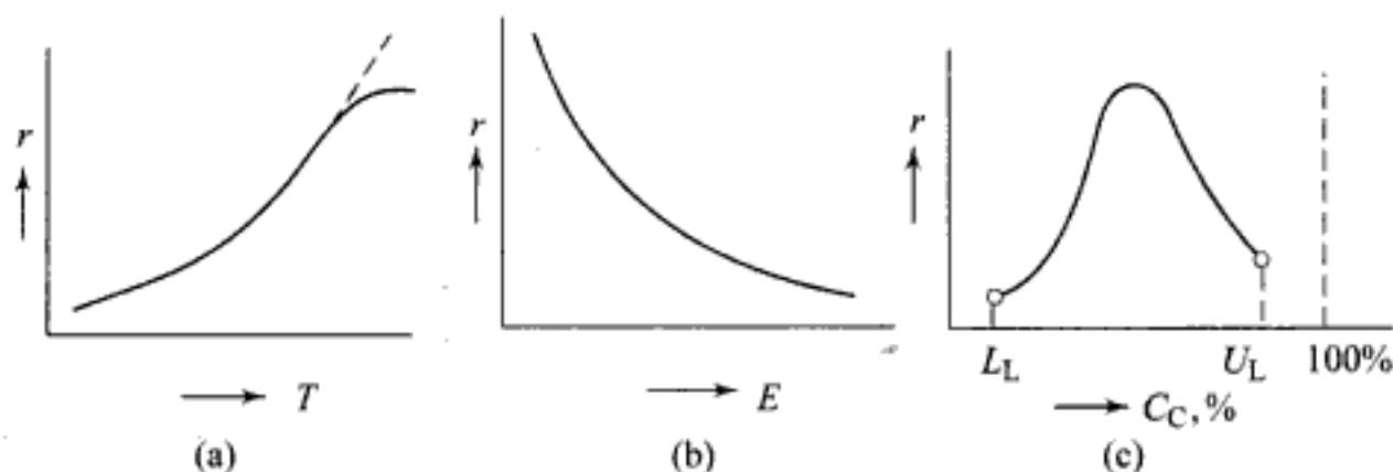
Fig. 5.3 Effect of (a) temperature, (b) activation energy and (c) concentration of combustible matter, on the reaction rate, LL = lower limit, UL = upper limit
