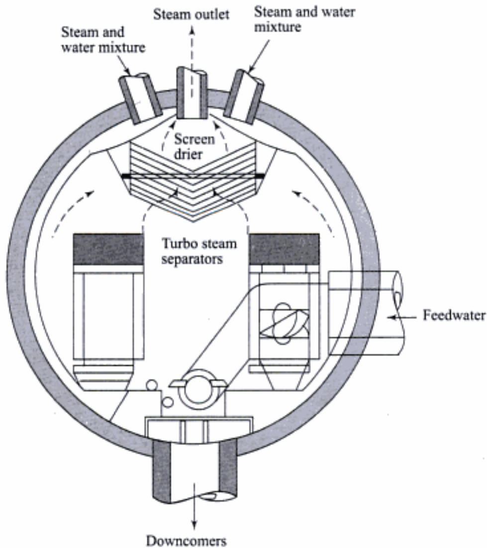
Fig. 6.15 (d) Drum internals of a controlled circulation boiler
