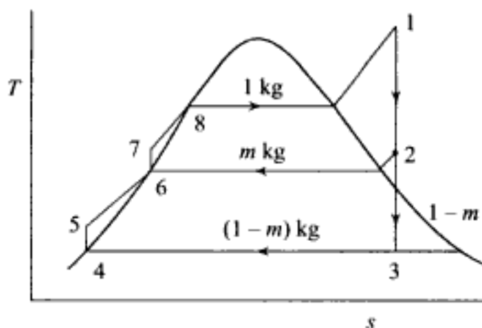
Fig. 2.24 Optimization of regenerative feedwater heating
