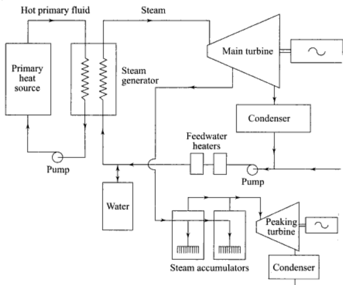
Fig. 12.18 Schematic flow diagram of a power plant with a pressurized water sensible energy storage system
