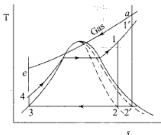
Fig. 2.10 Effect of superheat on the mean temperature of heat addition
