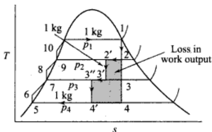
Fig. 2.20 Regenerative cycle for unit mass of fluid
