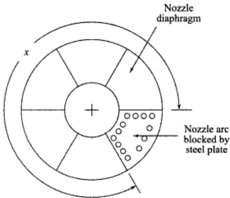
Fig. 7.39 Partial admission of steam in the initial stage
