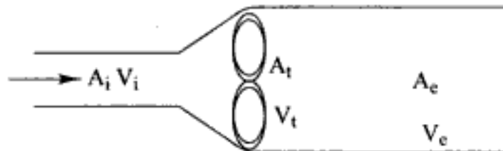
Fig. 14.16 (a) Theory of wind energy conversion
