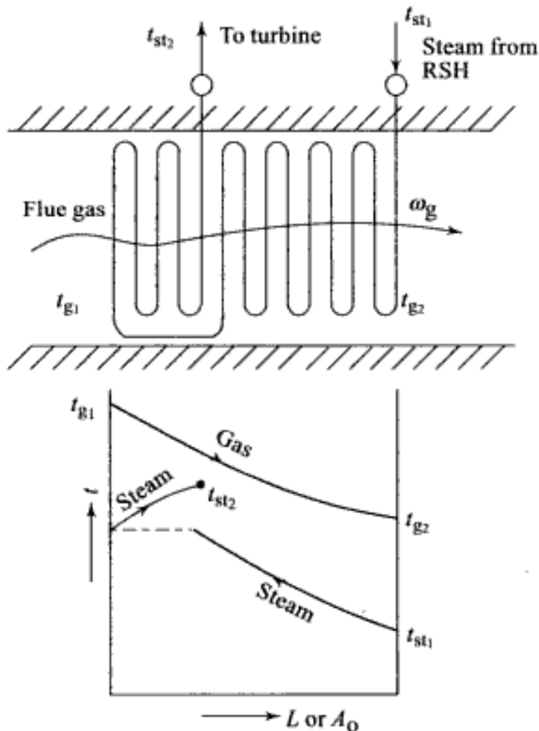
Fig. 6.30 Pendant (mixed flow) superheater
