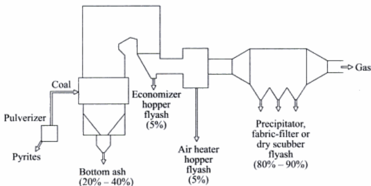
Fig. 6.65 Ash collection and transportation
