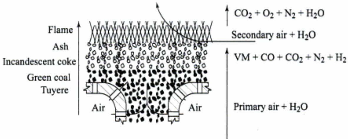
Fig. 5.8 (a) Underfeed fuel bed section receives fresh coal from retort underneath between two tuyeres
