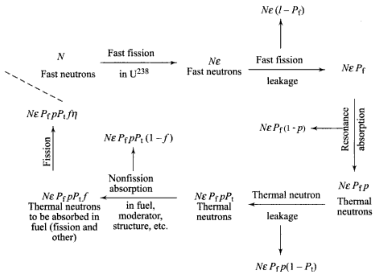
Fig. 9.10 Neutron life cycle in a thermal reactor
