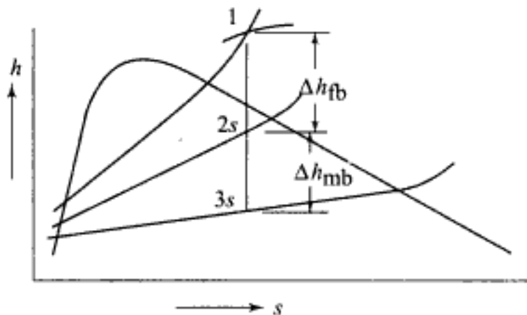
Fig. 7.33 Enthalpy drop in a 50% reaction stage
