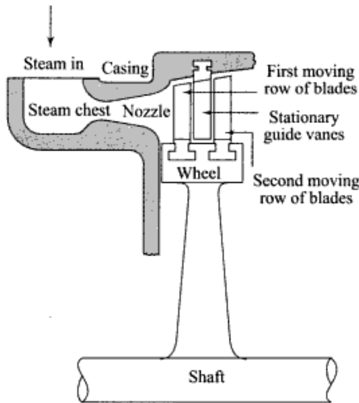
Fig. 7.25 (c) Nozzles and blades in a two-row Curtis stage
