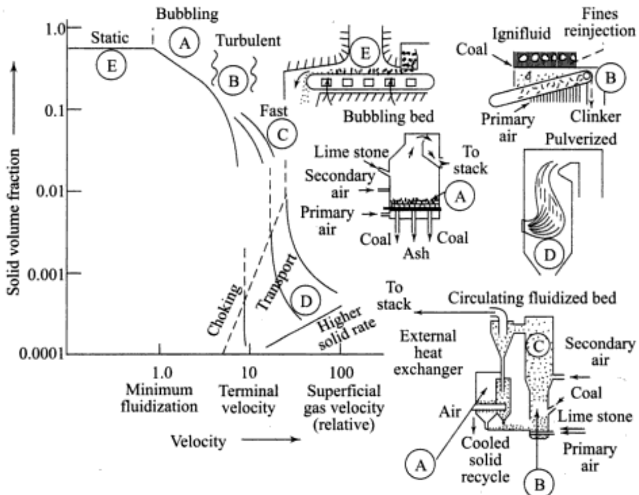
Fig. 5.37 (b) Different commercial combustion systems operating under different gas-solid flow regimes
