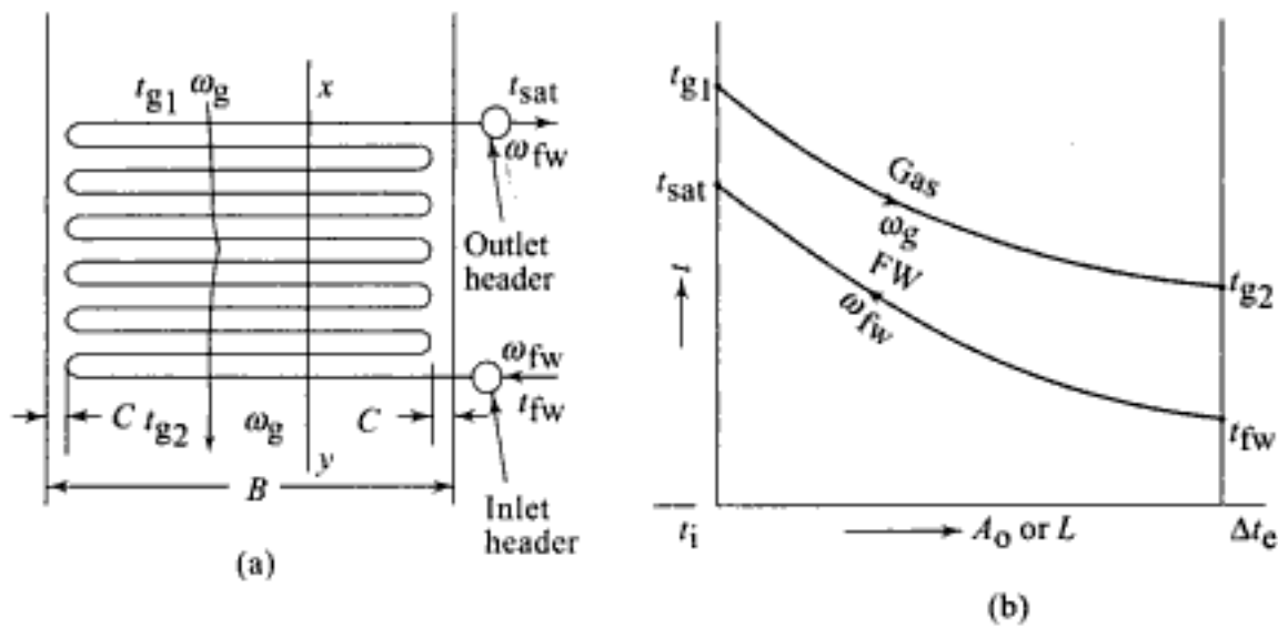
Fig. 6.25 Economiser coil and the temperature profiles of flue gas and water
