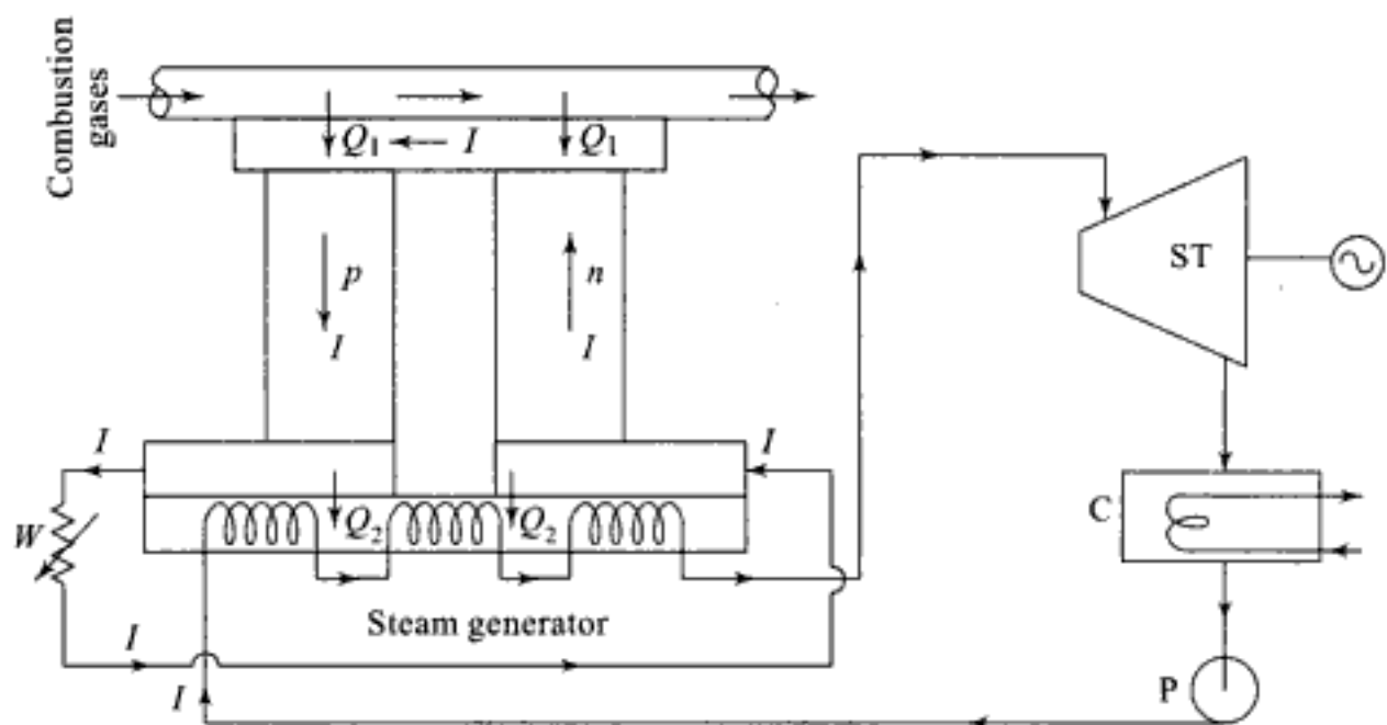
Fig. 13.18 A schematic of combined thermoelectric-steam power plant
