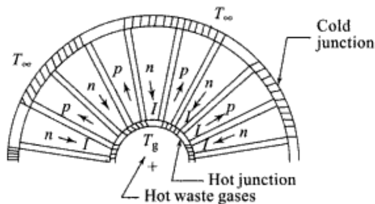
Fig. 13.19 Thermoelectric waste heat stack
