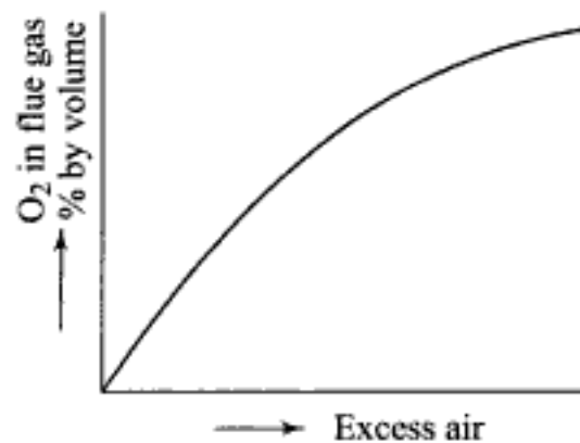
Fig. 4.10 \text{O}_2 variation in flue gas with excess air
