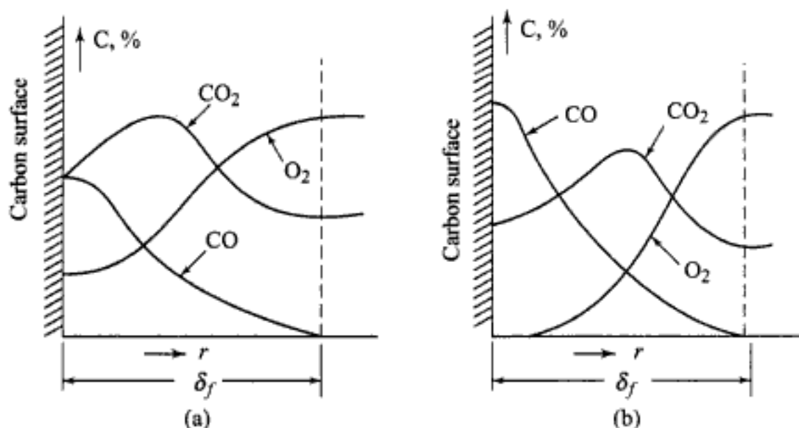
Fig. 5.4 Variation of concentration of gases near the burning carbon surface (a) at moderate temperature, (b) at high temperature; \delta_f = thickness of boundary layer of gases
