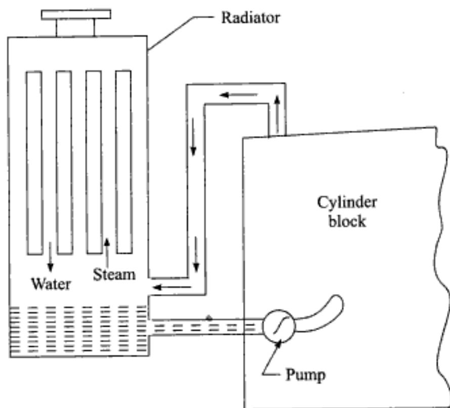
Fig. 11.13 Evaporative cooling
