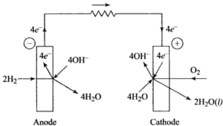
Fig. 13.24 Hydrogen-oxygen fuel cell, Type C
