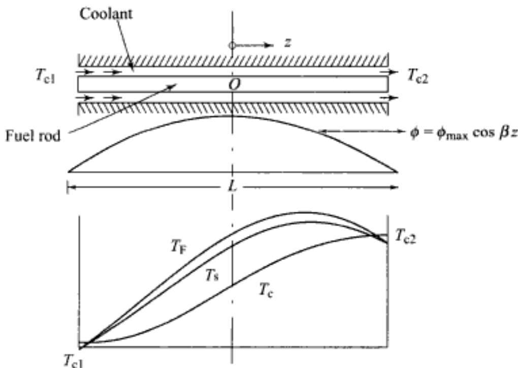
Fig. 9.14 Coolant flow and temperatures in the central fuel channel
