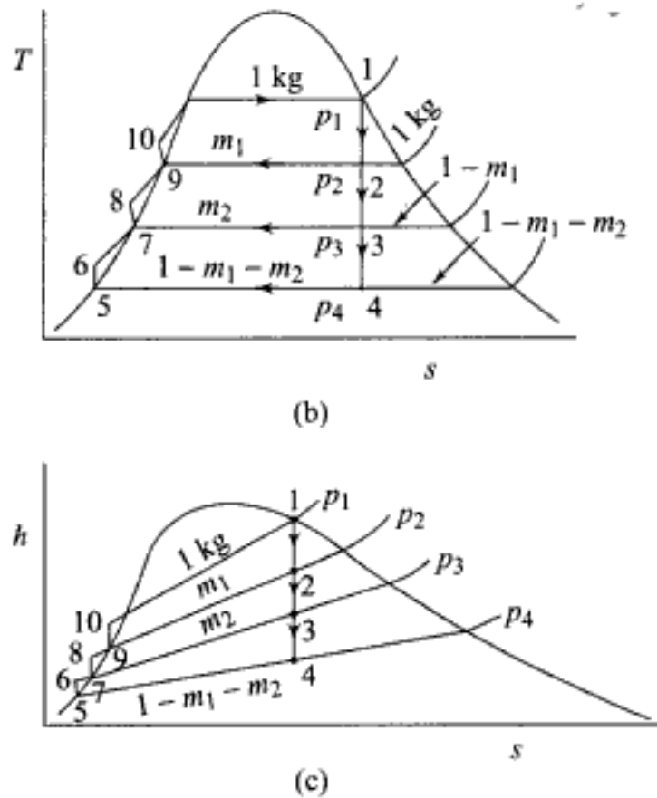
Fig. 2.19 Regenerative cycle with two direct-contact feedwater heaters
