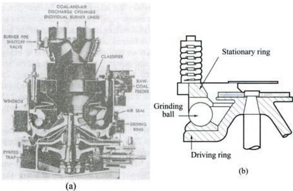
Fig. 5.17 Ball-race mill (a) B and W type, (b) Principle of working
