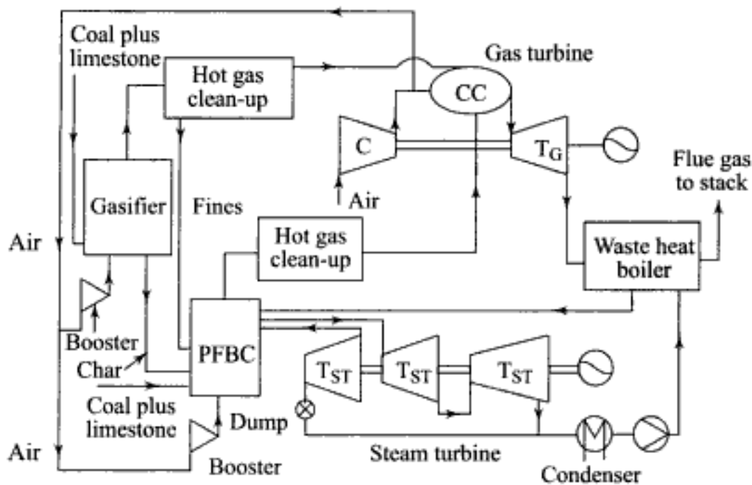
Fig. 3.24 Outline of PFBC topping cycle (single shaft gas turbine)
