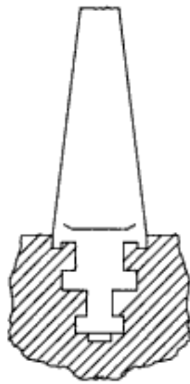
Fig. 7.61 Straddle fastening
