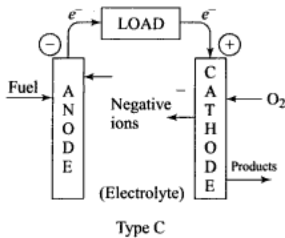
Fig. 13.22 Three different types of fuel-cell reactions
