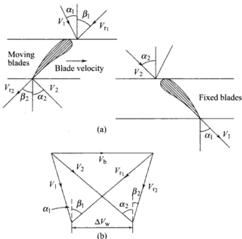
Fig. 11.59 (a) Typical blade sections (b) Blade velocity diagrams for an axial-flow compressor
