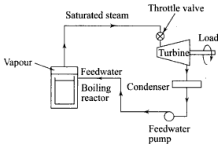
Fig. 9.19 Schematic of a direct-cycle BWR plant
