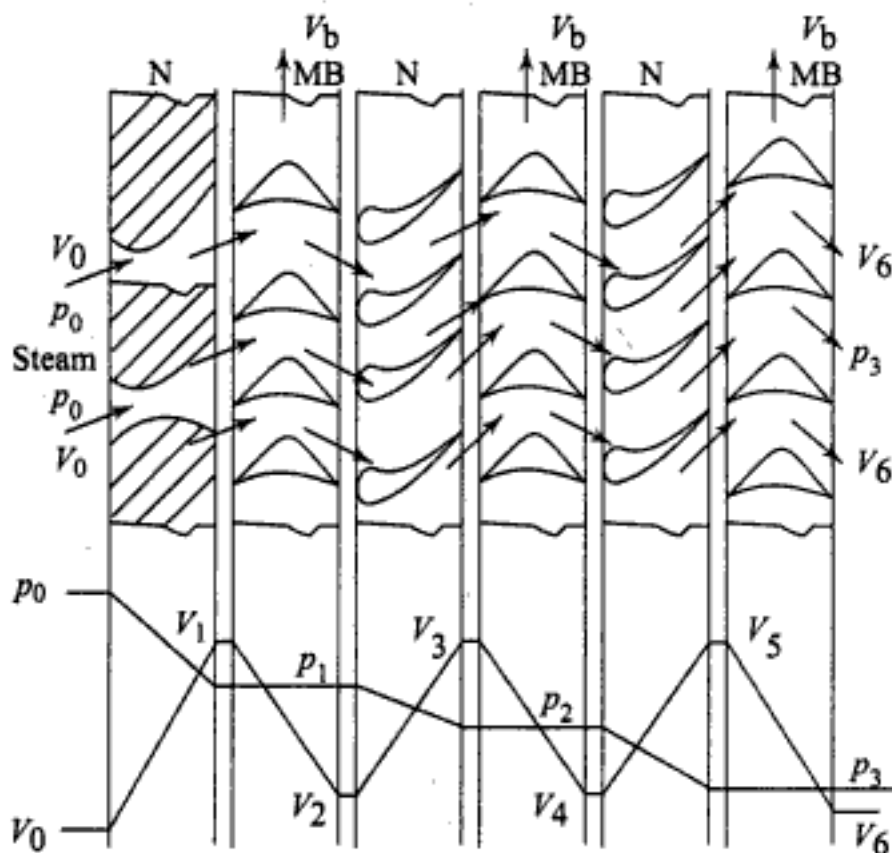
Fig. 7.23 (b) Three pressure (or Rateau) stages in series
