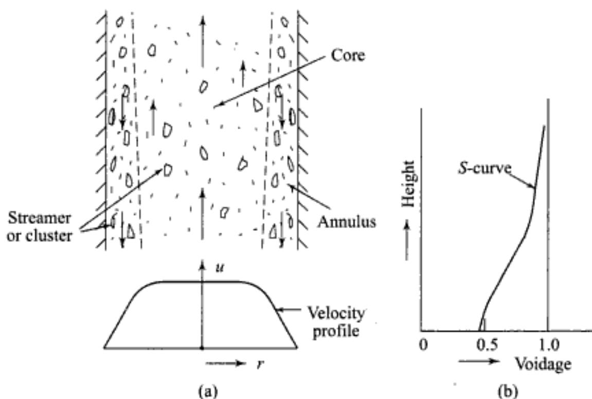
Fig. 5.41 (a) Core-annulus structure of a CFB: (a) upflowing core (dilute suspension of gas solid mixture) and downflowing annulus (dense phase of gas and solids), (b) voidage variation along height
