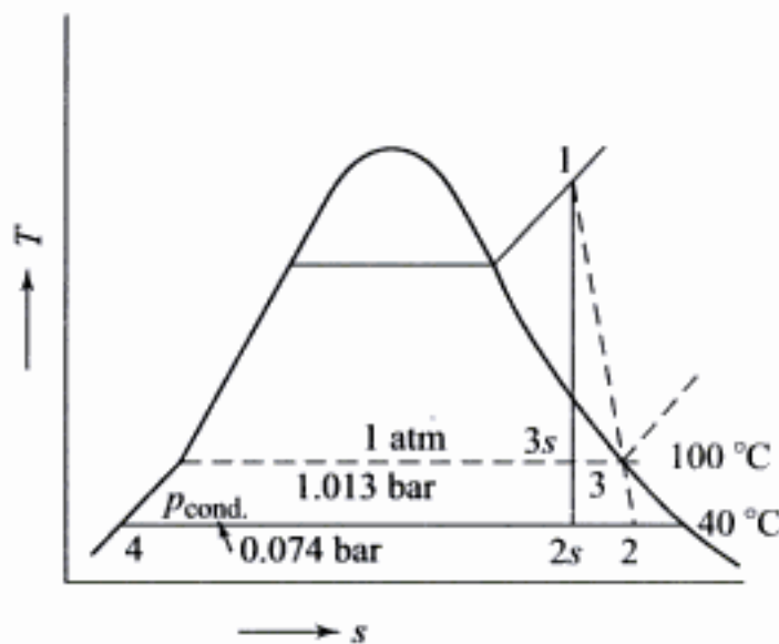
Fig. 8.1 The use of condenser increases the specific work output of turbine from (h_1 - h_3) to (h_1 - h_2)
