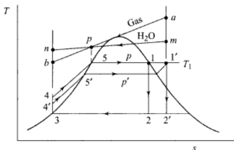
Fig. 2.11 Superheat may not be practical with hot pressurized water as heat source as in a PWR
