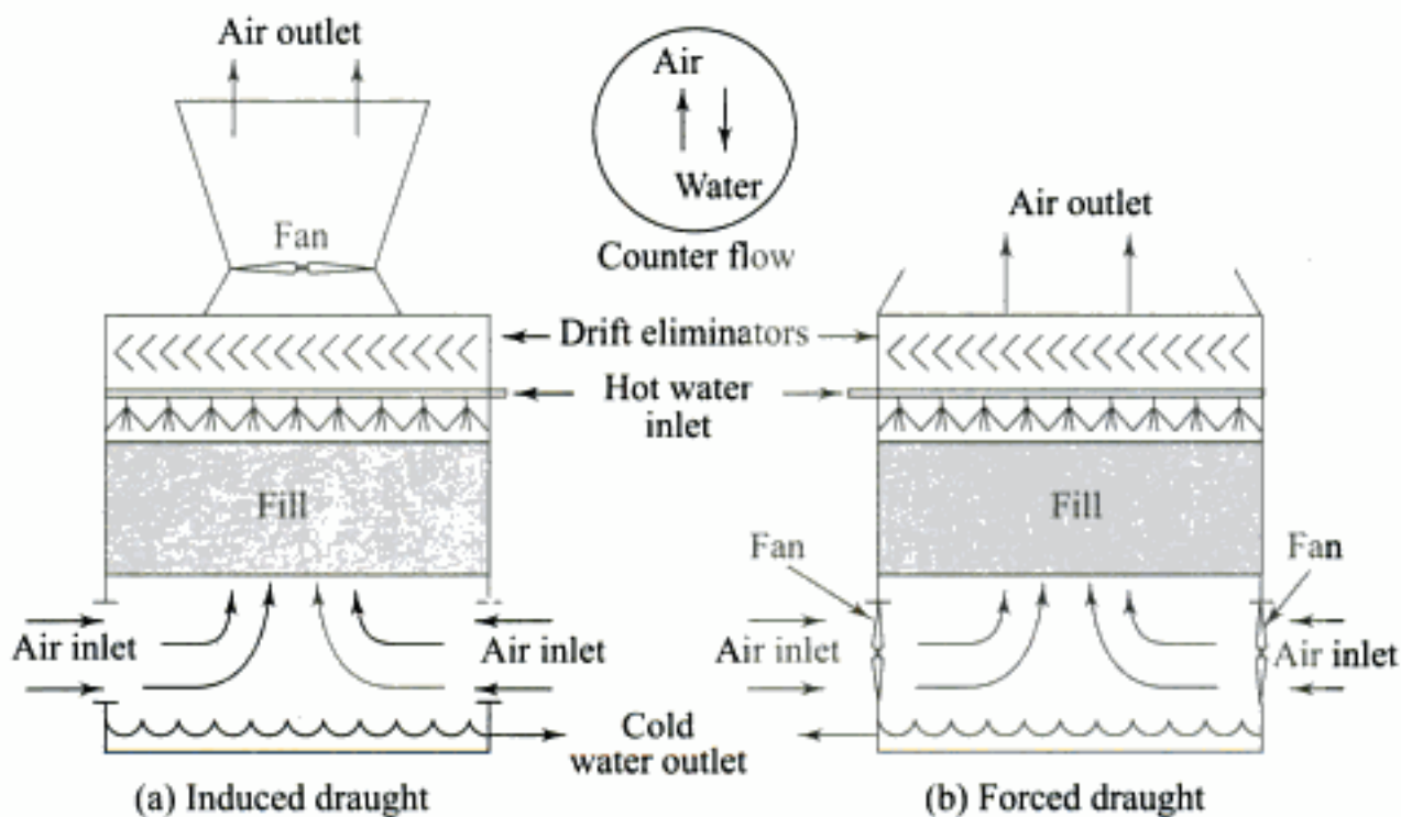
Fig. 8.19 Induced draught counterflow cooling towers
