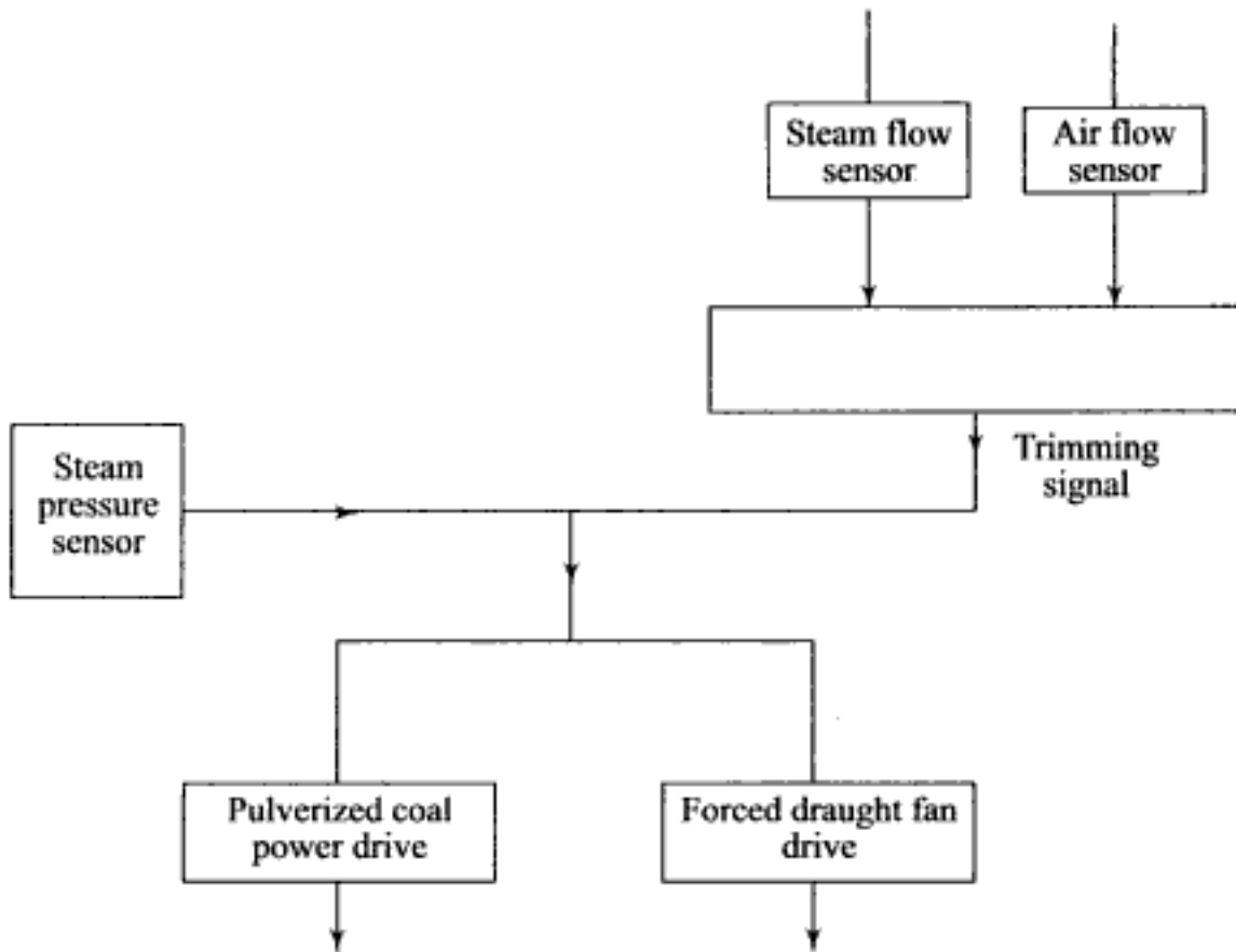
Fig. 6.35 Schematic of a steam pressure control system
