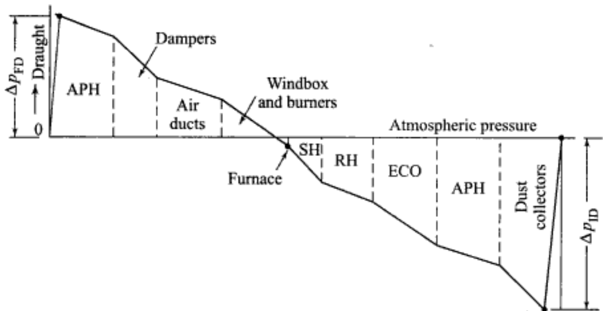
Fig. 4.16 Balanced draught system in a modern boiler
