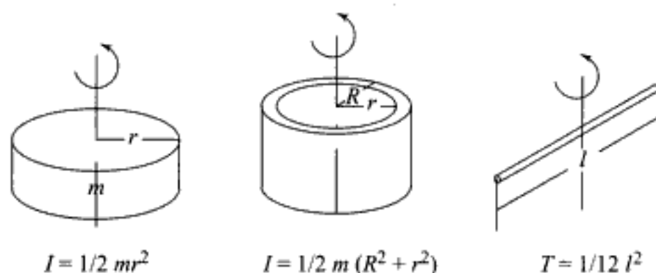
Fig. 12.10 Moment of inertia for disc, cylinder and bar shaped flywheel
