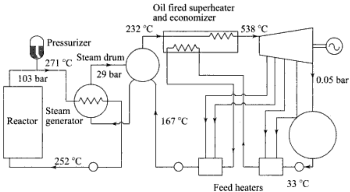
Fig. 9.17 The Indian Point (USA) PWR with oil-fired superheater
