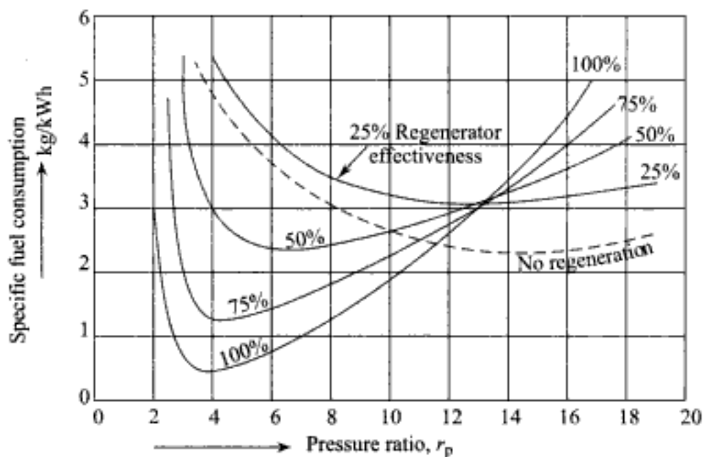
Fig. 11.49 Effect of regenerator effectiveness on specific fuel consumption
