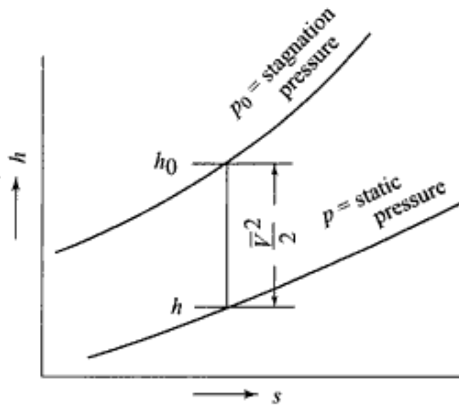
Fig. 7.3 Stagnation state
