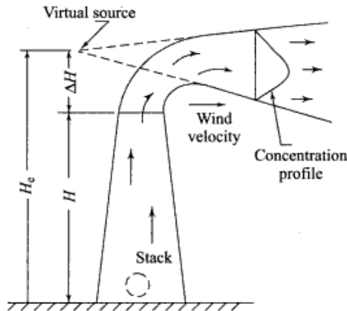
Fig. 4.15 Dispersion of flue gases at stack exit
