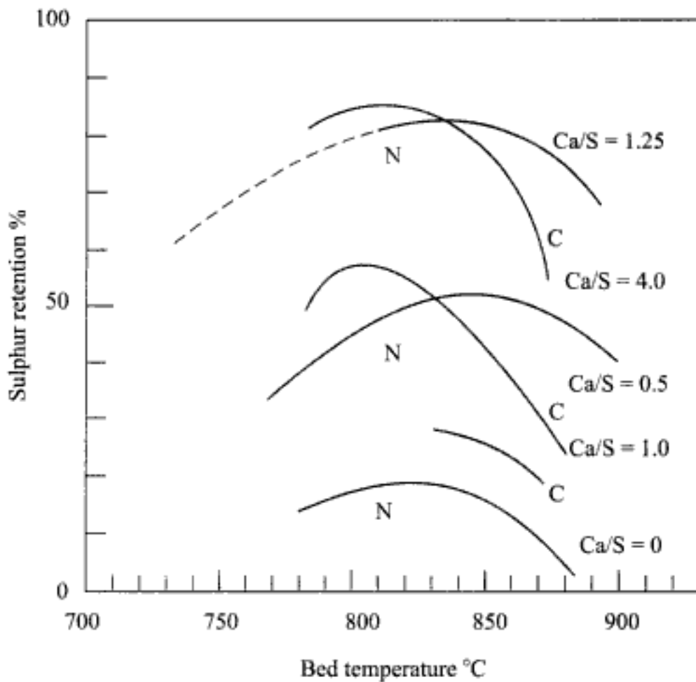
Fig. 6.55 (a) Sulphur capture in atmospheric BFBC at various Ca/S molar ratios as a function of bed temperature
