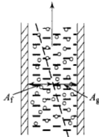
Fig. 6.12 Two phase flow in a riser
