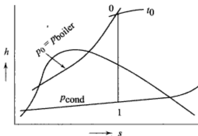
Fig. 7.22 Single stage expansion of steam
