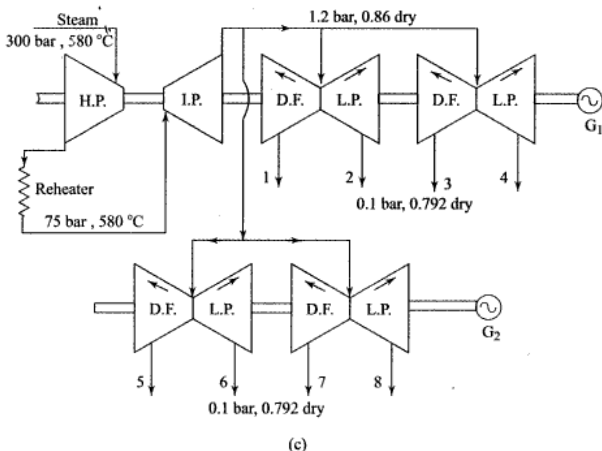
Fig. E7.27(c) Cross compounded octuple flow (8-exhausts) 6-casing, 2-shaft, 3000 rpm, 600 MW steam turbine with reheat
