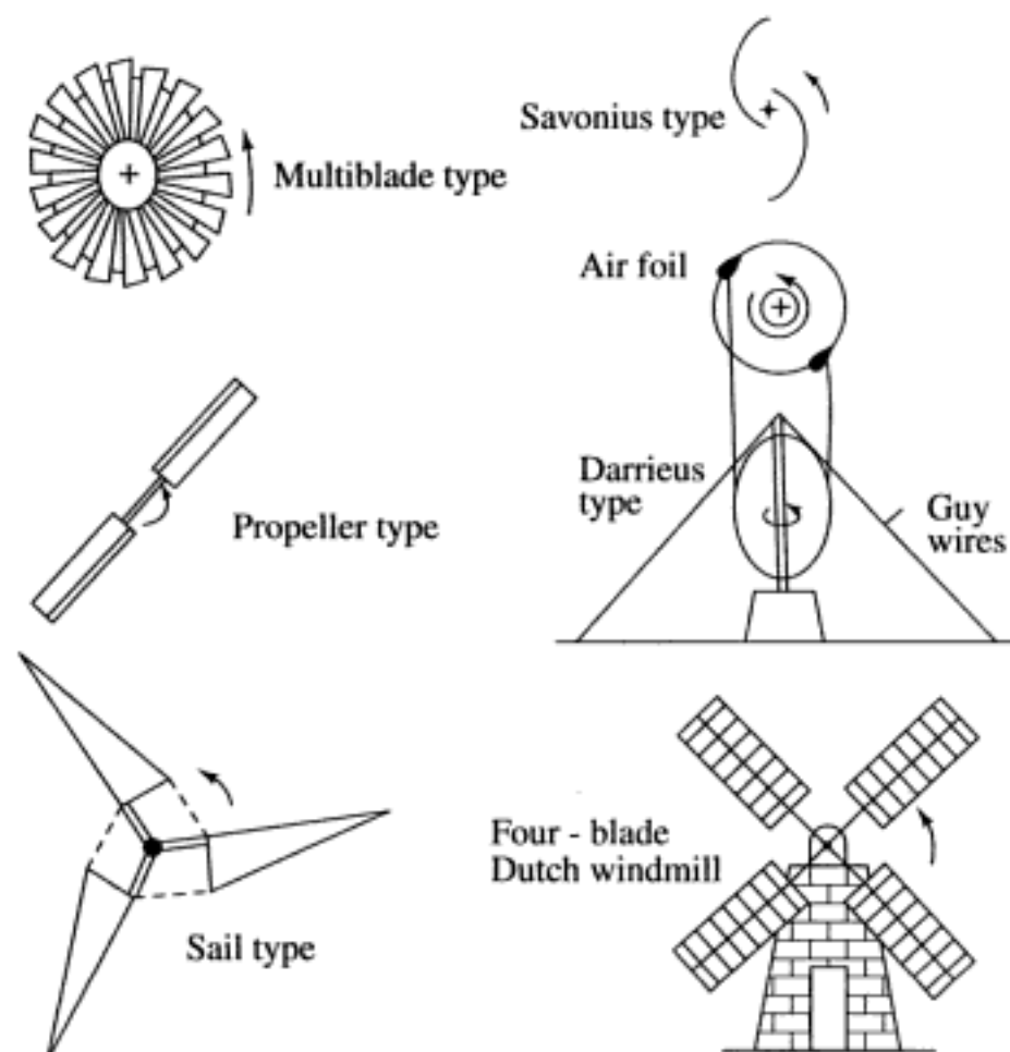
Fig. 14.15 Types of windmill rotors
