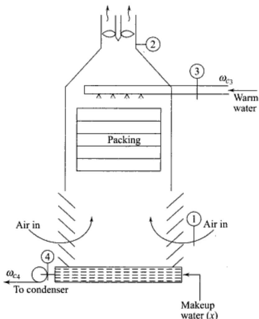
Fig. 8.28 Cooling tower calculations
