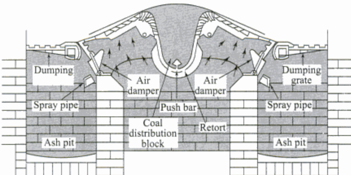
Fig. 5.8 (b) Single-retort stoker showing contour of fuel bed and ash dumps
