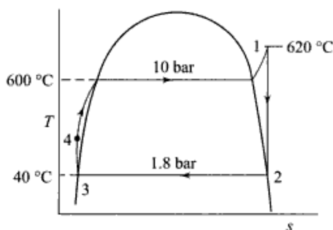
Fig. 3.1 T - s diagram of an ideal working fluid for a vapour power cycle
