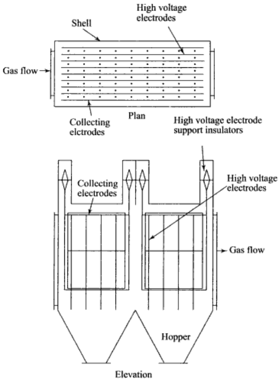
Fig. 6.62 Arrangement of an electrostatic precipitator
