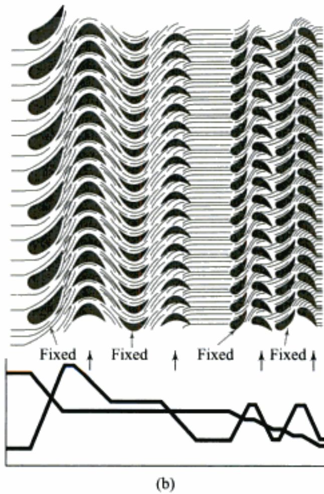
Fig. 7.30 Variation of pressure and velocity in (a) two reaction stages, (b) in a two-row Curtis stage followed by two reaction stages
