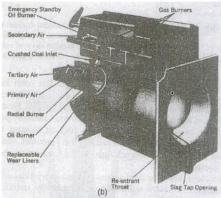
Fig. 5.35 Cyclone furnace
