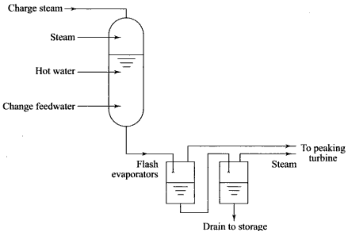
Fig. 12.22 Expansion accumulator with flash evaporator
