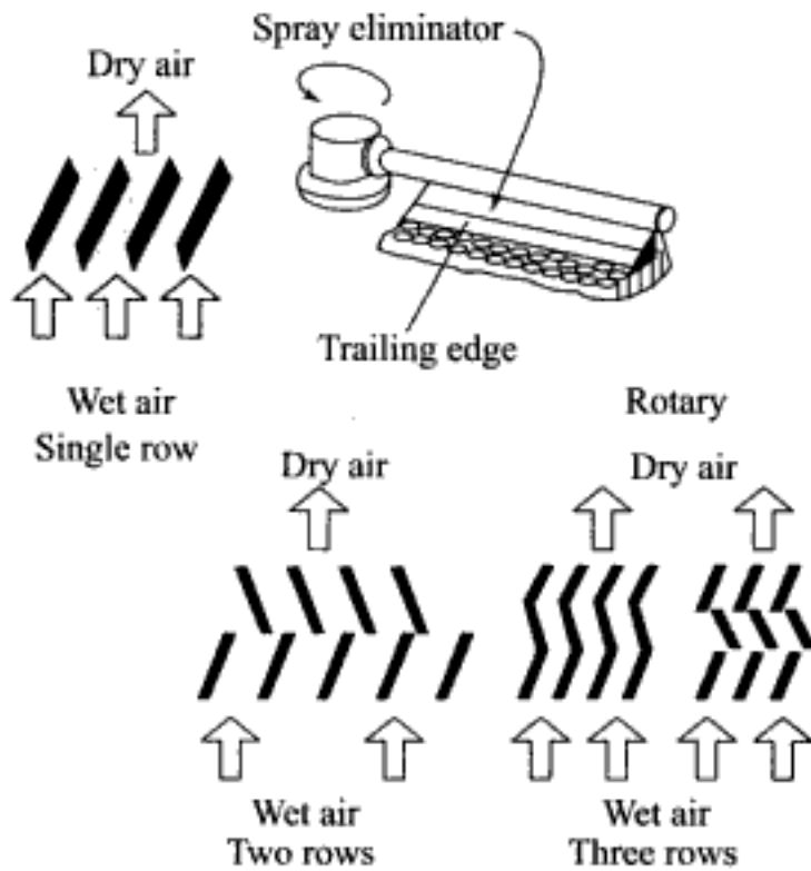
Fig. 8.21 Types of drift eliminators
