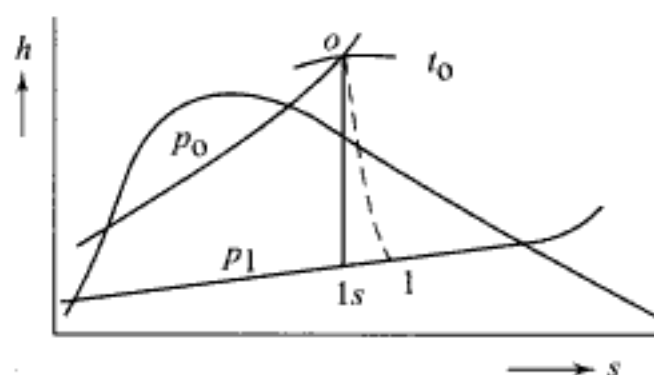
Fig. 7.8 Nozzle efficiency
