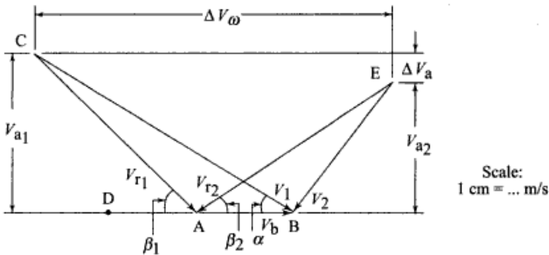
Fig. 7.19 Construction of velocity diagram
