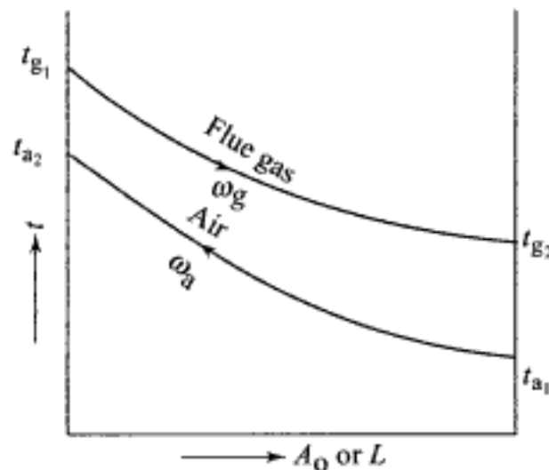
Fig. 6.46 Temperature profiles of gas and air in APH
