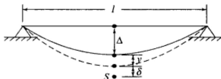
Fig. 7.67 Position of c.g. of shaft in horizontal supports
