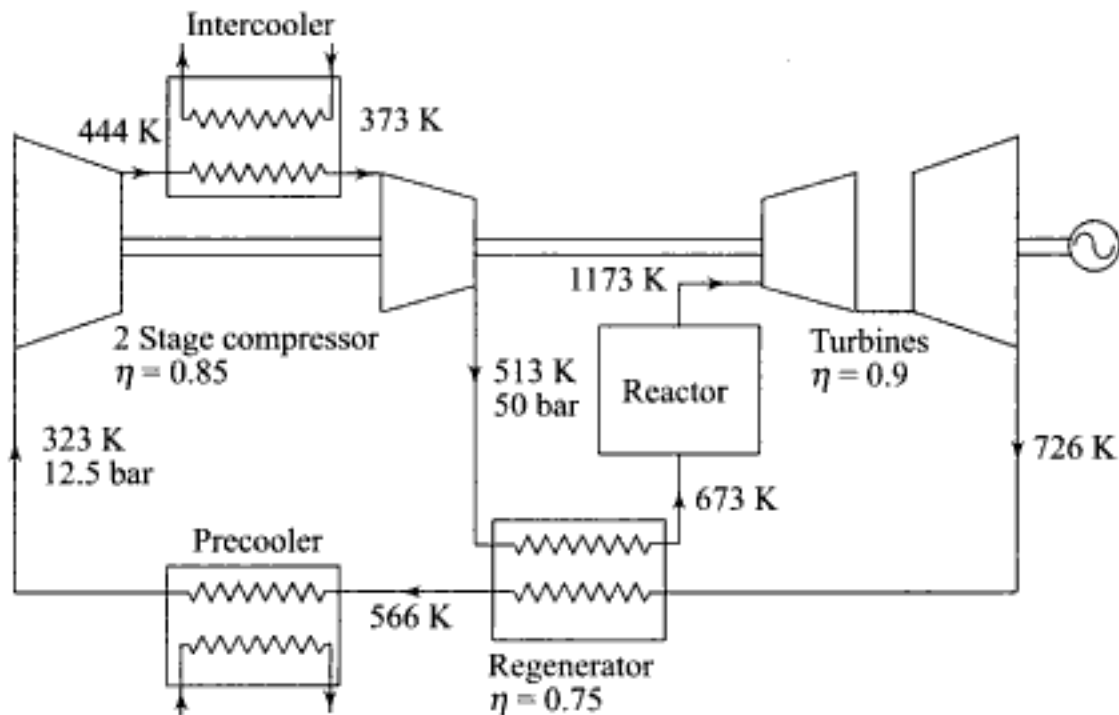
Fig. 9.23 A-HTGR direct cycle gas turbine plant using helium
