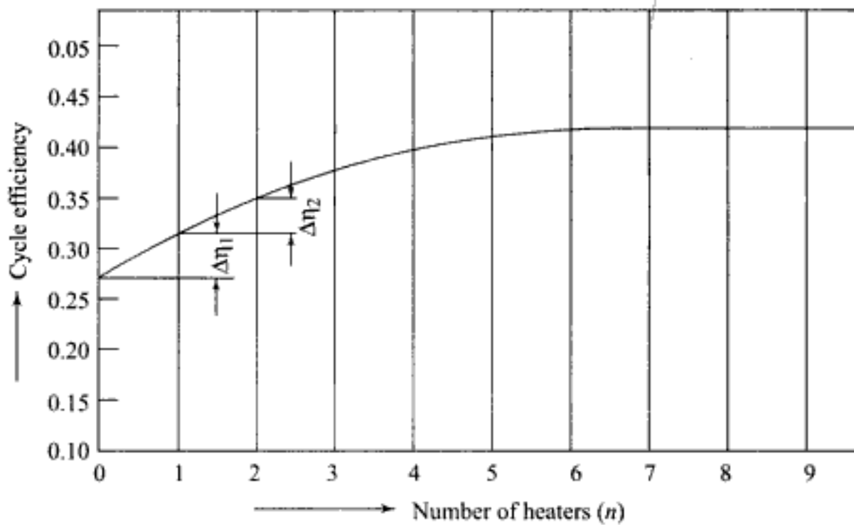
Fig. 2.26 Efficiency gain ( \Delta\eta ) successively diminishes with the increase in the number of heaters
