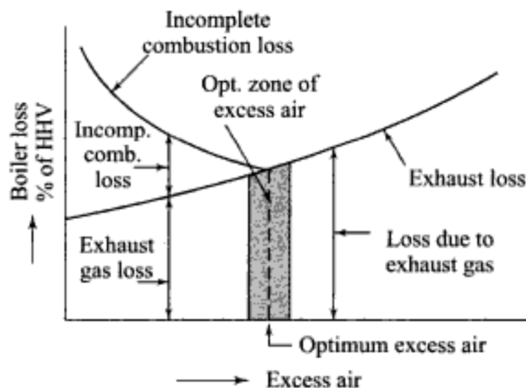
Fig. 4.11 Optimum excess air for maximum combustion efficiency
