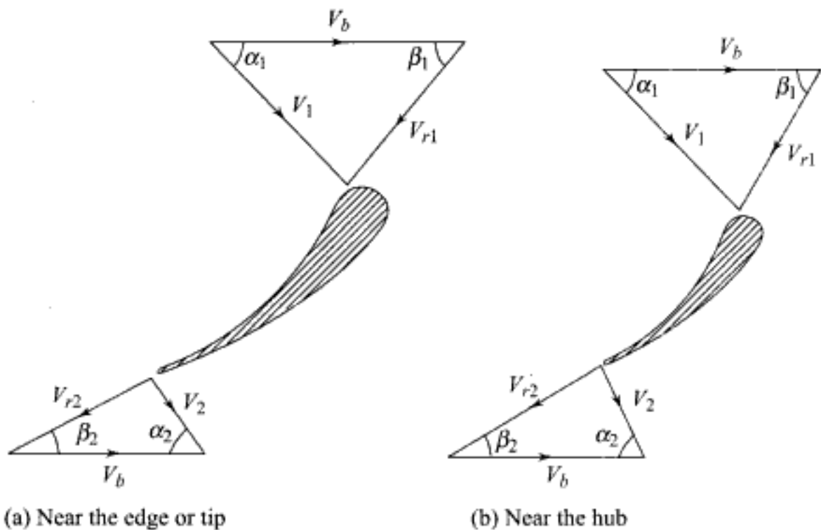
Fig. 10.32 Velocity triangles for propeller or Kaplan runner blade
