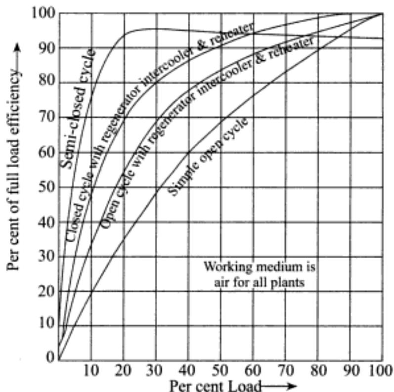
Fig. 11.48 Part load efficiencies of different plants
