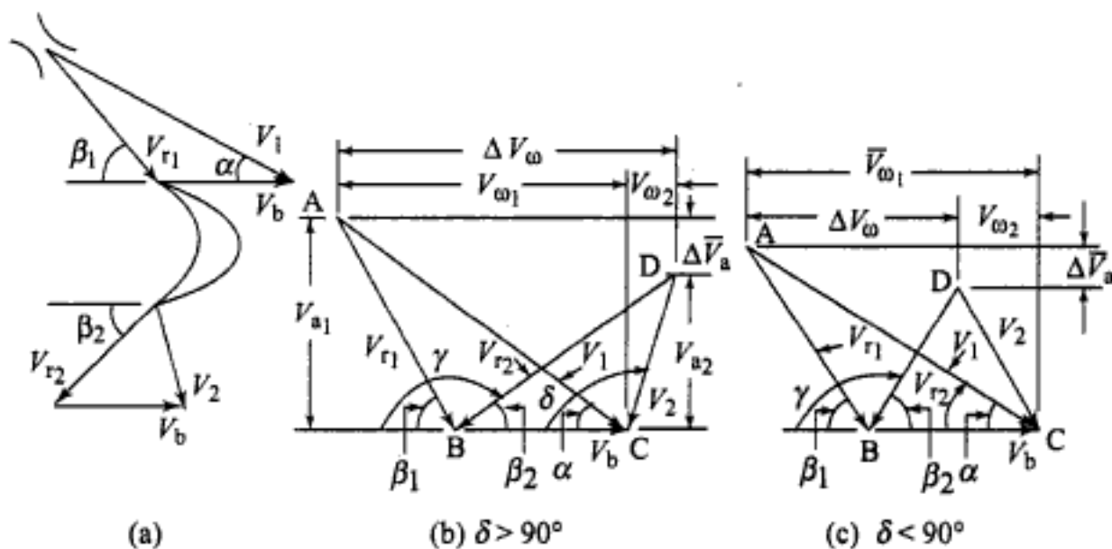
Fig. 7.18 Velocity diagrams for impulse blading
