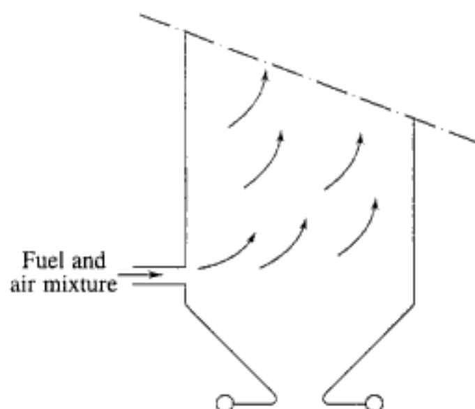
Fig. 5.2 Chamber-type or flame furnace
