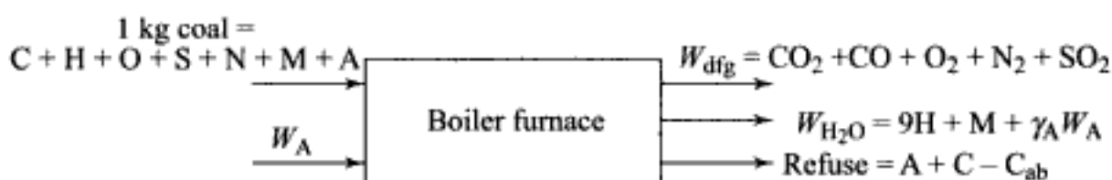
Fig. 4.12 Material balance for a boiler furnace
