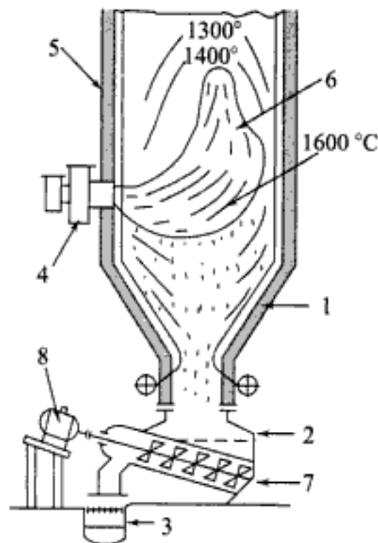
Fig. 5.23 Dry bottom furnace: 1-dry bottom hopper; 2-slag bath with water; 3-hydraulic ash disposal channel; 4-burner; 5-water walls; 6-flame core; 7-slag removing screw mechanism; 8-electric motor
