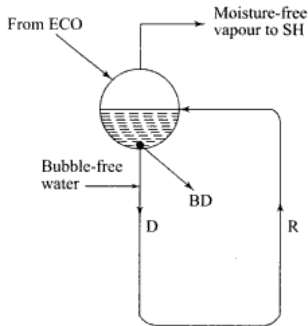
Fig. 6.14 Separation of two-phase mixture in the drum
