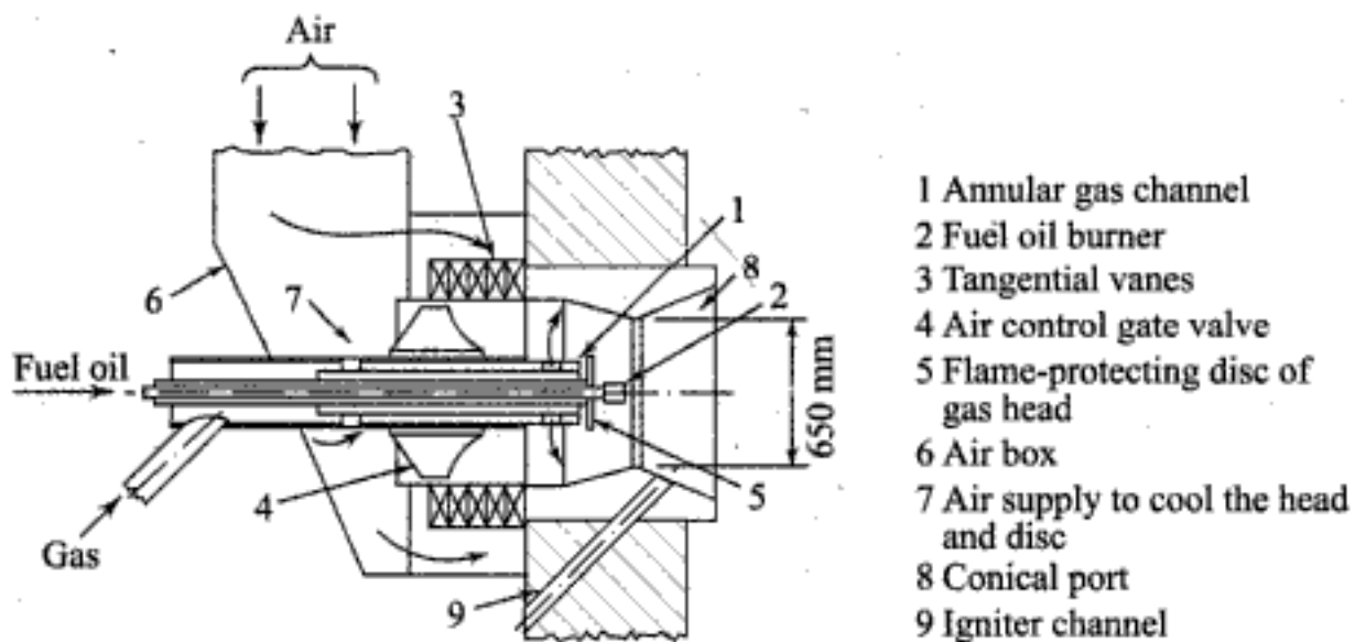
Fig. 5.60 Coaxial gas-fuel oil burner with central gas supply
