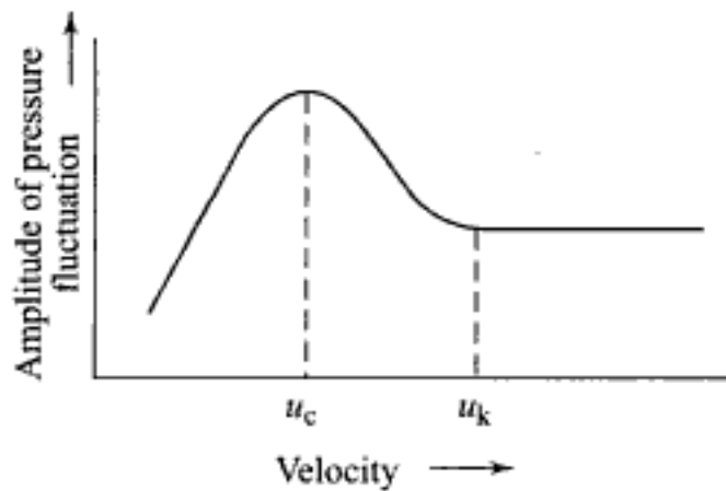
Fig. 5.39 Transition from bubbling to turbulent bed
