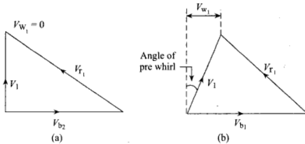
Fig. 11.56 Blade velocity diagrams at blade inlet of a centrifugal compressor (a) Without and (b) With pre-whirl
