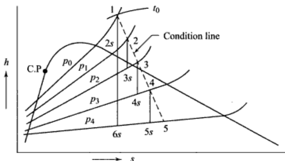
Fig. 7.49 Condition line for a four-stage turbine
