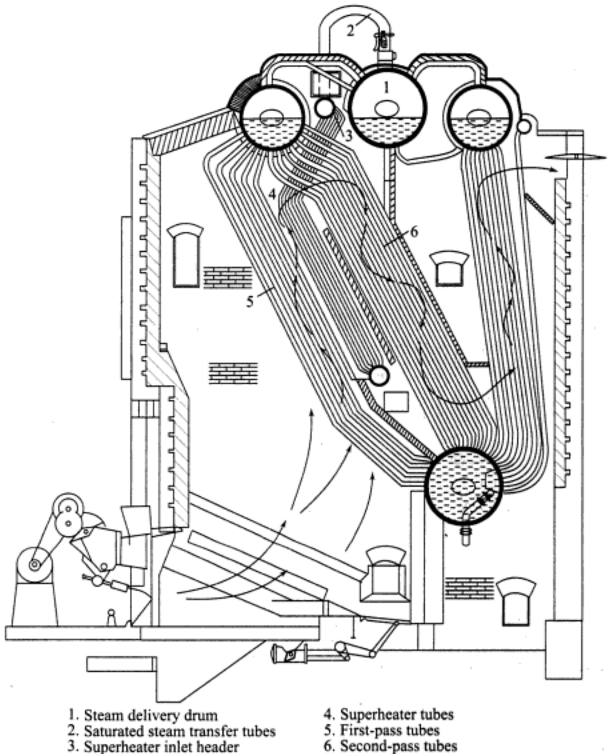
Fig. 6.5 Natural circulation four-drum Stirling boiler
