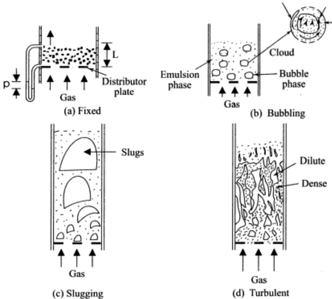
Fig. 5.38 Gas-solid contacting mode changing from one regime to another with the increase of gas velocity
