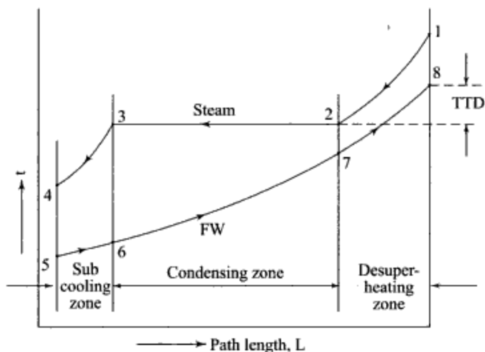
Fig. 8.13(b) Temperature profiles along the path length in a three-zone feedwater heater
