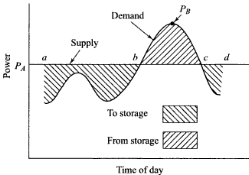
Fig. 12.2 Energy storage with constant thermal input as from fossil or nuclear fuel
