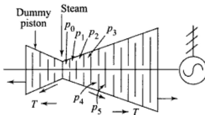
Fig. 7.57 Dummy or balance piston for reaction turbine
