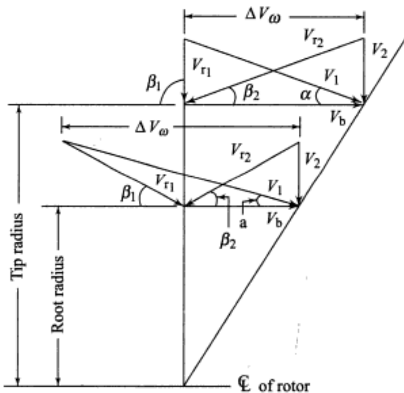
Fig. 7.37 Variation in low-pressure blade angles as influenced by vector diagrams for root and tip velocity
