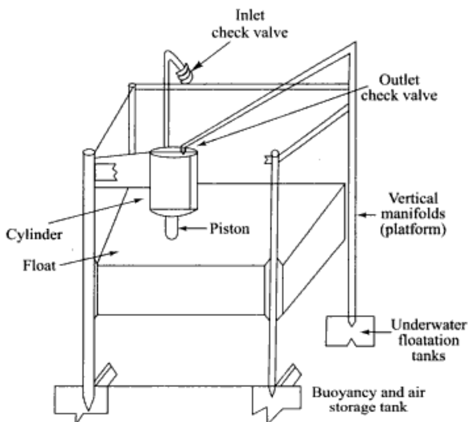
Fig. 14.18 Schematic of a float wave-power conversion machine
