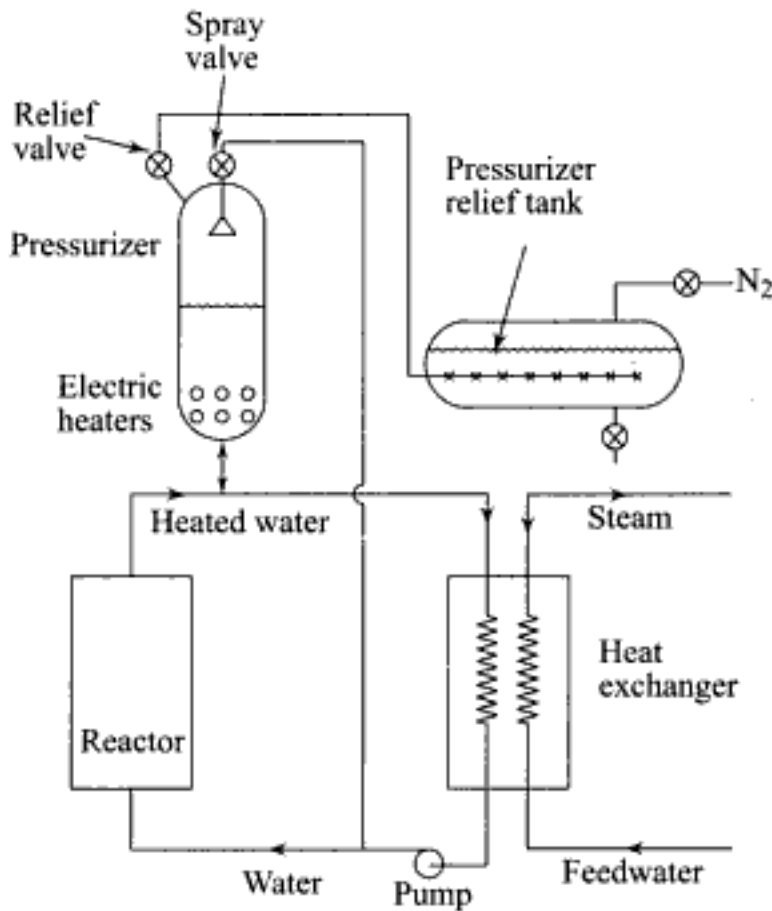
Fig. 9.18 A PWR primary loop with a vapour-type pressurizer system
