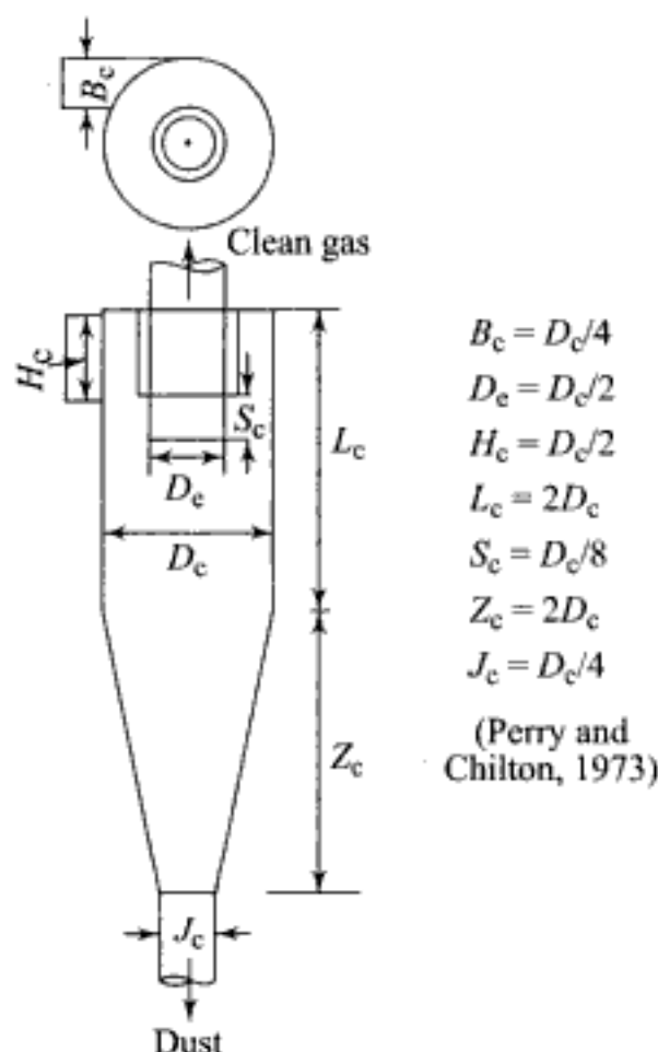
Fig. 6.54 Optimum dimensions for cyclones
