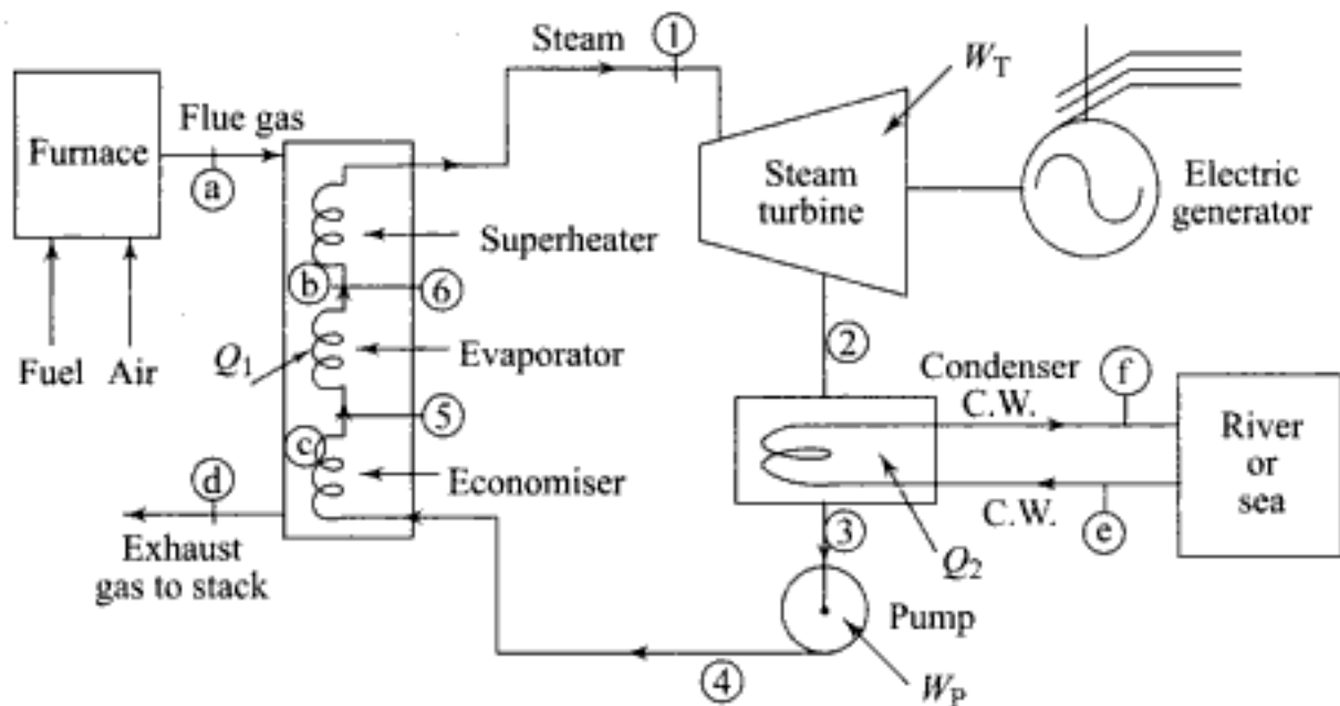
Fig. 2.2 A simple steam plant representing Rankine cycle
