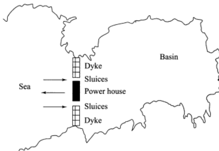
Fig. 14.26 (a) Single basin, single effect tidal power scheme
