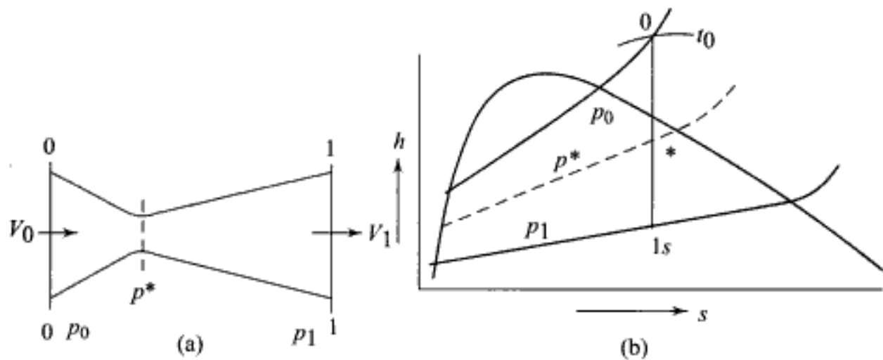
Fig. 7.7 Expansion of steam in a convergent divergent nozzle
