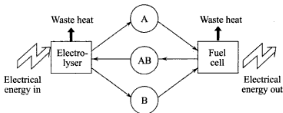
Fig. 12.15 Schematic diagram of an electrochemical fuel cell
