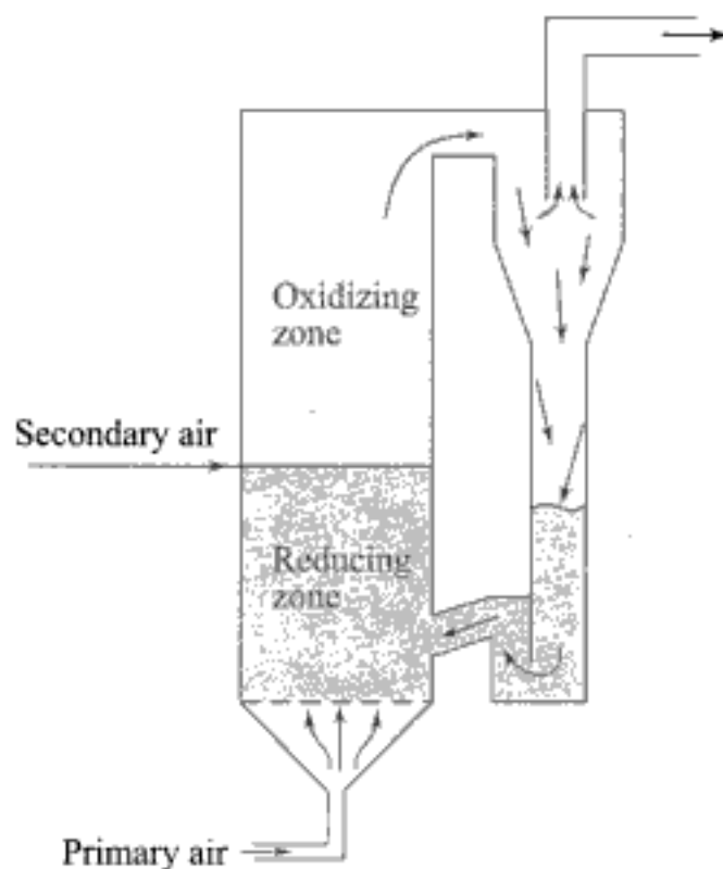
Fig. 6.55 (c) Staged combustion in a CFB
