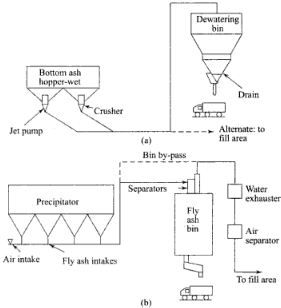
Fig. 6.66 (a) Bottom ash sluice conveyor, (b) Fly ash hydraulic vacuum conveyor
