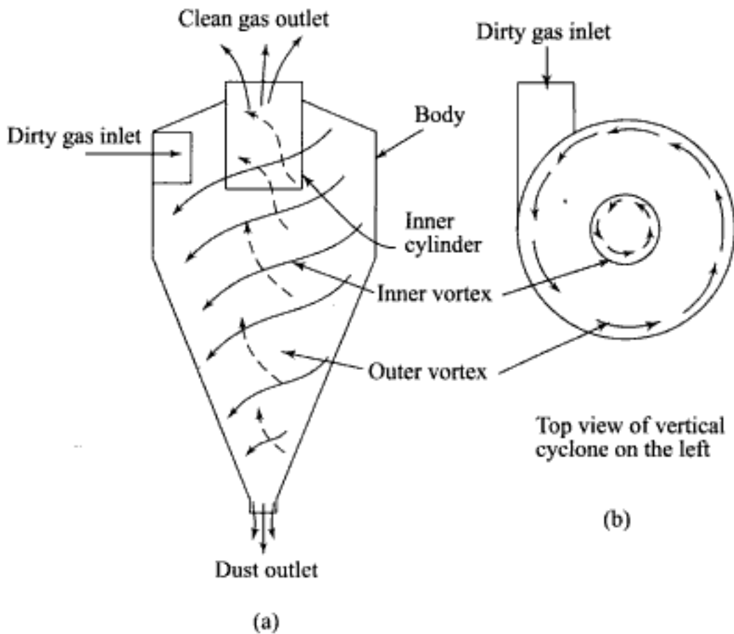
Fig. 6.53 A tangential inlet vertical cyclone separator
