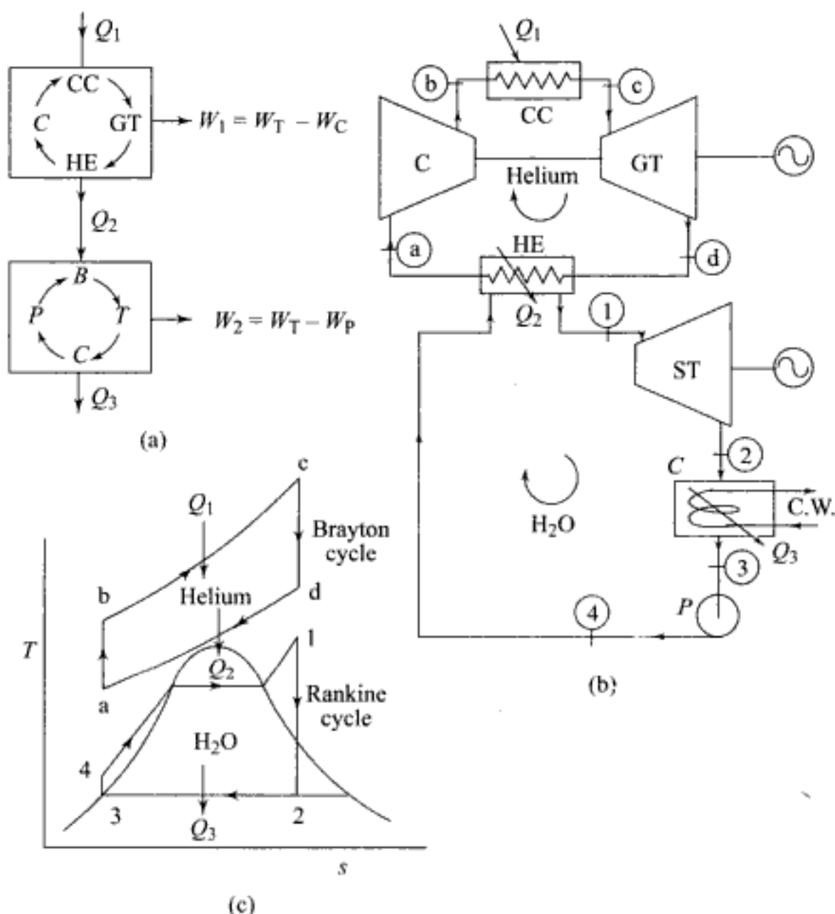
Fig. 3.7 Brayton/Rankine combined cycle plant
