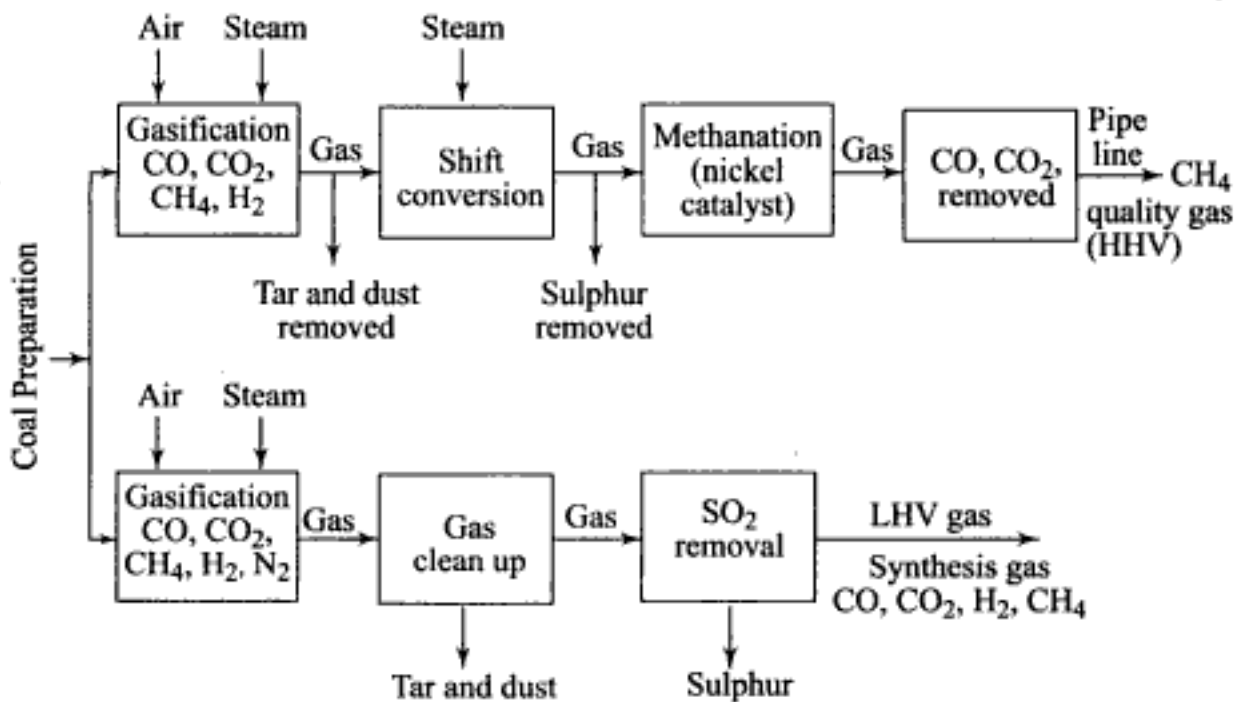
Fig. 4.2 Coal gasification processes
