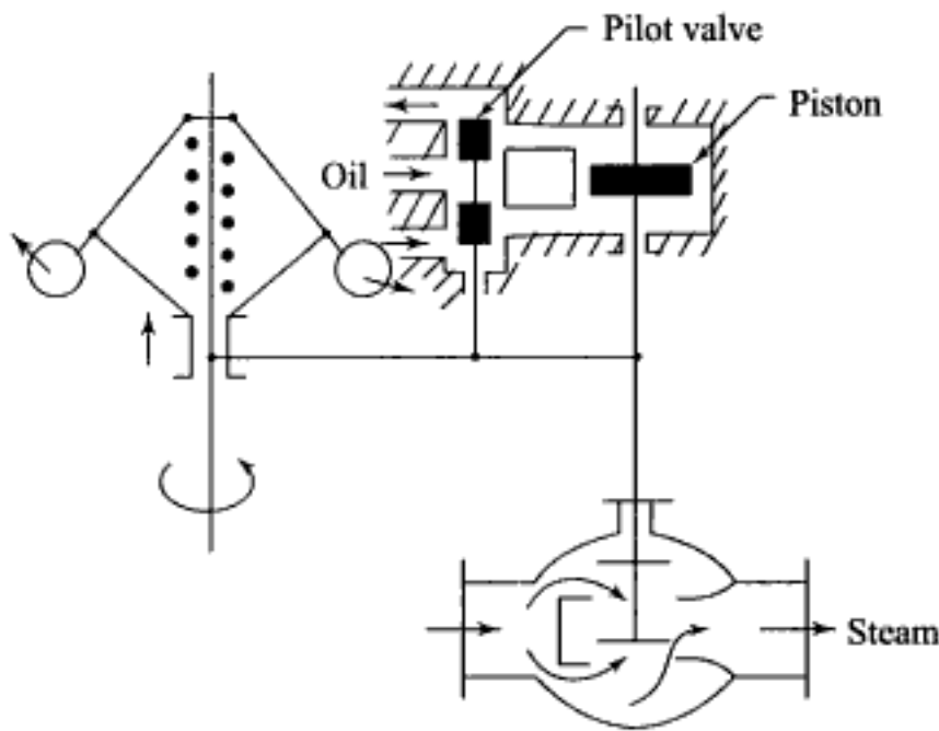
Fig. 7.51 Centrifugal governor with hydraulic power amplifier
