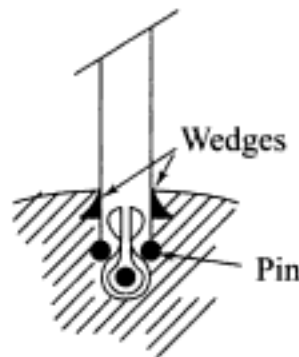
Fig. 7.59 Bulb and shank fastening
