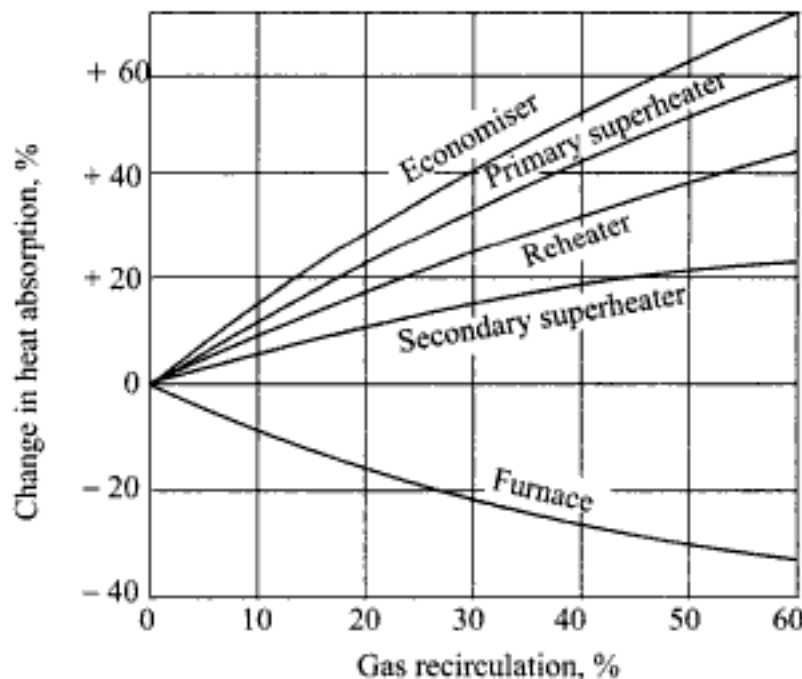
Fig. 6.42 Effect of gas recirculation on the heat absorption pattern at a constant firing rate
