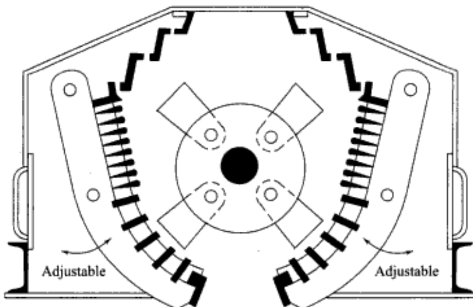
Fig. 5.14 A hammer-mill coal crusher
