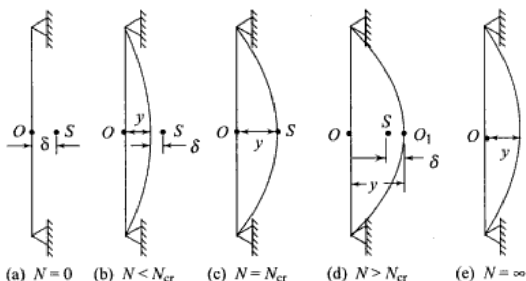
Fig. 7.66 Position of centre of gravity of shaft depending on its rpm
