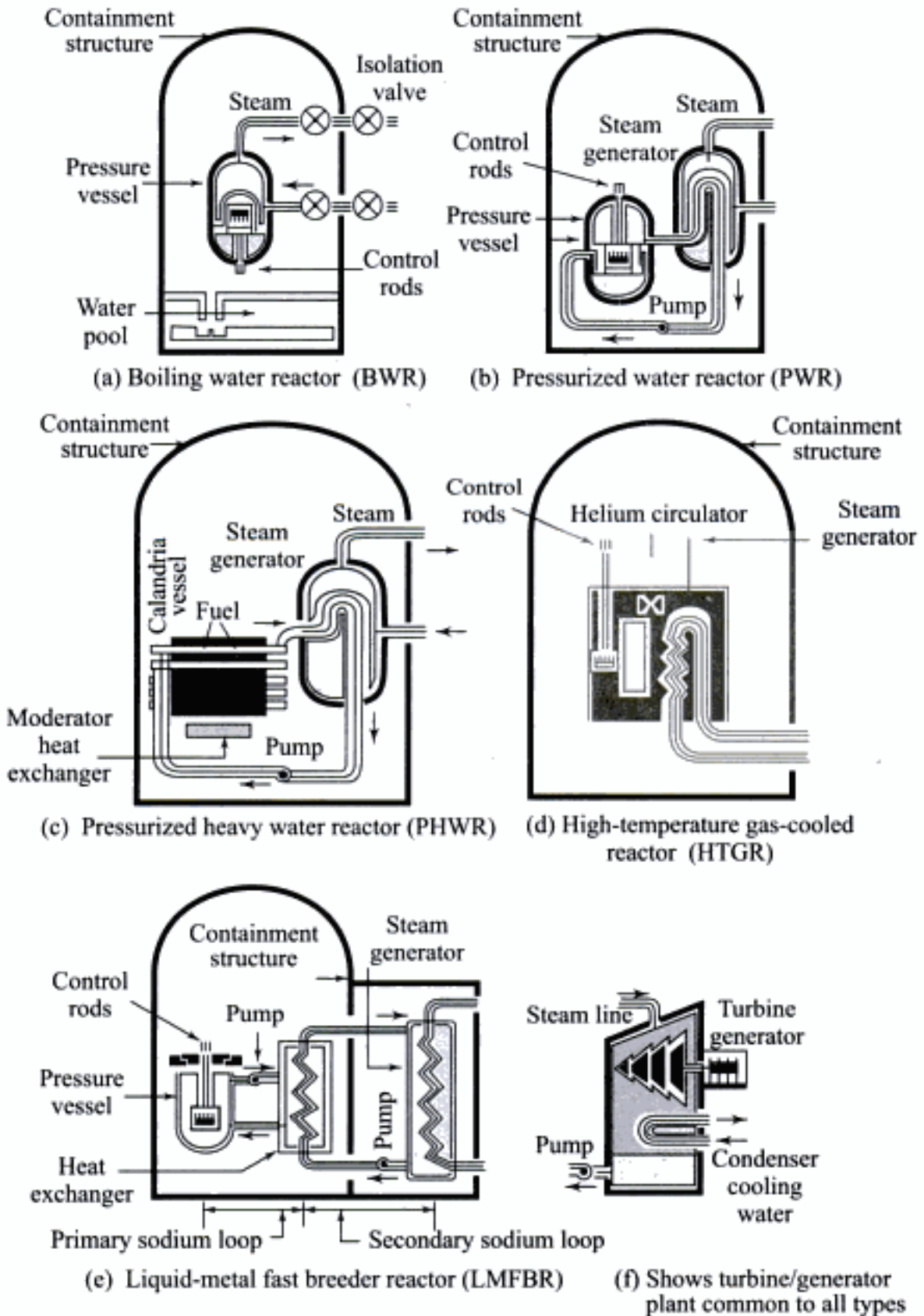
Fig. 9.15 Schematics for nuclear steam supply systems
