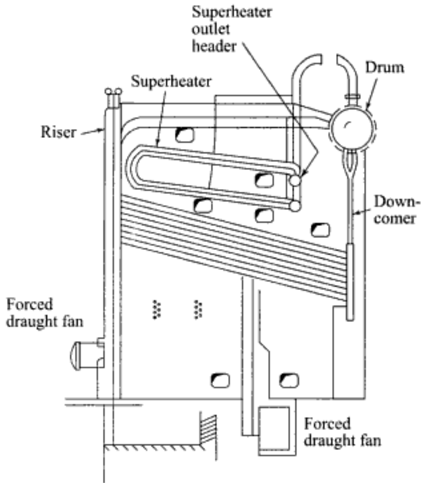
Fig. 6.3 Early water-tube boiler: (b) Cross drum
