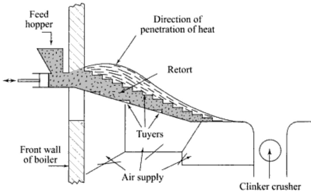
Fig. 5.11 Principle of retort-type stoker
