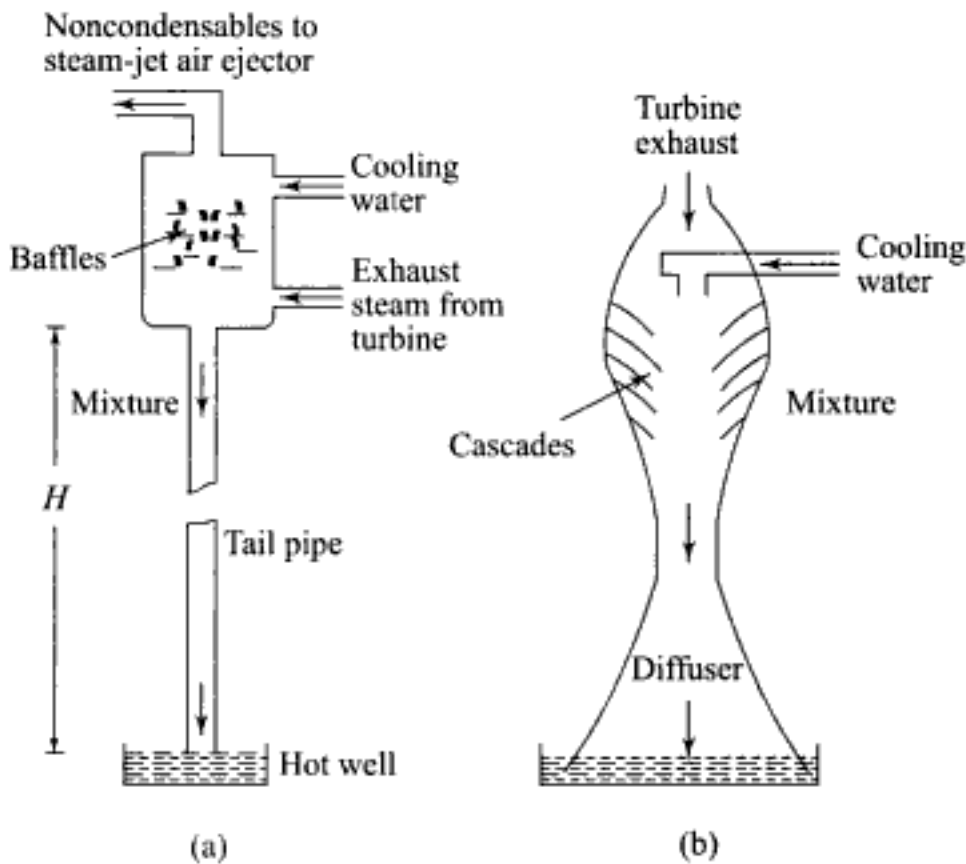
Fig. 8.3 Schematics of direct-contact condensers: (a) barometric, (b) diffuser or jet
