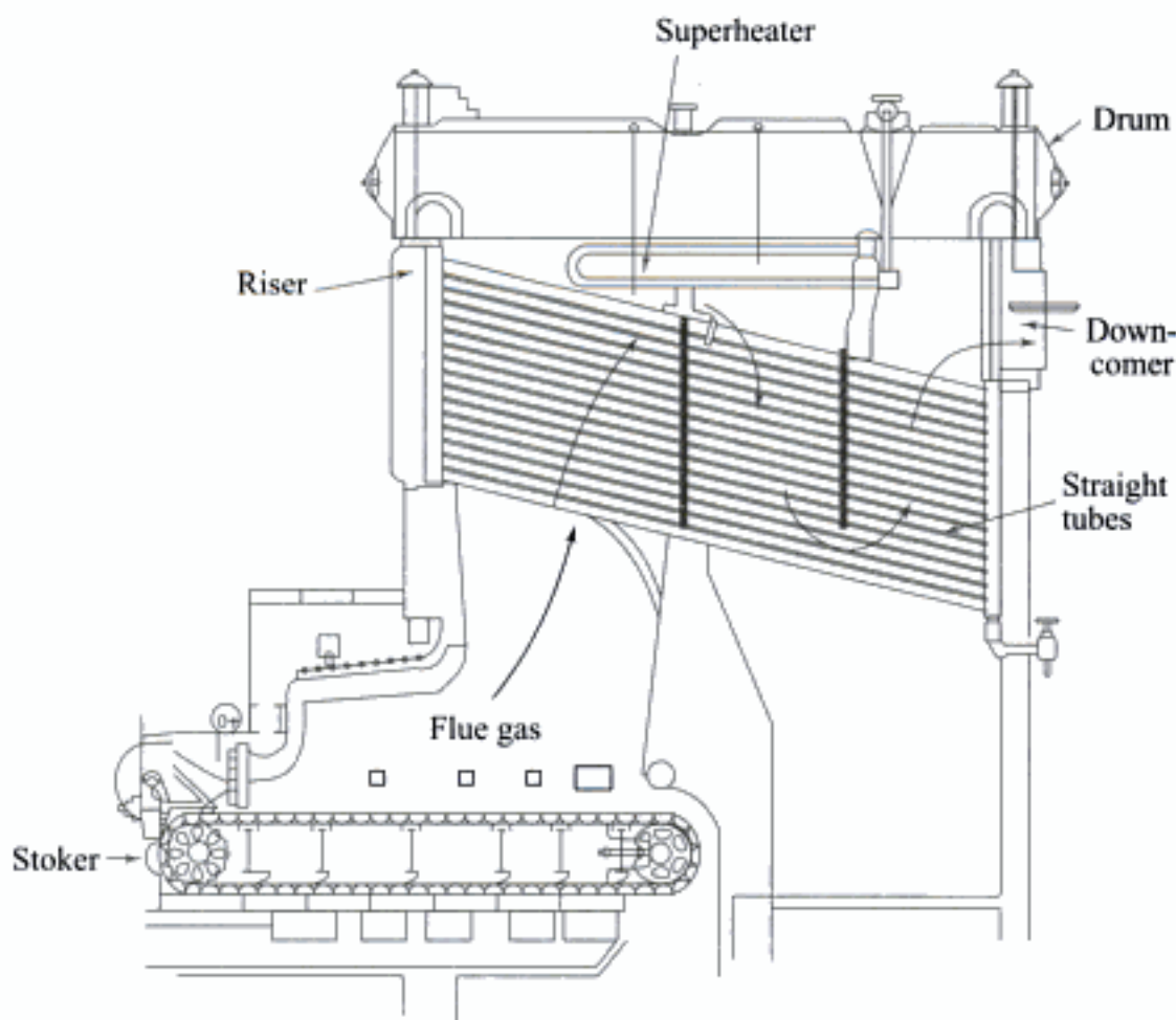
Fig. 6.3 Early water-tube boiler: (a) longitudinal drum
