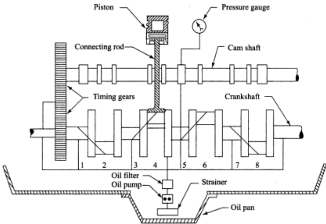
Fig. 11.15 Full pressure lubrication system
