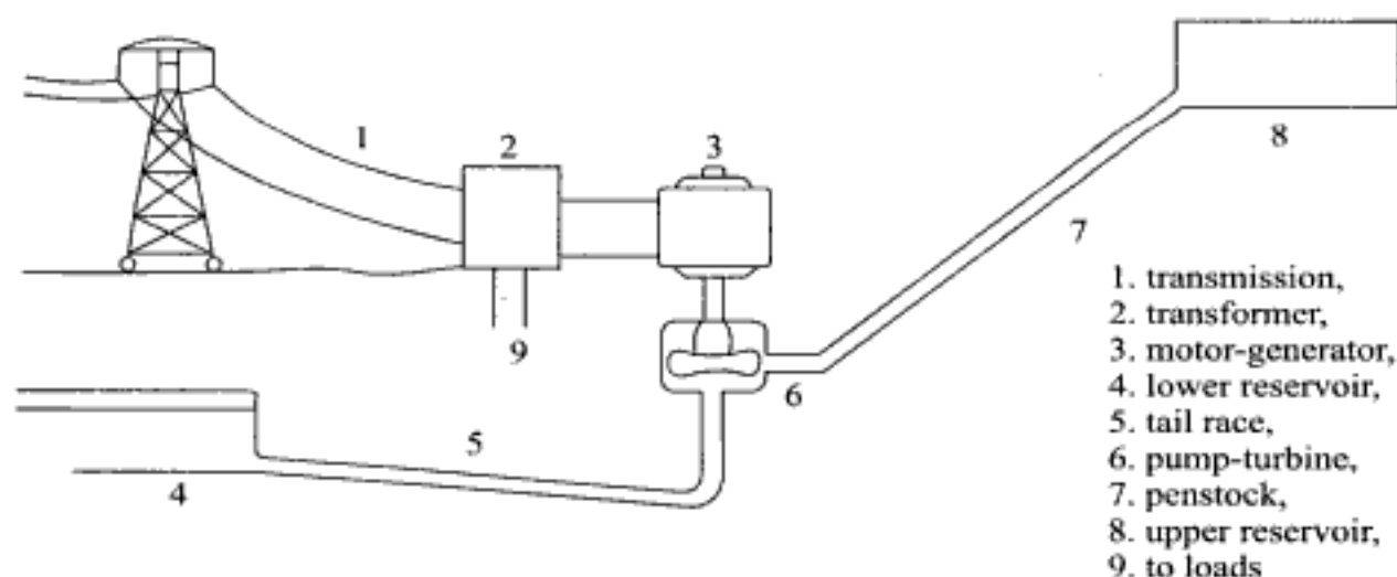
Fig. 12.3 Pumped hydroelectric energy storage
