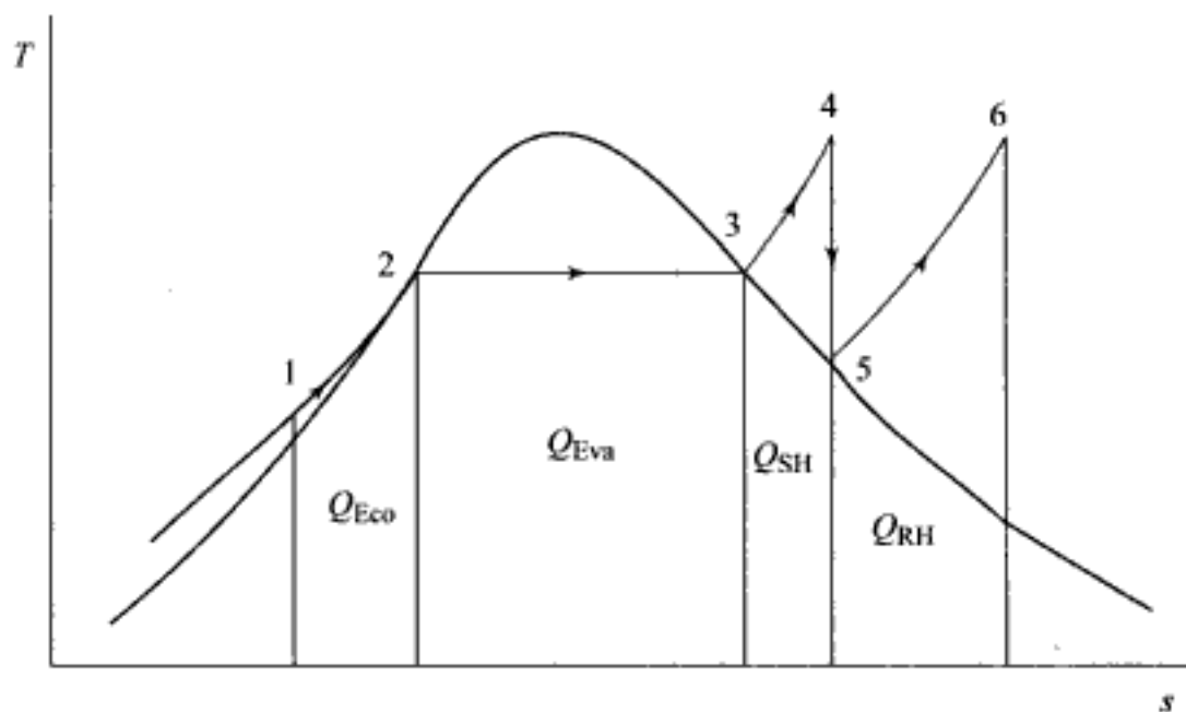
Fig. 6.7(b) Heat absorption in different heat exchangers of a water-tube boiler
