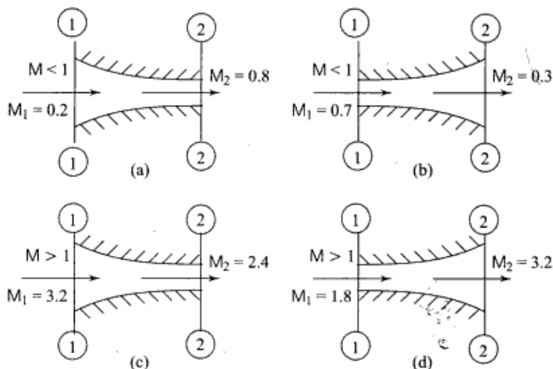
Fig. 7.4 Effect of area change on subsonic and supersonic flow: (a) subsonic nozzle, (b) subsonic diffuser (c) supersonic diffuser, (d) supersonic nozzle
