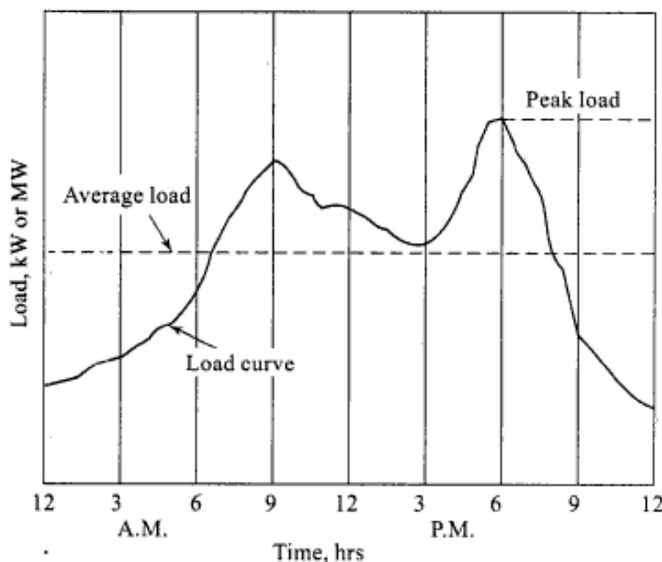
Fig. 1.2 Load curve
