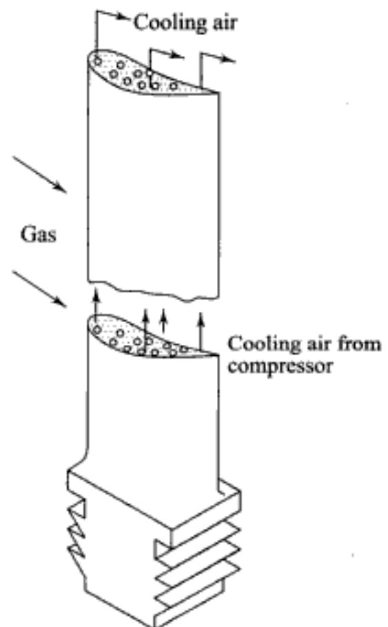
Fig. 11.62 Typical air-cooled gas turbine blade
