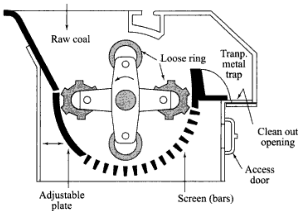
Fig. 5.13 A ring-type coal crusher
