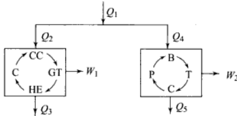
Fig. 3.9 Two cyclic plants operating in parallel
