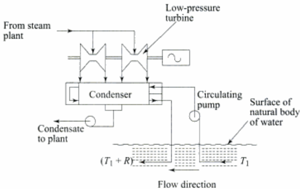
Fig. 8.16 Schematic of a once-through circulating water system
