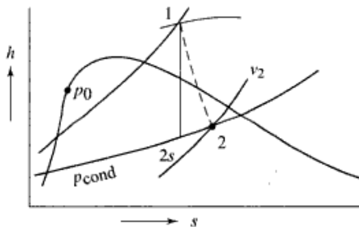
Fig. 7.42 Specific volume at turbine exhaust
