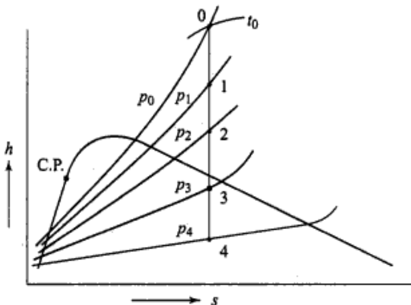
Fig. 7.24 Enthalpy drop per stage in a 4-stage turbine
