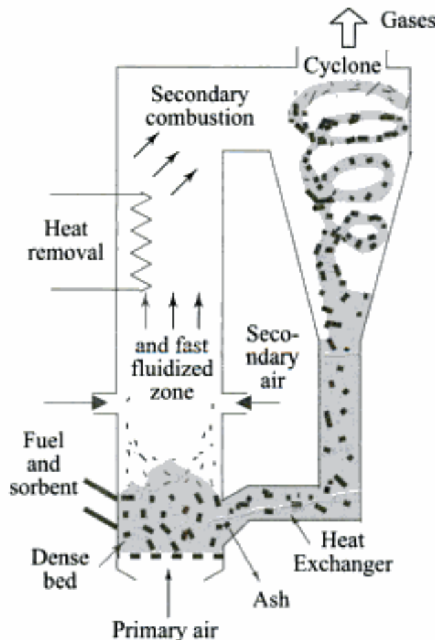
Fig. 5.46 Fast or circulating fluidized bed combustion system
