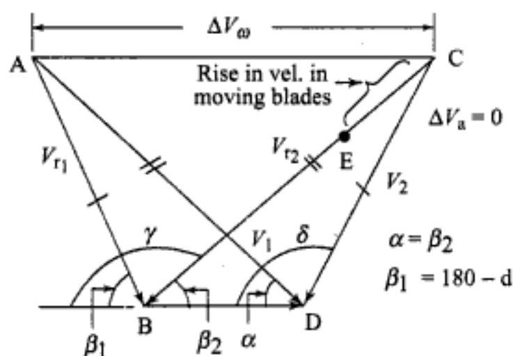
Fig. 7.31 Velocity diagram of a 50% reaction turbine
