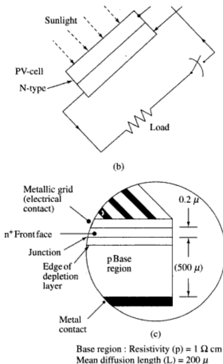
Fig. 14.12 Diagrams of (a) a silicon cell, (b) another view of a PV cell (c) a solar cell
