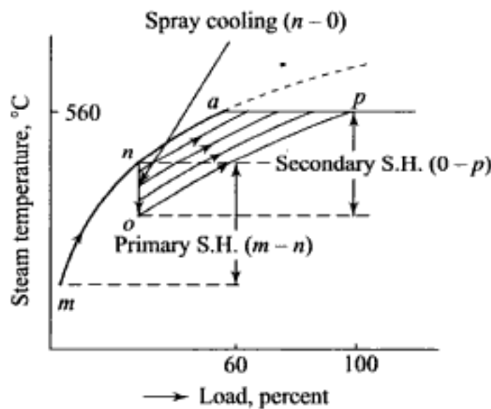
Fig. 6.39 Regulation of spray water results in a flat temperature curve
