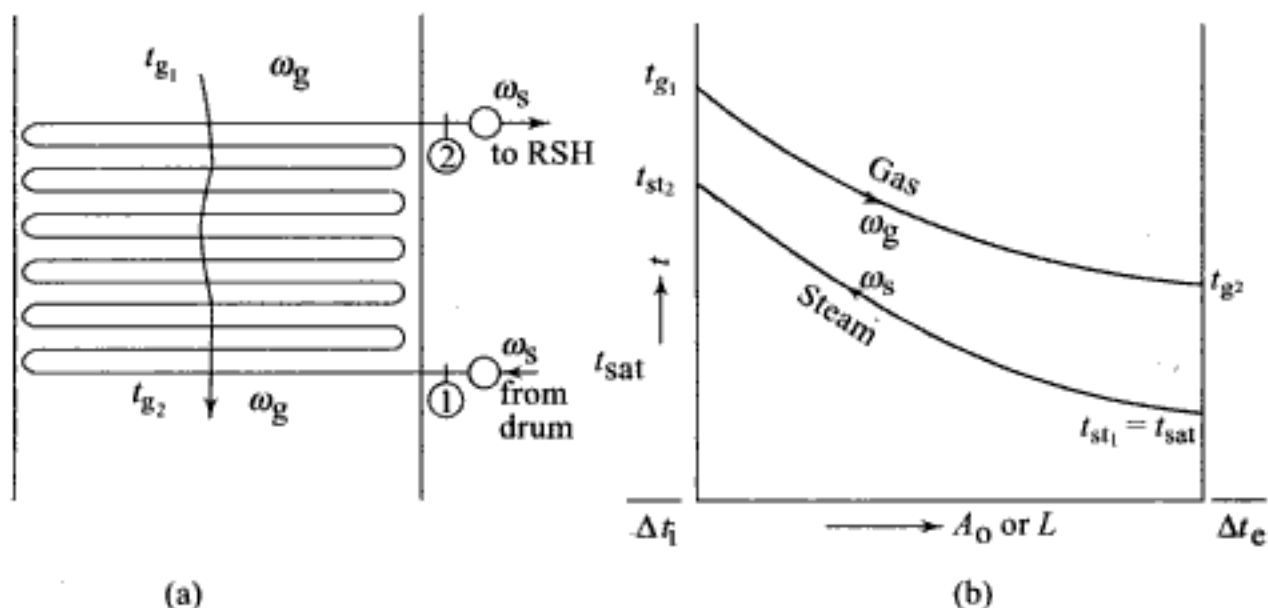
Fig. 6.28 Convective superheater coil and the temperature profiles
