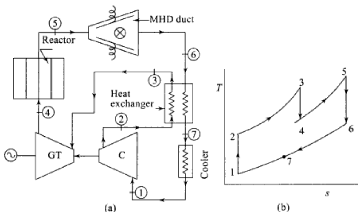
Fig. 13.6 Closed cycle MHD-gas turbine power plant
