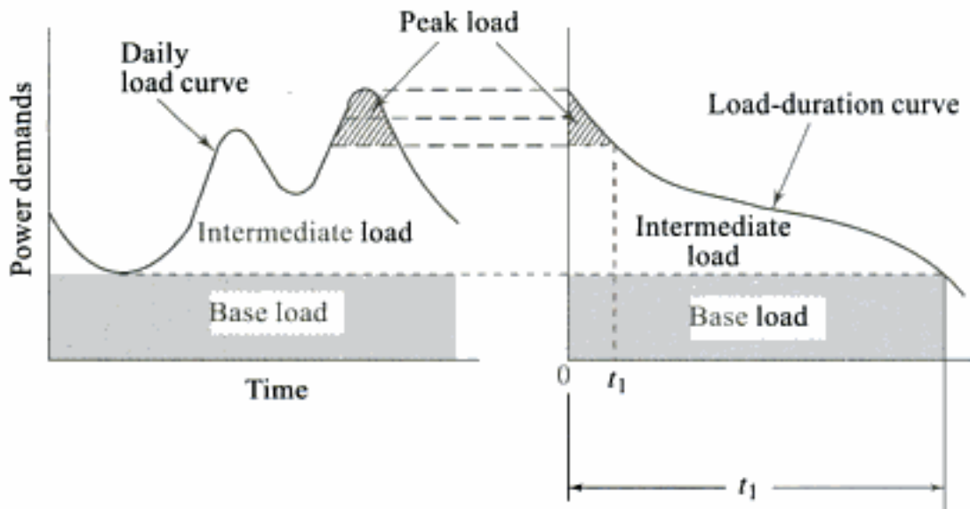
Fig. 1.5 Construction of the load-duration curve
