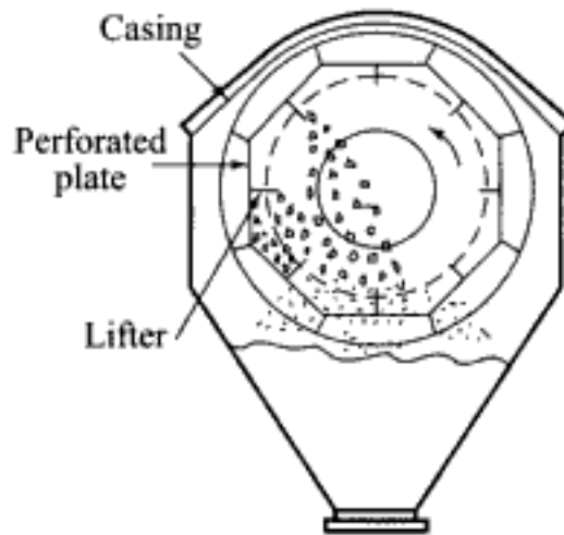
Fig. 5.15 A Bradford breaker
