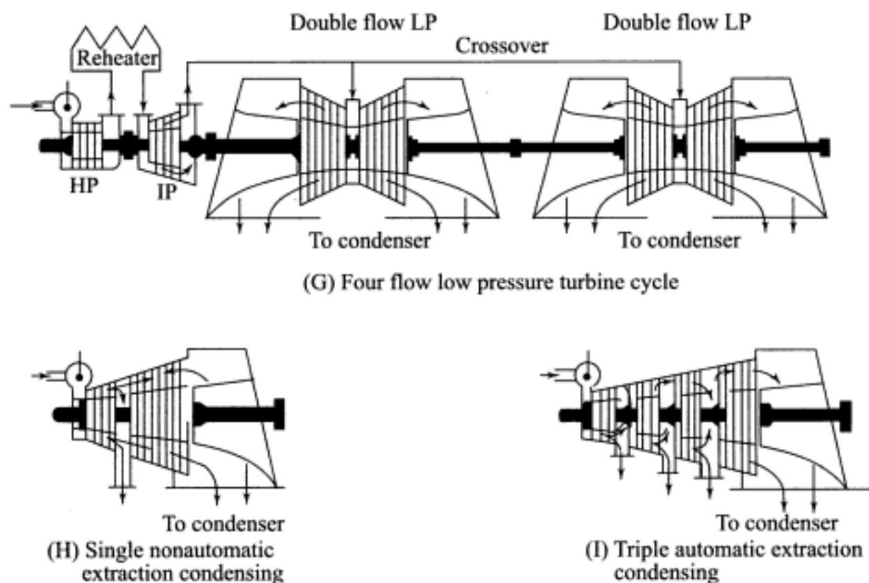
Fig. 7.1 (b) Turbine Types
