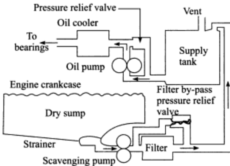
Fig. 11.17 Full flow dry sump lubrication
