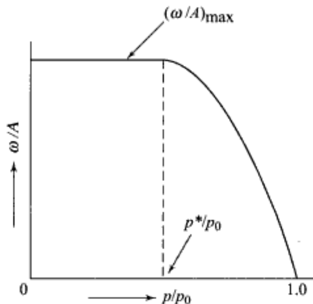
Fig. 7.6 Choking of nozzle
