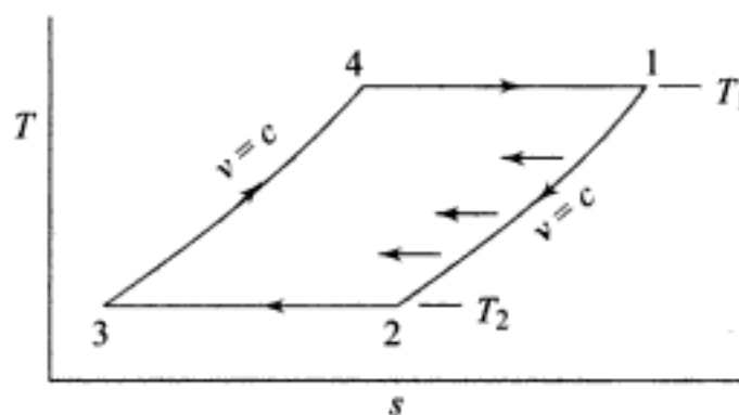
Fig. 2.17 Regenerative Stirling cycle with reversible heat transfer between processes 1–2 and 3–4
