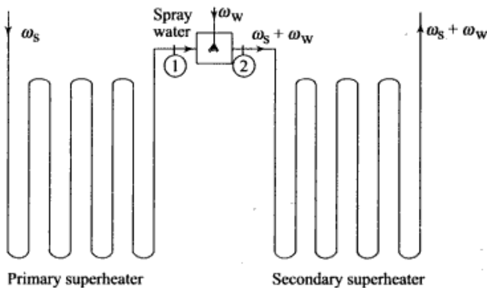
Fig. 6.38 Spray-type desuperheater
