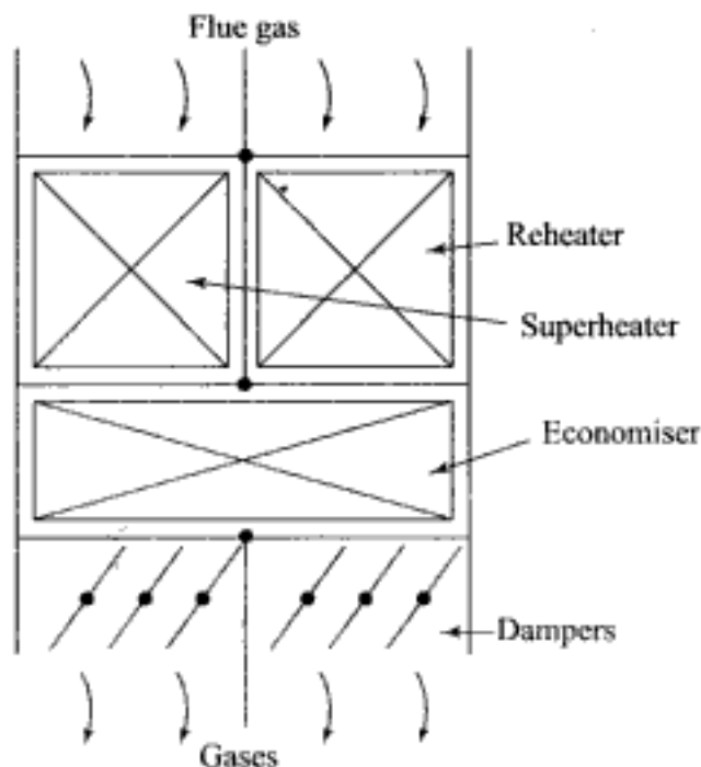
Fig. 6.40 Steam superheat by gas by-pass or damper control
