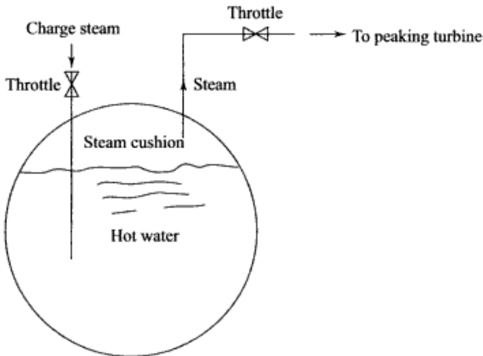
Fig. 12.21 Variable pressure accumulator
