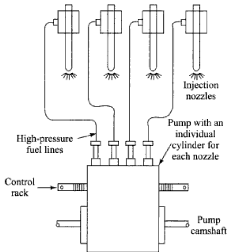
Fig. 11.6 Individual pump injection system
