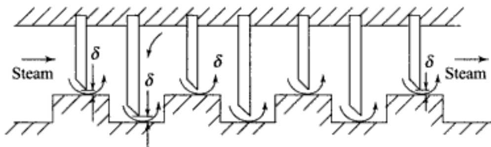
Fig 7.46 Stepped labyrinth seals
