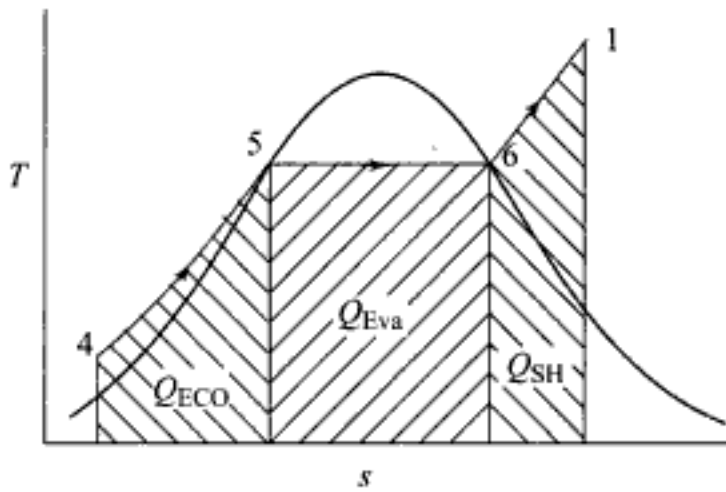
Fig. 2.4 Fraction of total heat transfer absorbed in the economiser, evaporator and superheater
