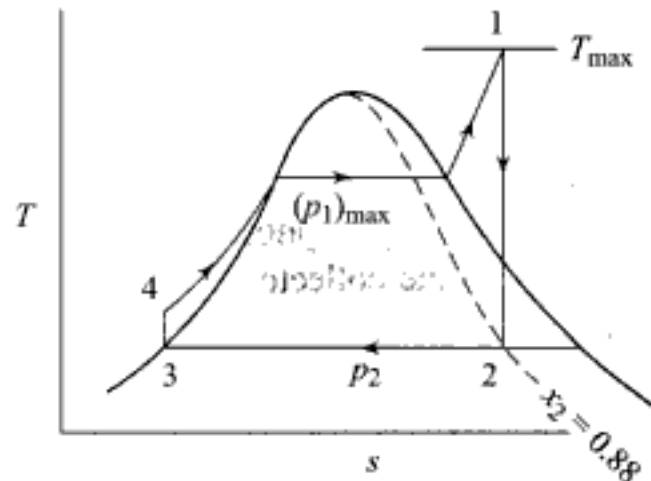
Fig. 2.13 Fixing of maximum steam pressure at turbine inlet
