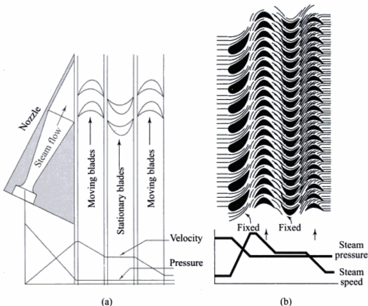
Fig. 7.25 (a) A two-row Curtis stage, (b) Pressure and velocity variation in a two-row Curtis stage
