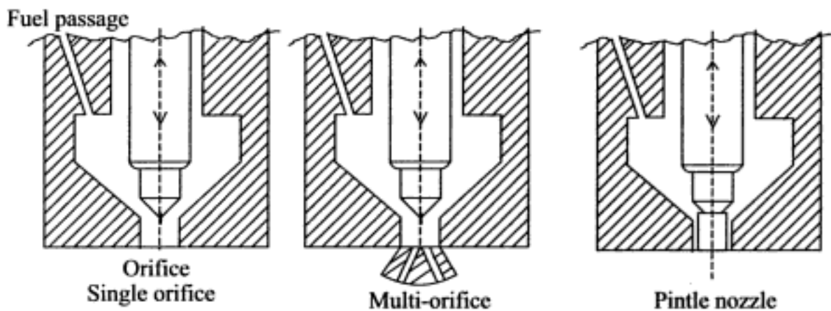
Fig. 11.10 Various types of nozzles
