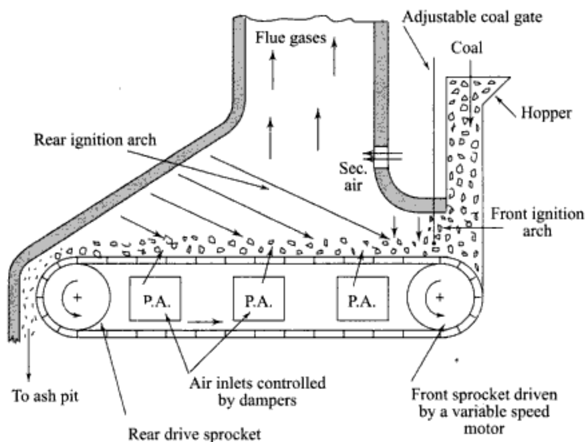
Fig. 5.9 (a) Travelling grate stoker moving like an endless belt carrying the fuel bed from right to the left
