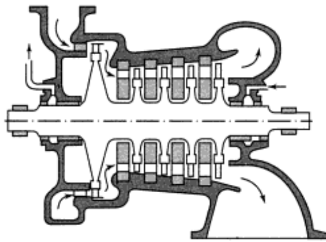
(a) Impulse turbine
