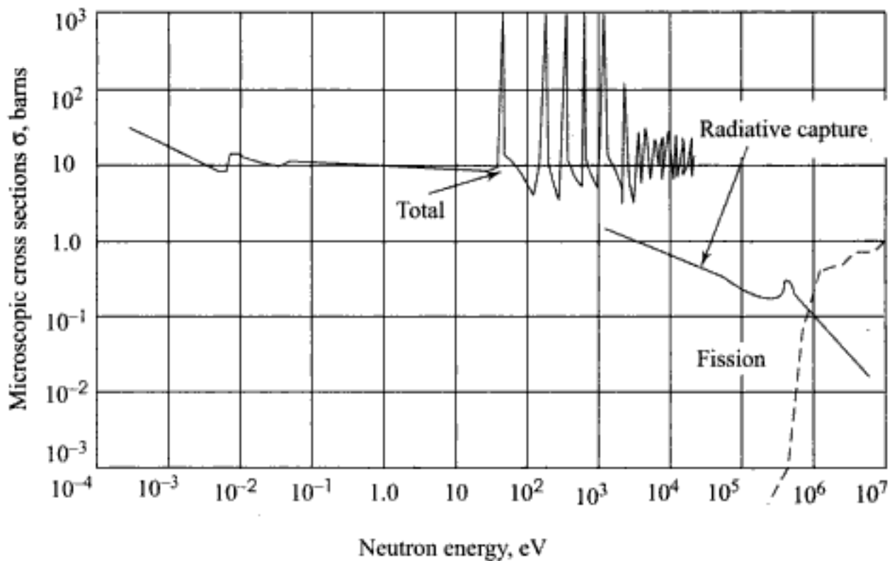
Fig. 9.9 Neutron cross-section for U-238
