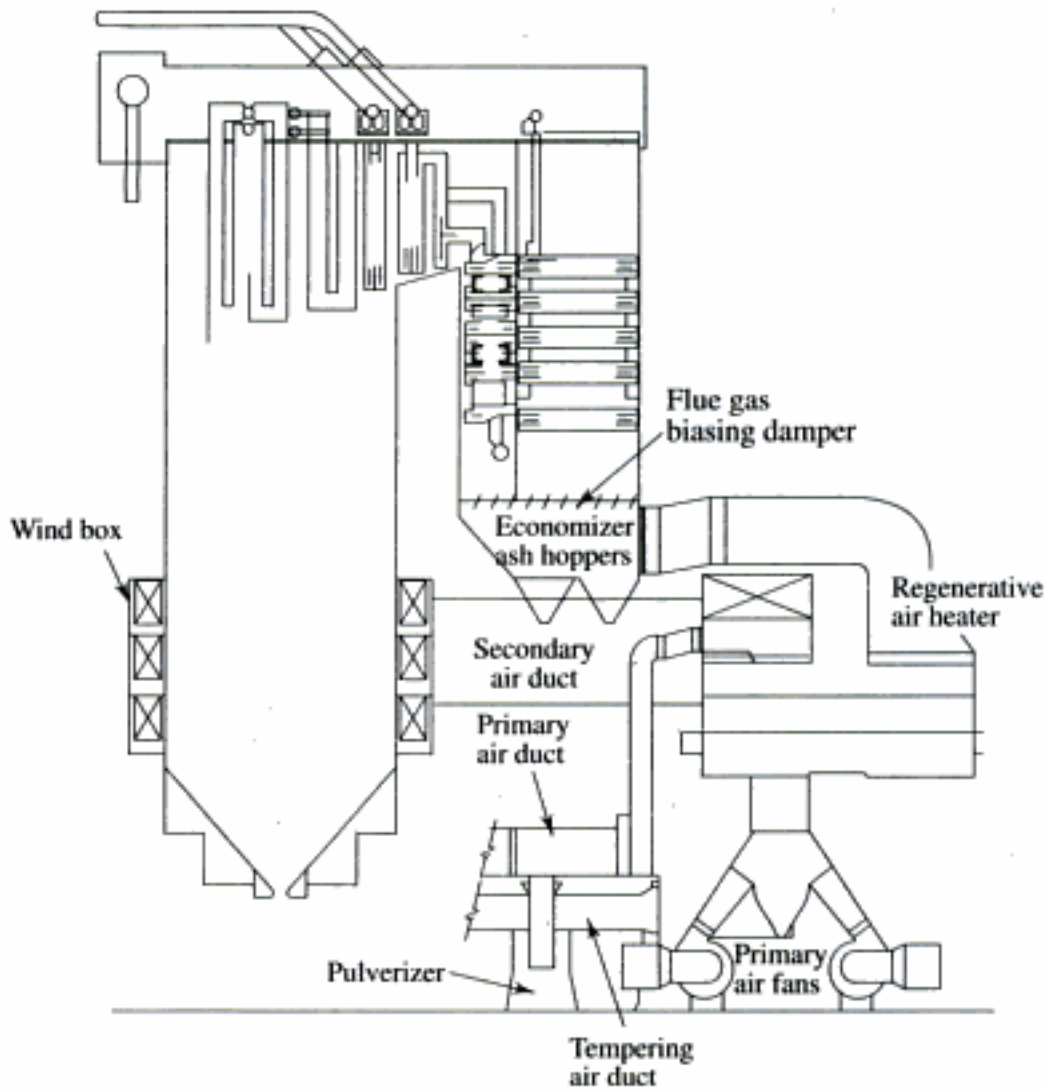
Fig. 6.6 (b) Typical wall-fired boiler cross-section with divided convection pass
